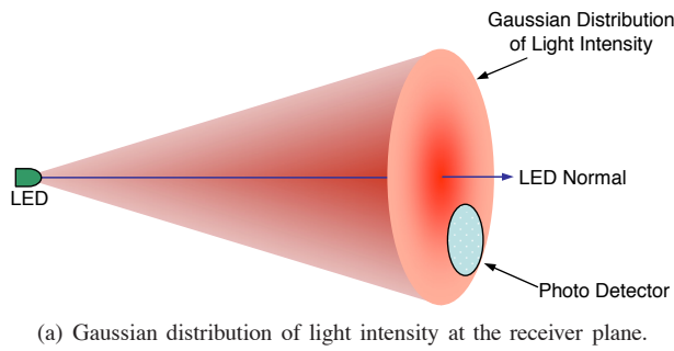
(a) Gaussian distribution of light intensity at the receiver plane.
