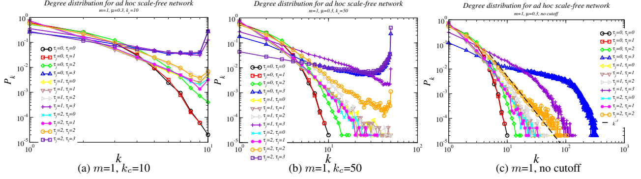
Figure 3. Degree distributions over ad-hoc nodes (i.e., \mu=0.3 ): P(k) for various networks generated by our framework for varying \tau_j and \tau_l .
