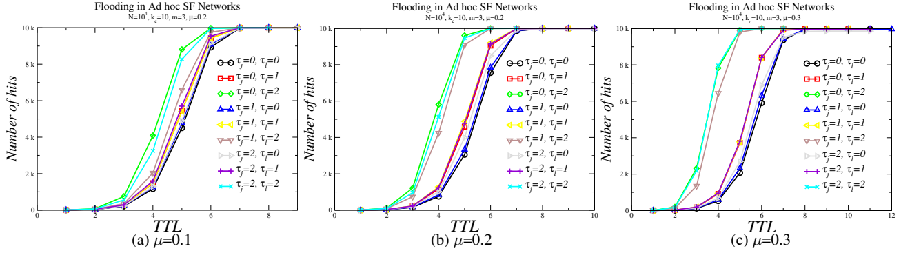
Figure 5. Flooding (FL) performance over topologies generated with k_c=10 and m=3 .
