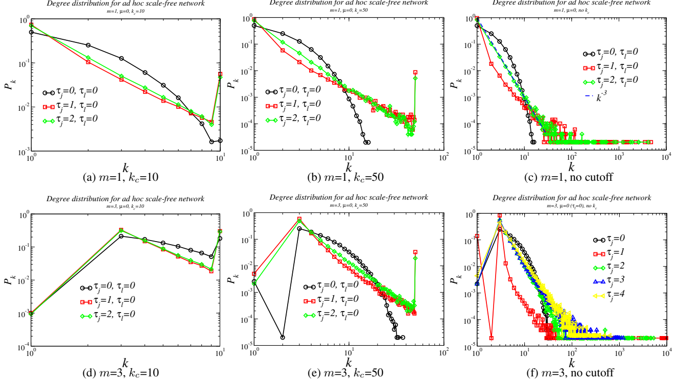
Figure 2. Degree distributions when there is no ad-hocness (i.e., \mu=0 ): P(k) for various networks generated by our framework for varying \tau_j .
