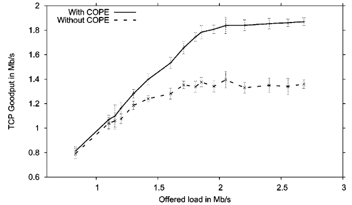
Fig. 9. COPE provides 38% increase in TCP goodput when the testbed topology does not contain hidden terminals.
