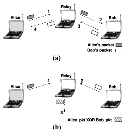
Fig. 1. A simple example of how COPE increases the throughput. It allows Alice and Bob to exchange a pair of packets using 3 transmissions instead of 4 (numbers on arrows show the order of transmission). (a) Current approach. (b) COPE.
