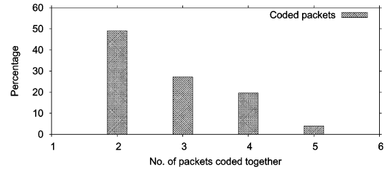
Fig. 12. Distribution of number of packets coded together in the test bed at the peak point of Fig. 10.
