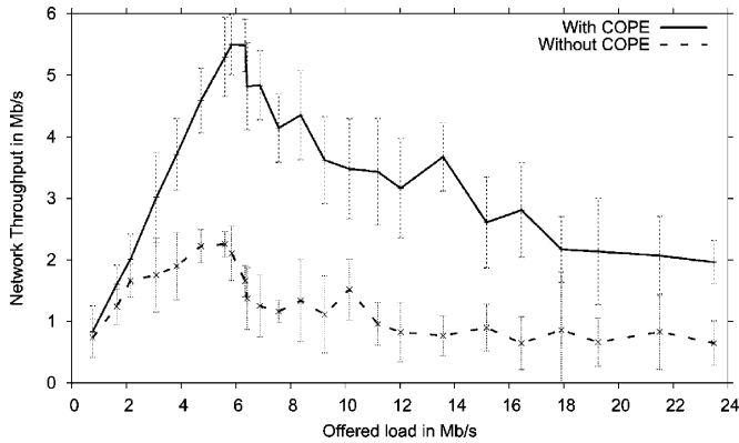
Fig. 10. COPE can provide a several-fold (3–4 \times ) increase in the throughput of wireless ad hoc networks. Results are for UDP flows with randomly picked source-destination pairs, Poisson arrivals, and heavy-tail size distribution.
