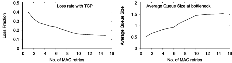
Fig. 8. End-to-end loss rate and average queue size at the bottlenecks for the TCP flows in the testbed. Loss rates are as high as 14% even after 15 MAC retries; TCP therefore performs poorly. The queues at the bottlenecks almost never build up resulting in very few coding opportunities and virtually no gains.
