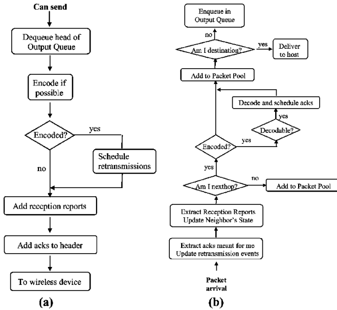
Fig. 5. Flow chart for our COPE Implementation. (a) Sender side. (b) Receiver side.
