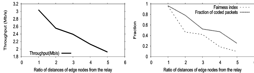
Fig. 14. Effect of unequal channel qualities on coding opportunities and throughput gain in the Alice-and-Bob topology. COPE aligns the fairness and efficiency objectives. Increased fairness increases coding opportunities and hence improves the aggregate throughput.
