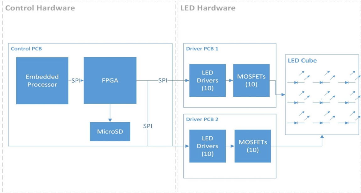
Figure 5.2: LED Cube Hardware Block Diagram
