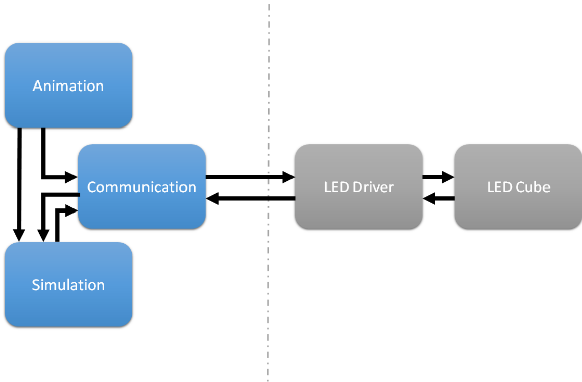
Figure 4.10: Software Architecture
