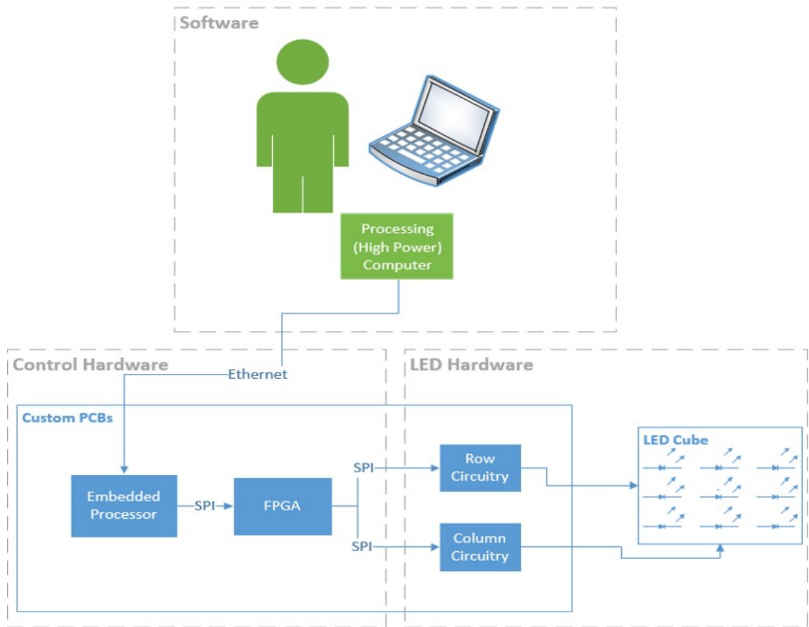
Figure 5.1: LED Cube Block Diagram
