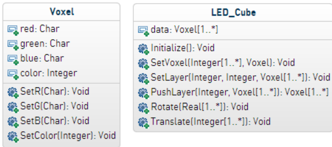
Figure 4.15: LED Cube Class Diagrams
