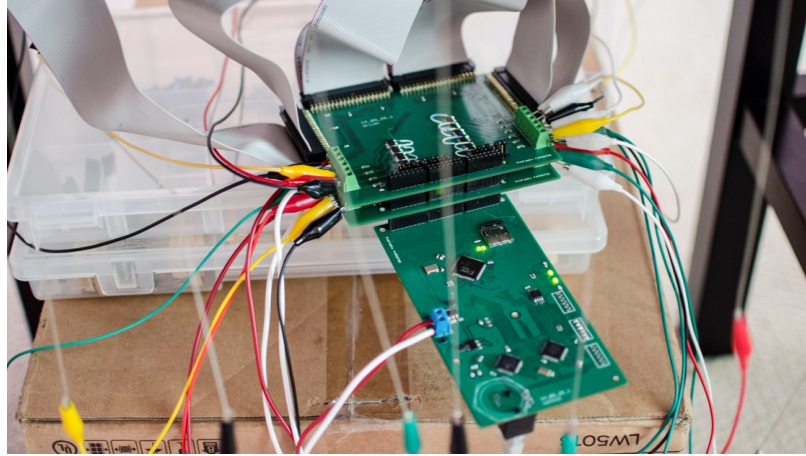
Figure 7.2: Integrated PCBs
