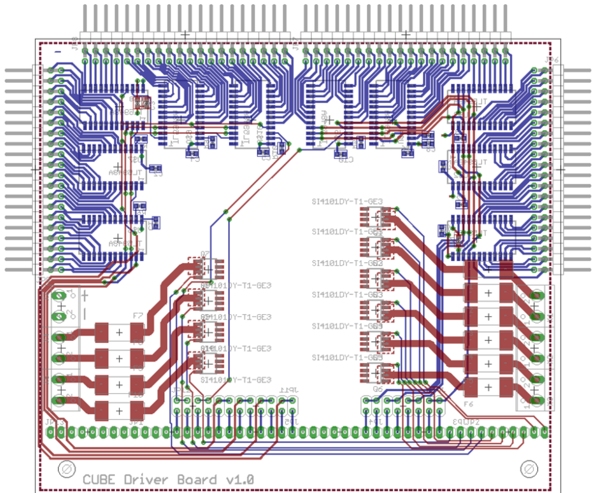
Figure 4.22: Driver PCB
