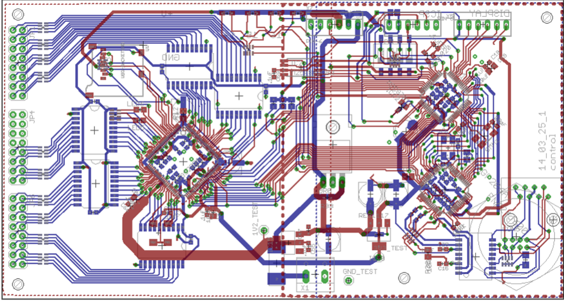
Figure 4.21: Control PCB
