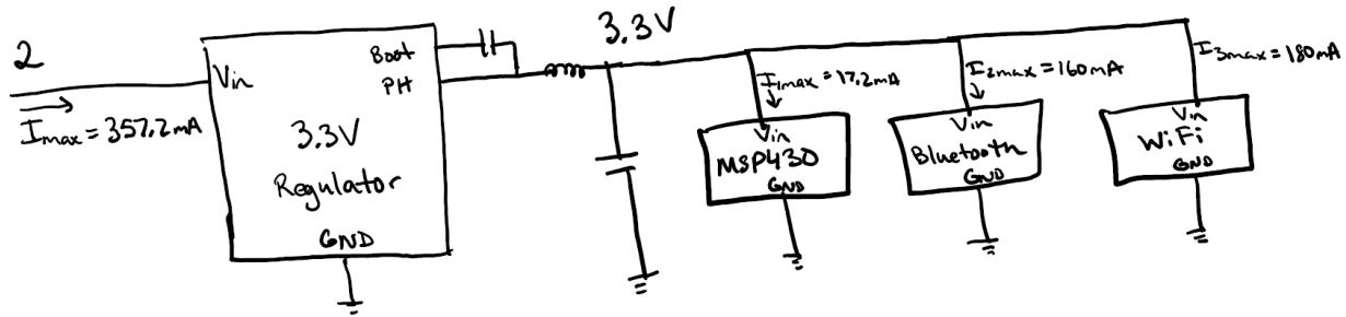
Figure 4.7.1.C – Subsystem 2 (3.3V)
