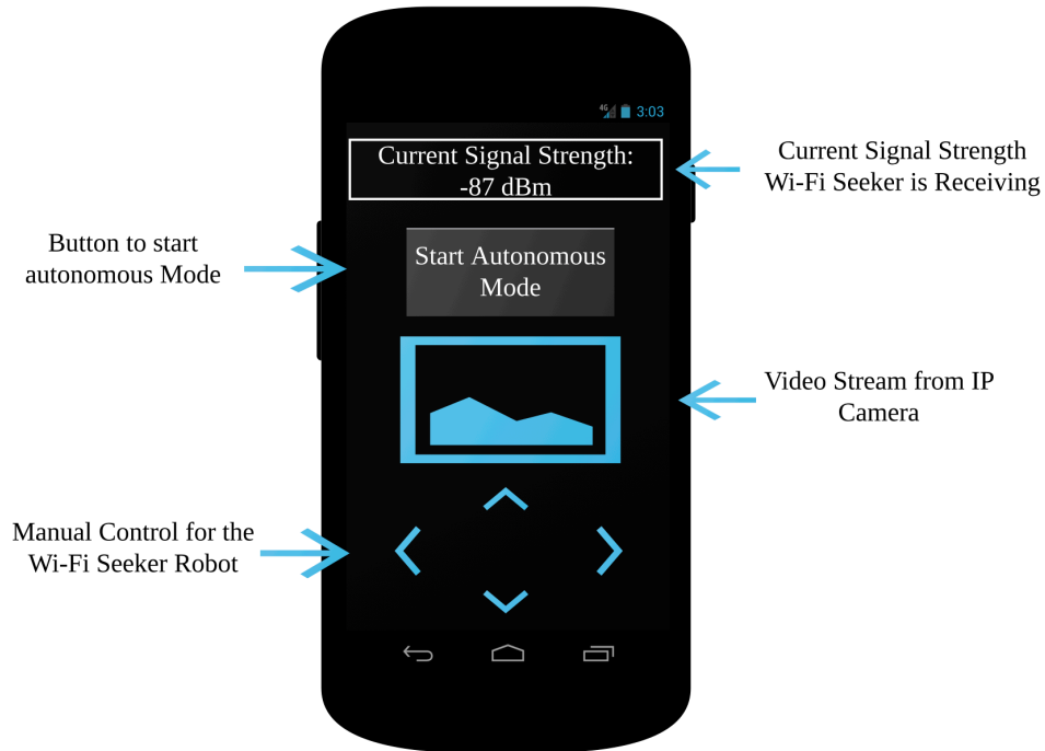
Figure 4.4.C - Android Main Activity: Manual Mode
