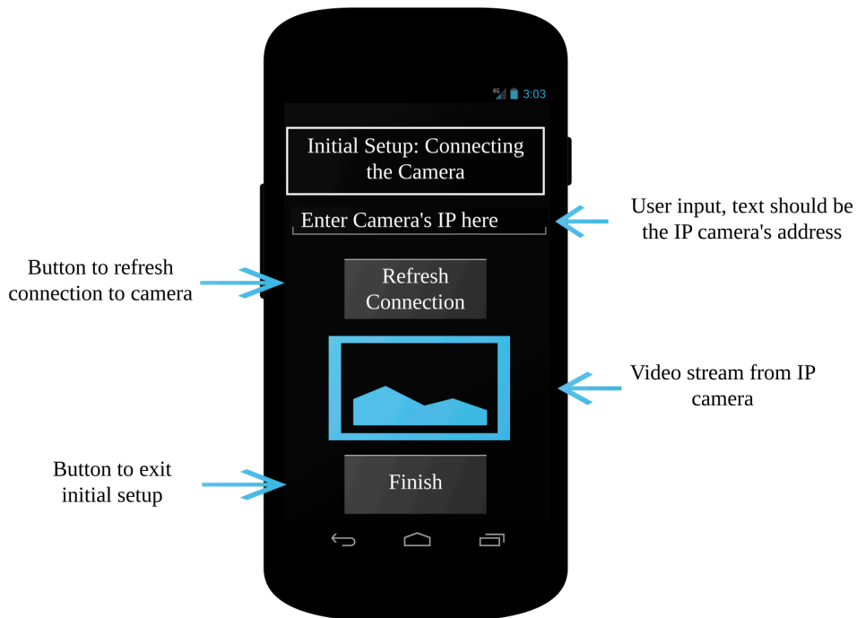
Figure 4.4.B - Android Initial Camera Setup
