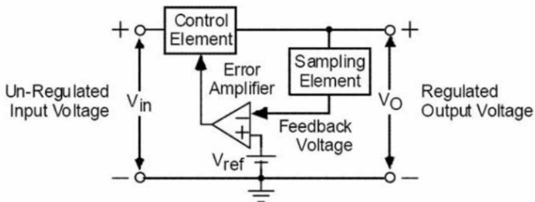
Figure 3.2.17.A - Linear Voltage Regulator Circuit Permission Pending
