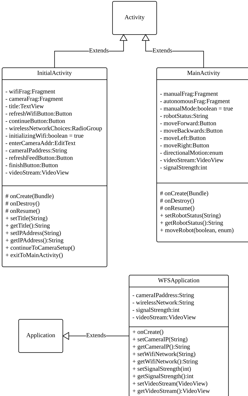
Figure 5.2.2.A - Android UML Class Diagram
