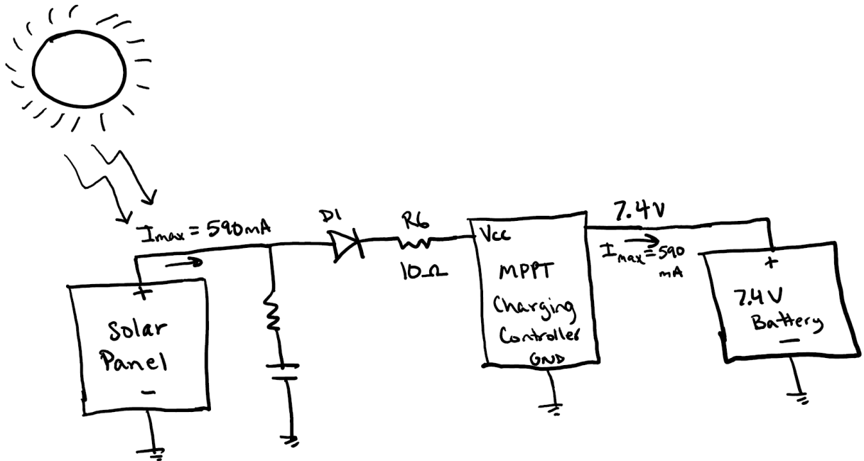
Figure 4.7.2.A – Connecting the Solar Panel to the Charge Controller and Battery
