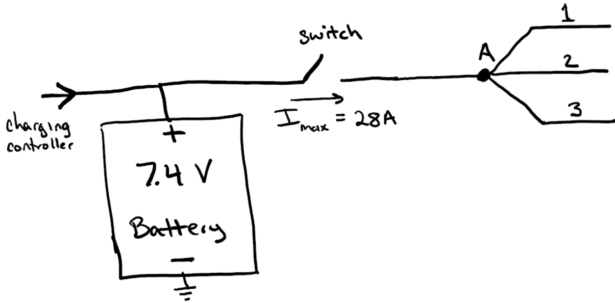
Figure 4.7.1.A – Splitting the Power into Three Subsystems
