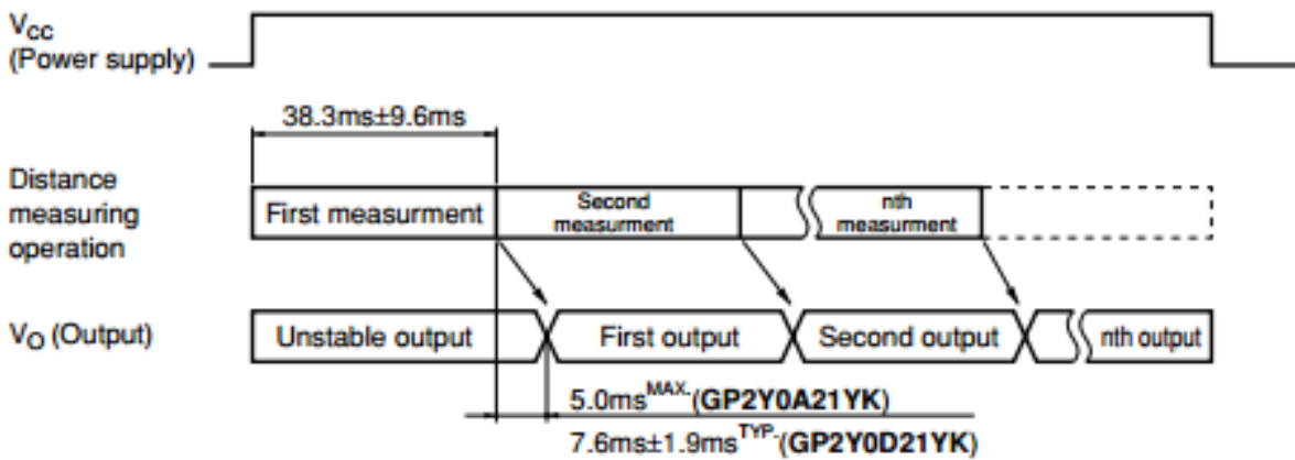
Figure 5.1.6.B - Sharp GP2Y0A21YK Timing Diagram
