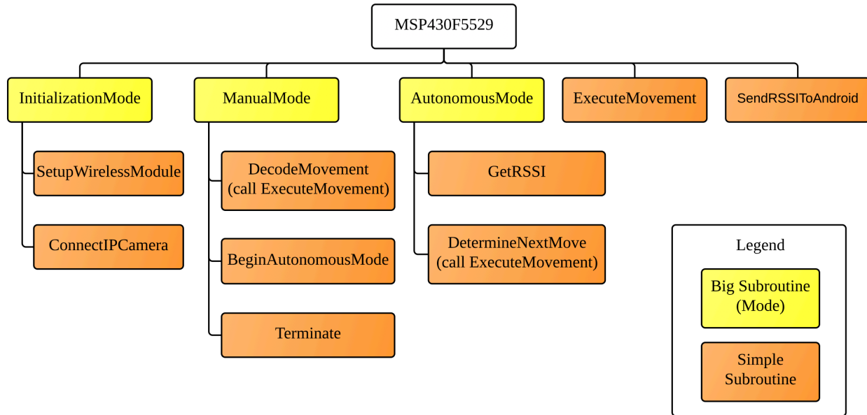
Figure 6.3.2.A - MSP430F5529 Code Structure and Key Subroutines
