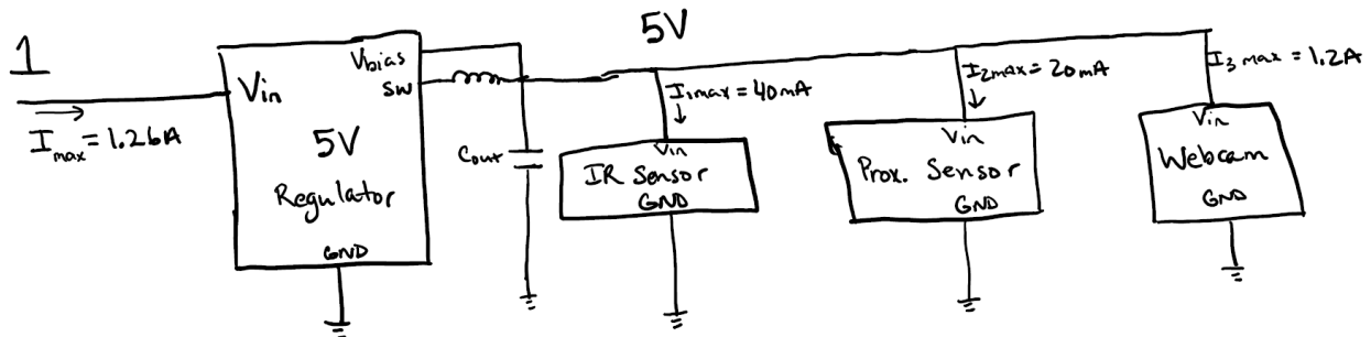
Figure 4.7.1.B – Subsystem 1 (5V)
