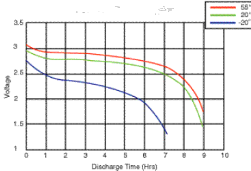
Figure 3.2.16.A - Battery Voltage Over Discharge Time At Various Temperatures
