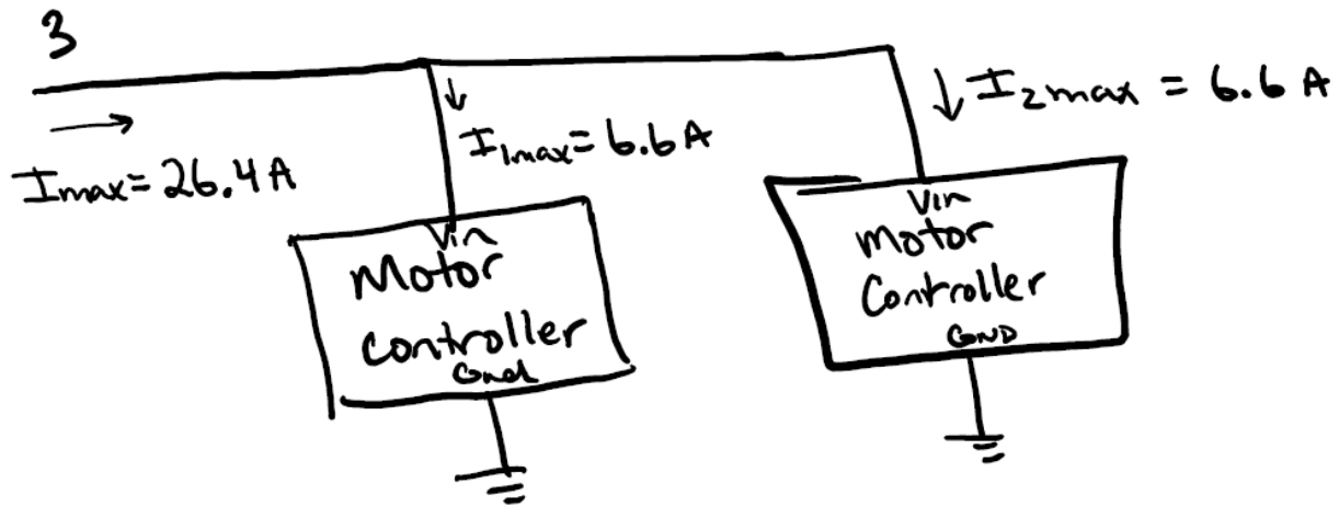
Figure 4.7.1.D – Subsystem 3 (Motor Controllers)
