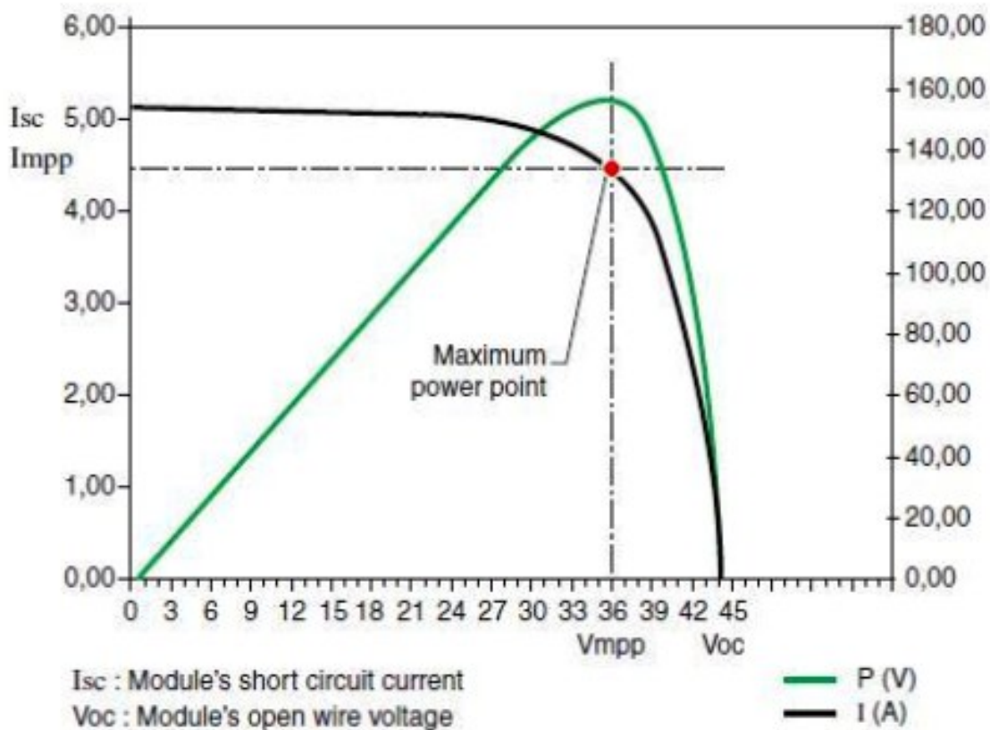
Figure 3.2.15.A - Maximum Power Point of a Solar Panel Permission Pending
