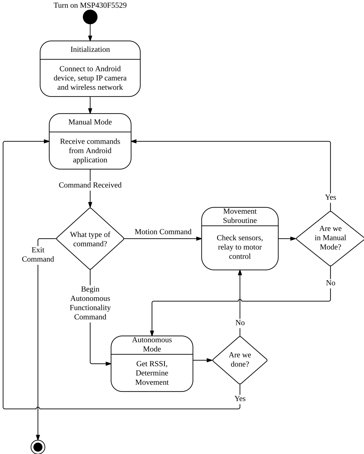
Figure 5.2.3.A - Microcontroller Code State Diagram
