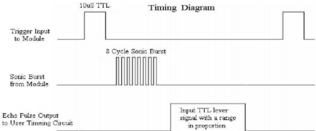
Figure 5.1.6.A - HC-SR04 Timing Diagram
