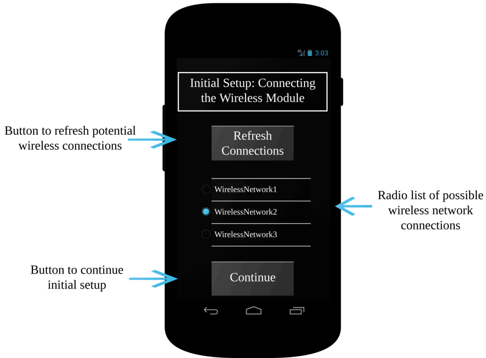
Figure 4.4.A - Android Initial Wireless Module Setup
