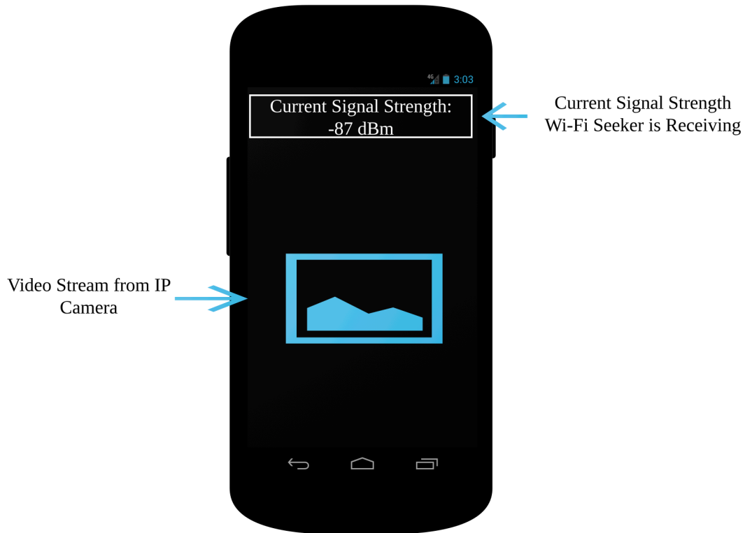
Figure 4.4.D - Android Main Activity: Autonomous Mode
