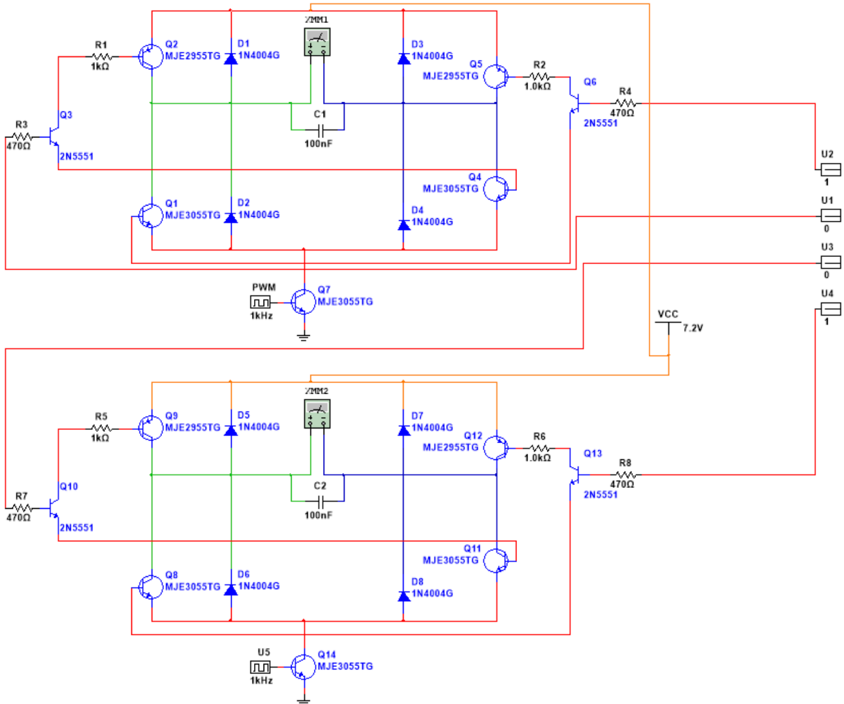
Figure 4.3.2.B - Full H-Bridge Schematic For Wi-Fi Seeker Robot
