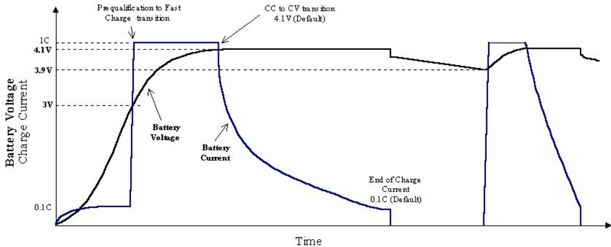
Figure 3.2.16.B - Lithium Polymer Battery Charging Cycle Permission Pending
