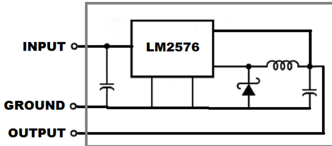
Figure 4.8a: Battery Distribution Block
