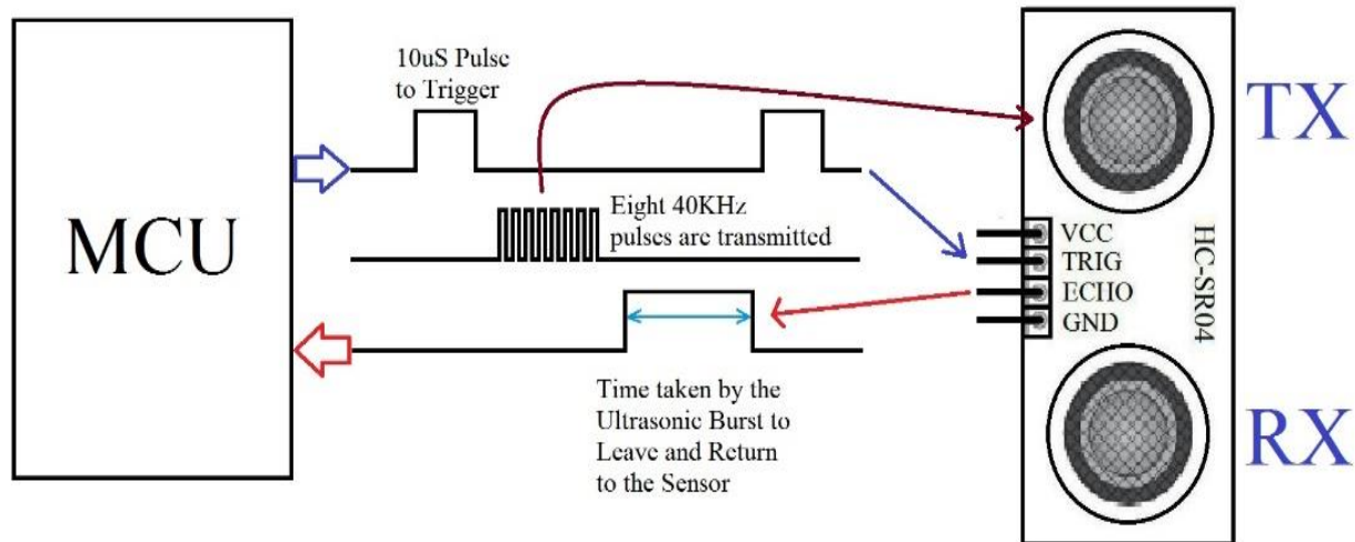
Fig. 4.1.1 shows a simple diagram of the 4 pin layout of the HC-SR04 module and the connection to the microcontroller.
