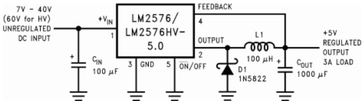
Figure 3.4.7.2.: Switching Regulator
