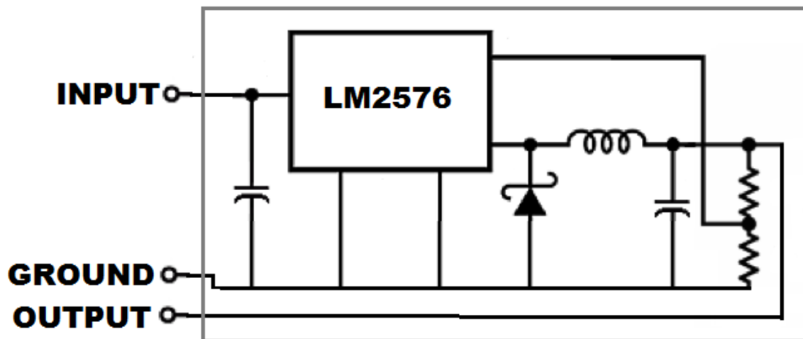
Figure 4.8b: 9 Volt Switching Regulator
