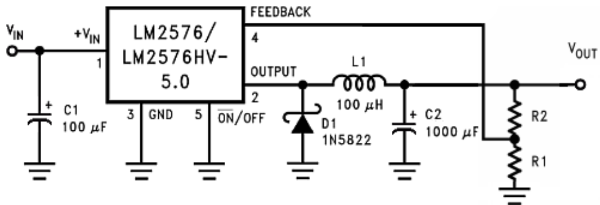
Figure 4.5.1d: Switching Regulator
