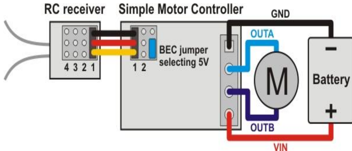
Figure 4.4.1: Receiver Connection
