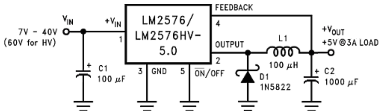
Figure 4.5.1b: Switching Regulator
