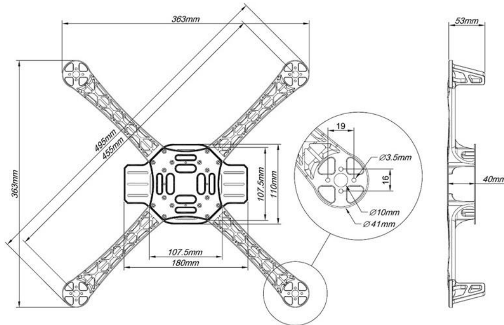
Figure 3: DJI F450 Frame Dimensions.
