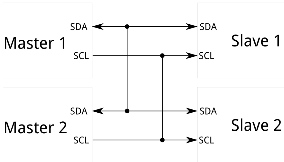
Figure 9: I2C Communication Regular Set Up. (Courtesy of Sparkfun)
