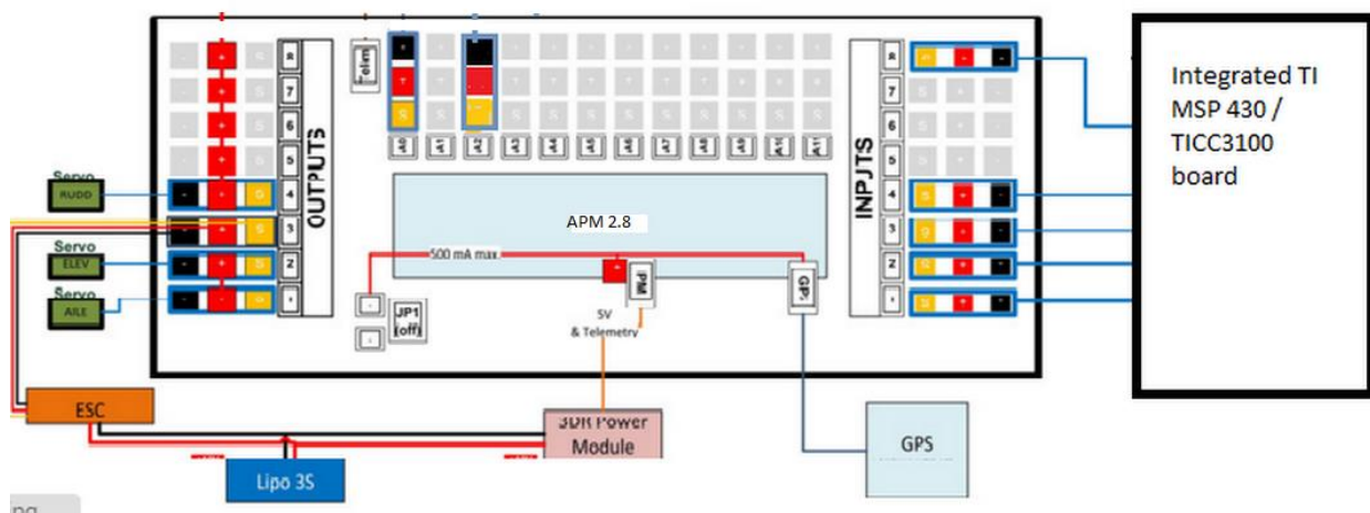
Figure 11: Analog input – MSP430 PWM signal communication
