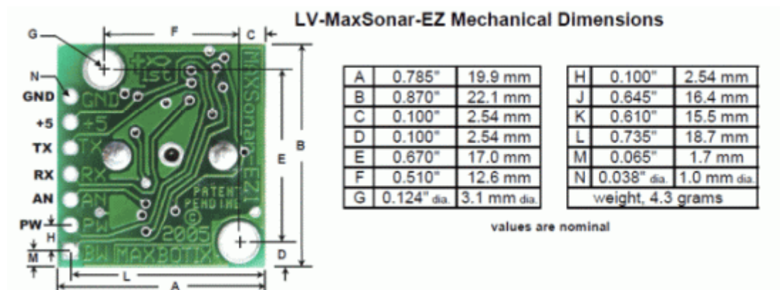
Figure 32: Mechanical dimensions of the MaxSonar-EZ Sensor. (Courtesy of Maxbotix)
