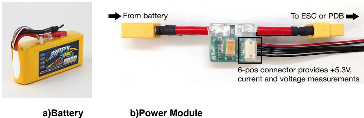
Figure 14: Zippy 5800mAh LiPo Battery
