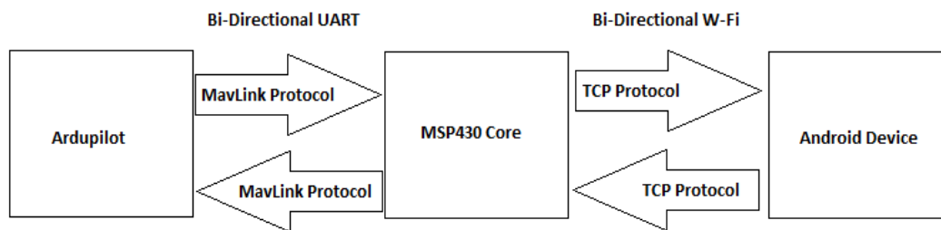
Figure 69: Bi-directional Communication
