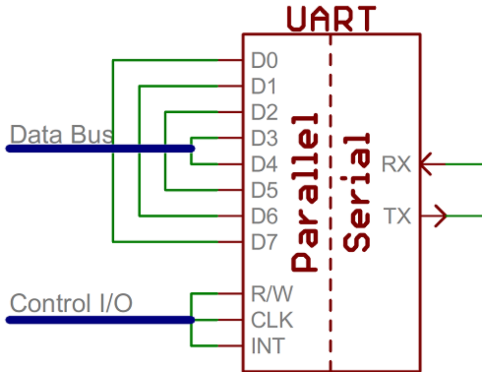
Figure 35: Simplified UART interface. (Courtesy of Sparkfun)
