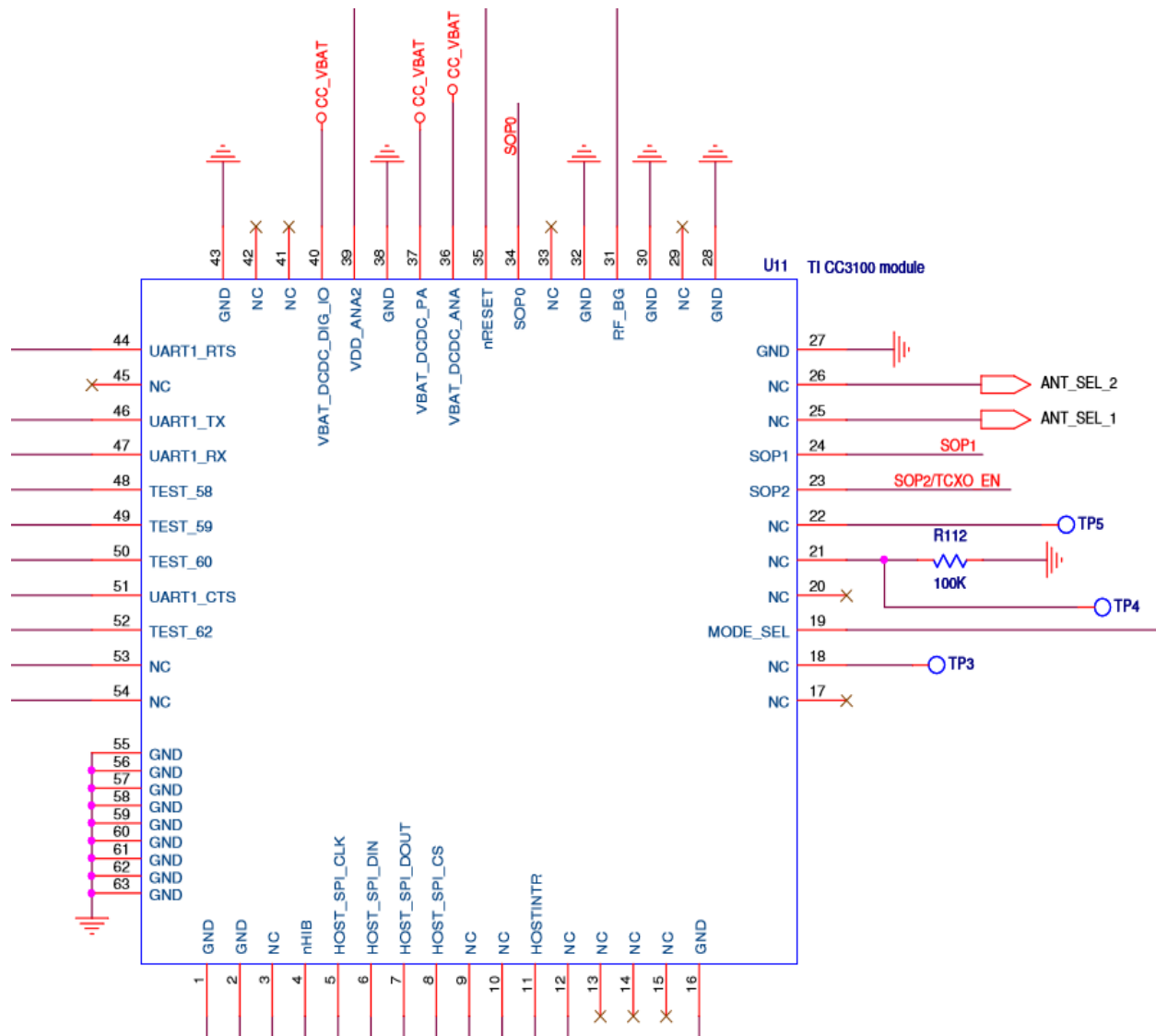
Figure 29: CC3100 Eagle CAD Schematic (Courtesy of Texas Instrument)
