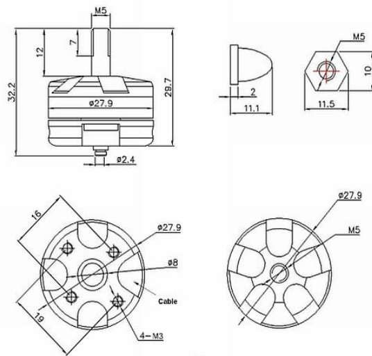
Figure 4: Dimensions of RHD 2212/920kV motor.
