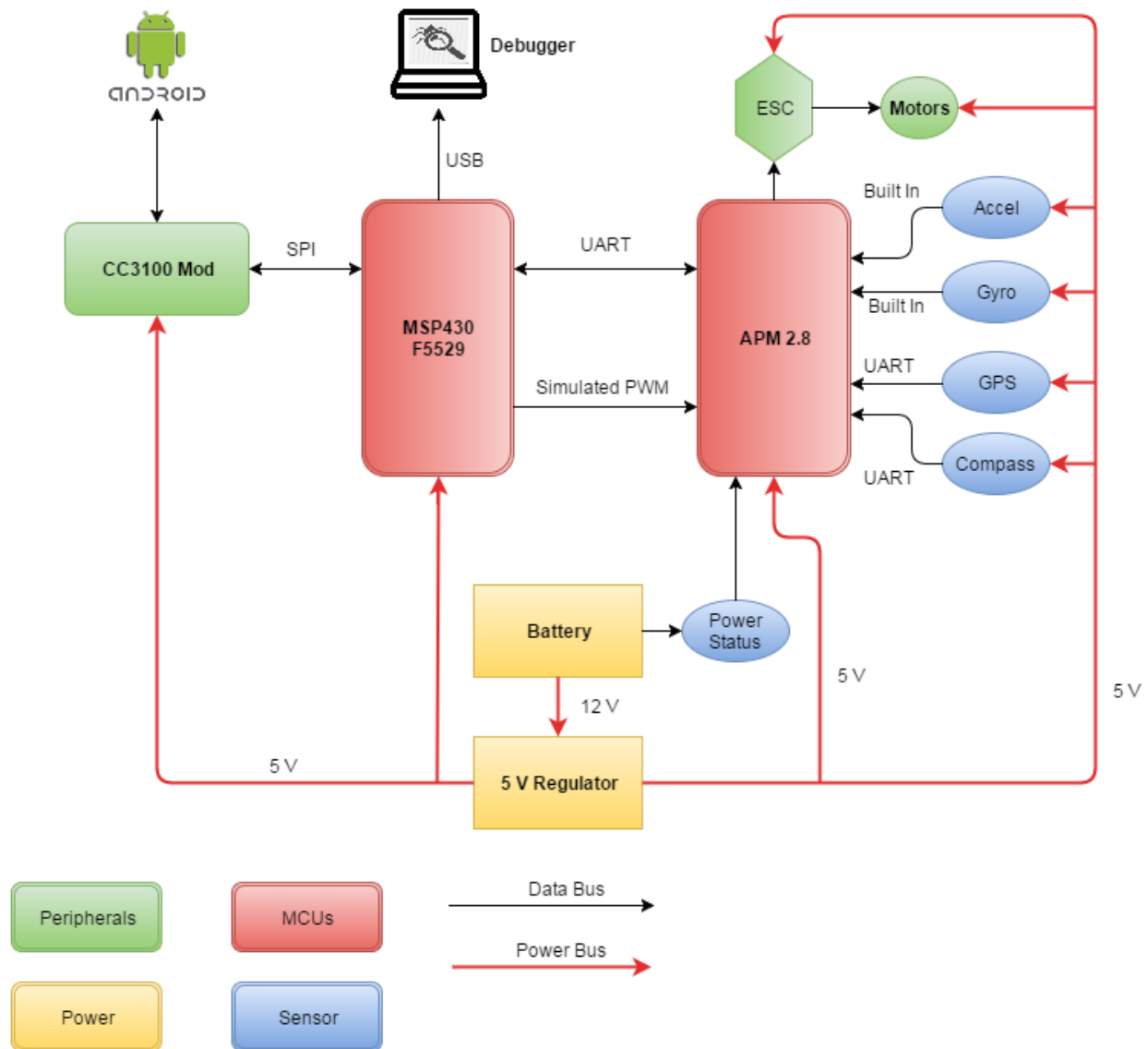
Figure 17: Overall Block Diagram
