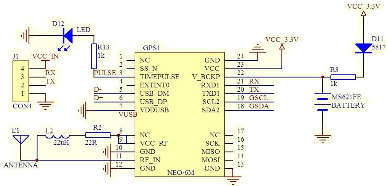
Figure 20: Neo 6M GPS schematic
