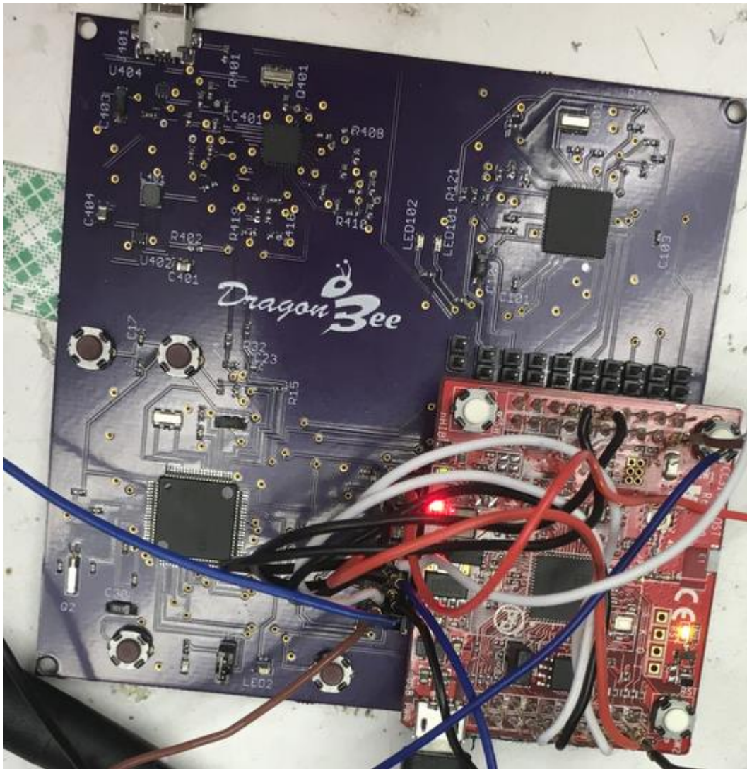
Figure 56: Dragon Bee-CC3100 connections
