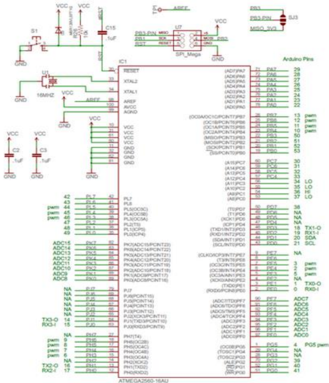
Figure 18: APM design diagram
