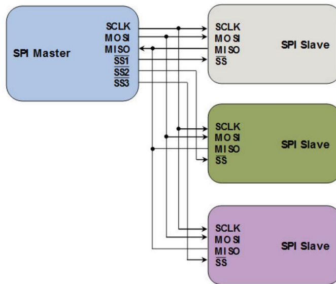
Figure 10: SPI Master & Slave Connections (Courtesy of Sparkfun)
