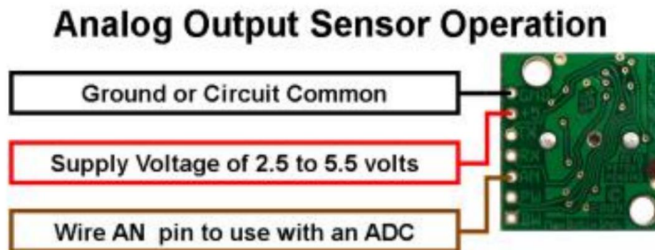
Figure 34: MaxBotix EZ Wiring Diagram
