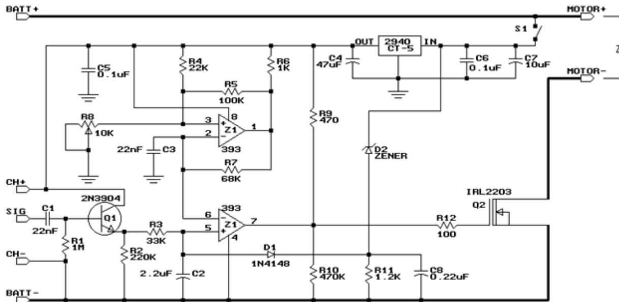
Figure 25: 30A ESC with BEC schematic
