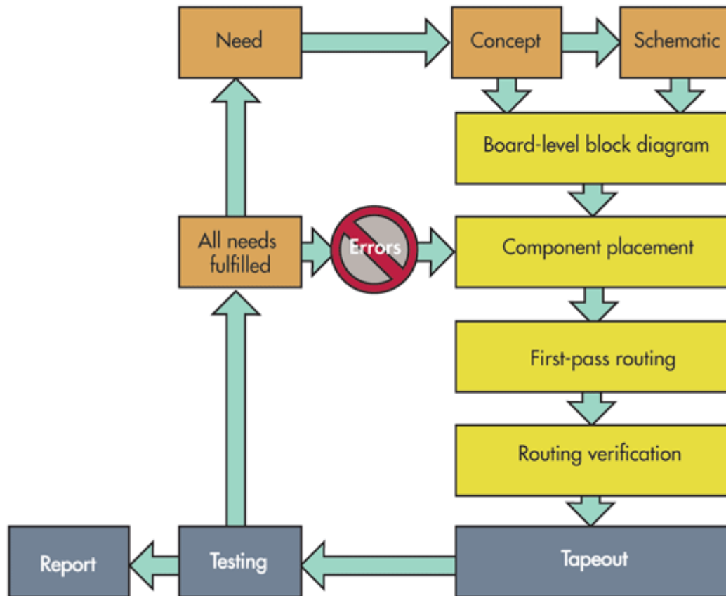
Figure 6: PCB Fabrication Steps
