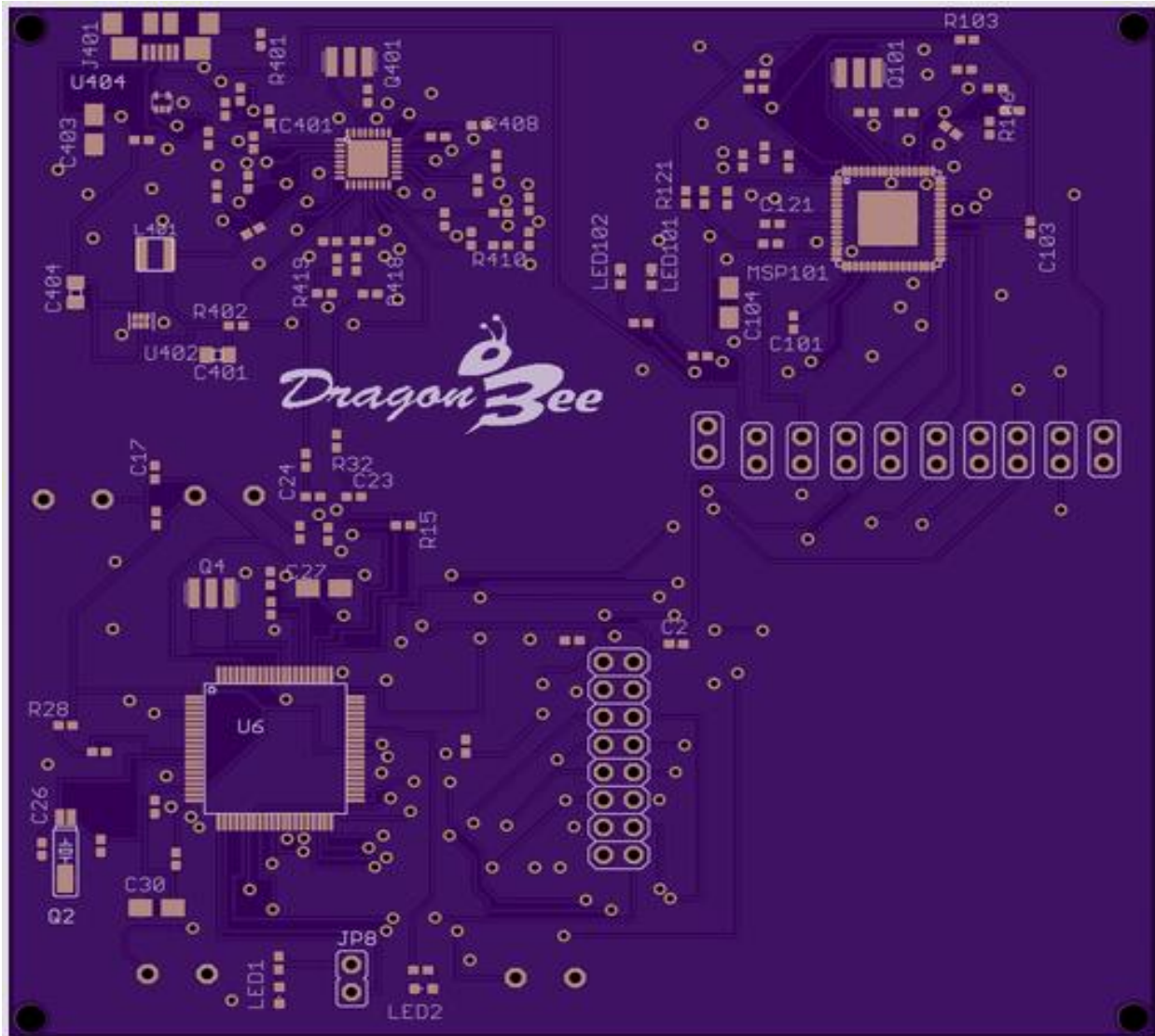
Figure 54: Dragon Bee PCB top view
