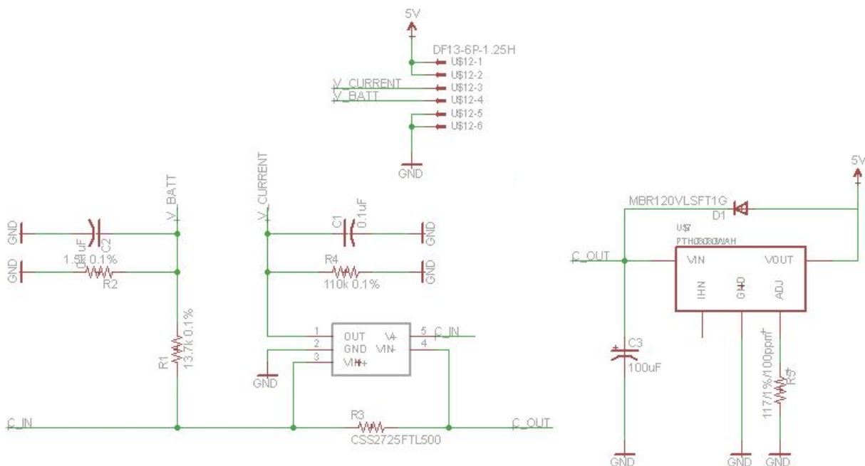
Figure 27: APM PM schematic
