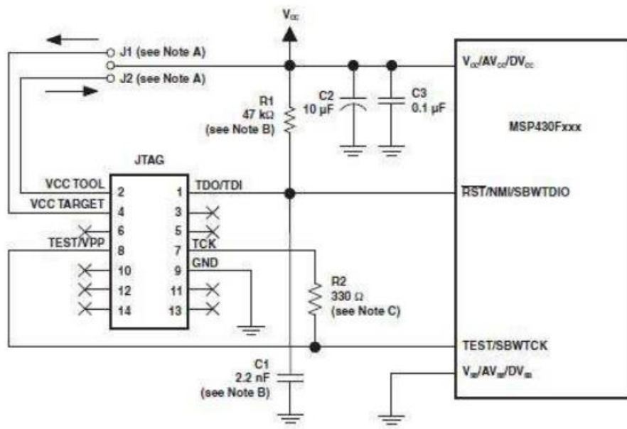
Figure 23: JTAG connection schematic, T.I. Wiki
