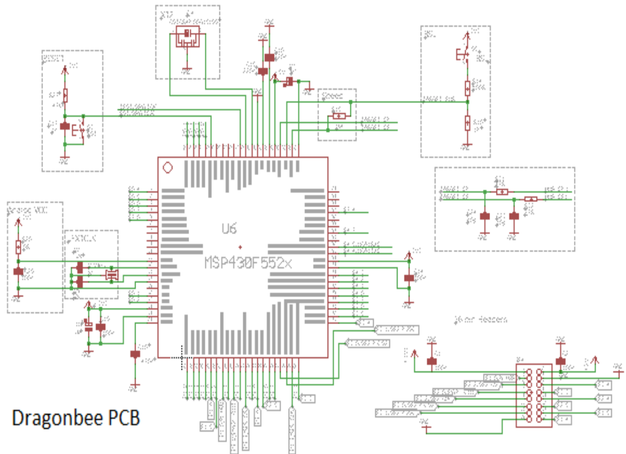
Figure 21: Dragon Bee Schematic diagram
