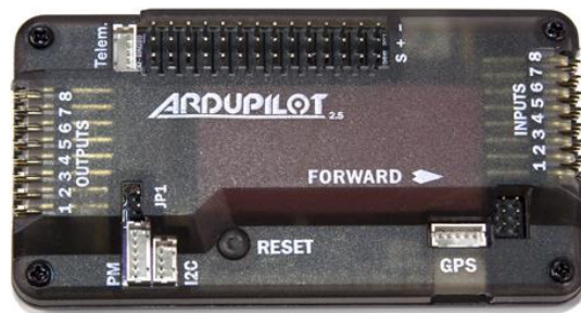
Figure 37: Picture of Ardupilot 2.8 (Mega)
