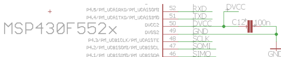
Figure 24: MSP430 Power Diagram (Courtesy of Texas Instrument)
