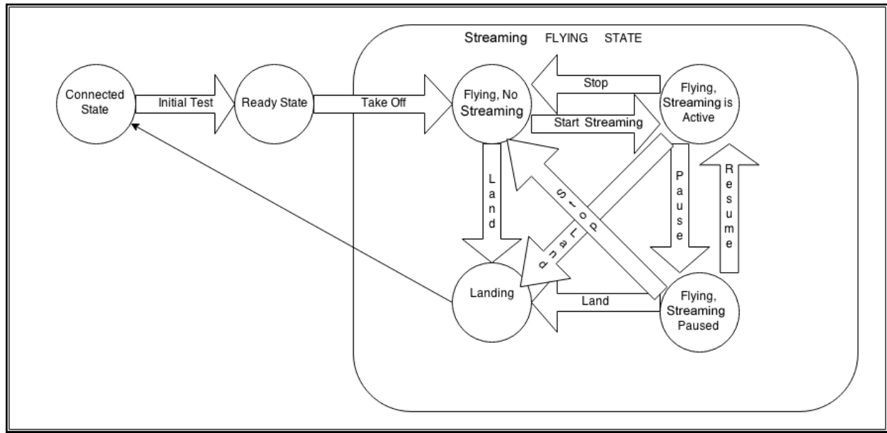
Figure 50: State transition diagram for streaming
