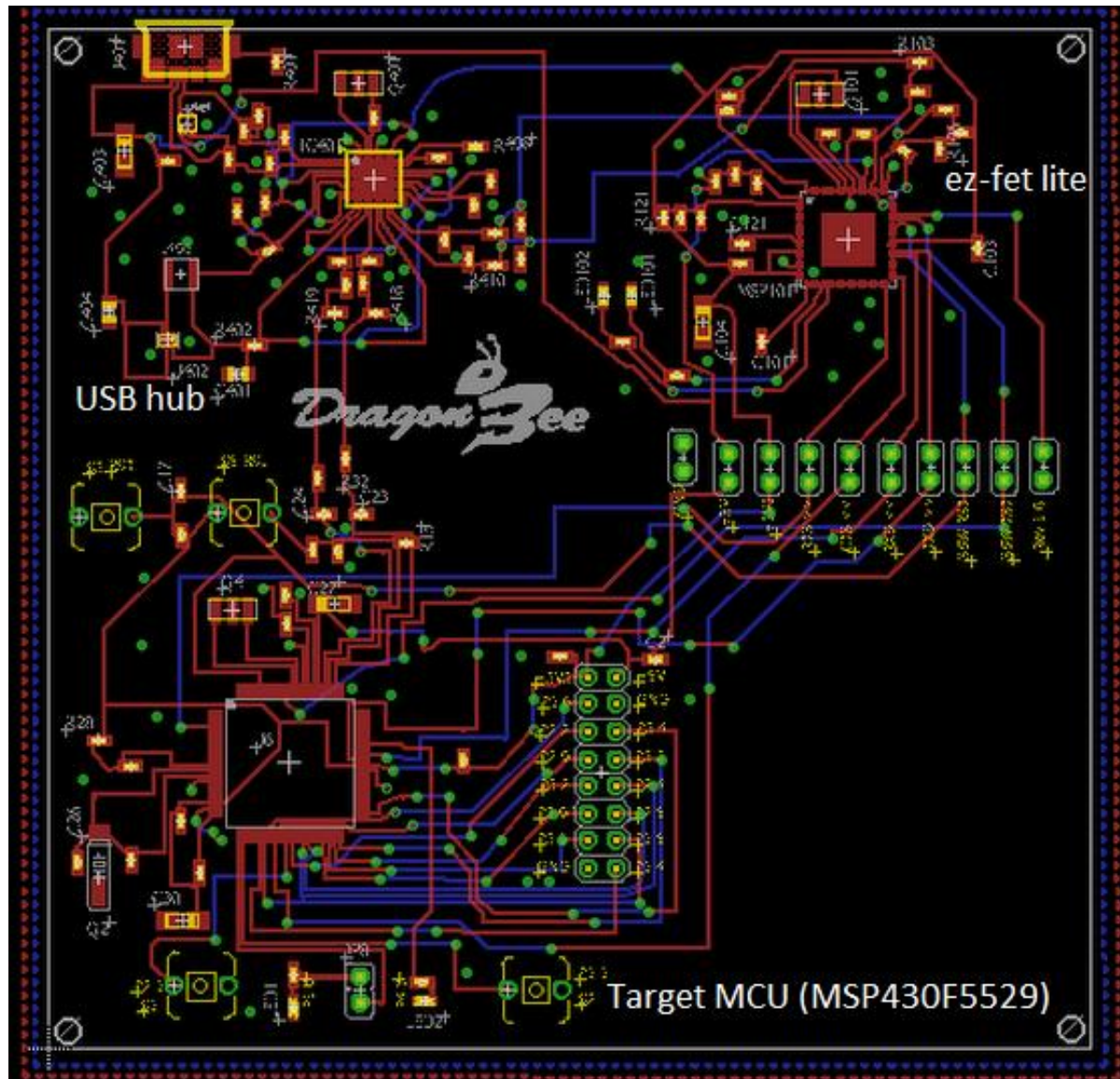
Figure 22: Dragon Bee Layout View
