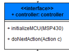
d) Controller interface class
