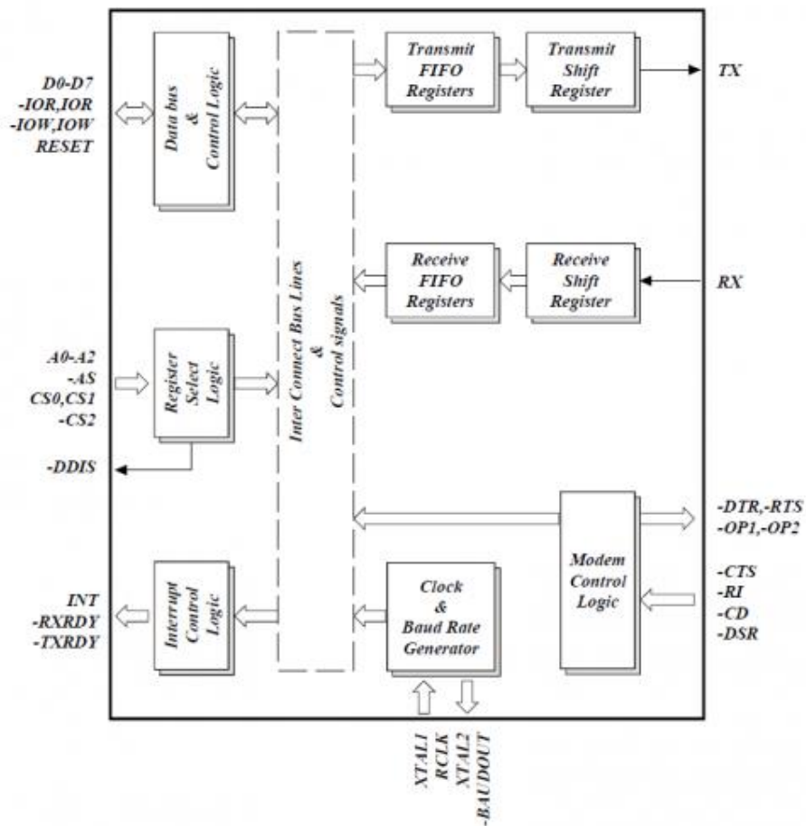
Figure 8: UART Internal Block Diagram. (Courtesy of Sparkfun)
