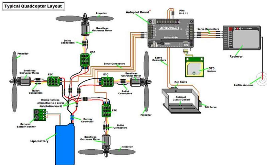
Figure 53: Overall layout of “Dragon Bee” drone
