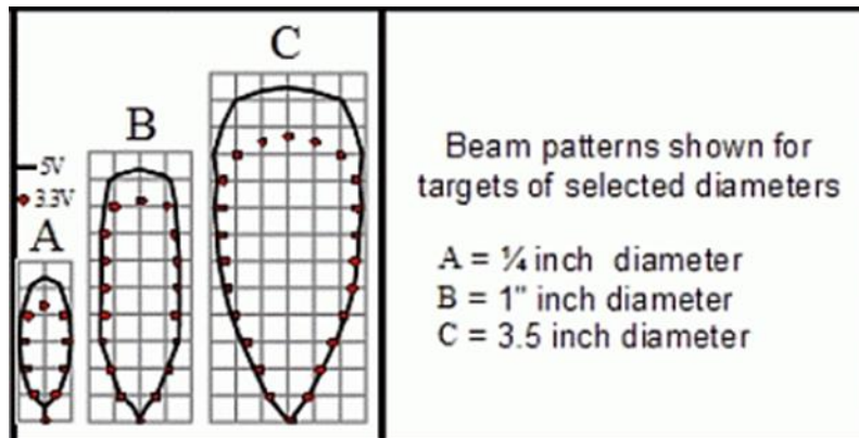
Figure 31: MaxSonar EZ beam pattern diagram. (Courtesy of Maxbotix)
