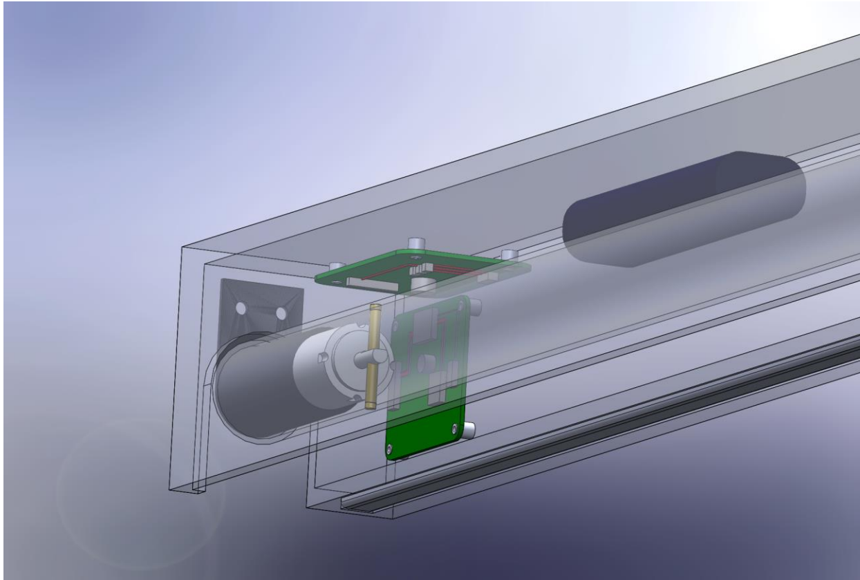
Figure 6.2.ii Board Location Within System Housing
