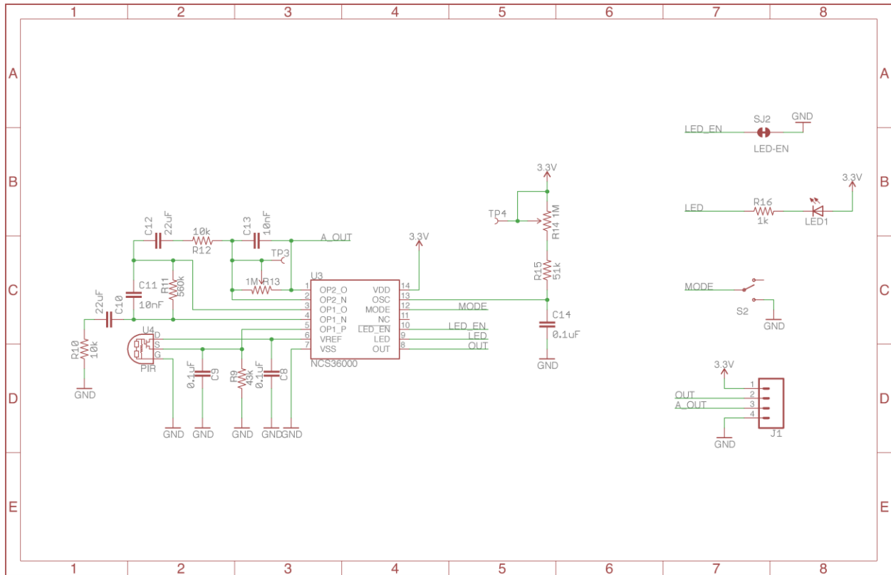
Figure 5.1.iv Initial PIR Schematic
