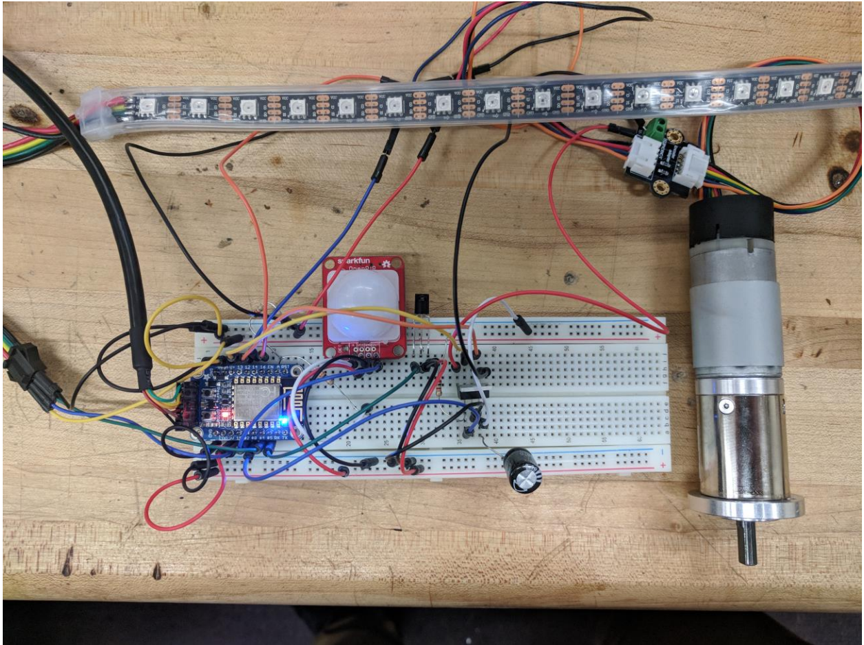
Figure 7.6.i Full Hardware Prototype
