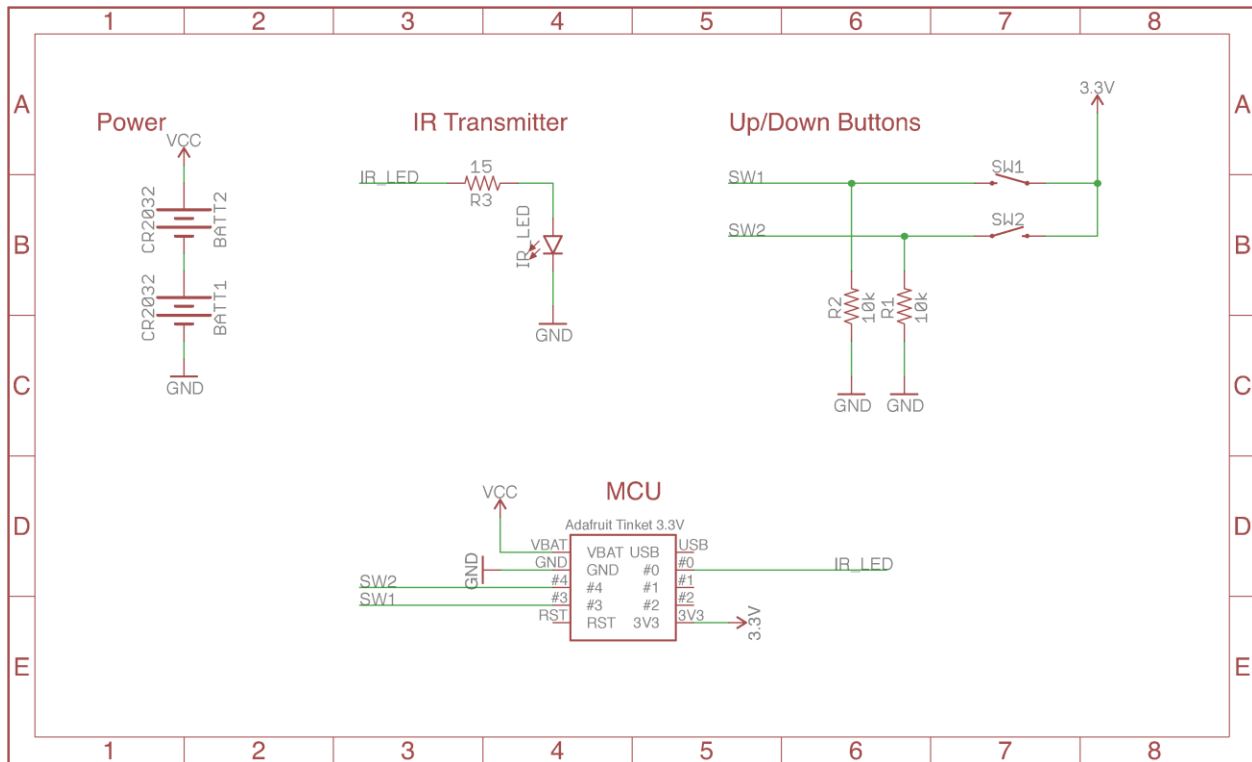
Figure 5.1.vi Initial IR Remote Schematic
