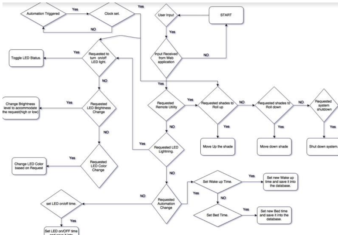
Figure 3.4.ix Code Flowchart
