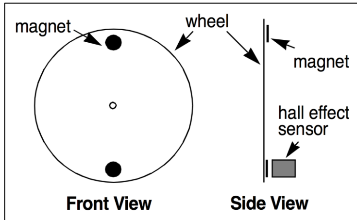
Figure 3.2.vii Hall Effect Encoder [19] (Permission Requested)
