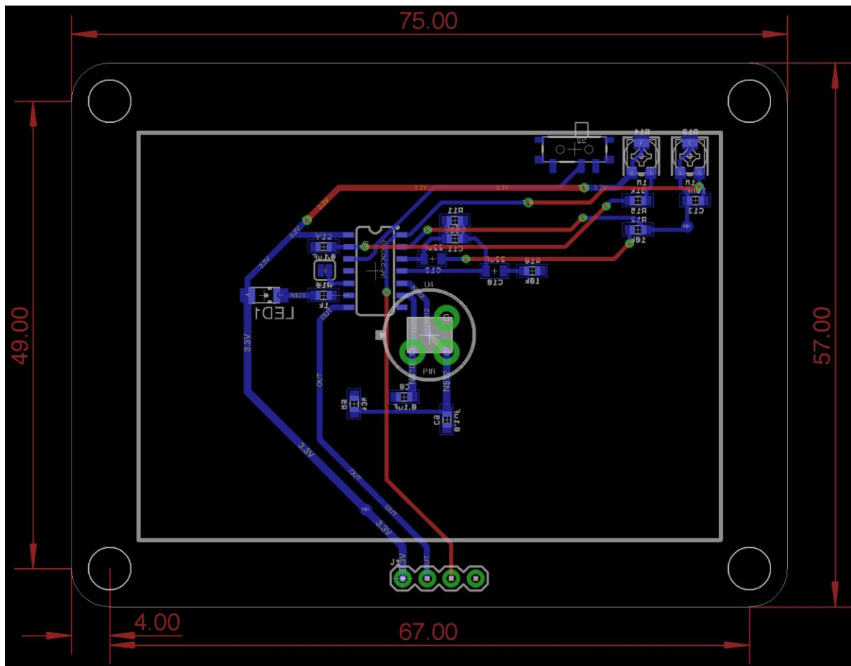
Figure 5.1.v Initial PIR Board Layout
