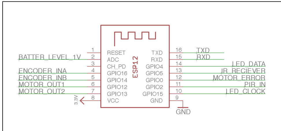
Figure 3.4.iii ESP12 Pinout
