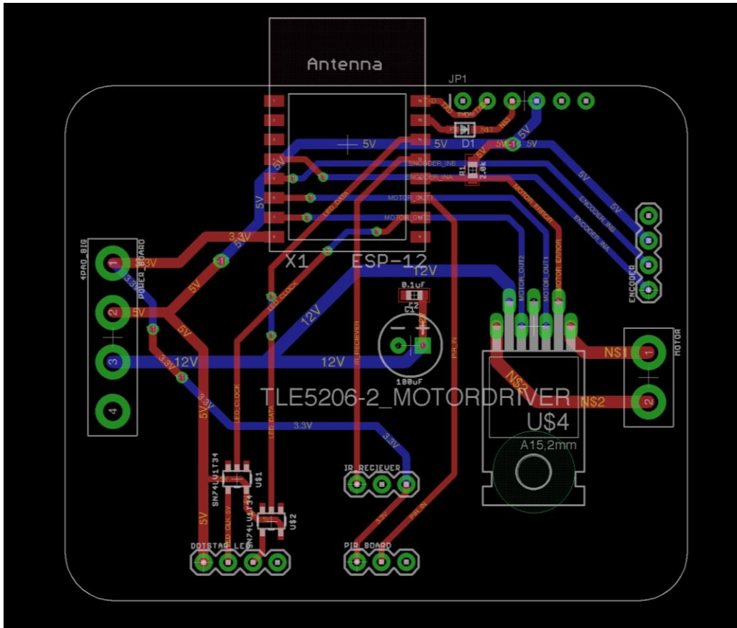
Figure 5.1.iii Initial Main Control System Board Layout
