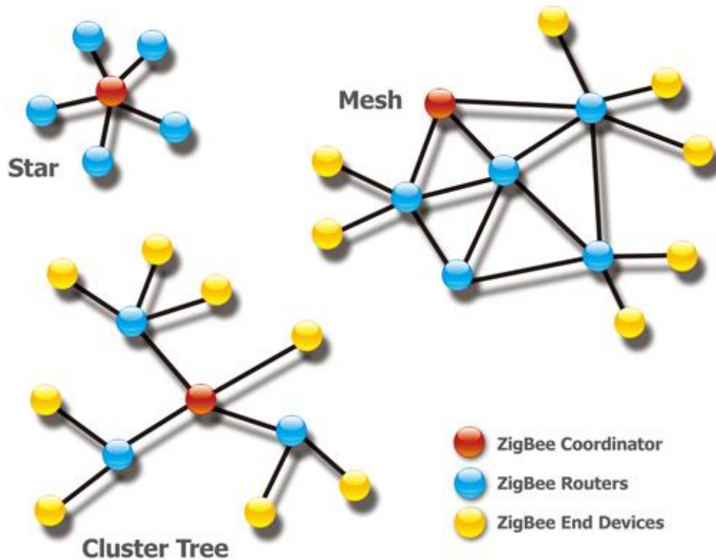
Figure 3.2.xvi Zigbee-supported Networks [138] (Permission Requested)
