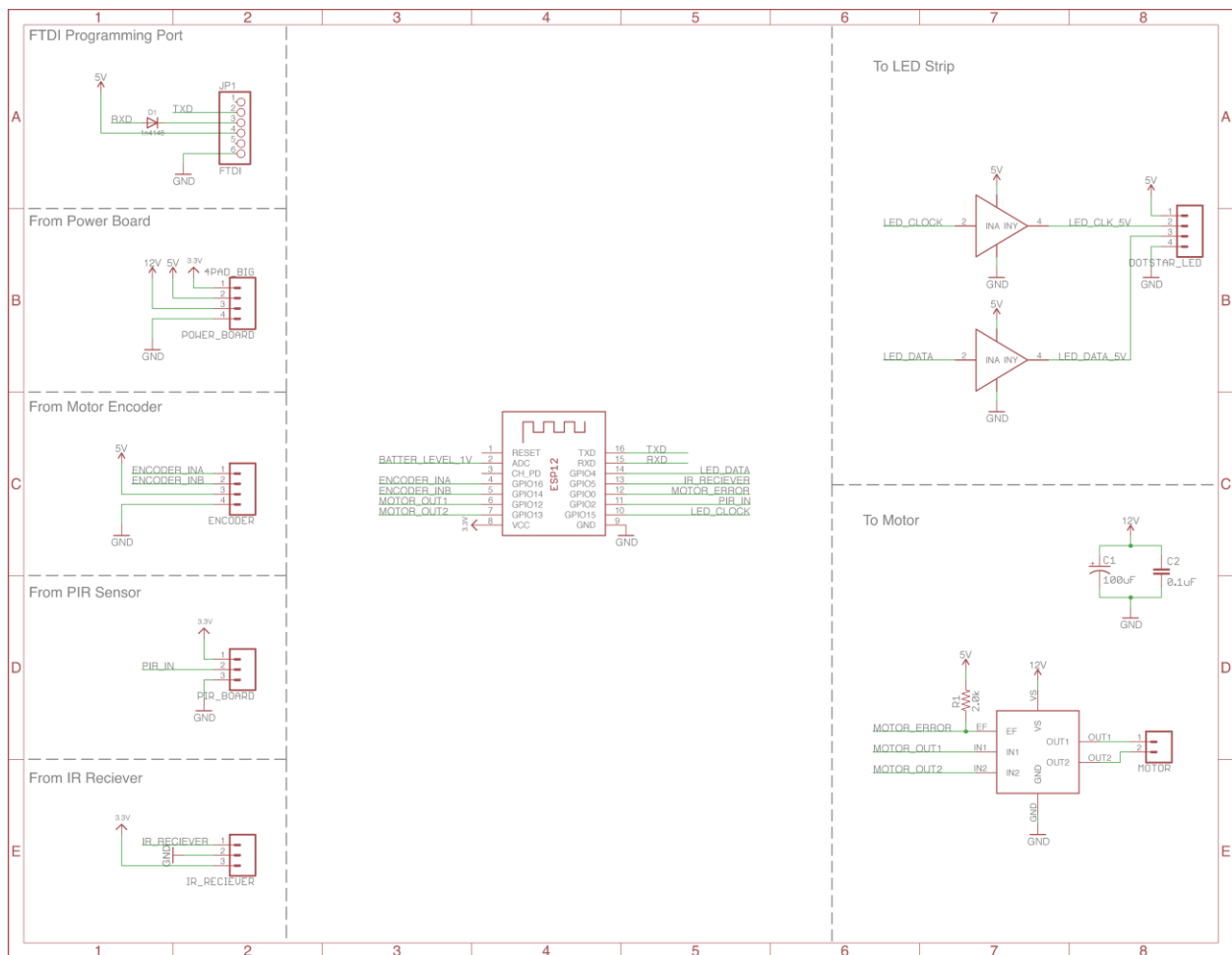
Figure 5.1.ii Initial Main Control System Schematic
