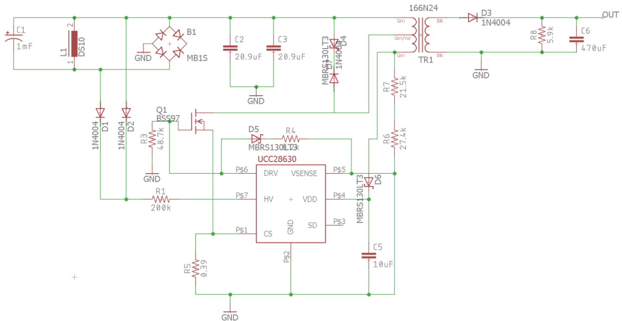
Figure 5.1.i Initial Power System Schematic
