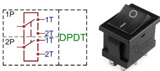
Figure 9 - “double-pole, double-throw” Switch
