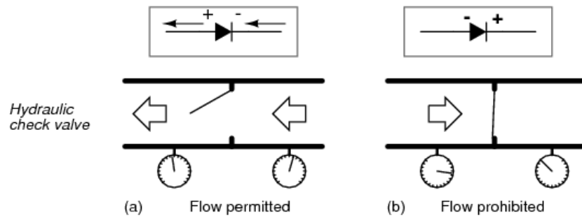
Figure 11: Hydraulic check valve analogy: (a) Electron current flow permitted. (b) Current flow prohibited
