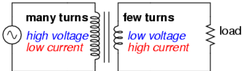
Figure 9: Step-Down Transformer
