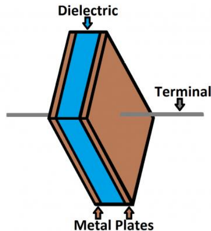
Figure 15: Capacitor Construction
