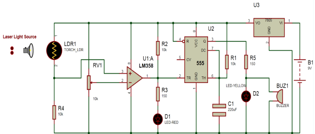
Figure 34: Laser Security Alarm Circuit
