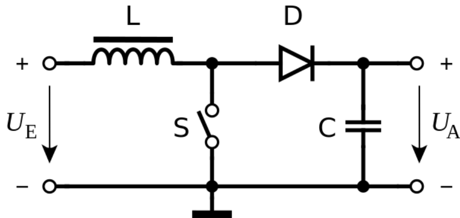
Figure 18: Boost Converter (Public Domain)
