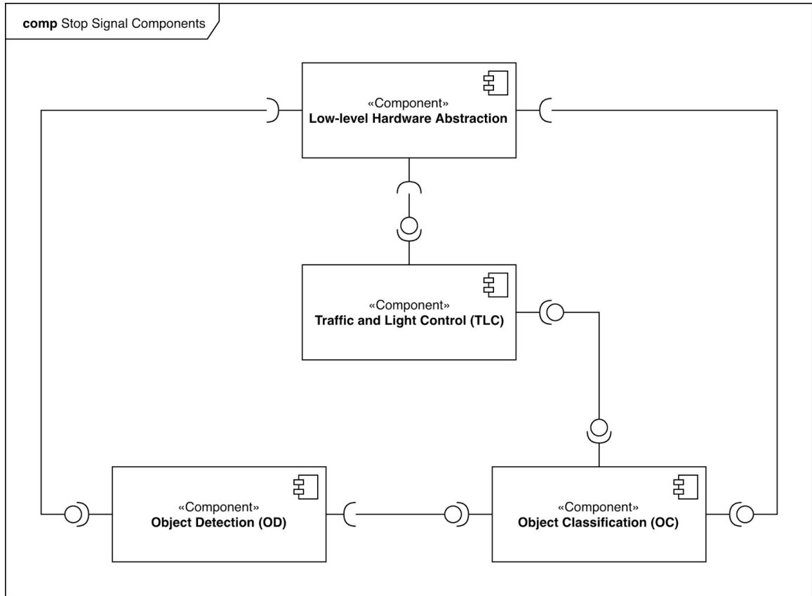
Figure 33: Component Diagram
