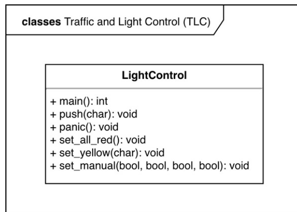
Figure 36: Traffic and Light Control Class Diagram
