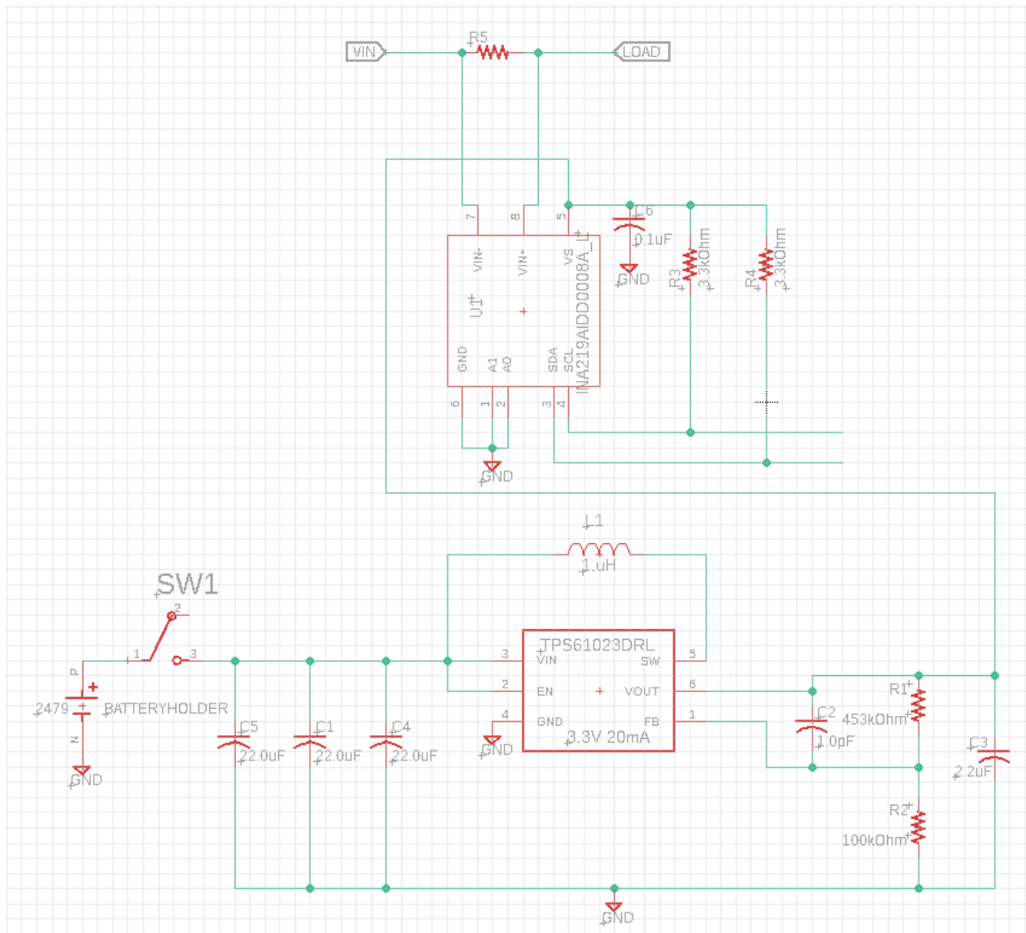
Figure 8: Voltage/Current Sensor Schematic.
