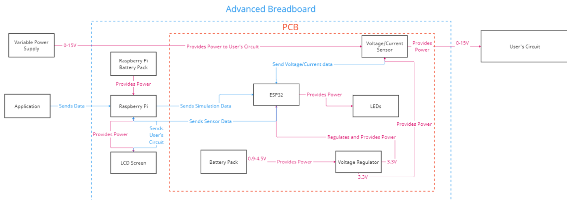
Figure 6: Subsystem Block Diagram.
