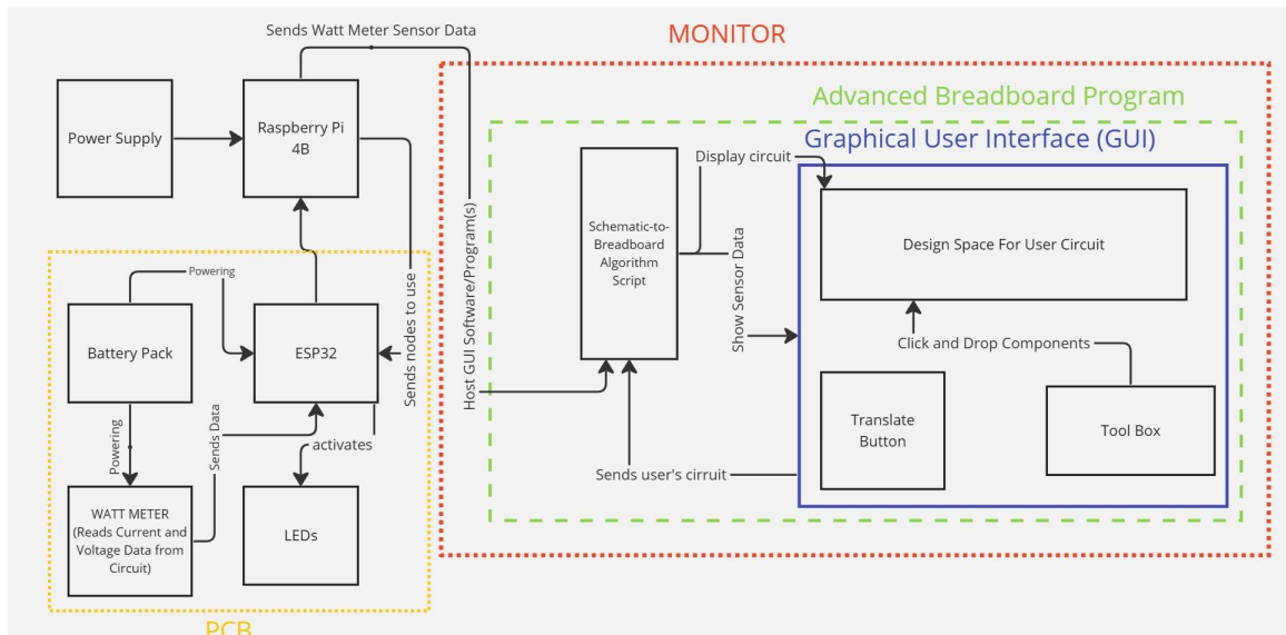
Figure 16: Software Subsystem Block Diagram.
