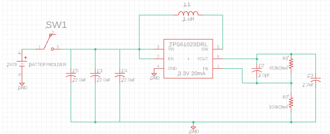
Figure 7: Power Supply Schematic.
