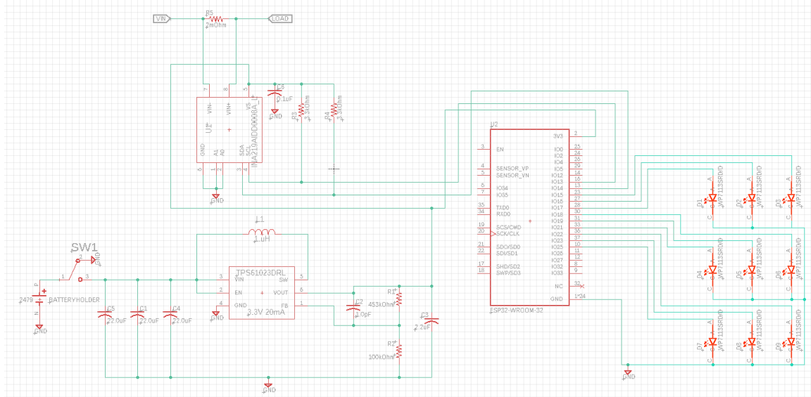
Figure 9: ESP32 and LEDs Schematic.
