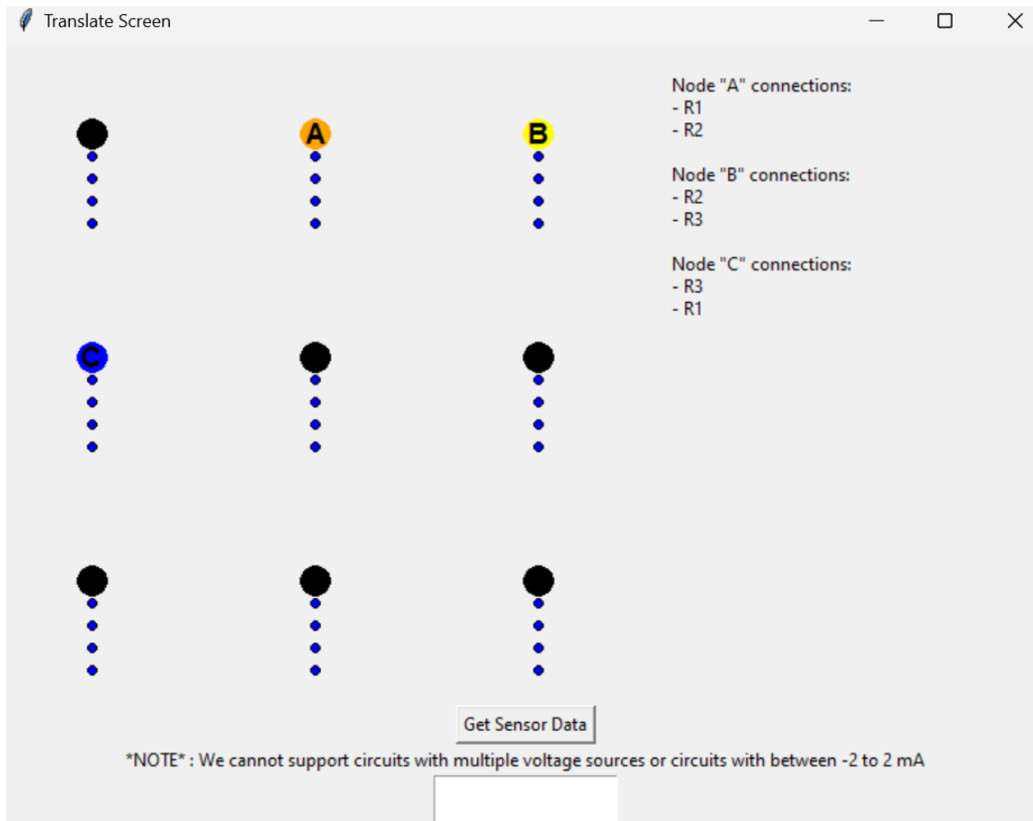
Figure 27. Final GUI Design (Translate Screen).
