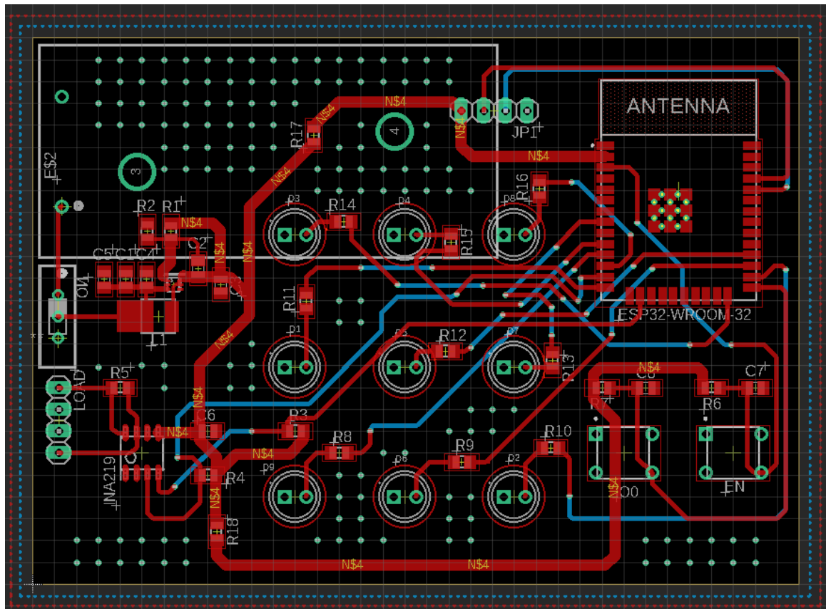
Figure 17: PCB Layout.
