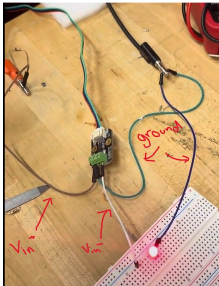
Figure 20: Power Distribution Through Sensor.
