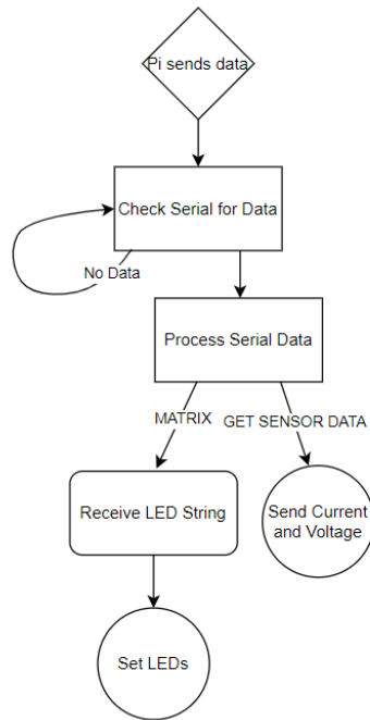
Figure 17. ESP32 Programming.
