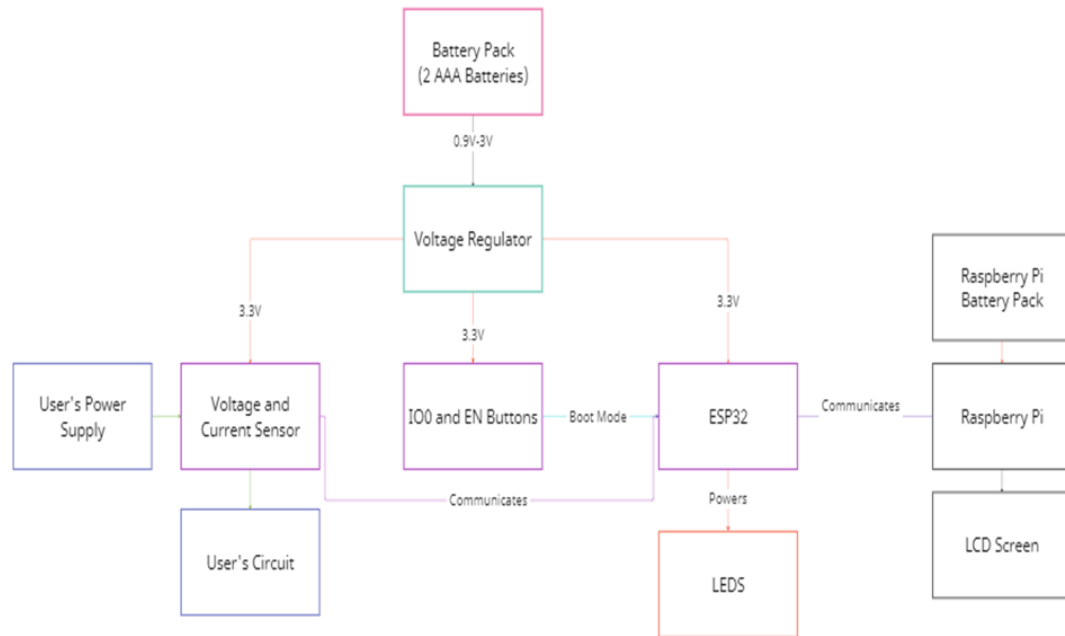
Figure 4: Hardware Flowchart
