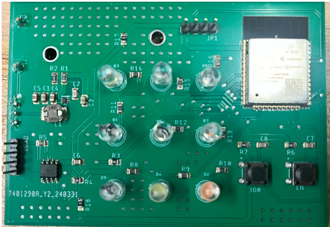
Figure 25: Final PCB
