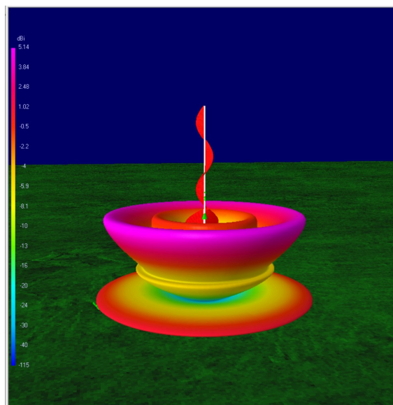
Figure 3.14 J-Pole Antenna Radiation Pattern
