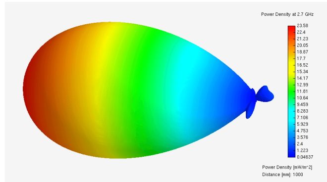
Figure 3.15 YAGI Antenna Radiation Pattern
