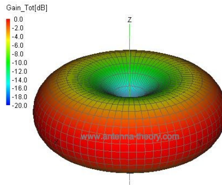
Figure 3.13 Dipole Antenna Radiation Pattern
