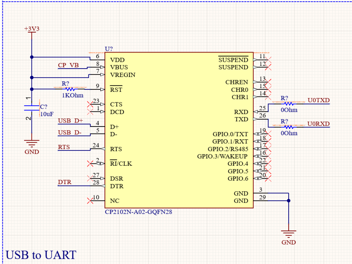
Figure 6.2.3: CP2102 Schematic
