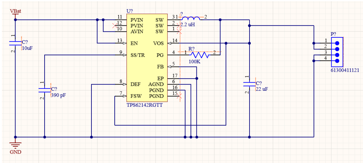
Figure 6.7.1 3.3V Buck Regulator
