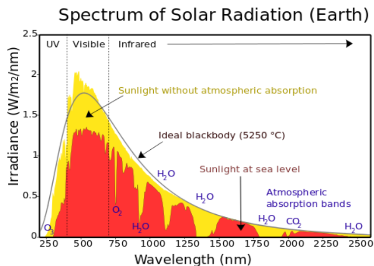
Figure 2.1: Solar Spectrum.
