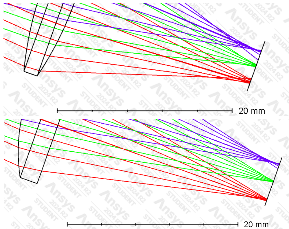
Figure 3.11 Double convex versus plano-convex lenses simulated in the spectrometer setup, respectively
