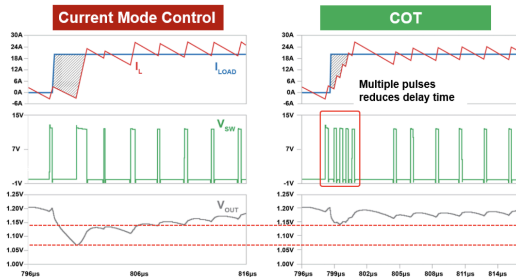
Figure 3.17 CMC vs COT
