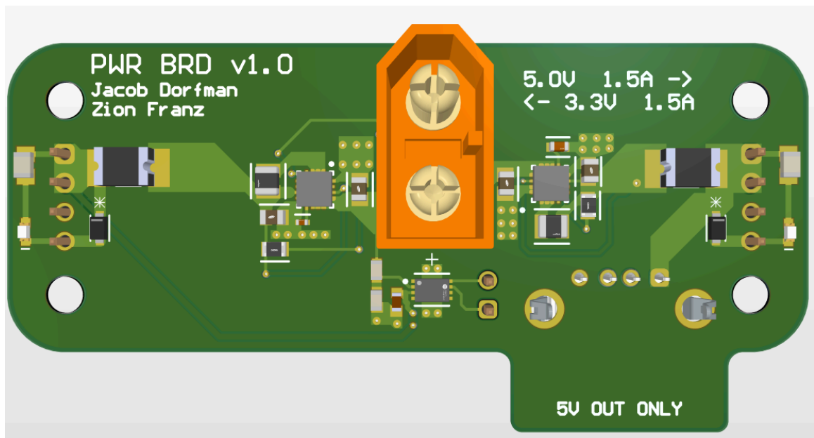
Figure 8.3: 3D Power Board Layout
