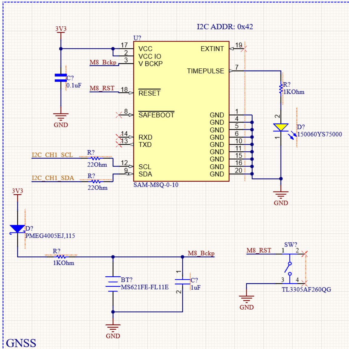
Figure 6.5.1: GNSS Schematic
