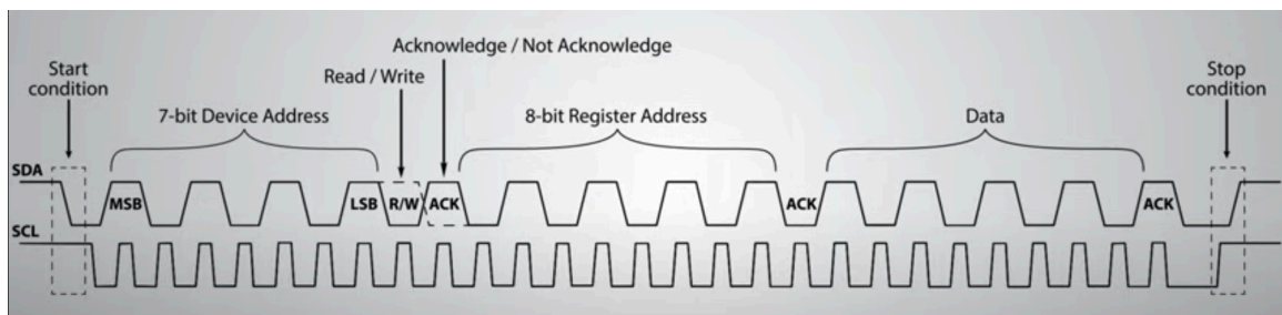
Figure 4.2: I2C Data.
