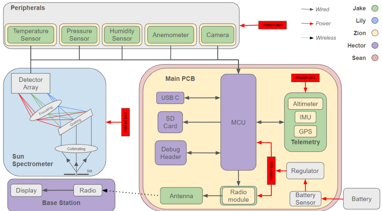
Figure 2.2: Hardware Diagram
