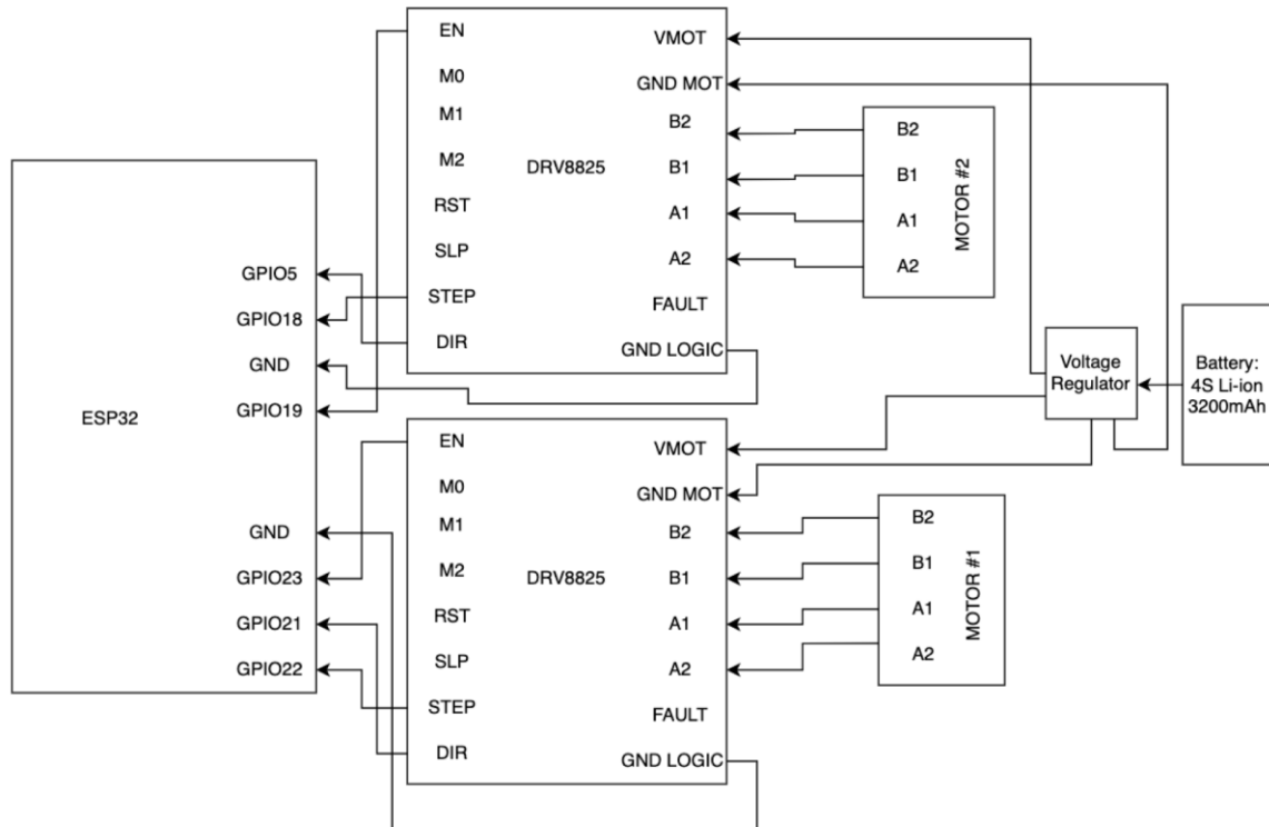
Figure 6.1.1 Motor Subsystem Block Diagram
