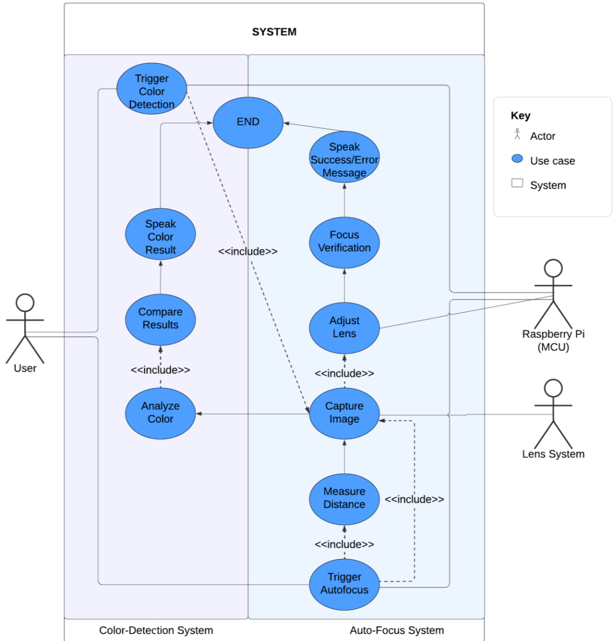
Figure 7.1.1 Use Case Diagram
