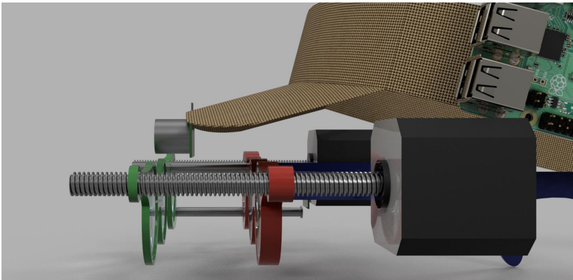
Figure 6.1.4 Motor #2 Structural Model
