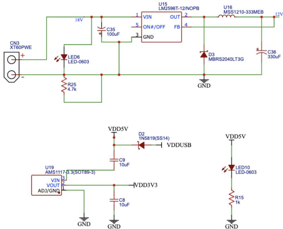
Figure 6.1.12 12V Regulator and 3.3V regulator (top schematic and bottom schematic accordingly)
