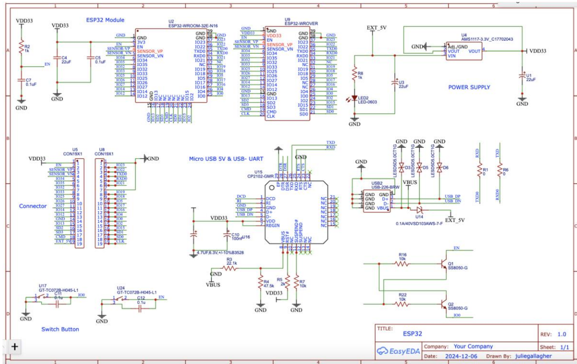
Figure 8.1.1 Main PCB Schematic
