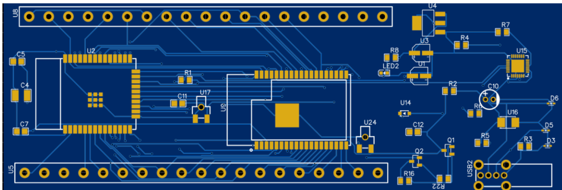
Figure 8.1.2 Main PCB Layout
