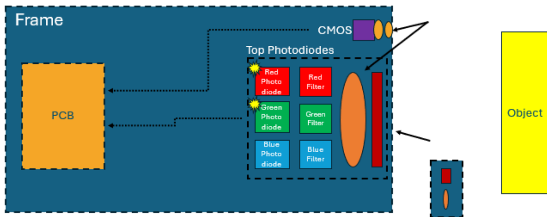
Figure 2.4.2 Color-Identifying Feature Diagram
