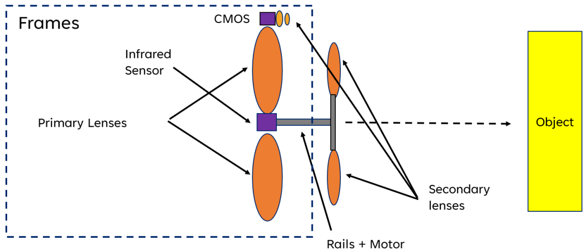
Figure 2.4.1 Auto-Focusing Feature Diagram
