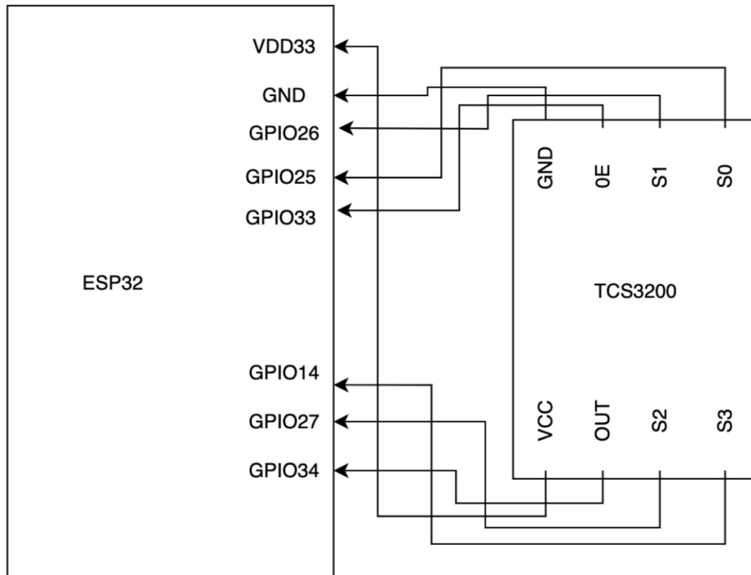
Figure 6.1.5 Colorimeter Subsystem Block Diagram
