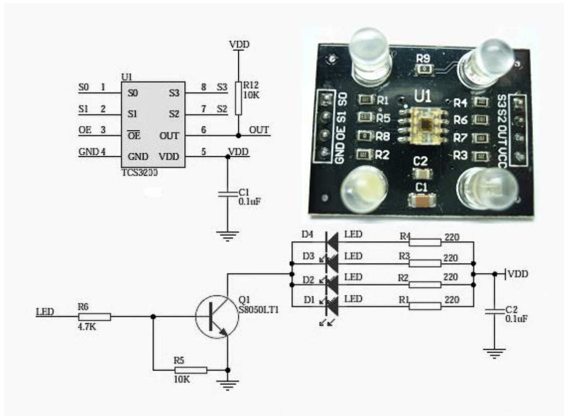
Figure 6.1.6 Colorimeter Subsystem Schematic and Assembled sensor [86]
