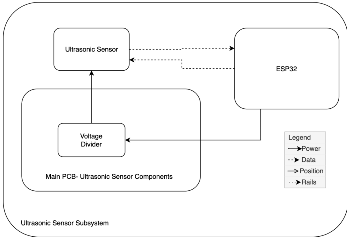
Figure 6.1.9 Ultrasonic Sensor Subsystem
