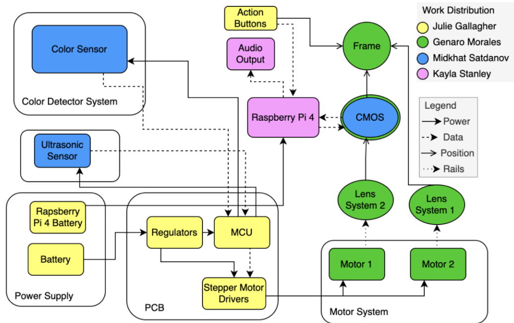
Figure 2.7.1 Hardware Block Diagram
