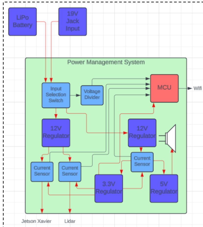
Figure 2.7.2: Hardware Block Diagram for Power Management System
