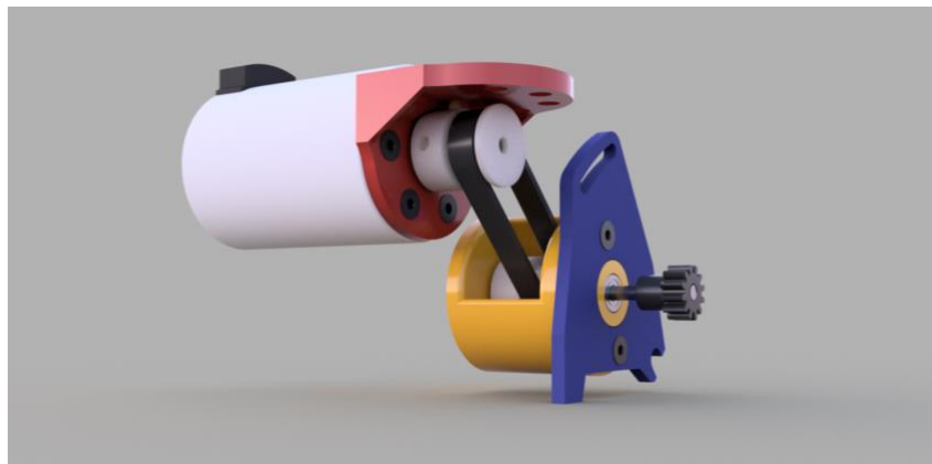
Figure 6.1.1.3: Drivetrain modifications final 3D model
