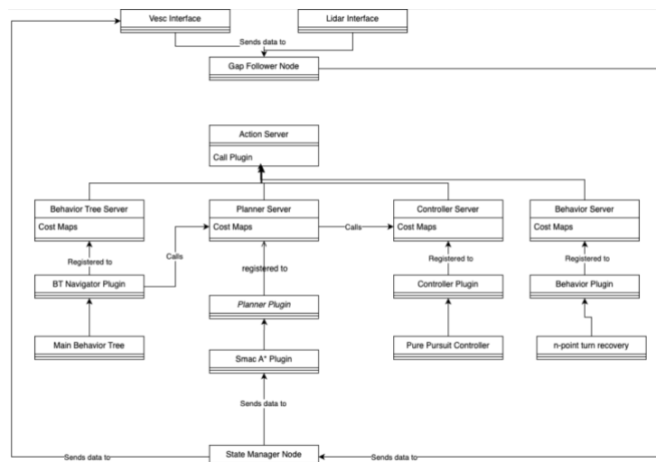
Figure 7.1: Vehicle Control Diagram
