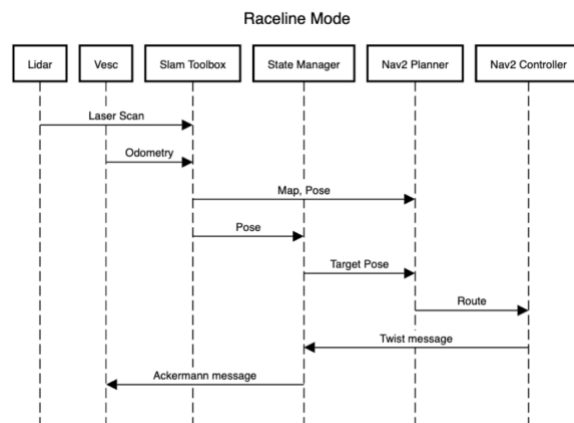
Figure 7.1.3: Raceline Following Diagram
