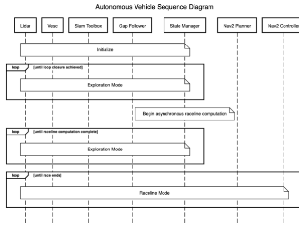
Figure 7.1.4: State Manager Diagram
