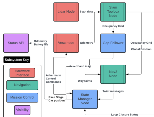
Figure 7: Car Software Flow Chart
