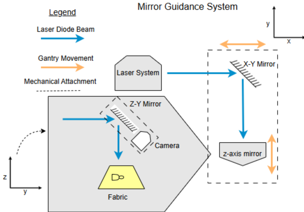
Figure 2: Mirror Guidance Optical Design
