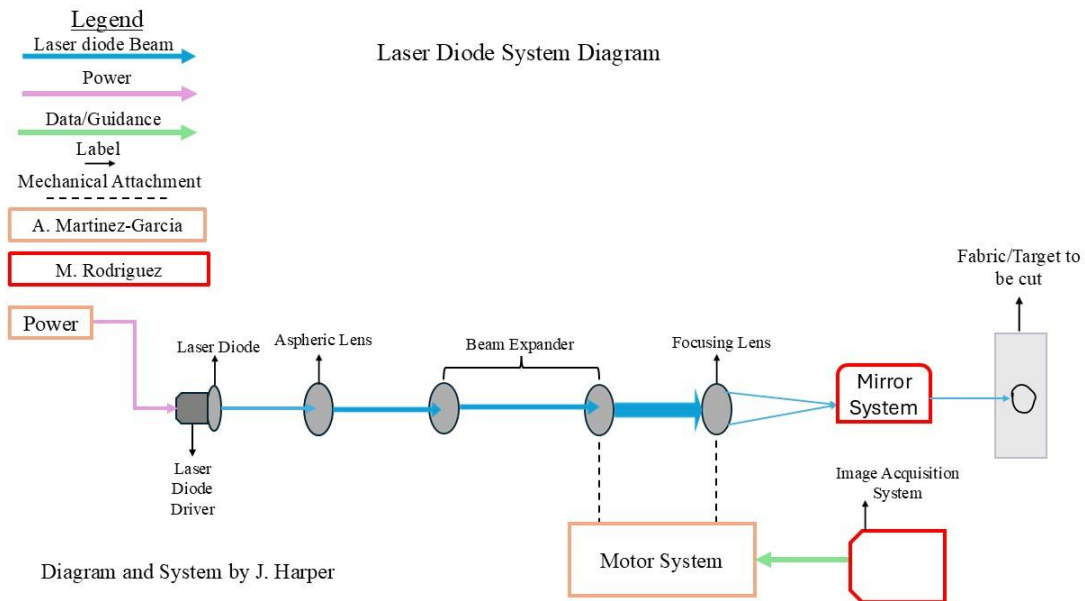
Figure 1: Laser Diode System Diagram
