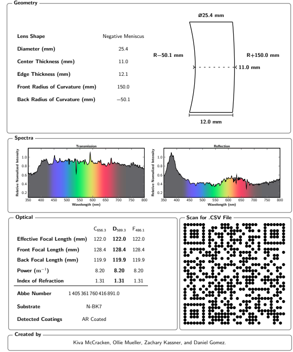
Fig. 7: Generated datasheet.
