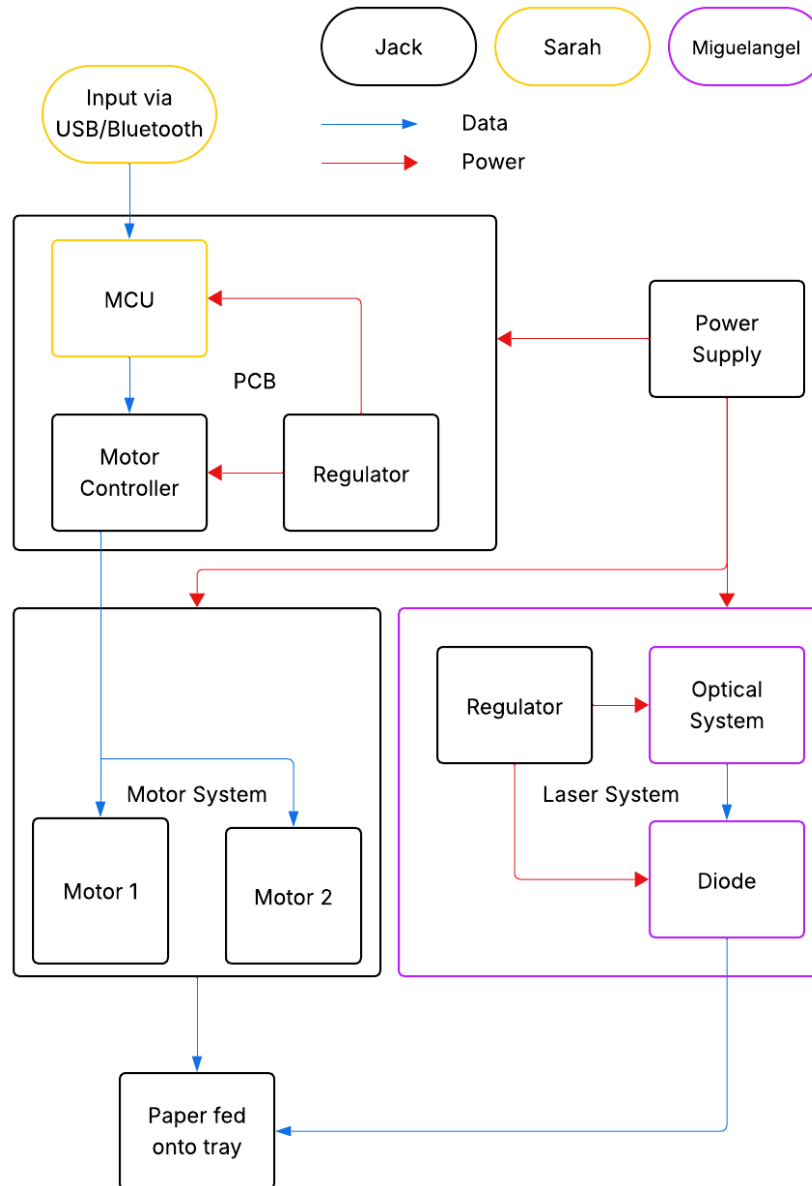
Figure 12: Subsystem Block Diagram
