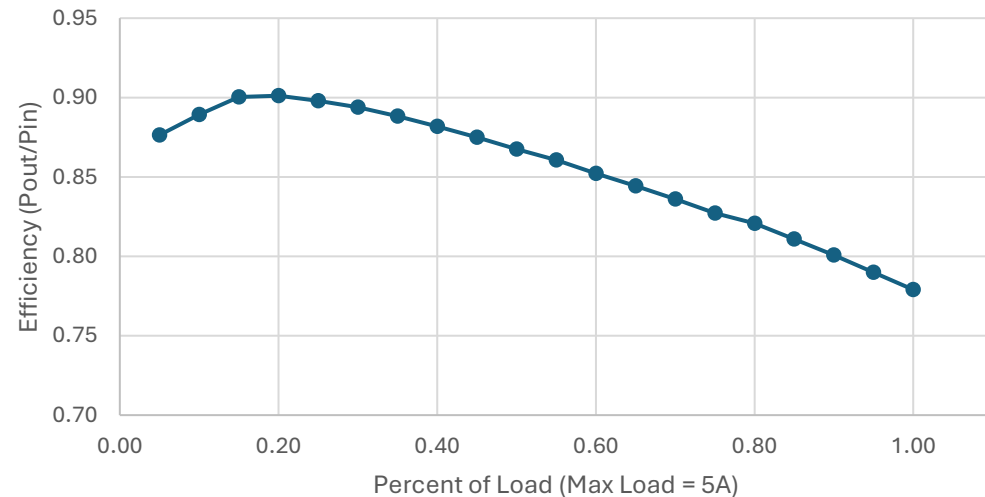
SBC PSU Efficiency Chart
