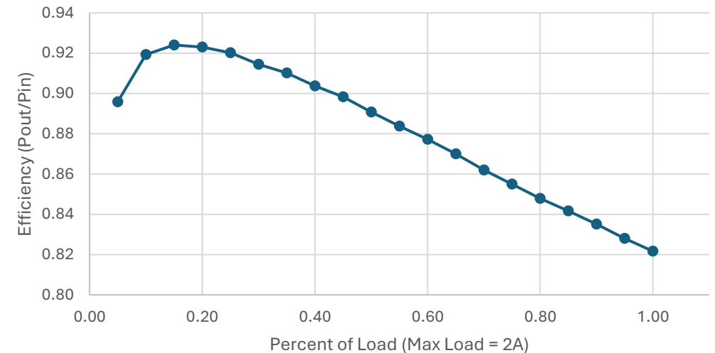
Motor Driver PSU Efficiency Chart
