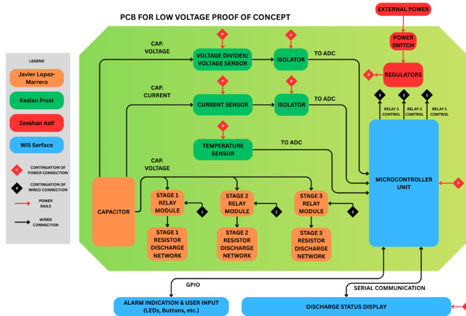
Figure 2: Hardware Diagram
