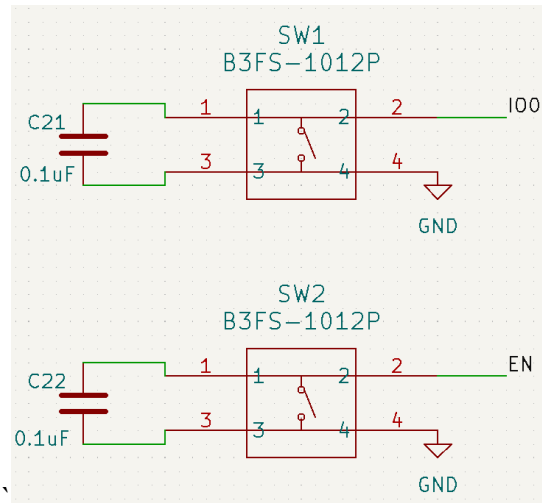
Figure 21: Manual Boot and Reset Button Schematics
