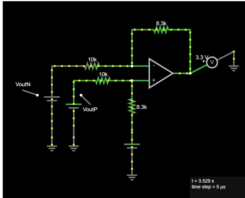
Figure 13: Summing Amp Simulation
