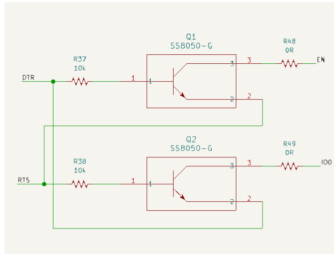
Figure 22: Auto Program Circuit Schematic
