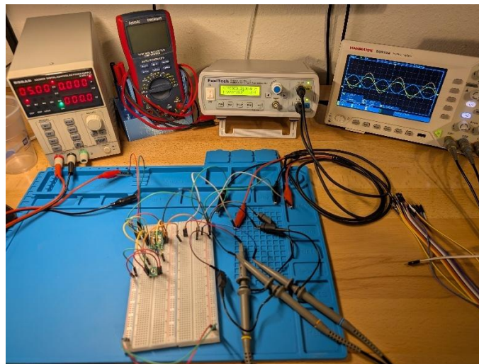
Figure 41: Dual to Single Ended Conversion Stage Testing
