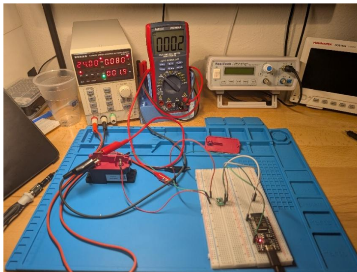
Figure 42: Contactor Driving Testing
