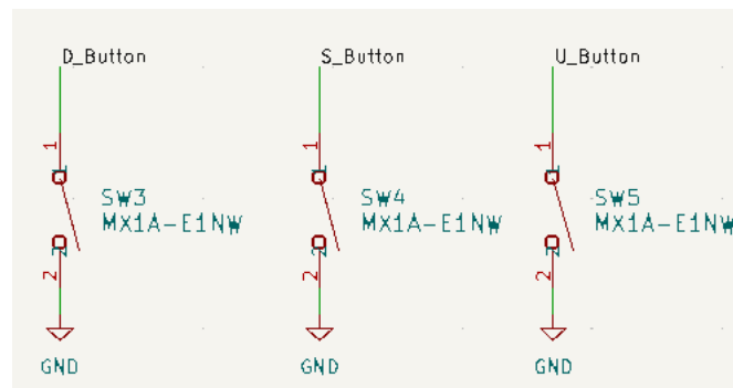
Figure 19: User Input Buttons Schematic
