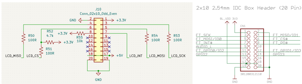
Figure 17: Board and Display Header Comparison
