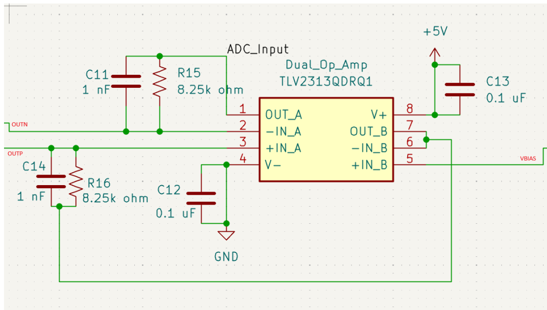
Figure 12: Low Side of Isolation Amplifier
