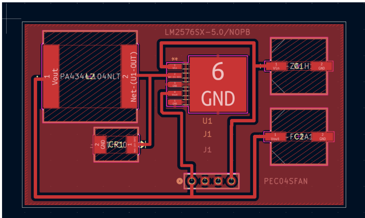
Figure 39: LM 2576 5V regulator board
