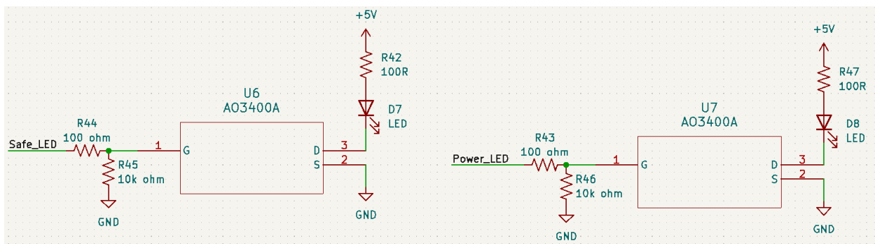
Figure 18: Safe and Power LED Schematic
