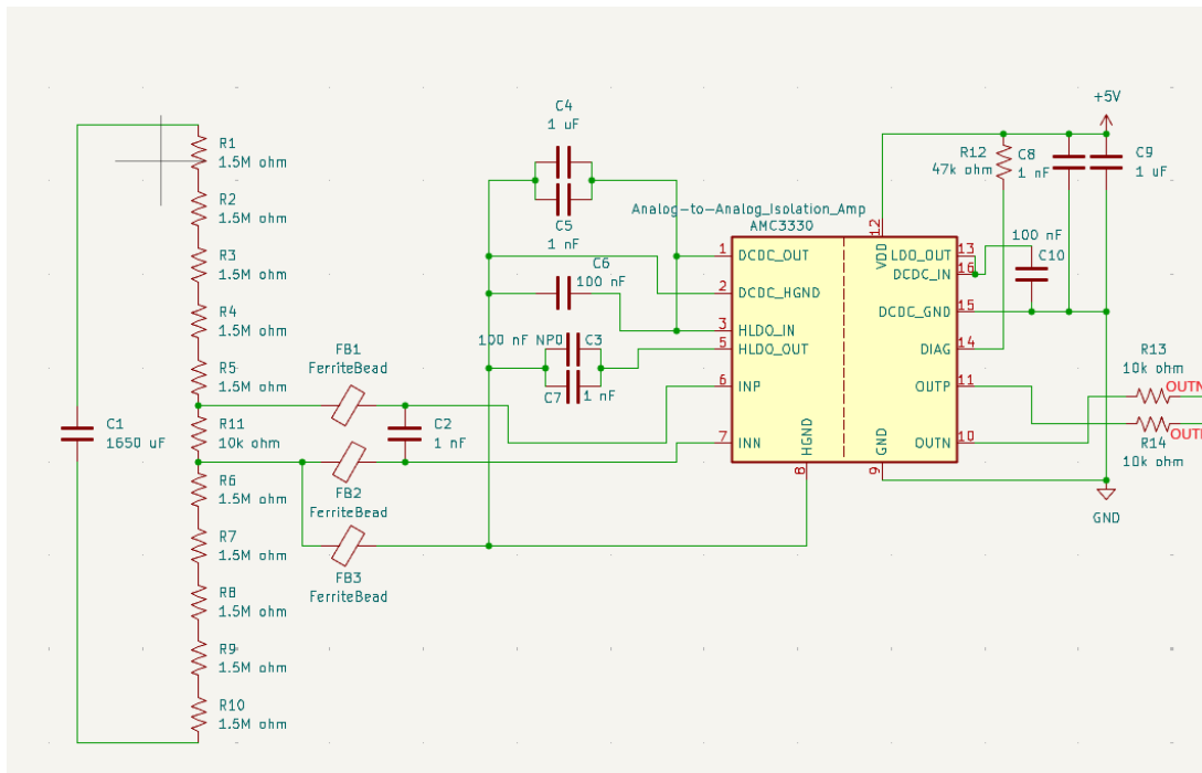
Figure 11: High Side of Isolation Amplifier
