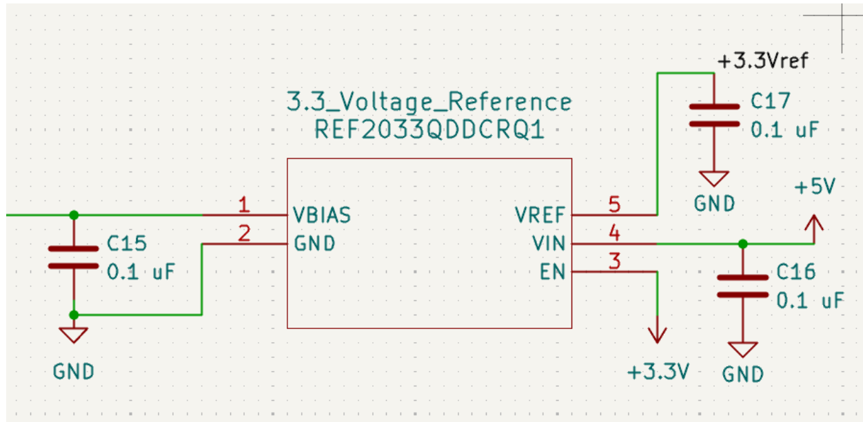
Figure 14: Voltage Reference Schematic
