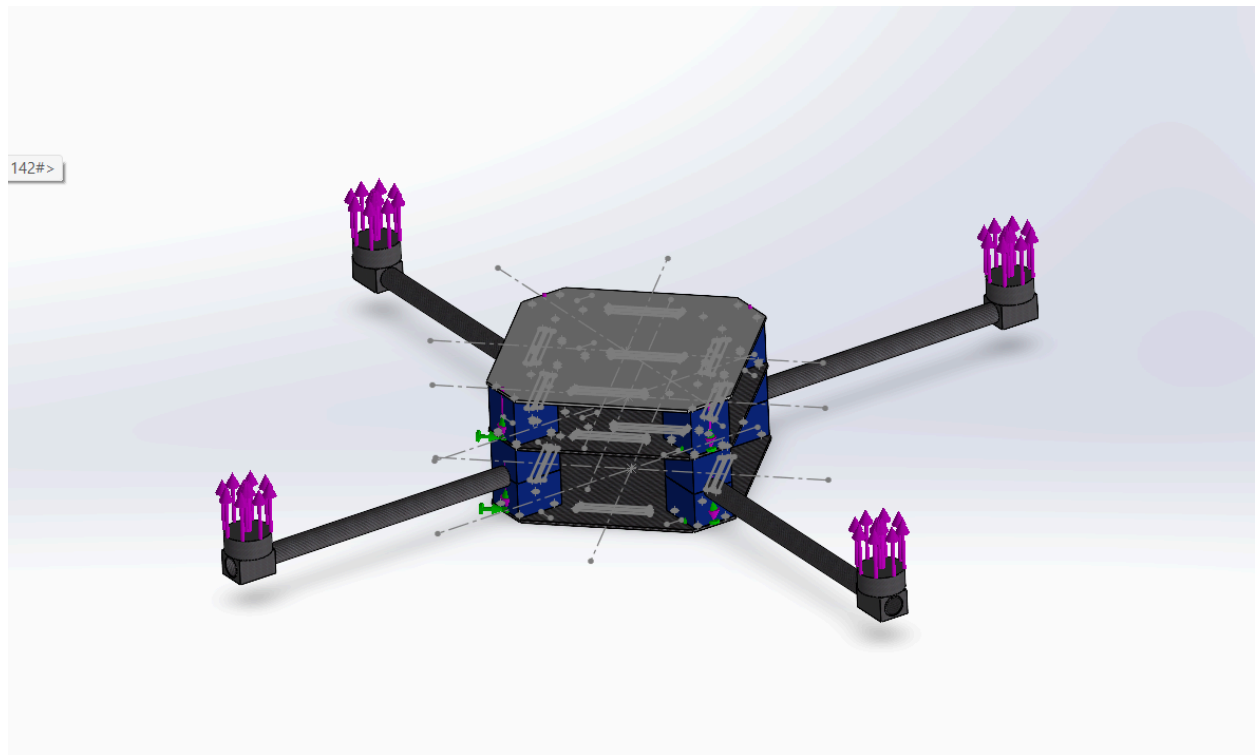
Figure 6.2.1.1 FEA Set-Up of Loads and Meshing
