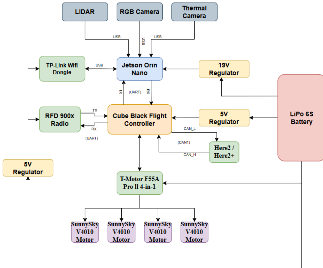
Figure 7.1 SOAR System-Level Electronic Architecture
