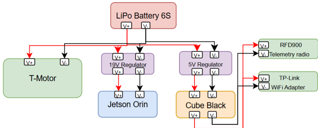
Figure 7.6 Power Supply Wiring
