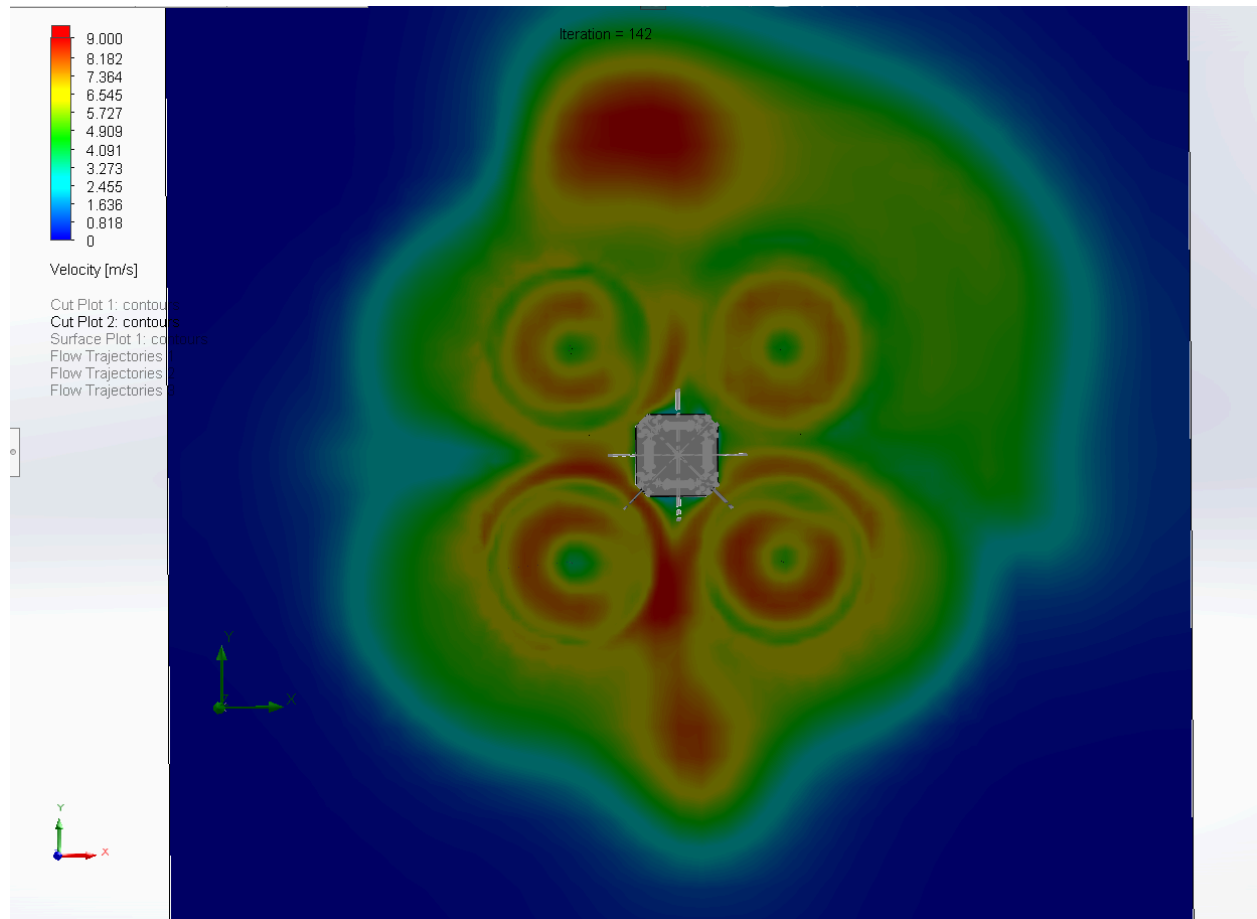
Figure 6.3.3.1 Velocity Contours at Propellers (Top)
