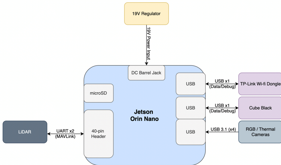
Figure 7.3 Jetson Orin Connectivity Diagram
