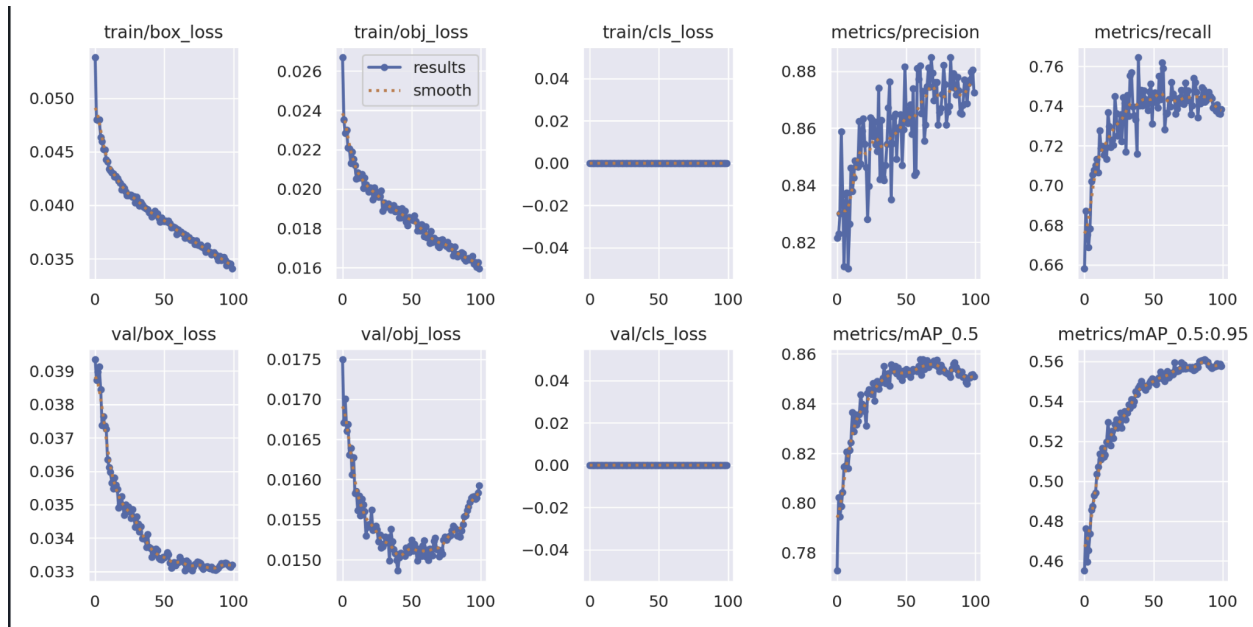
Figure 10.1.8 Model 8 Datasets Performance
