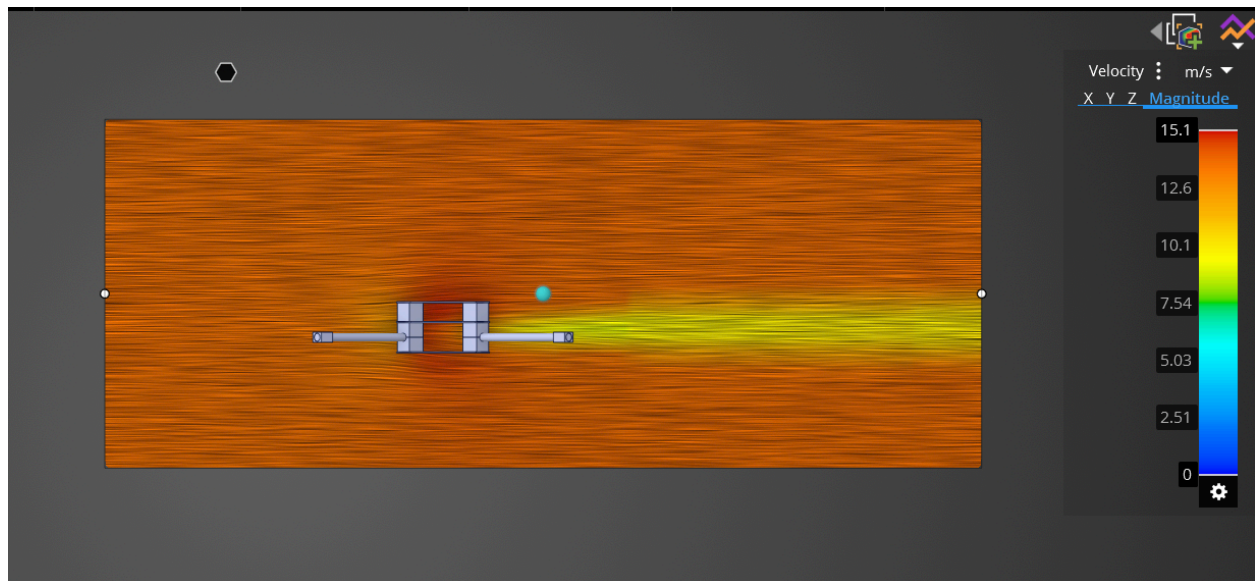
Figure 6.3.2.1 Drag Analysis on Drone Center
