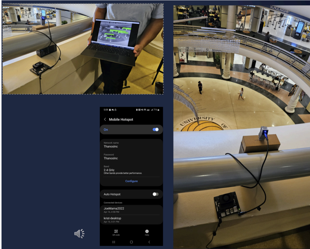
Figure 10.2.1 Testing Procedure Setup
