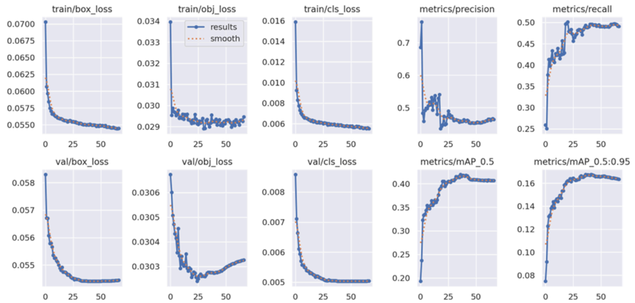
Figure 10.1.4 Model 4 Datasets Performance
