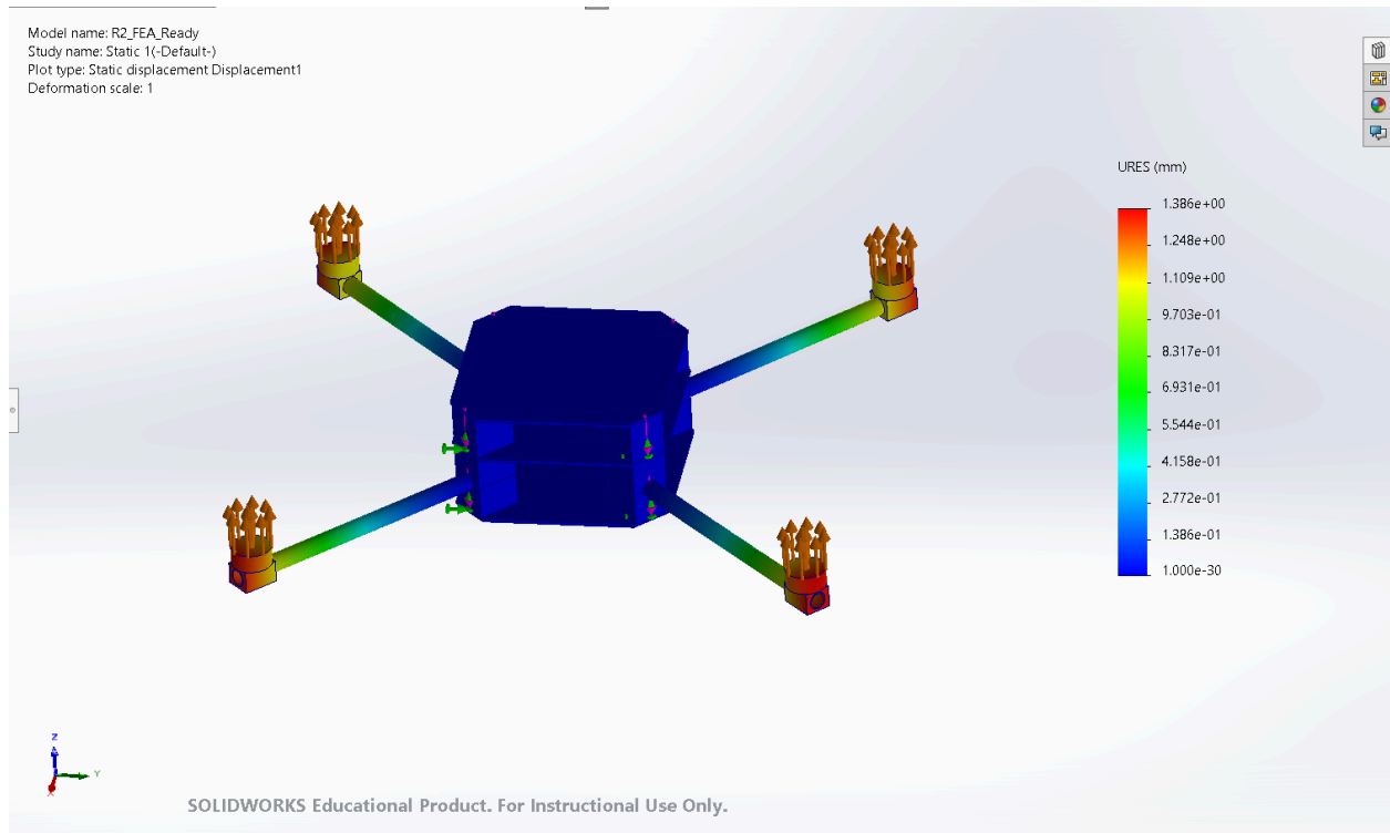
Figure 6.2.2.1 FEA Displacement Results
