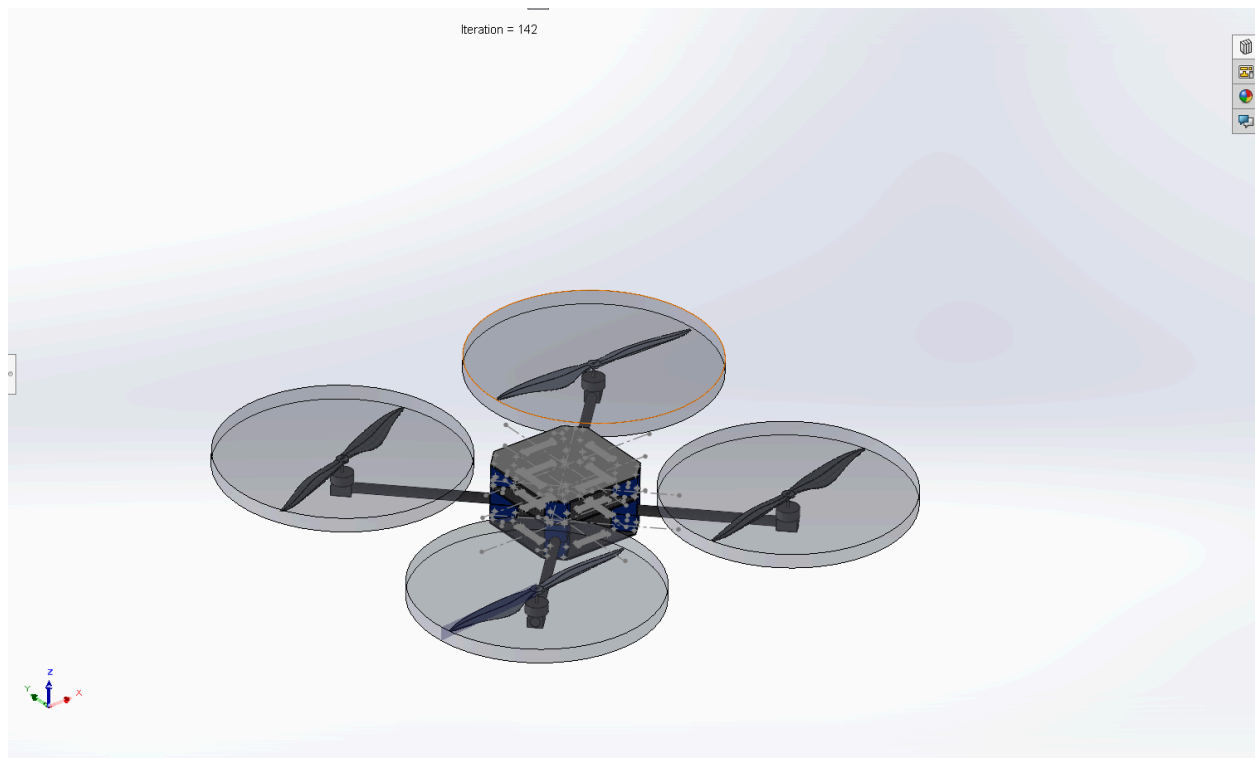
Figure 6.3.1.1 CFD Set-Up of Geometry and Meshing
