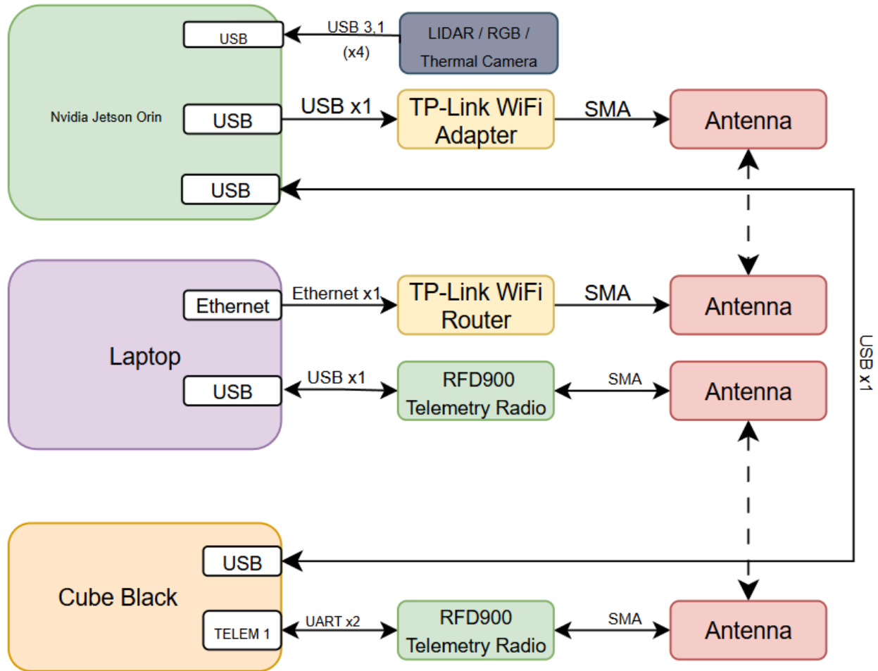
Figure 7.7 Communications Wiring and Signal Flow
