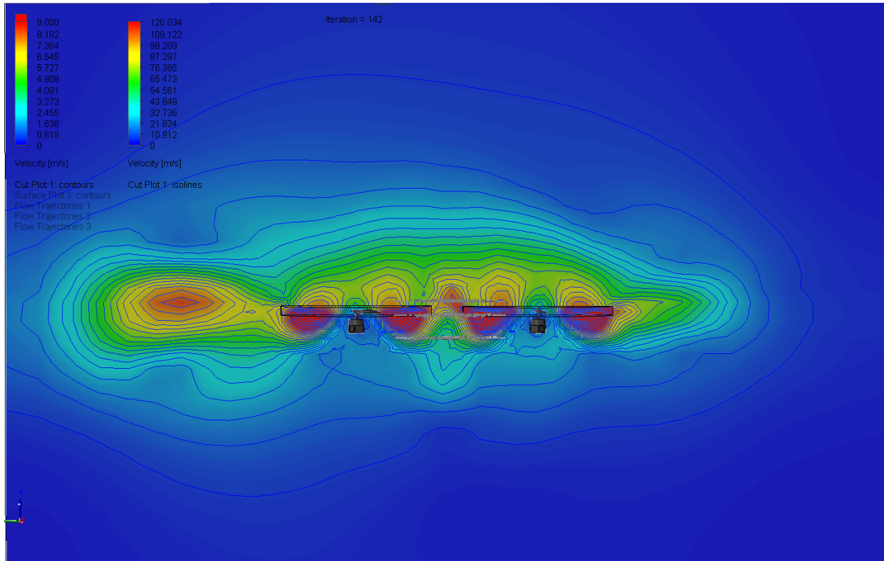
Figure 6.3.3.2 Velocity Contours at Propellers (Side)
