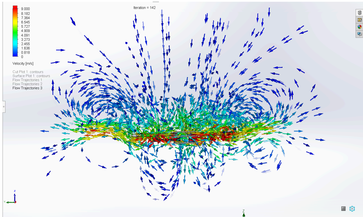
Figure 6.3.3.3 Flow Visualization due to Propeller Rotation
