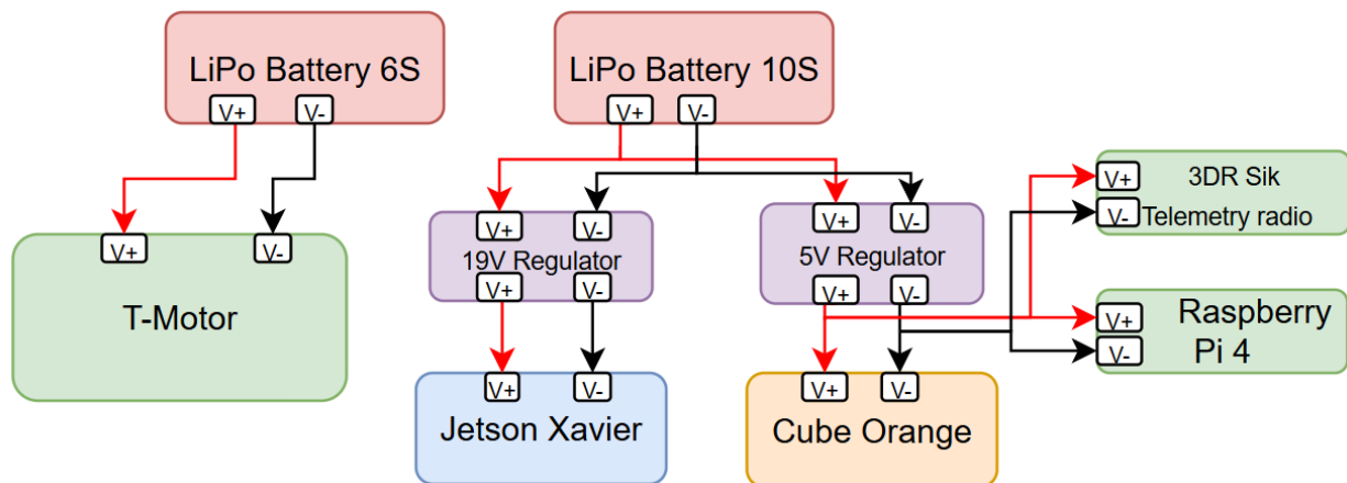
Figure 7.6 Power Supply Wiring By Authors
