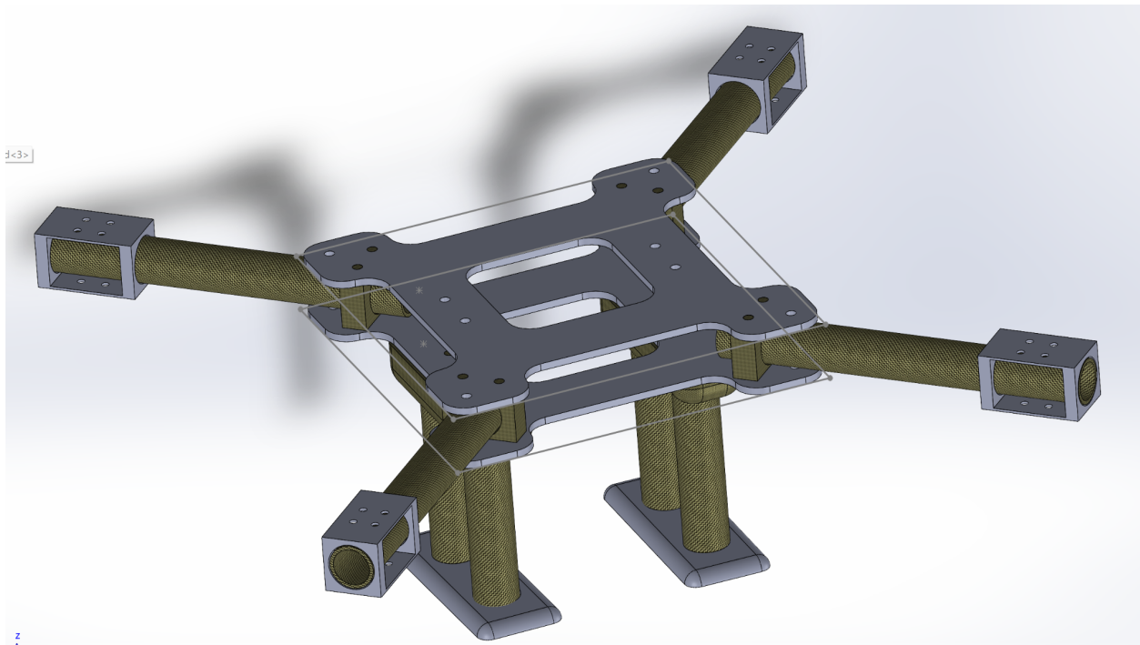
Figure 6.1 Initial CAD Model By Authors
