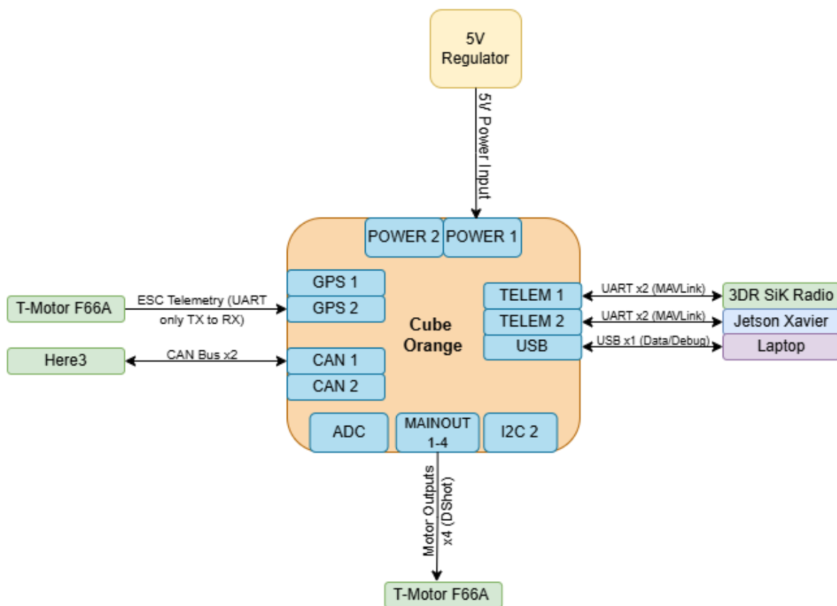
Figure 7.2 Cube Orange Flight Controller Connection Diagram By Authors
