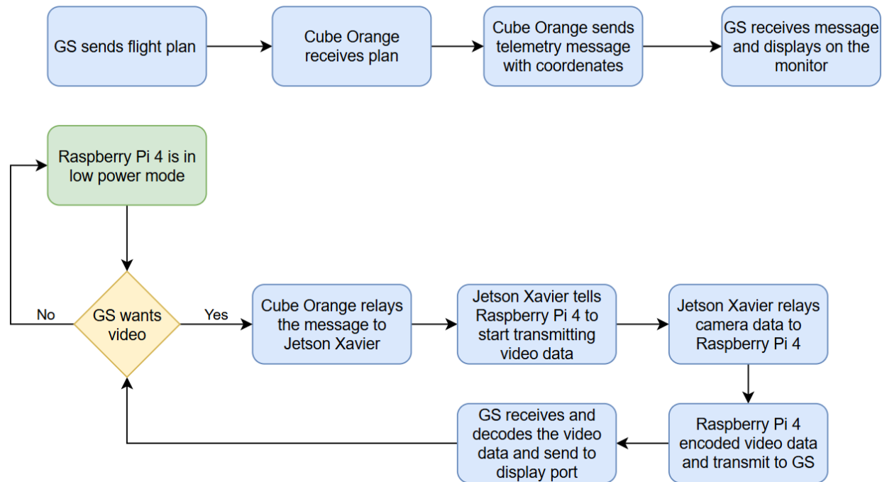
Figure 8.2 Communication Process for Raspberry Pi 4 By Authors
