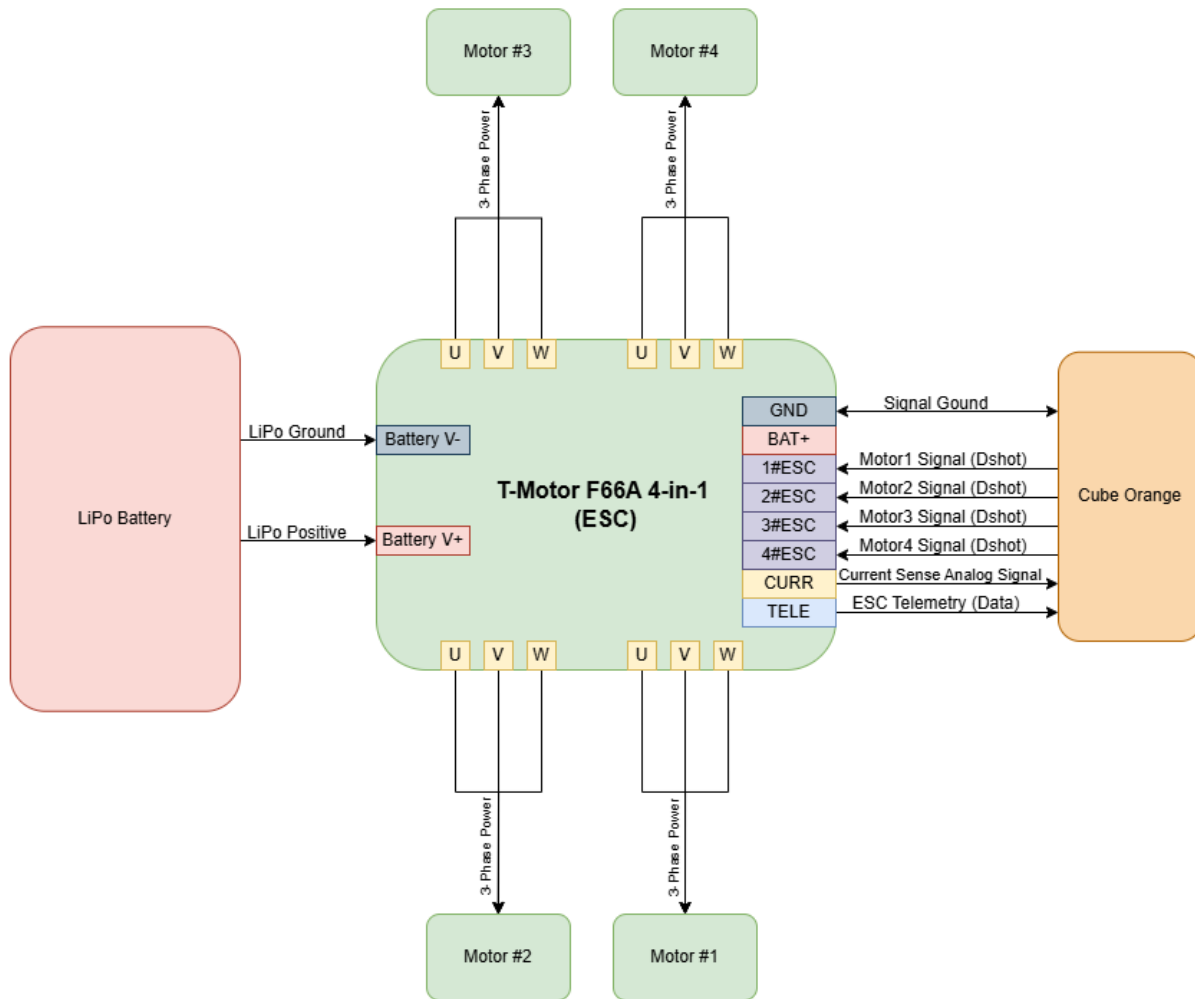
Figure 7.4 T-Motor F66A 4-in-1 ESC Wiring and Signal Flow By Authors
