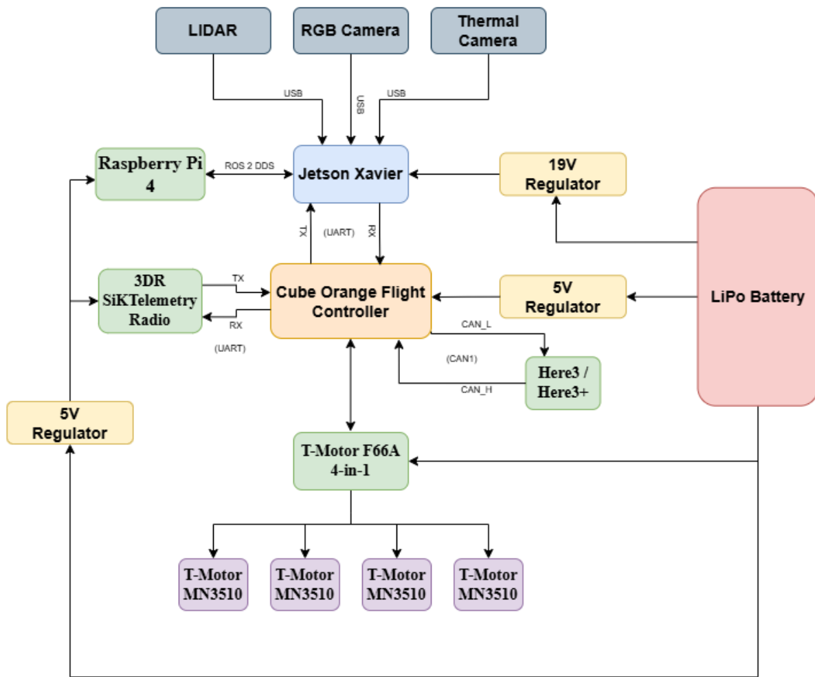
Figure 7.1 SOAR System-Level Electronic Architecture By Authors
