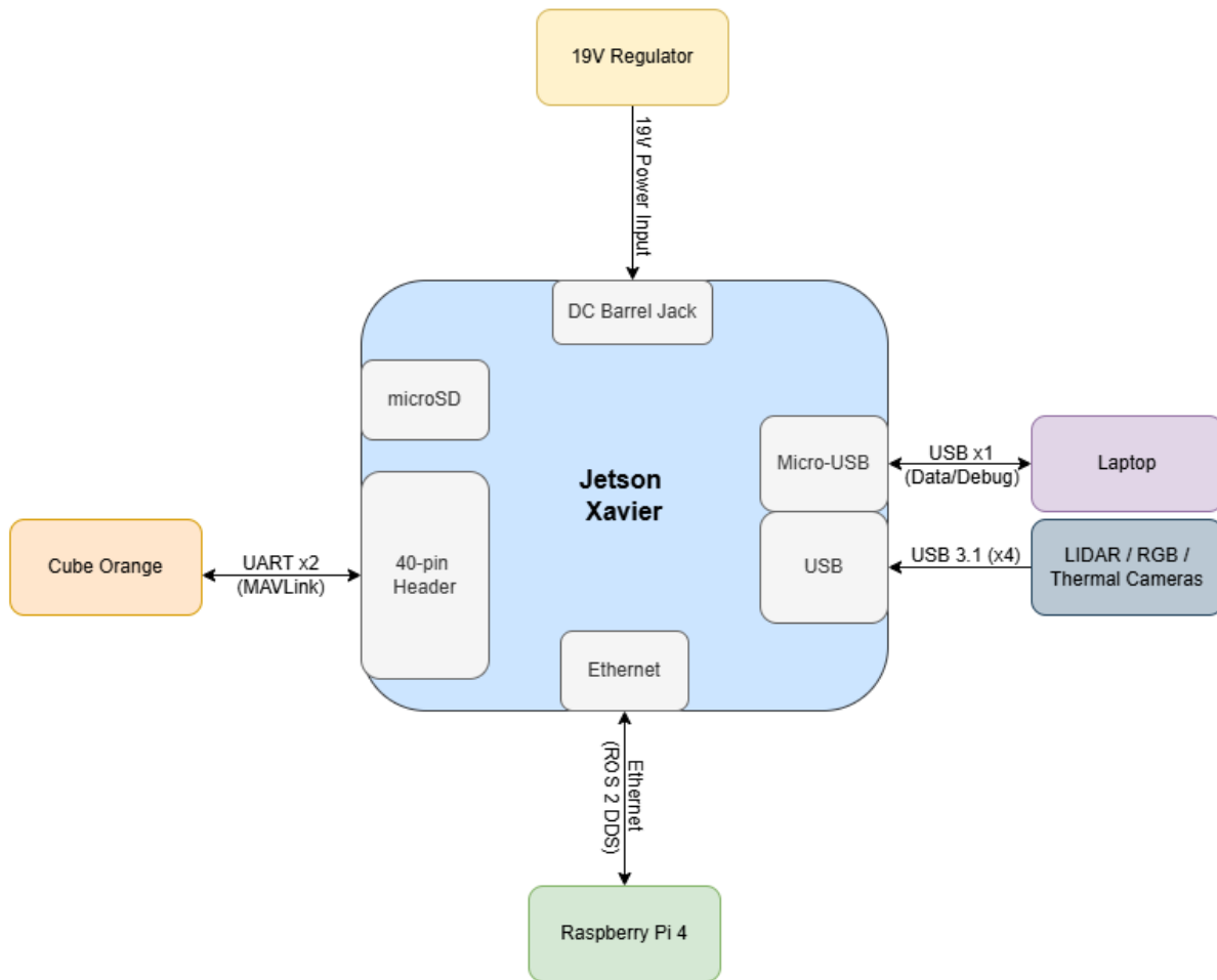
Figure 7.3 Jetson Xavier Connectivity Diagram By Authors
