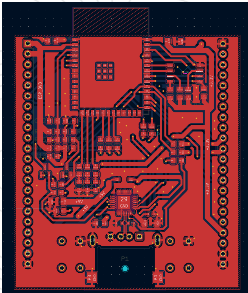
Trace Layout
