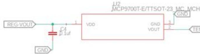
Temperature Sensor
