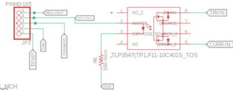
Solid-State Relay
