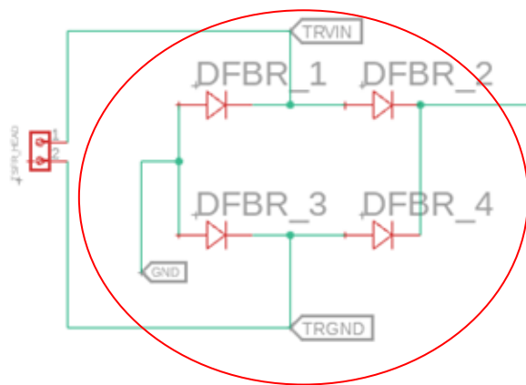
Full-Wave Rectifier
