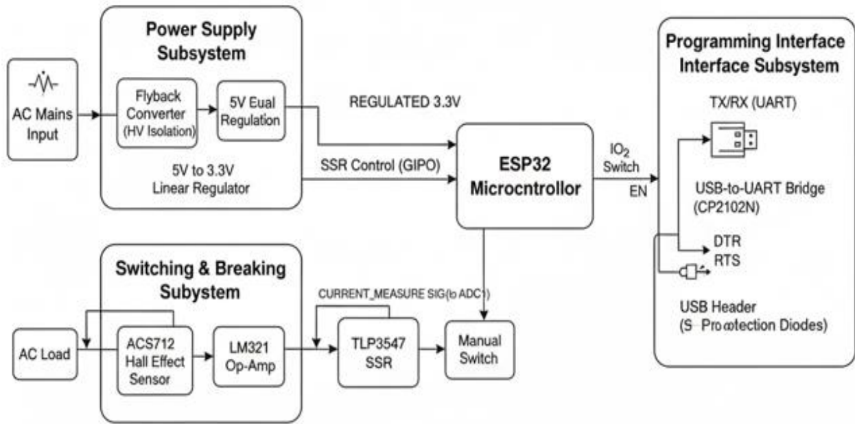
Figure 6.1: Hardware Block Diagram
