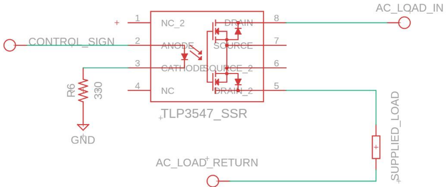
Figure 6.2: Current Switching Subsystem by Authors
