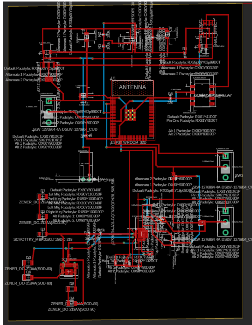
Figure 8.1: Main PCB Layout (Wiring Diagram)
