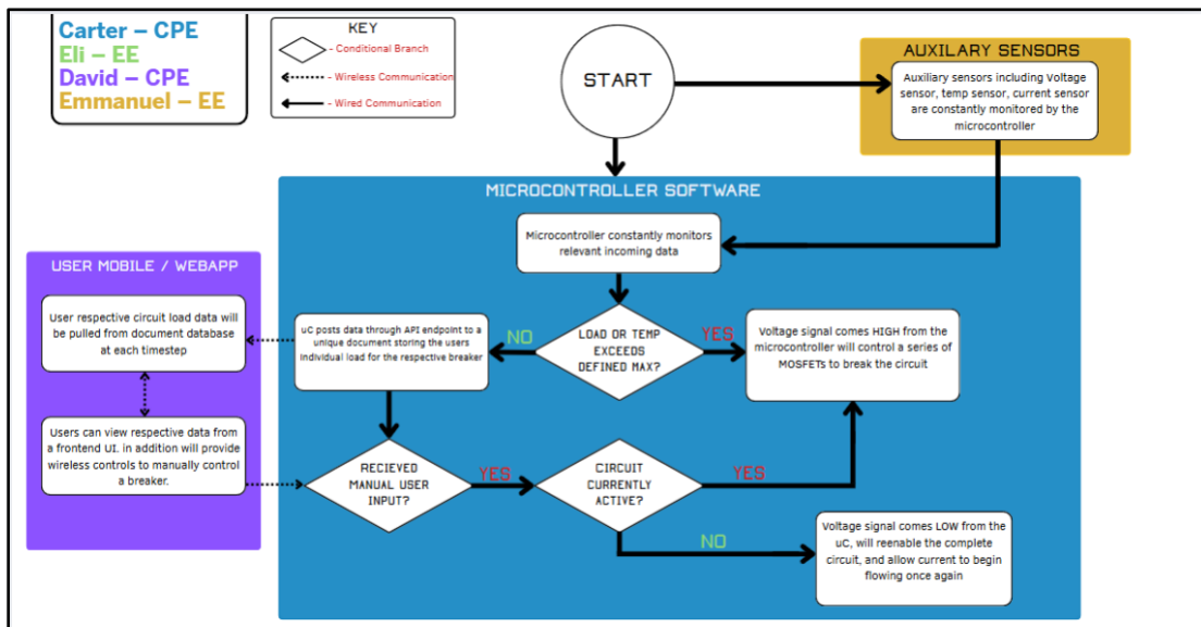
Figure 2.2: Software Block Diagram
