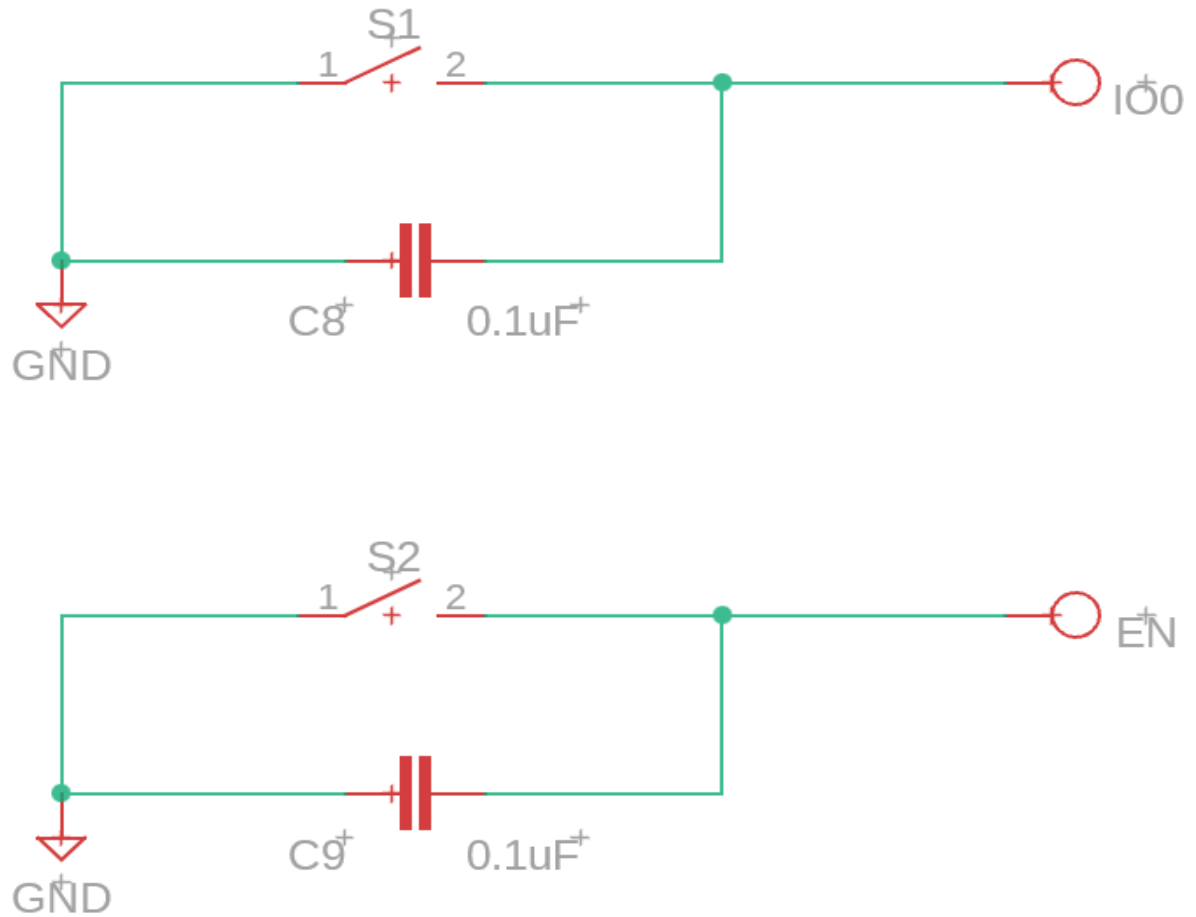
Figure 6.8: Manual Programming Schematic by Authors
