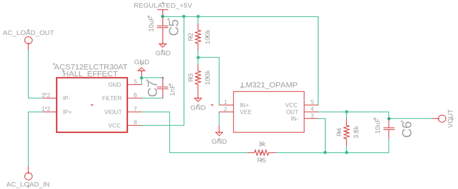
Figure 6.3: Current Measuring Subsystem Authors
