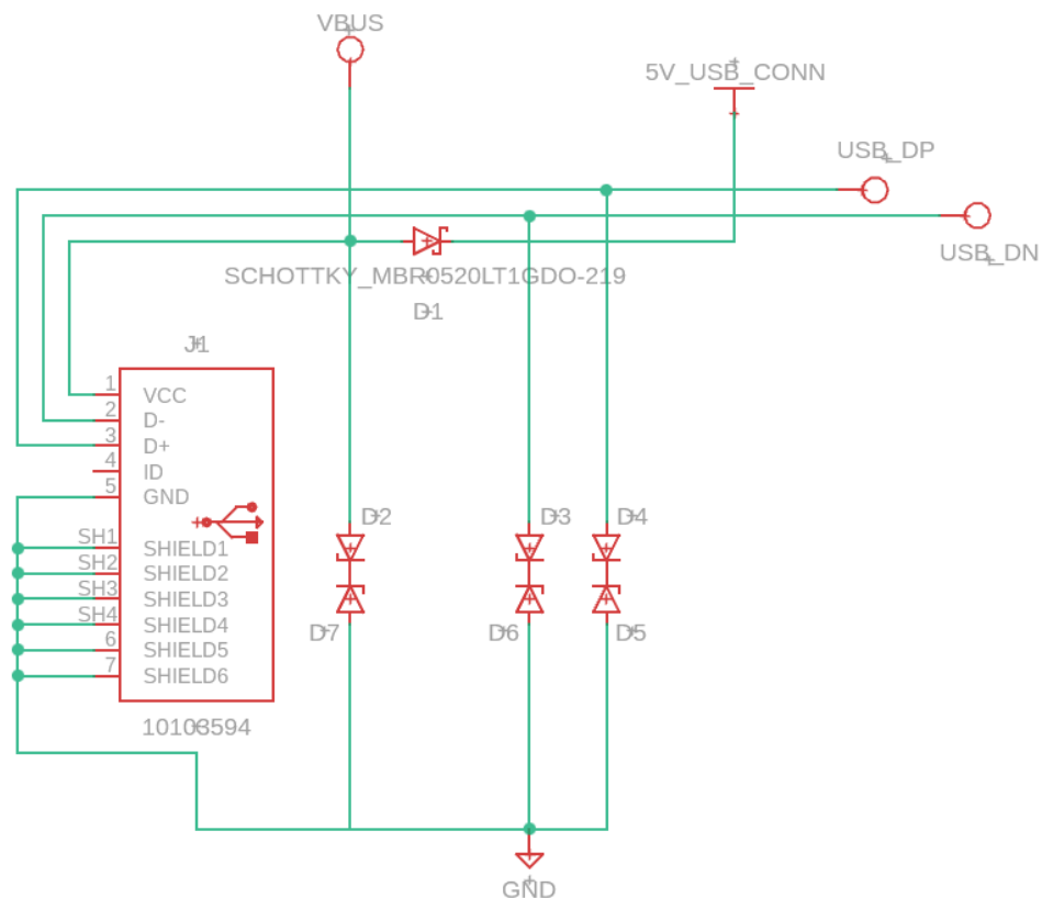
Figure 6.5: USB Header Schematic by Authors
