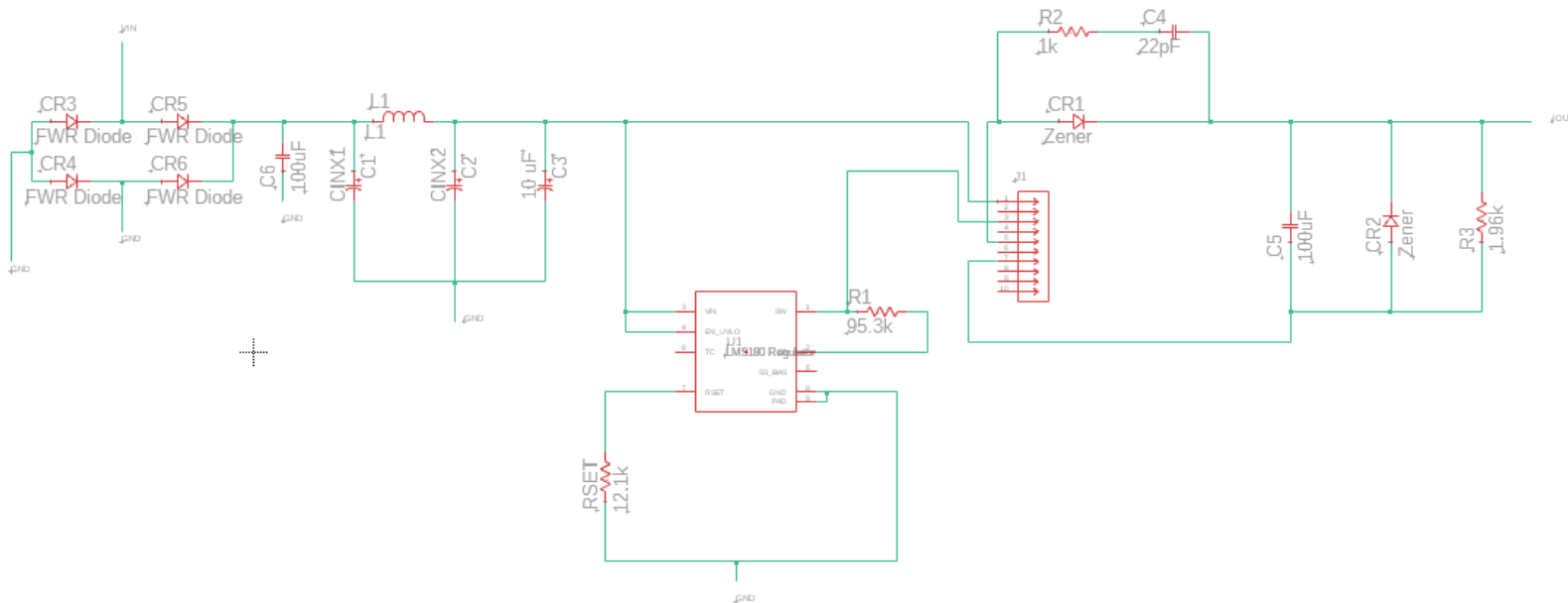
Figure 6.2: Flyback Buck Converter by Authors
