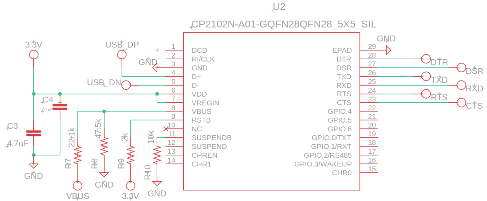
Figure 6.6: UART Bridge Controller Schematic by Authors
