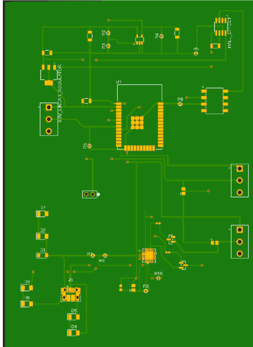
Figure 8.2: Main PCB Layout (Manufacturing Preview)
