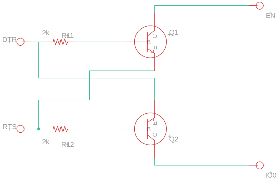
Figure 6.7: Automatic Programming Schematic by Authors
