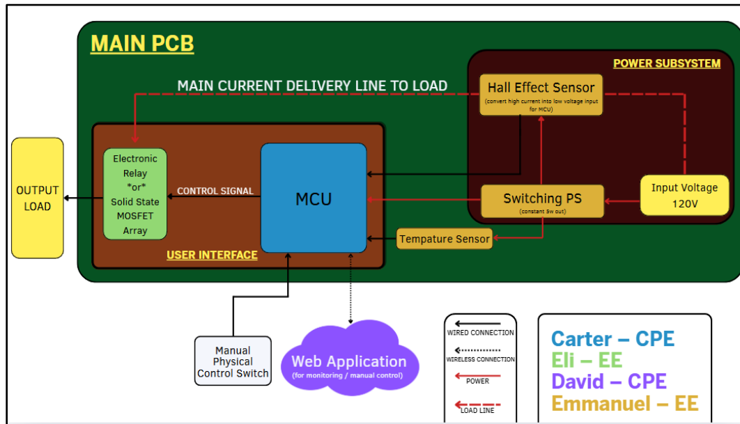
Figure 2.1: Hardware Block Diagram
