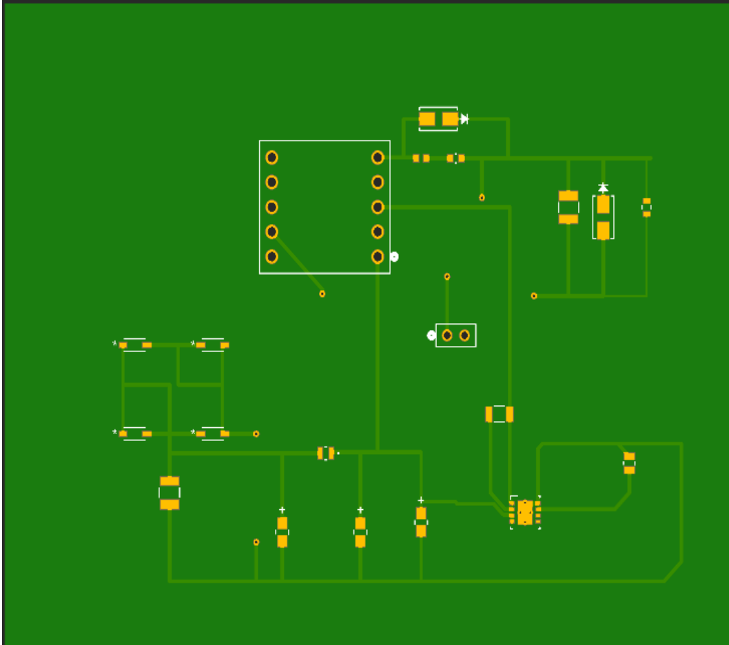
Figure 8.4: SMPS/Rectifier Manufacturer Preview
