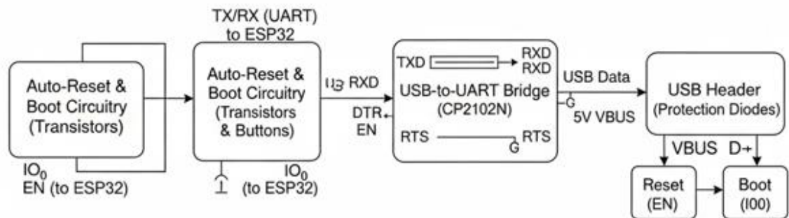
Figure 6 4: Programming Interface Block Diagram
