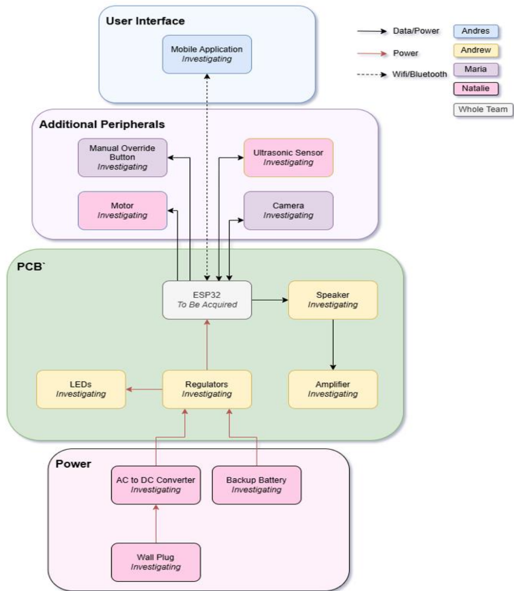
Figure 1: Hardware Diagram by Authors
