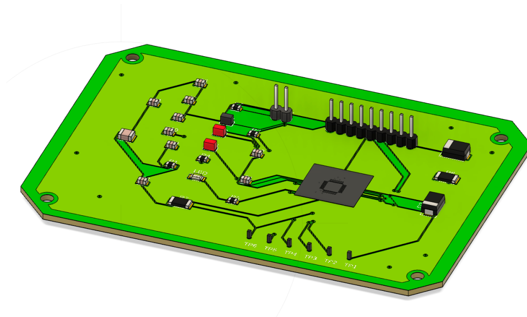
Figure 3228: 3D of Motor Driver Board
