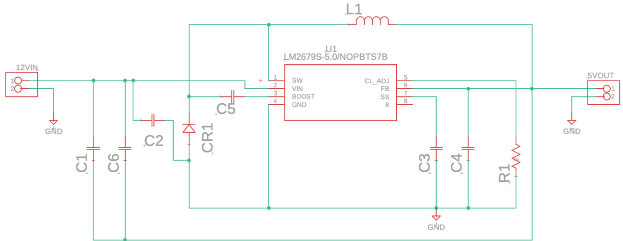
Figure 7: 5V Voltage Regulator Schematic
