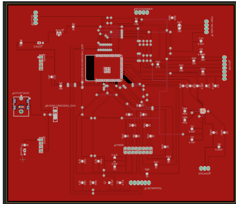
Figure 3329: PCB Layout (With Ground Polygon)
