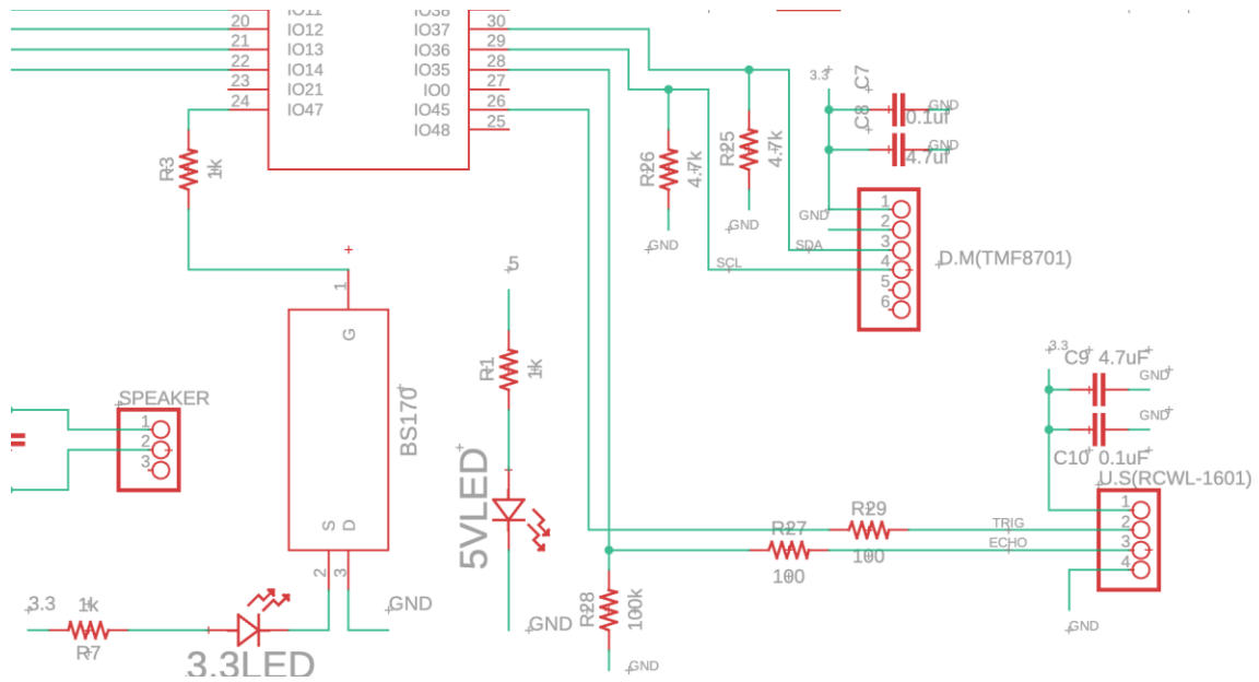
Figure 16: Depth Module, Ultra Sonic Sensor, 3.3 & 5V LEDs
