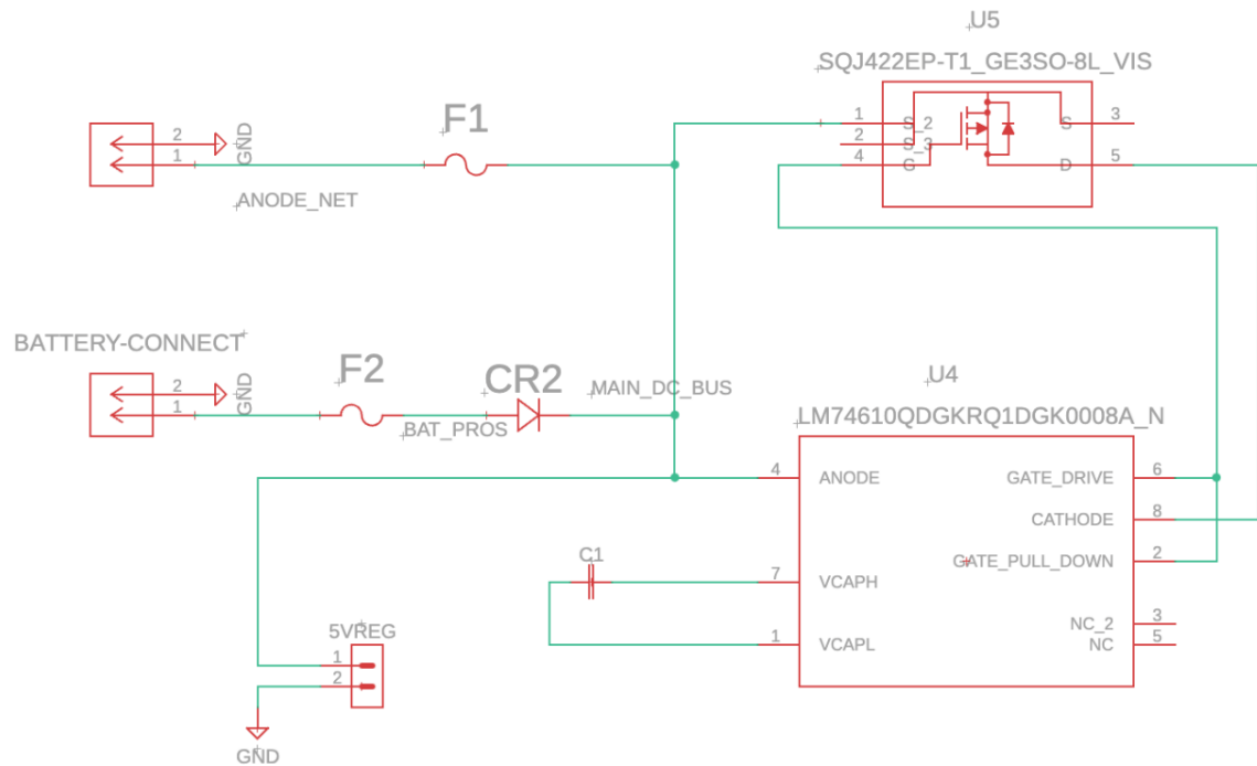
Figure 9: Battery Backup Schematic
