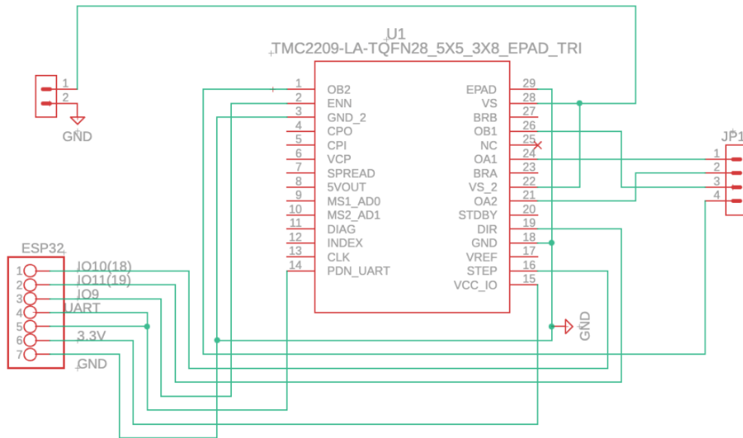
Figure 11: Motor Driver Schematic
