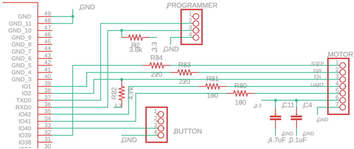
Figure 15: Programmer, Motor, and Button Close-Up
