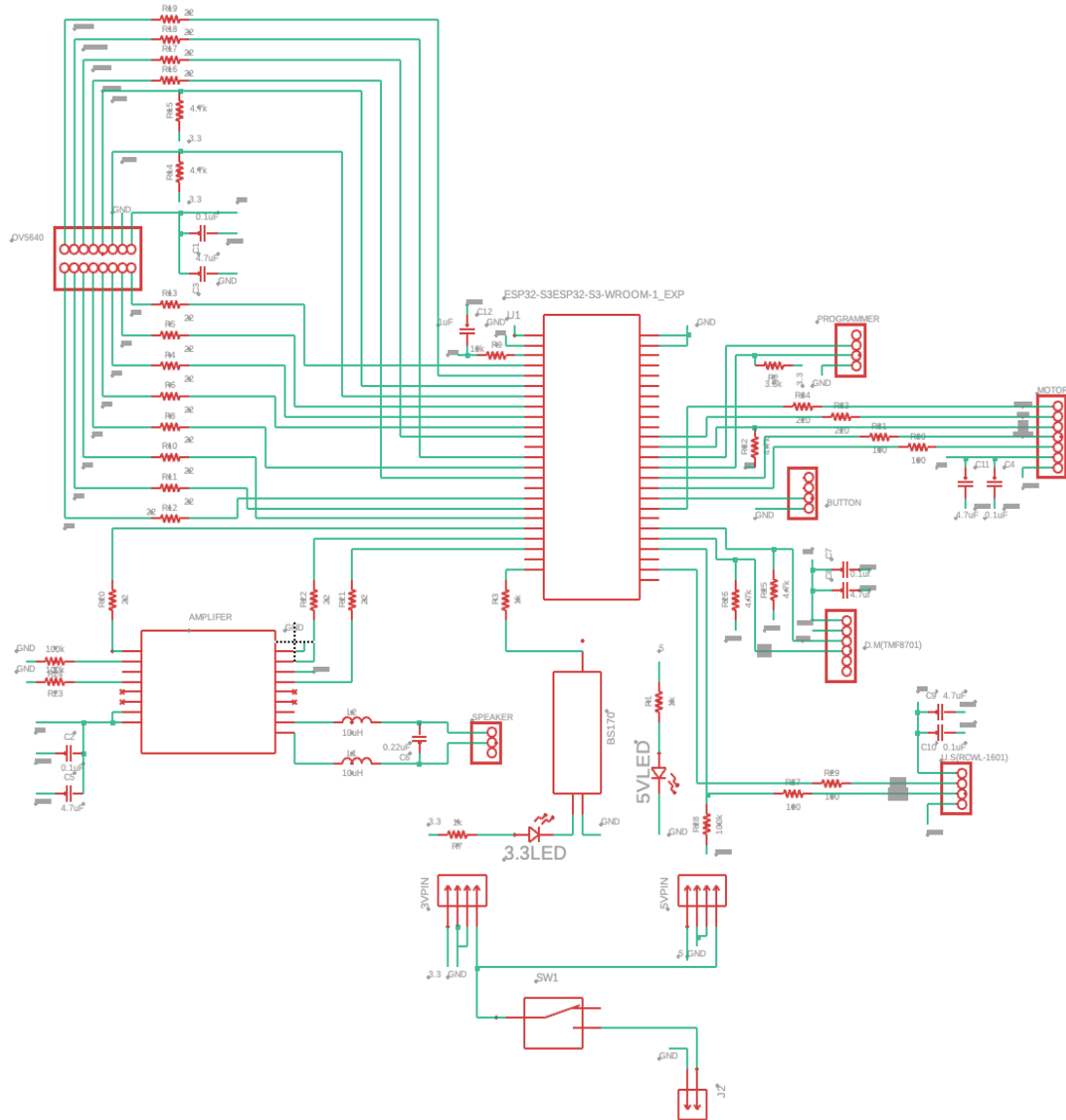
Figure 12: Entire MCU Schematic
