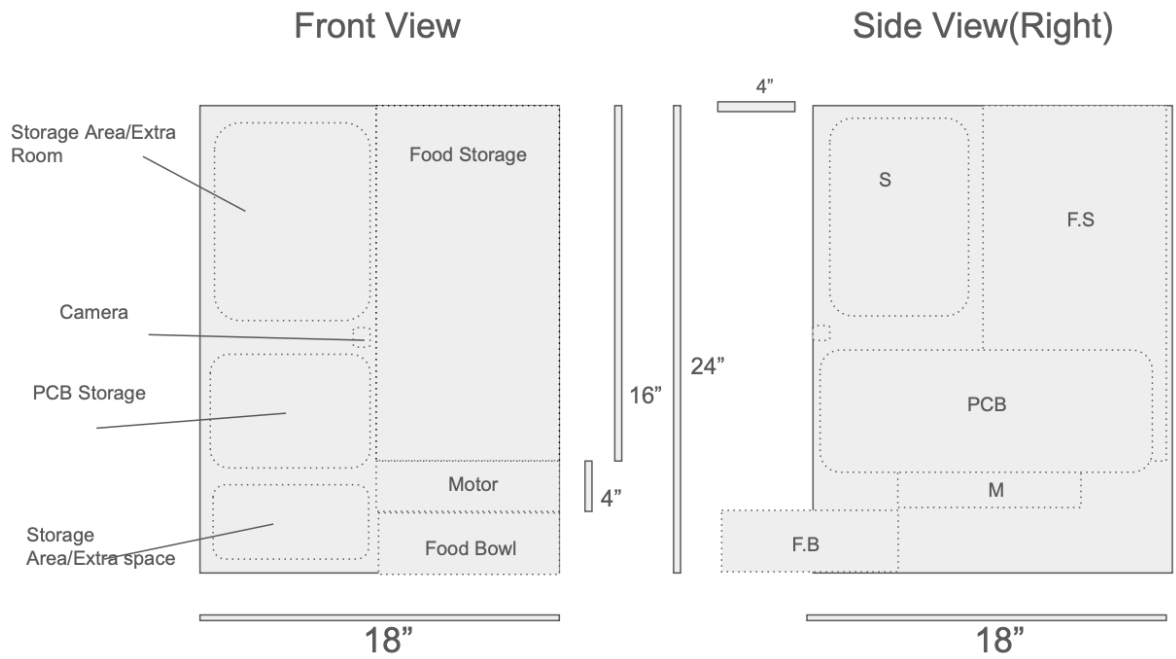
Figure 4: Prototype Illustration
