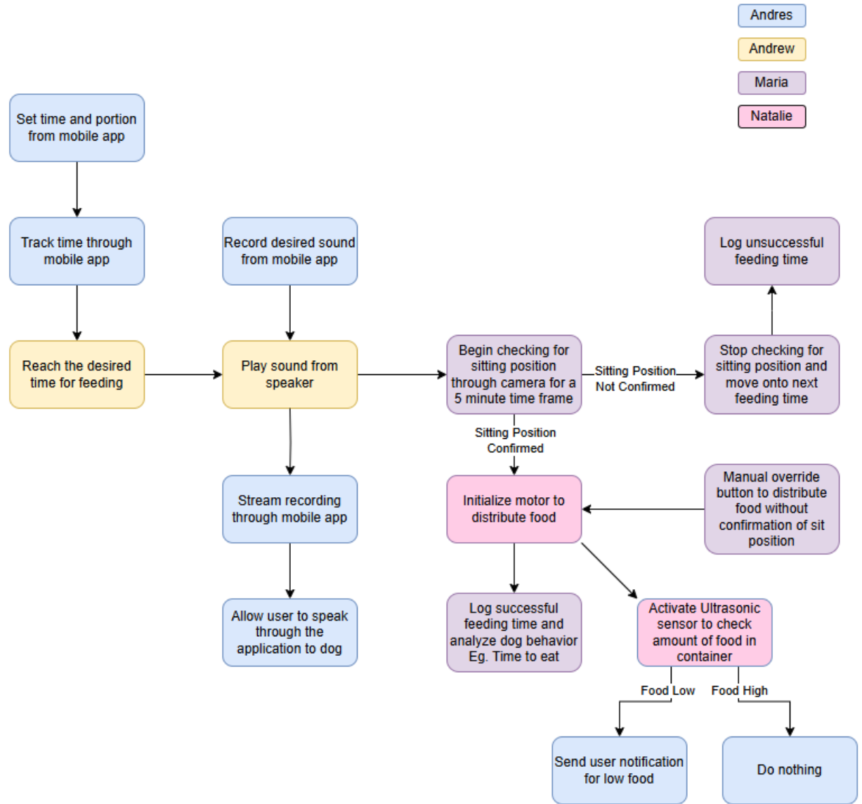
Figure 2: Software Diagram by Authors
