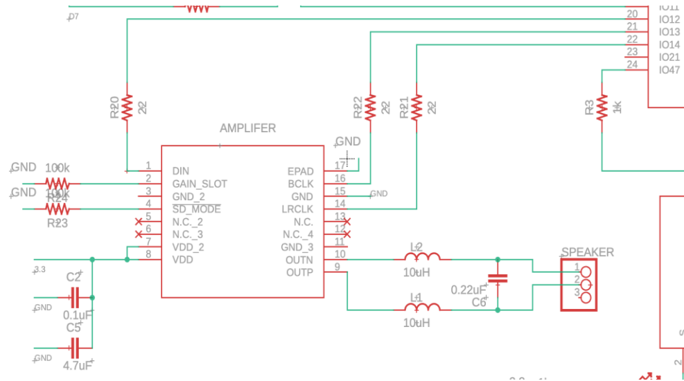
Figure 14: MAX98357A Amplifier and Speaker Schematic Close-Up
