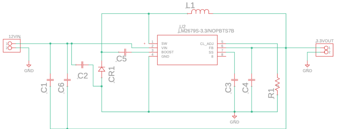
Figure 8: 3.3V Voltage Regulator Schematic
