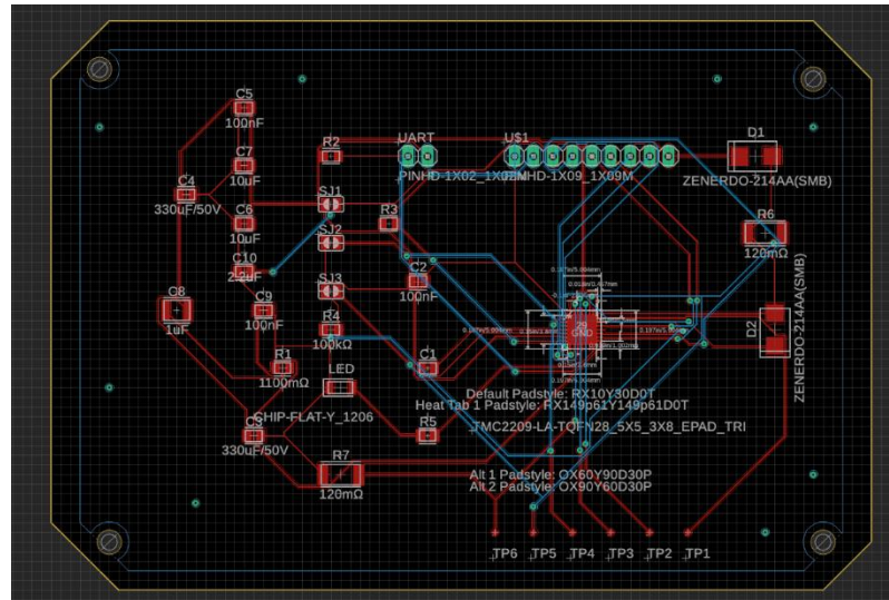
Figure 3127: Motor Driver PCB
