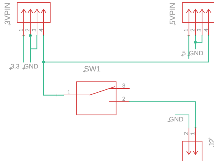
Figure 17: Regulator Headers and Power Input Schematic
