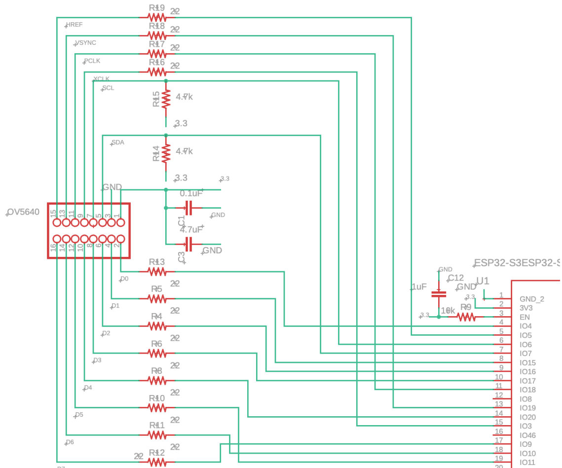
Figure 13: OV5640 Camera Schematic Close-Up
