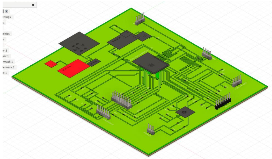
Figure 35: 3D View of PCB
