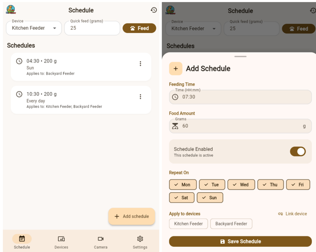
Figure 2320: Schedule Page and Add Schedule Widget
