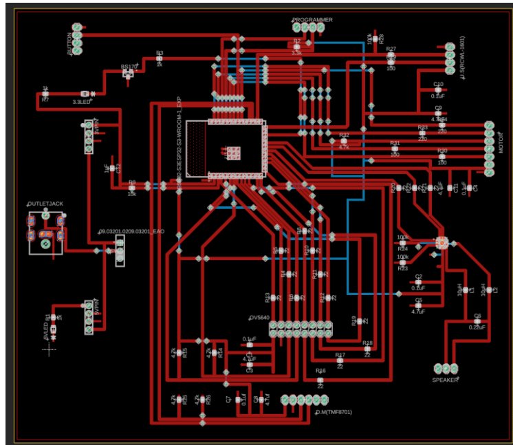
Figure 34: PCB Layout (Ground Polygon Hidden)
