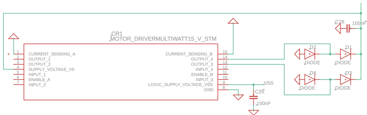
Figure 6.6 Motor driver schematic
