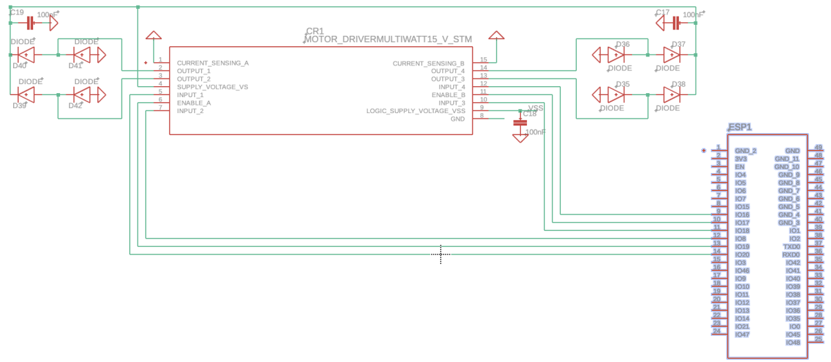
Figure 6.7 Motor driver to ESP schematic
