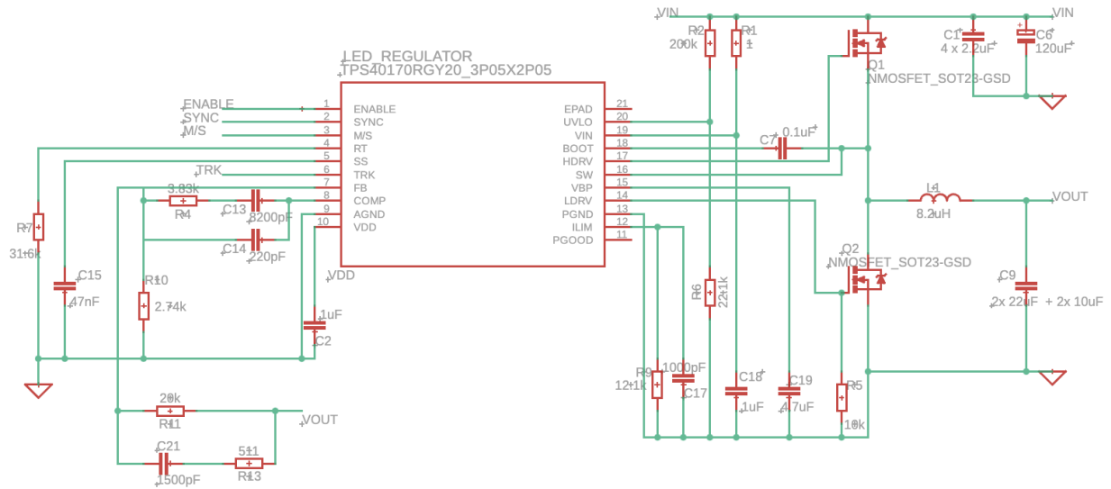
Figure 6.1 LED regulator schematic
