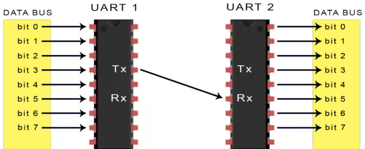
Figure 4.4. Basics of UART Block Diagram by Image Source:
