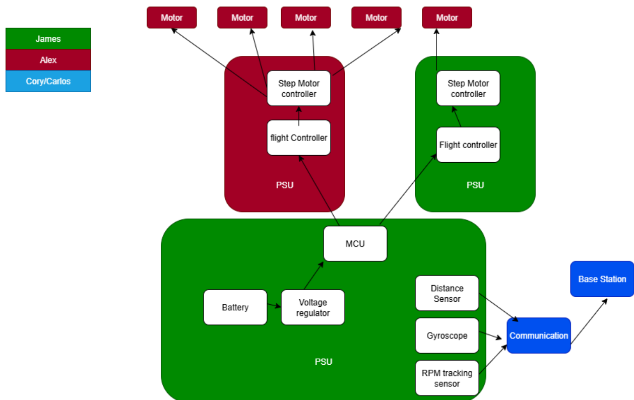
Figure 2.4. Hardware Diagram
