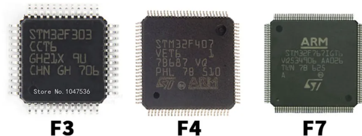
Figure 3.13. Comparison between F4 and F7 (FC)
