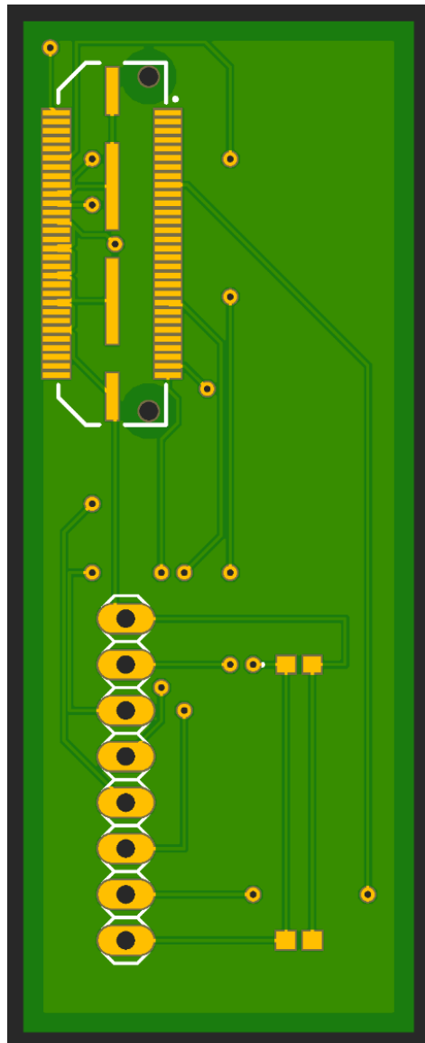
Figure 28: Radar module PCB
