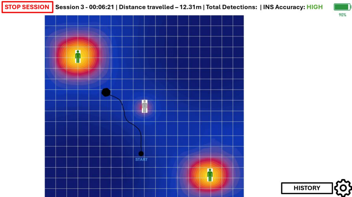
Figure 25: Sketch of Heatmap View.
