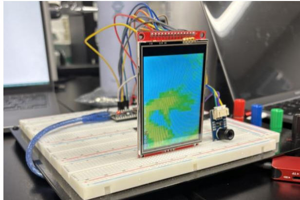
Figure 31: Testing the IR sensor with the LCD.
