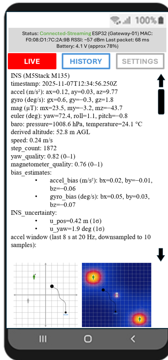
Figure 26: Sketch of Smartphone App UI.
