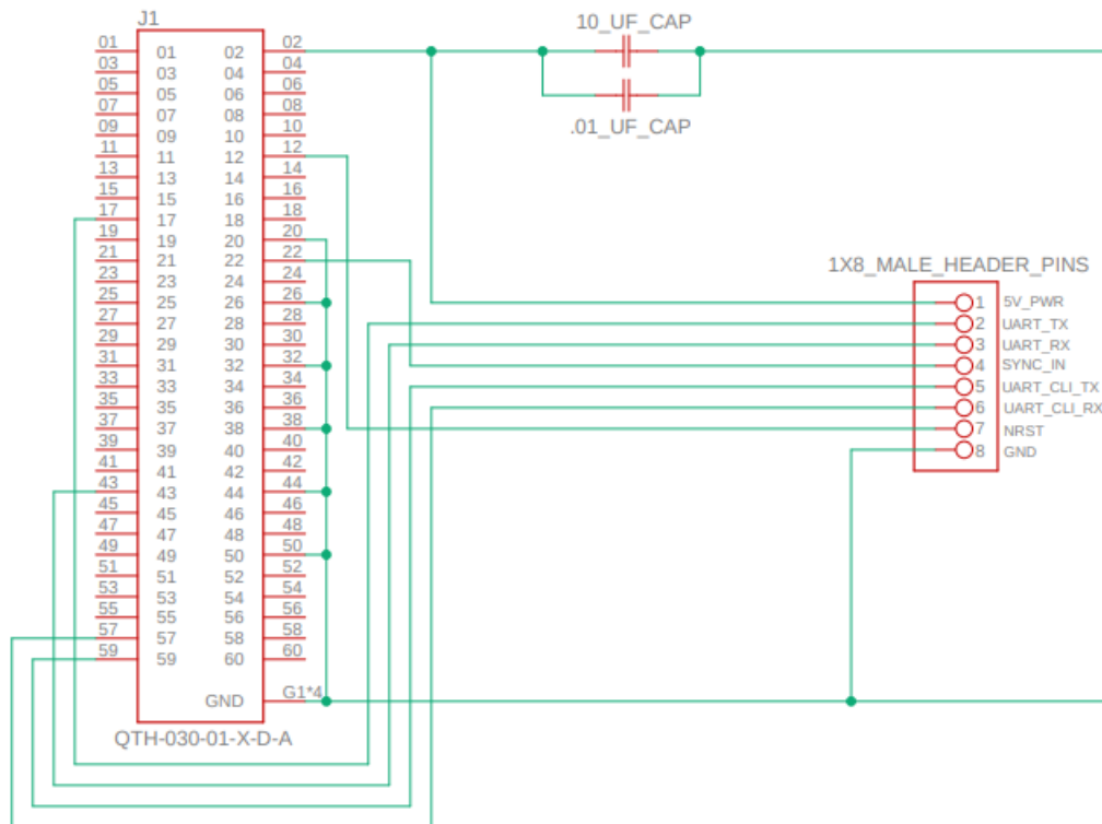
Figure 8: Radar Module PCB Schematic.
