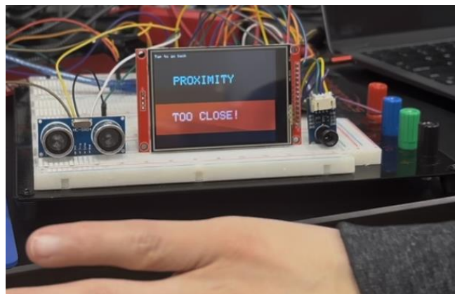
Figure 34: Testing the USS to ensure it displays when someone is too close.
