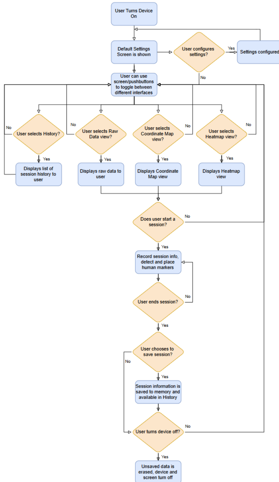
Figure 21: Overall UI Flowchart
