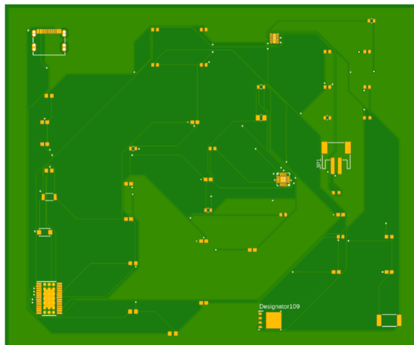
Figure 30: Power Subsystem PCB
