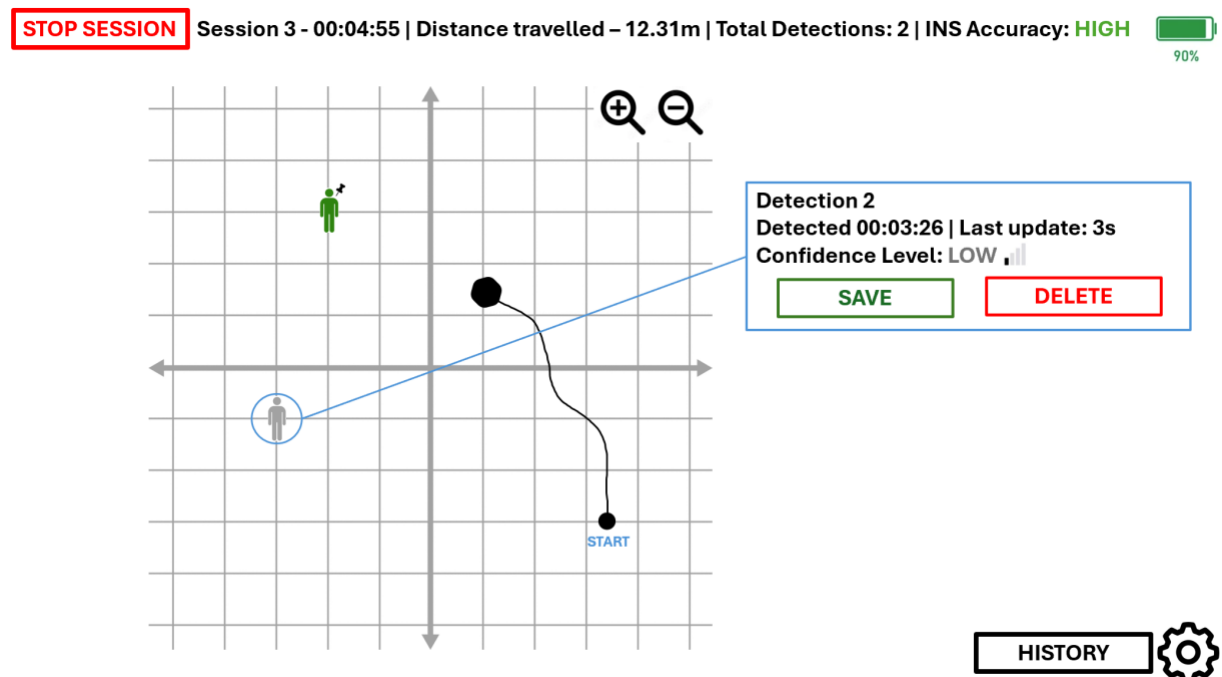
Figure 23: Sketch of Coordinate Map View.
