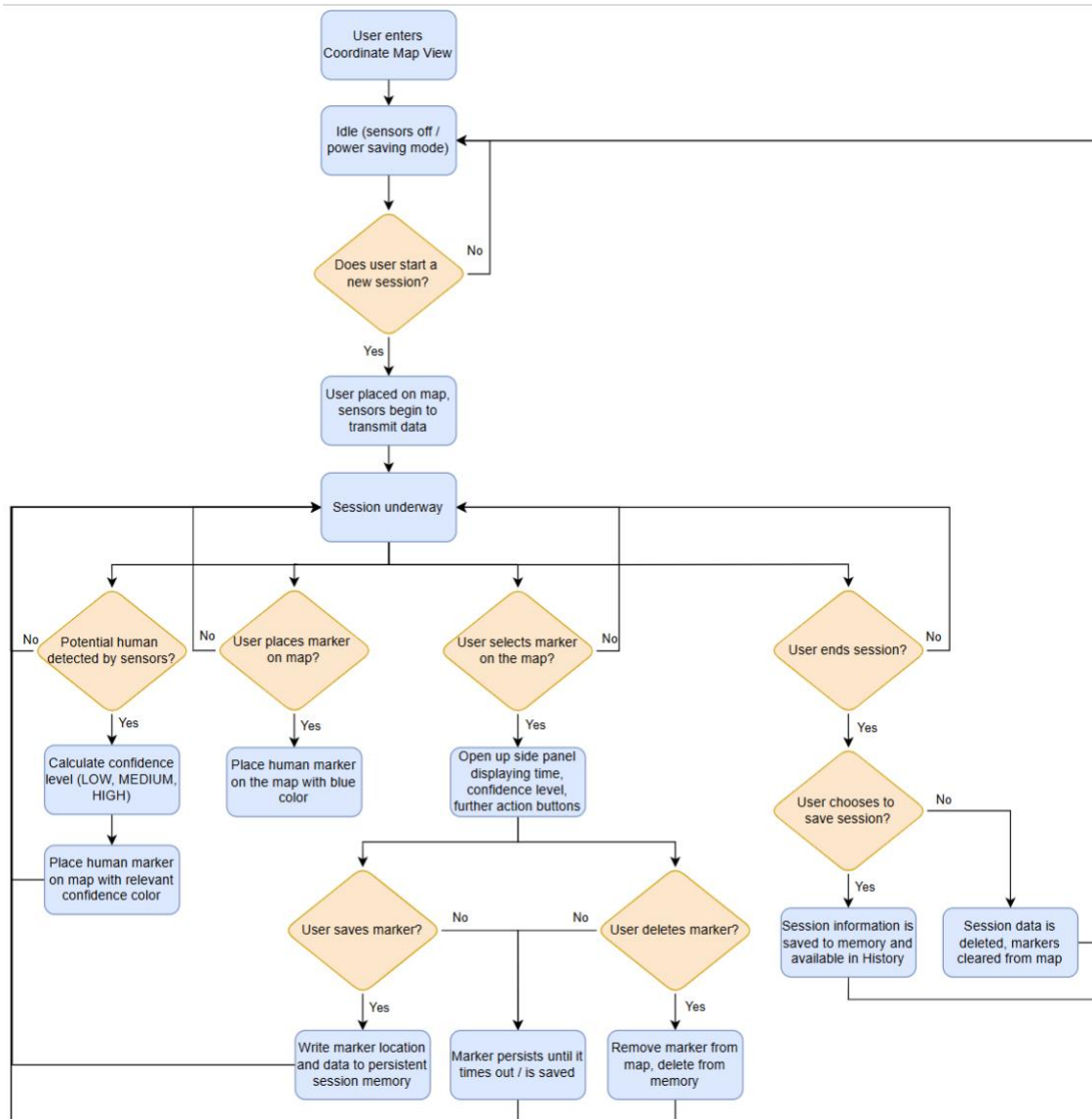
Figure 24: Coordinate Map View Flowchart
