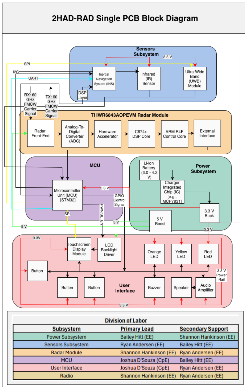
Figure 7: Hardware Block Diagram
