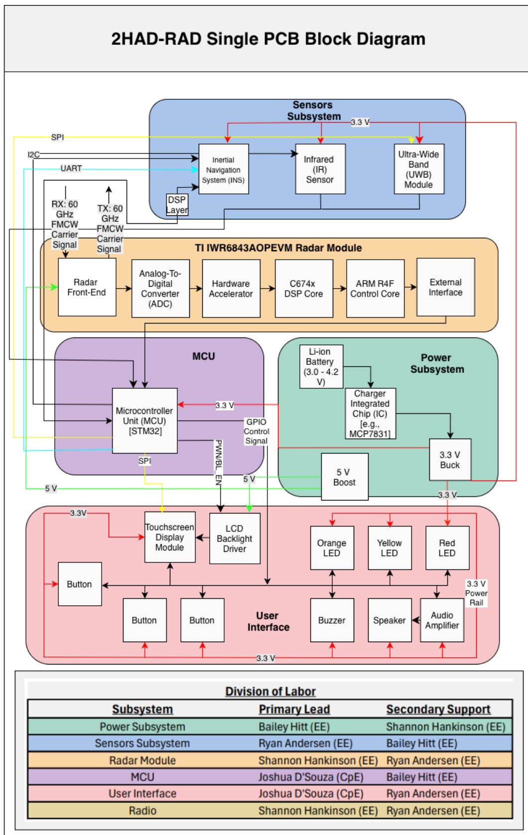
Figure 1: Hardware Block Diagram for 2HADRAD
