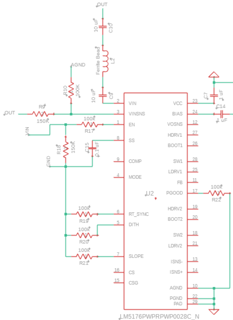
Figure 19: LM5176 Buck-Boost Regulator
