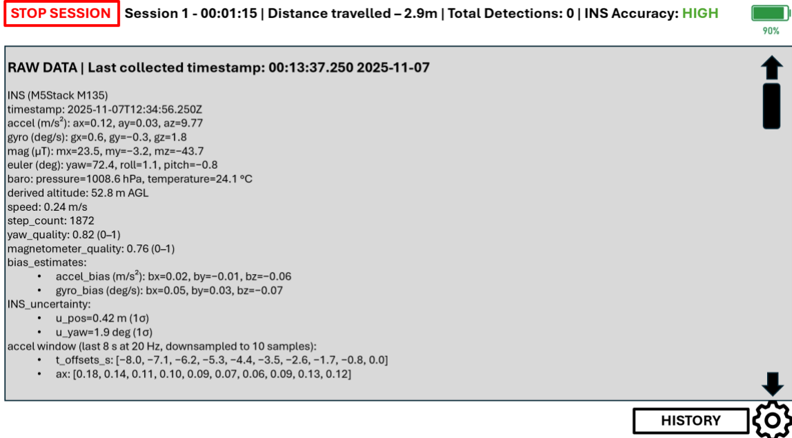
Figure 22: Sketch of Raw Data View.
