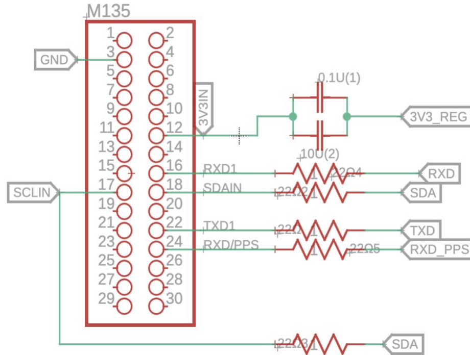
Figure 9: M135 module schematic
