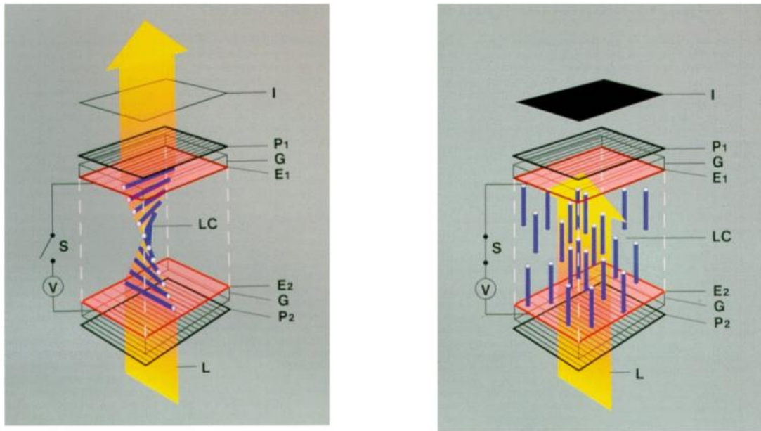
2.2.1 Figure 1: Example of off/on characteristics of TN LCD printed with permission of GNU Free Documentation License, under the creative commons license
