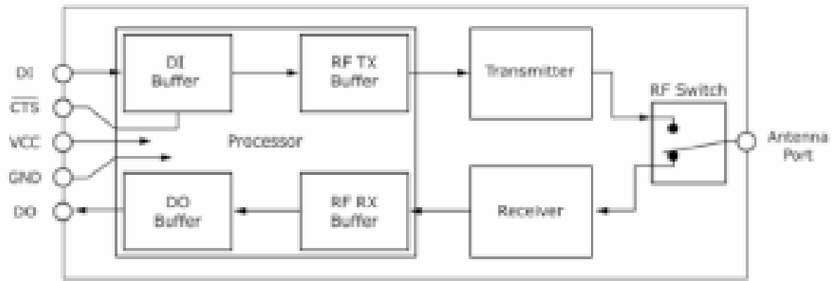
3.3.4 Figure 2: Flow chart on how data is sent in and how it goes out of the XBee
