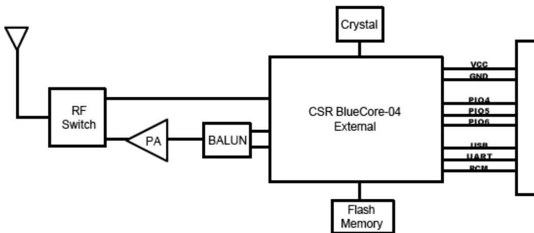
2.2.4.2 Figure 3: Flow chart for Bluetooth chip
