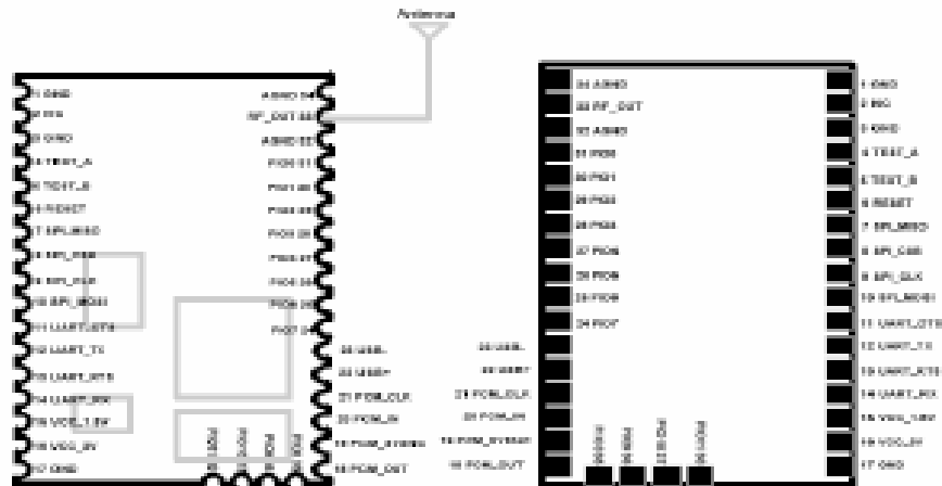
2.2.4.2 Figure 2: Pin Assignments for Bluetooth
