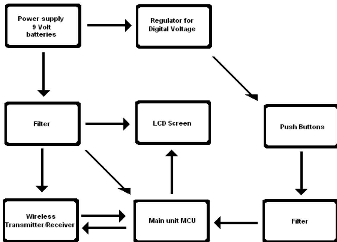
3.3.8 Figure 1: Main unit PCB block diagram
