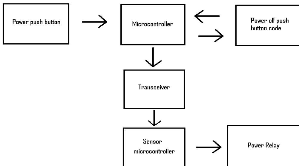
3.3.5 Figure 2: Power On/Off pushbutton block diagram.
