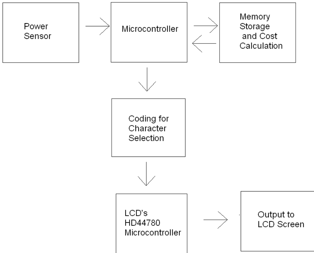
3.3.1 Figure 1: LCD block diagram
