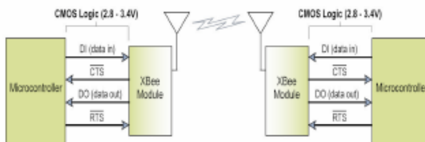
3.3.4 Figure 1: Flow chart on how data is sent between the microcontroller and the XBee module
