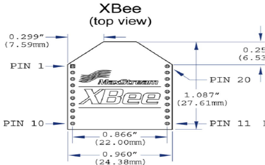
3.1.4.3 Figure 1: Drawing of XBee with dimensions and chart to show pin assignments and distribution.
