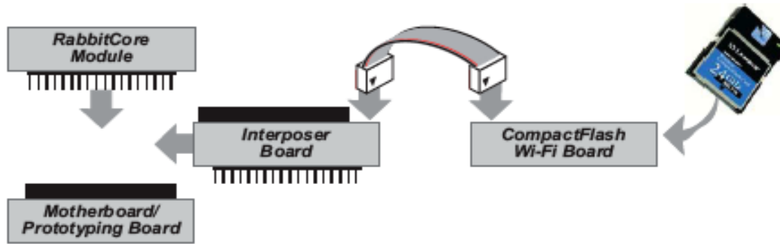
2.2.4.3 Figure 2: Basic illustration of add-on chip
