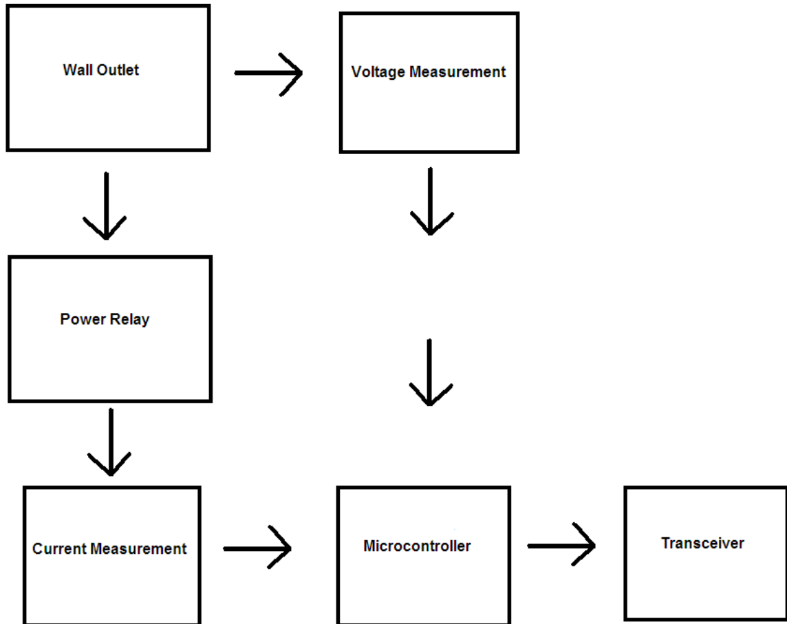
3.3.2 Figure 1: Power meter block diagram
