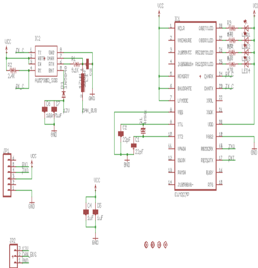
Figure 10.2.1 – ELM327 Schematic
