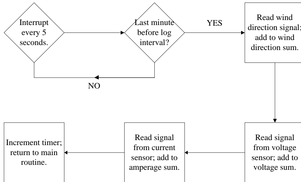
Figure 45: Data Measurement Subroutine
