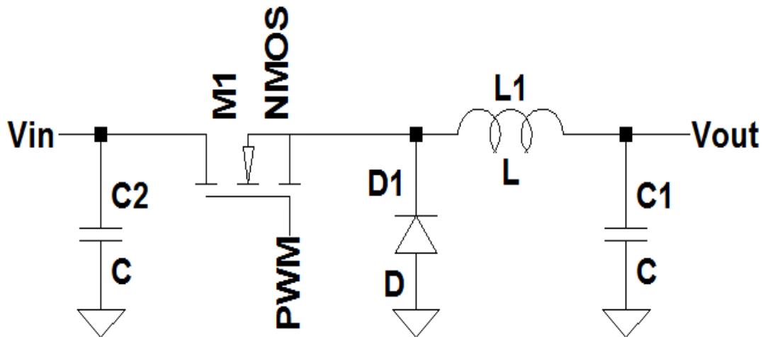
Figure 8: Buck Converter
