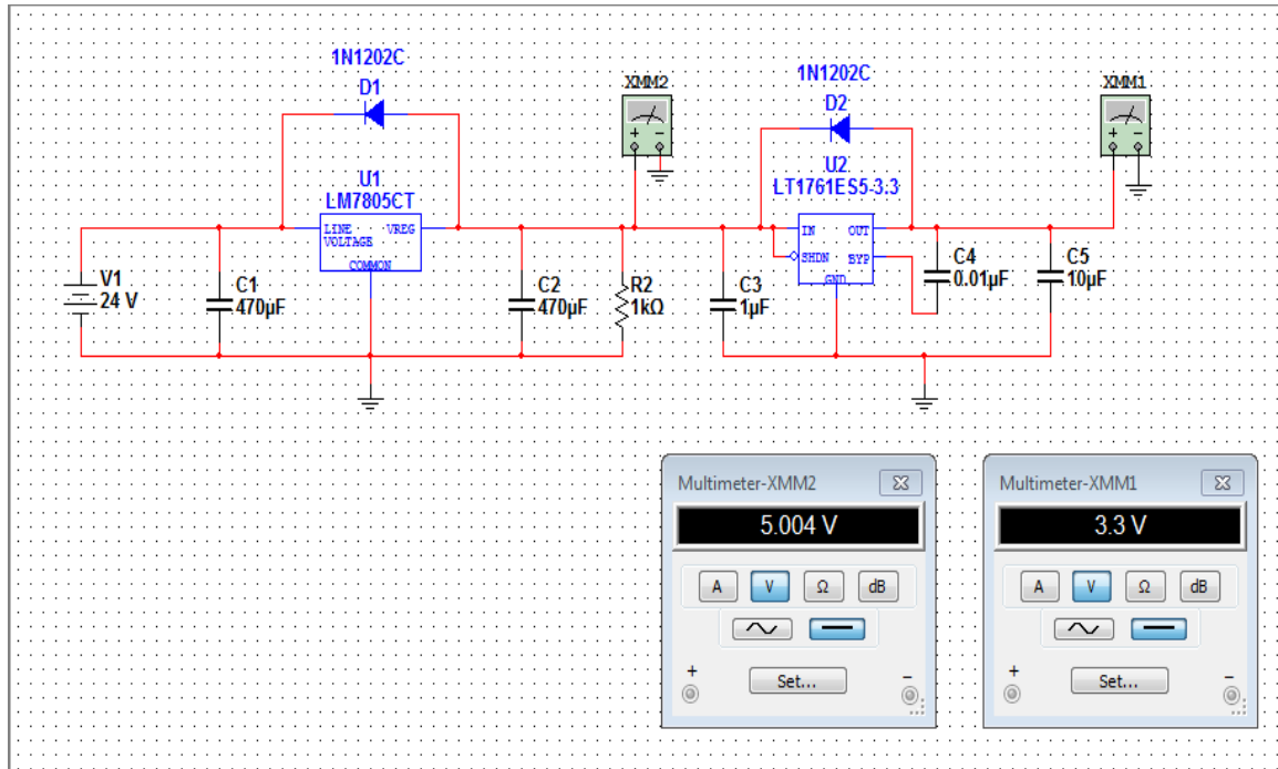
Figure 38: LCD Power Supply
