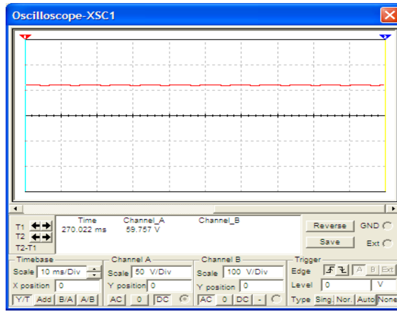
Figure 6: Output of Bridge Rectifier with smoothing circuit
