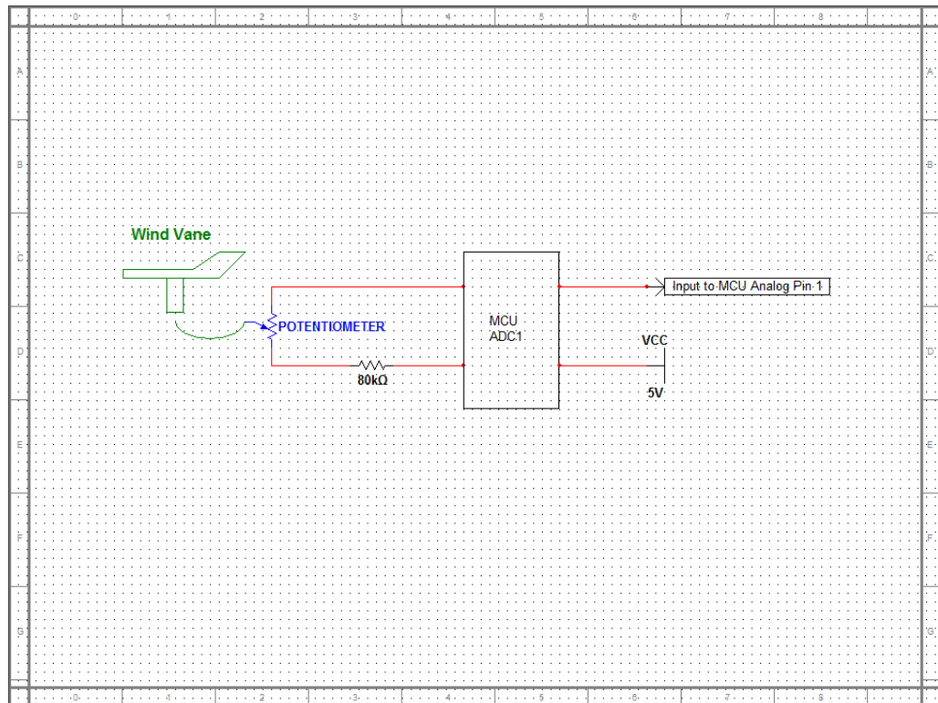
Figure 34: Wind Direction Interfacing Circuit
