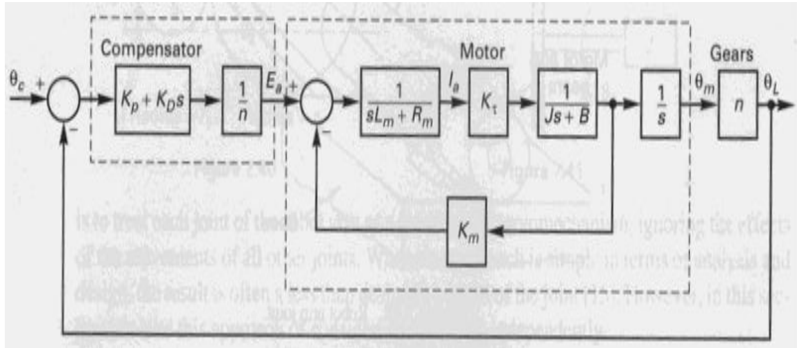
Figure 41: Control System with Gear
