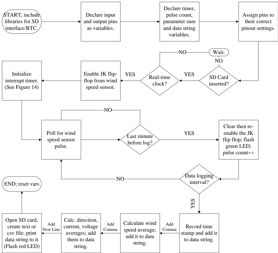
Figure 44: Sketch of Main Data Logging Routine
