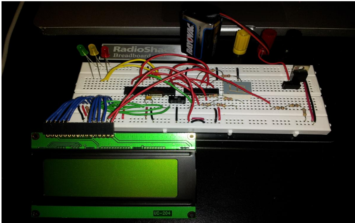
Figure 49: LCD Display Circuit Prototype
