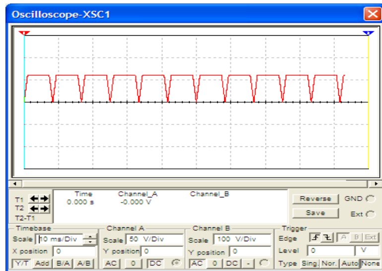
Figure 5: Output of Bridge Rectifier without smoothing circuit
