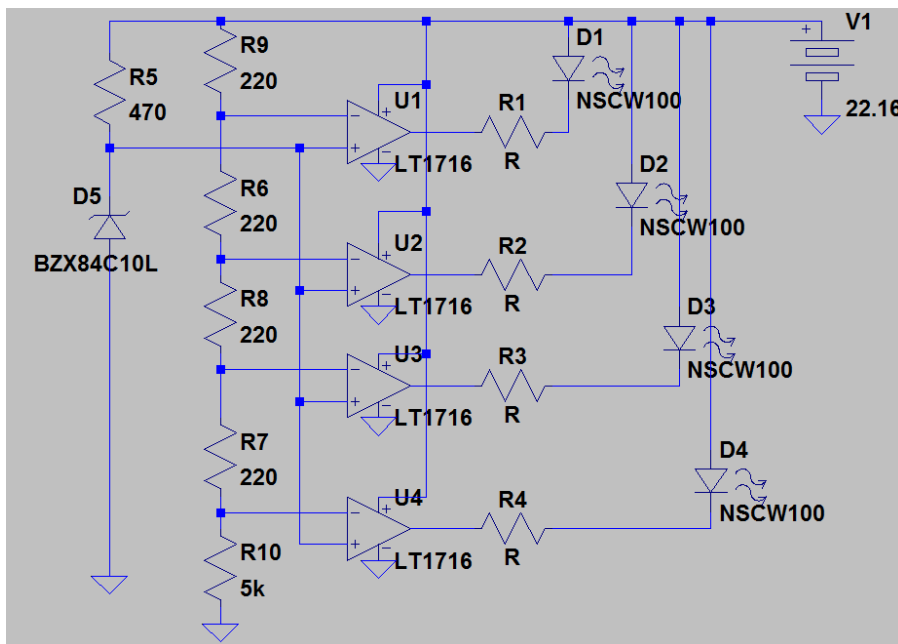
Figure 26: Battery Monitor for 24V System
