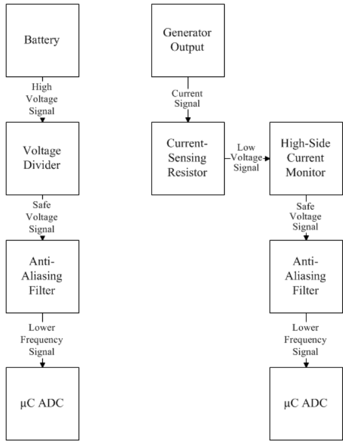
Figure 19: Current and Voltage Sensing Process
