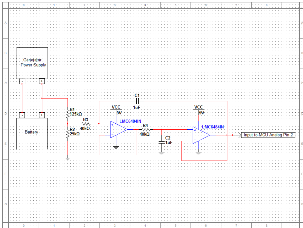
Figure 35: Voltage Sensing System
