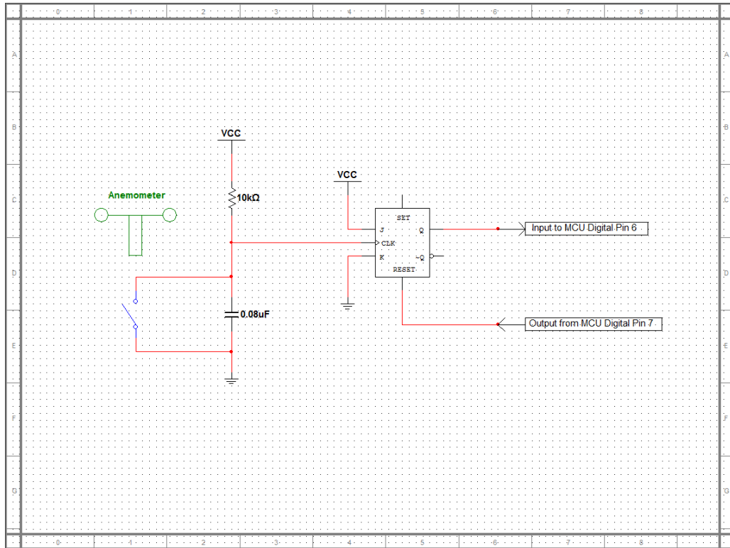
Figure 33: Wind Speed Interfacing Circuit
