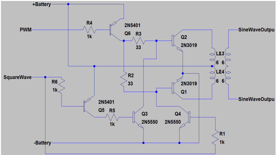
Figure 31: Inverter Circuit Stage 2: Sine Wave Generator
