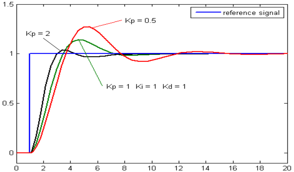
Figure 21: Compensator response for different values of K_p (Permission Pending)
