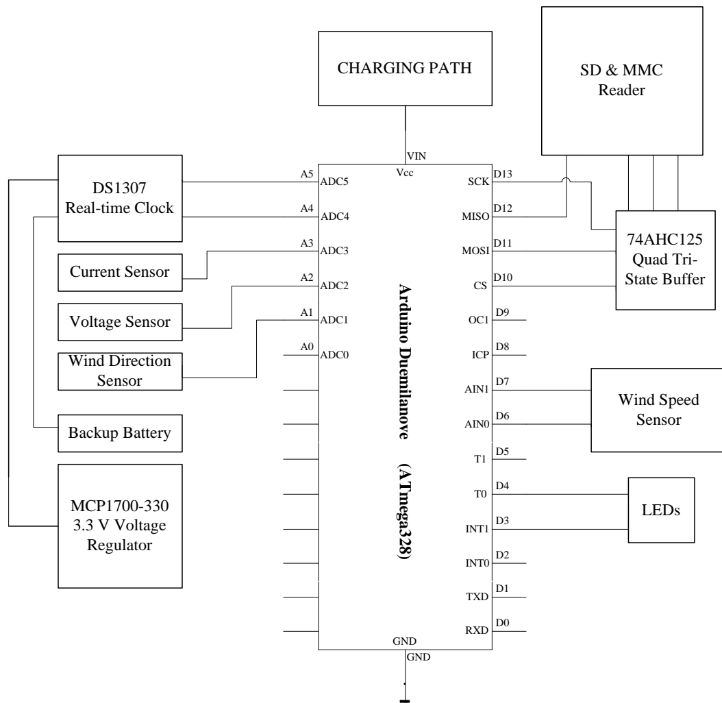
Figure 43: Connections between Host Board and Data Logger
