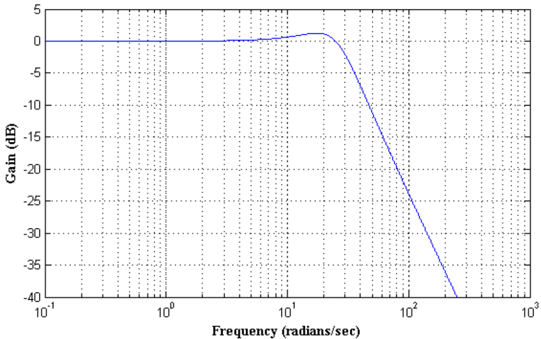
Figure 37: Bode Plot of Second-Order Low-Pass Filter
