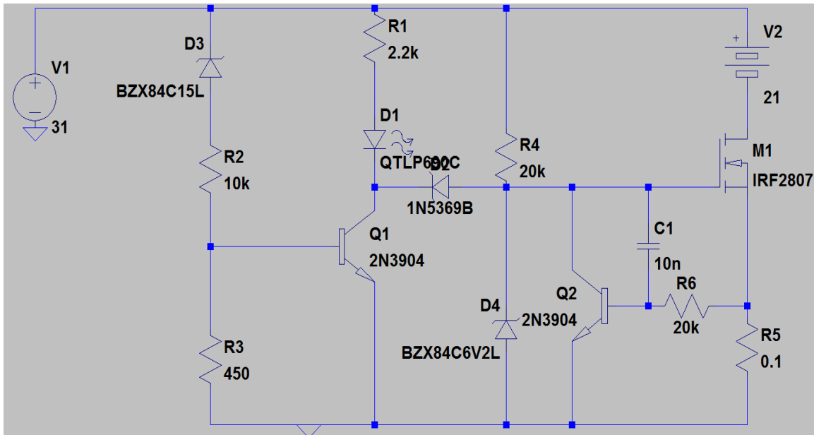
Figure 28: Charge Controller Circuit
