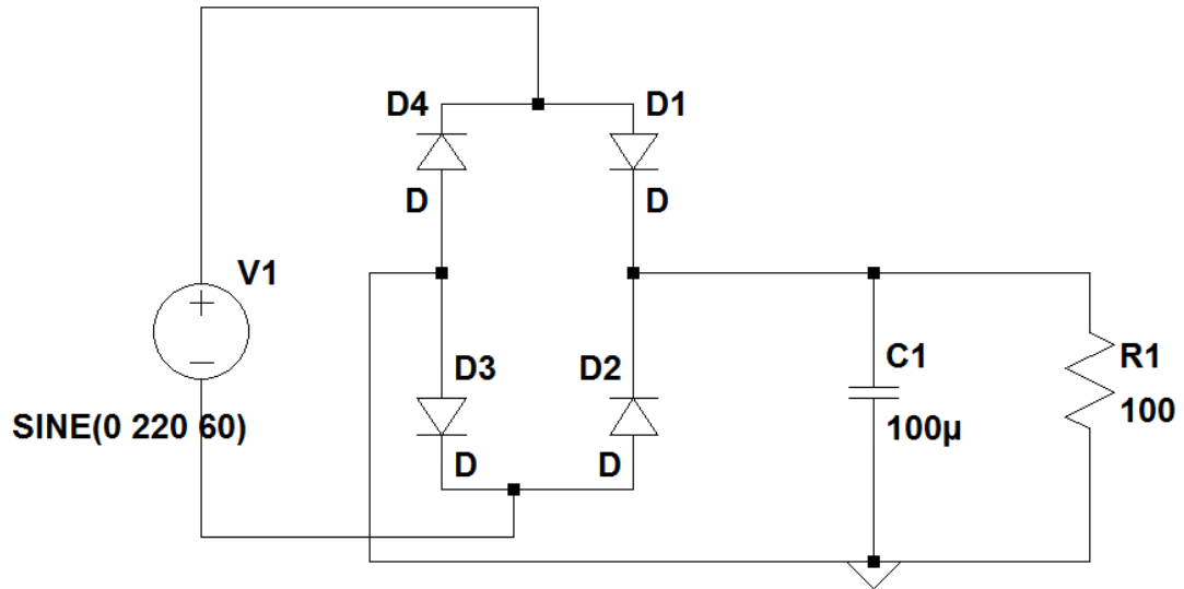
Figure 4: Bridge Rectifier with smoothing circuit
