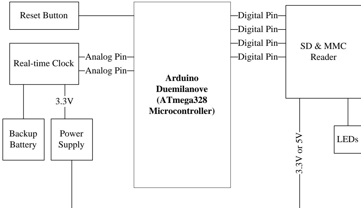
Figure 17: Interface between Arduino & Data Logging Shield
