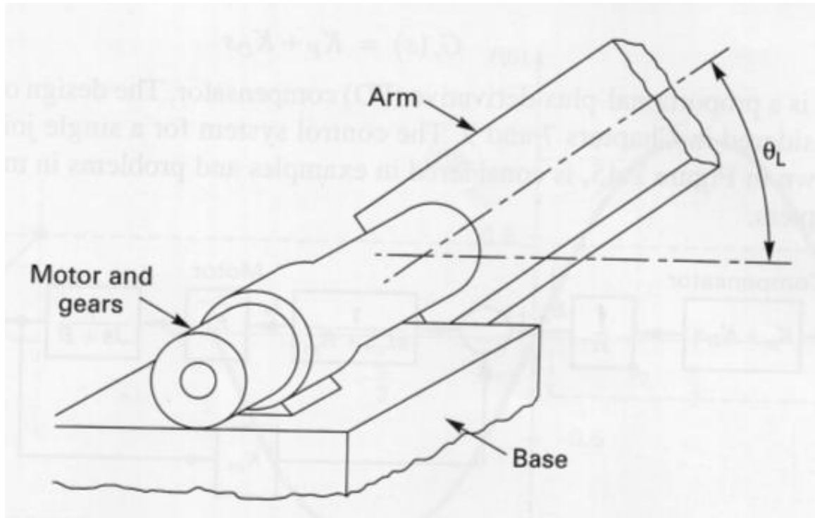
Figure 42: Motor and Gear Connection
