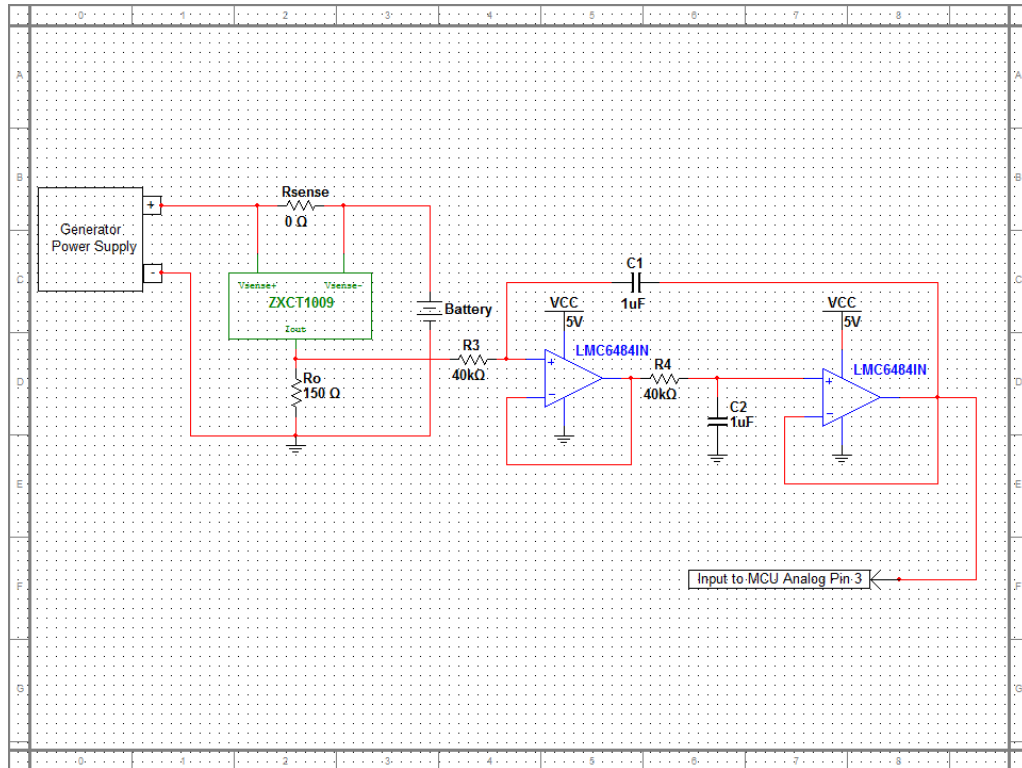
Figure 36: Current Sensing System
