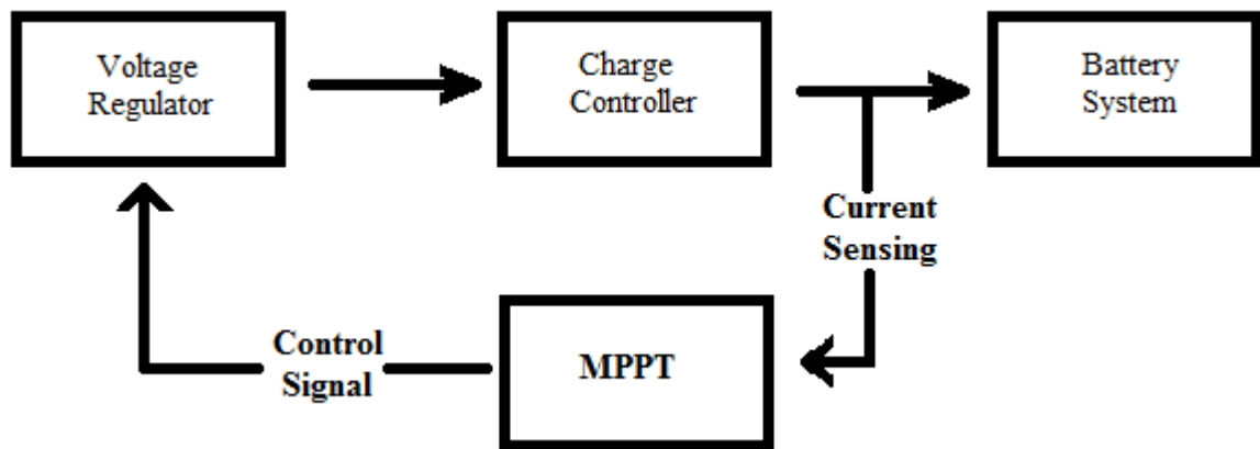
Figure 29: Maximum Power Point Tracking Block Diagram
