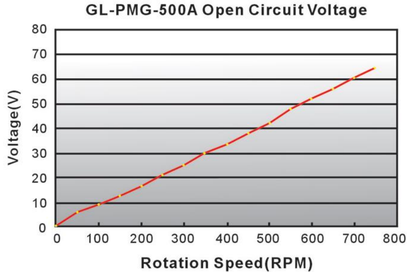
Figure 46: Voltage Output vs. RPM
