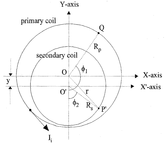
Fig. 4. Front view of the two filamentary coils.
