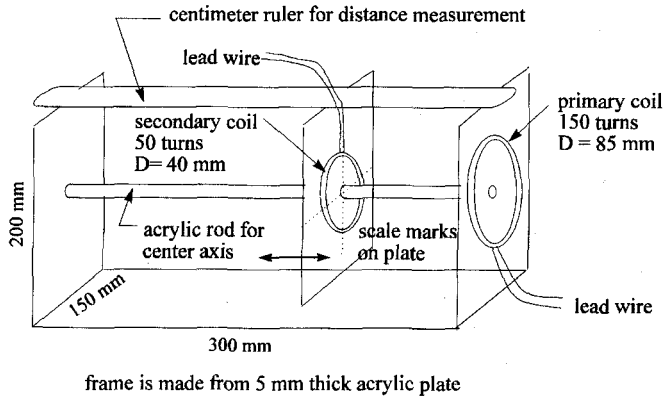
Fig. 8. Experimental setup.
