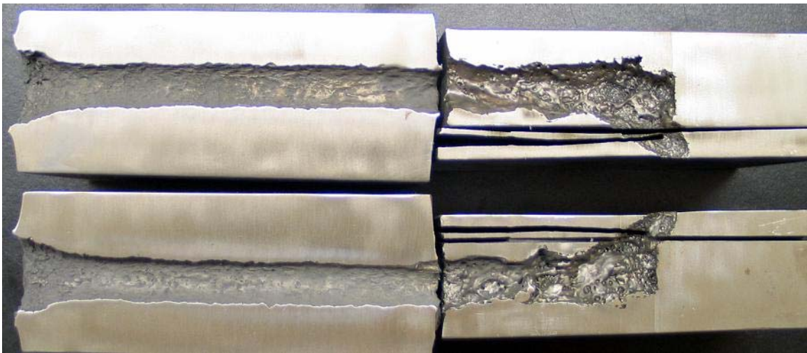
Figure 11. Shot 797 crater cross section.
