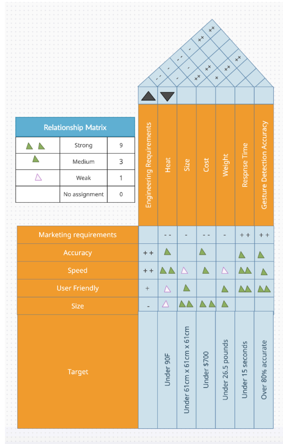
Figure 2.4.2: House of Quality.
