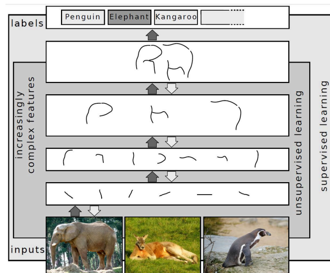
Figure 3.5.5: This figure shows the process of Deep Learning when it is processing images.
