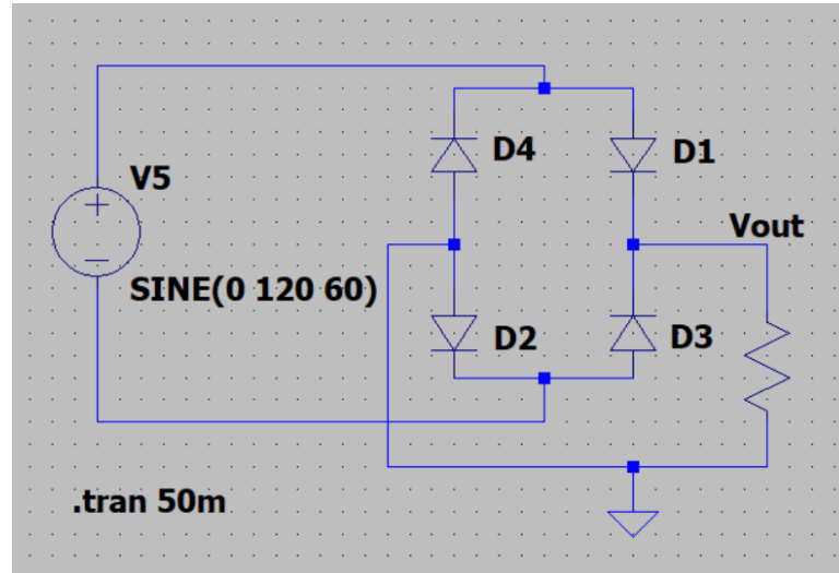
Figure 3.3.1.1: Full Wave Bridge Rectifier in LTspice.
