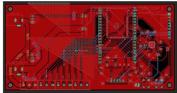
Fig 1. Main PCB.
