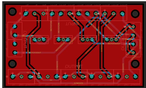
Fig. 2. Secondary PCB.
