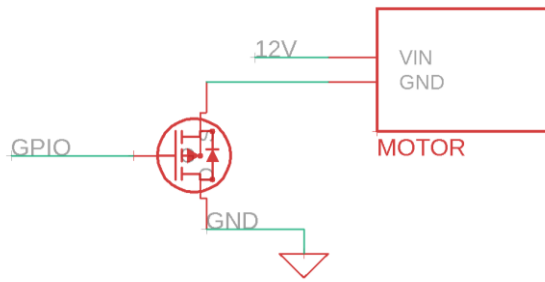
Fig 7. MOSFET and Motor Configuration.
