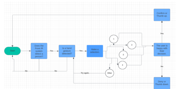
Fig. 12. Object Detection Flowchart.
