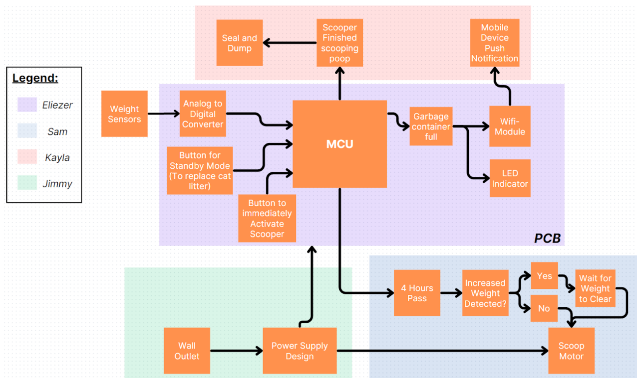
Figure 2A: Hardware Block Diagram
