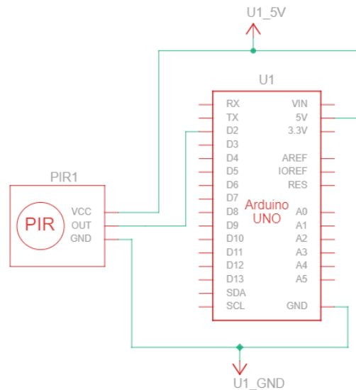
Figure 6E PIR Testing Schematic
