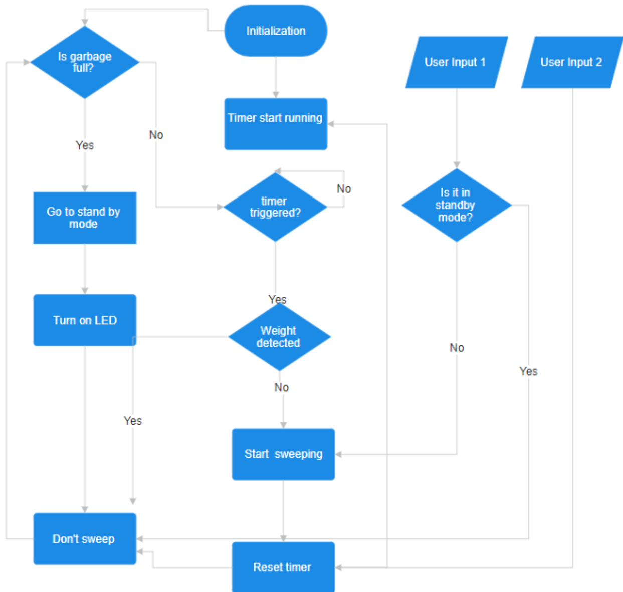
Figure 3A: Software Flowchart
