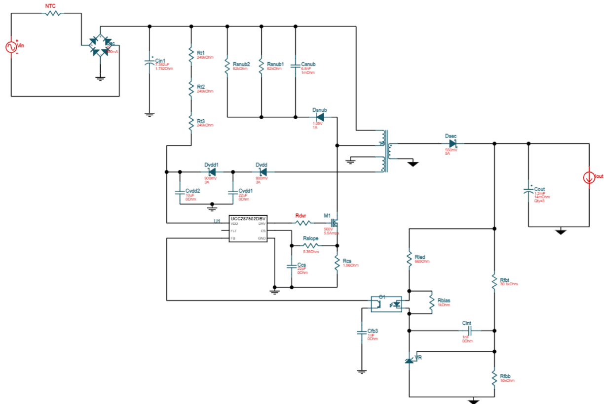
Figure 6B AC-DC Converter Schematic
