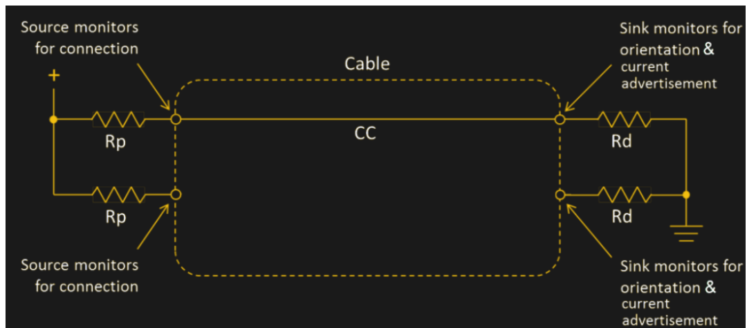
Figure 8B: Example of CC Pins [32]
