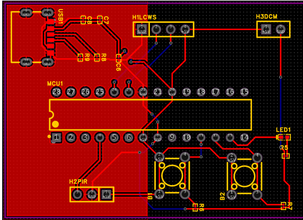
Figure 8C: Physical PCB Layout Design
