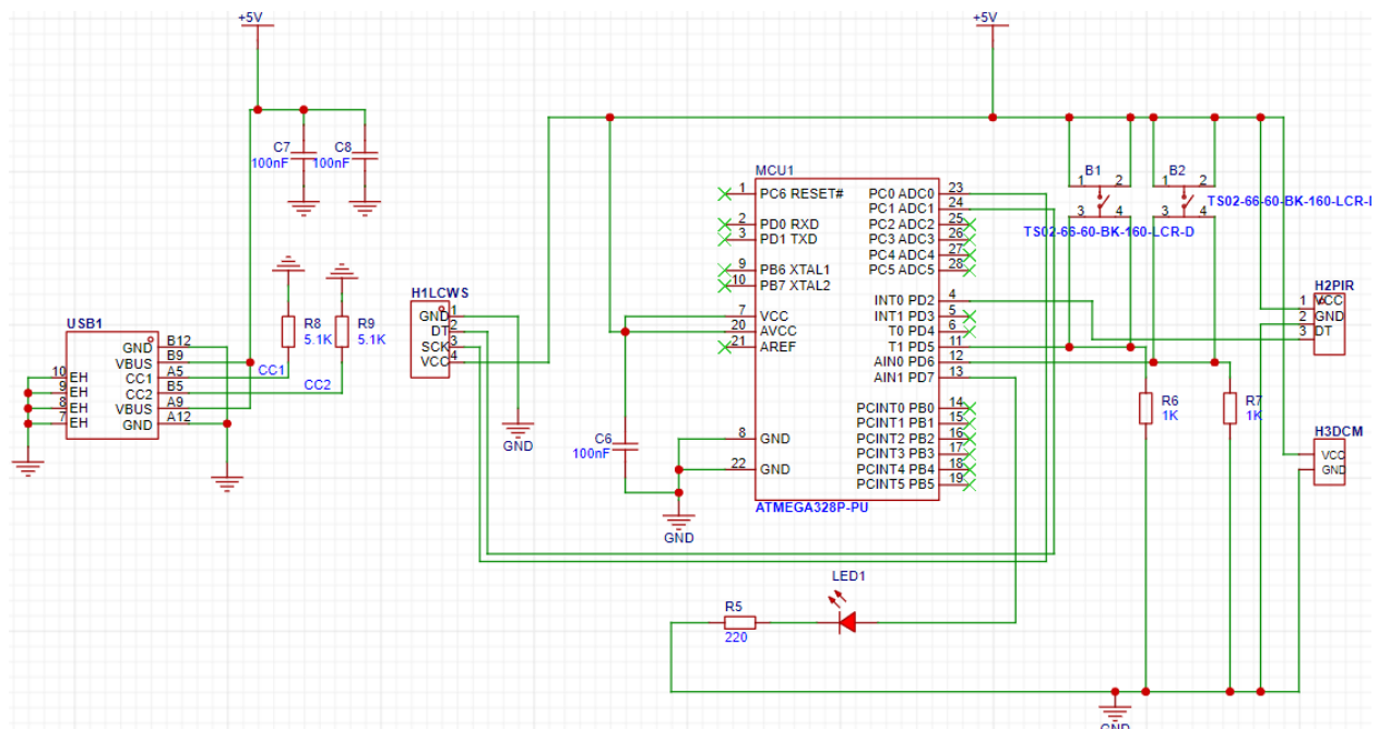
Figure 8A: PCB Schematic
