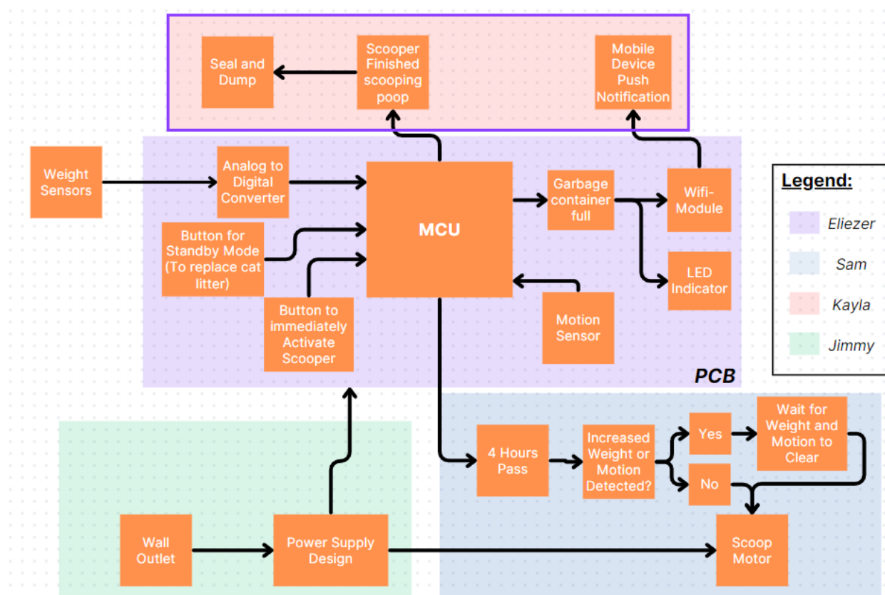
Figure 2D: Hardware Block Diagram
