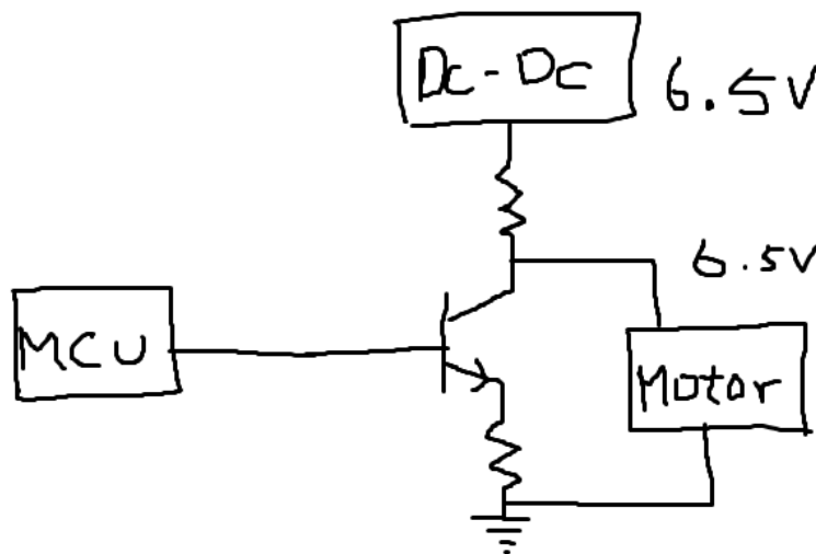
Figure 6J: Motor Controller
