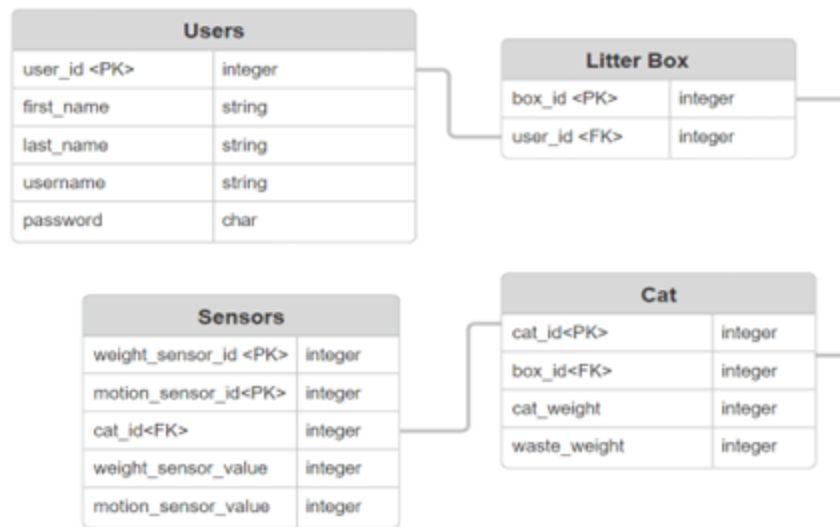
Figure 7C: Entity Relationship Diagram
