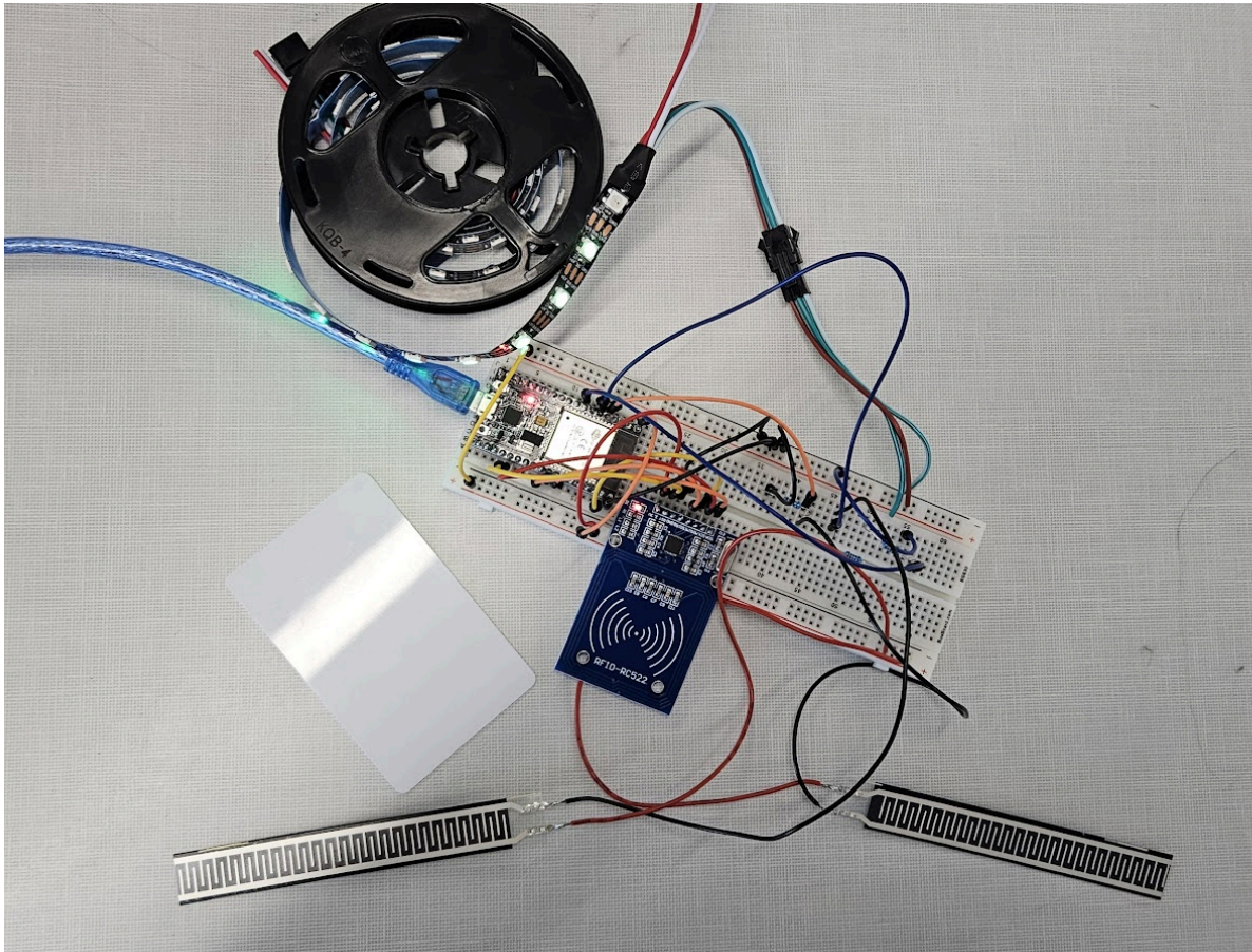
Image 9.4: Tool Detection Component Testing
