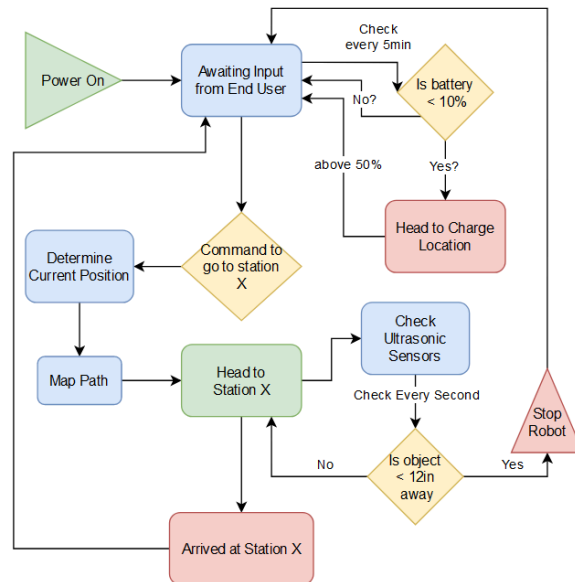
Image 7.7: State Diagram for Basic Movement
