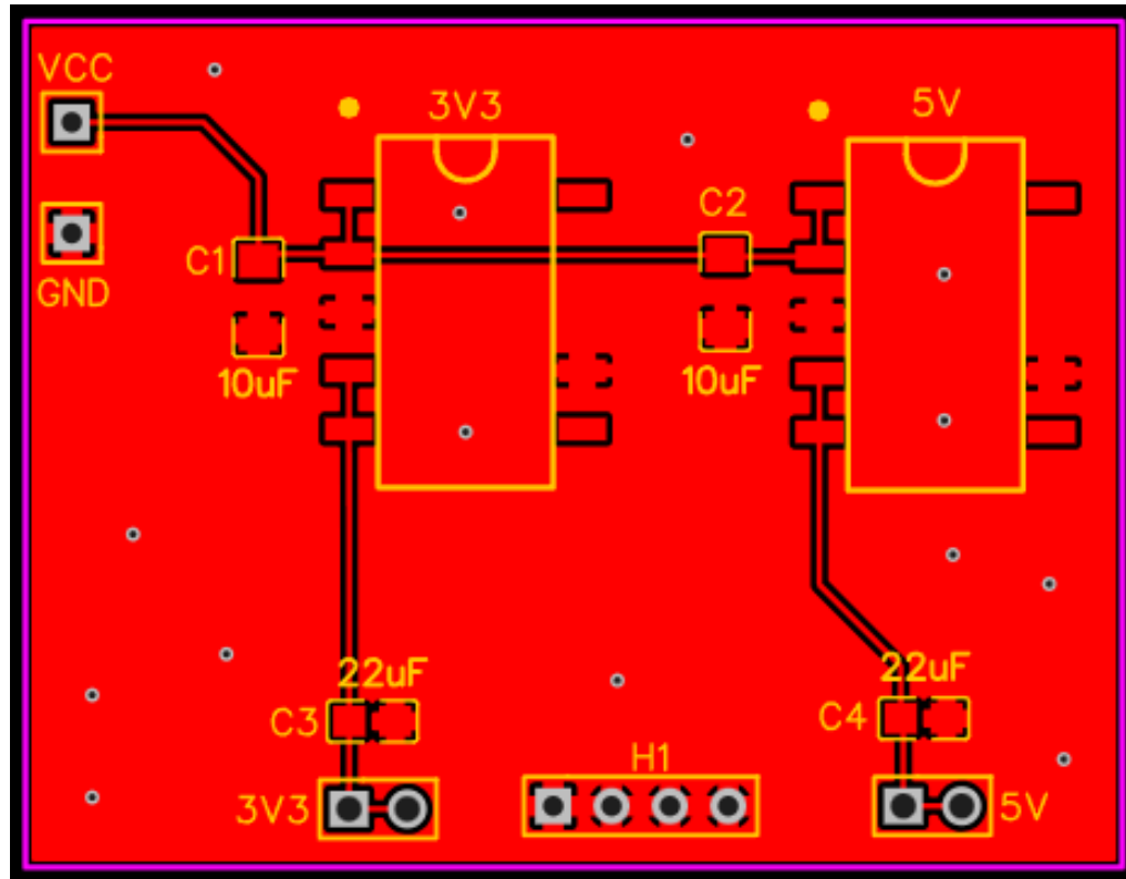
Image 8.2: Power delivery Unit PCB
