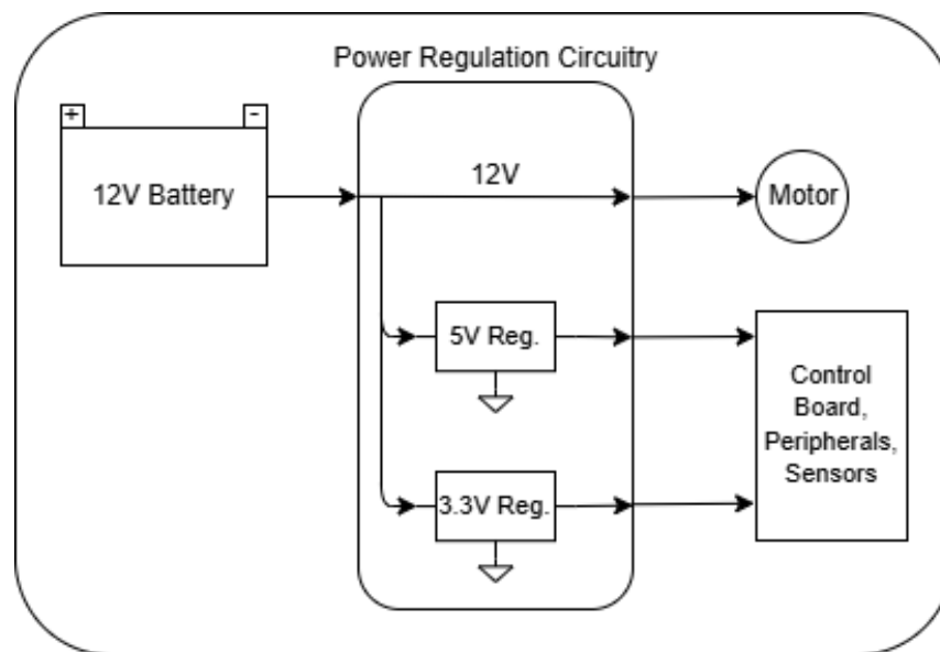
Image 6.4: Power Distribution Board Block Diagram
