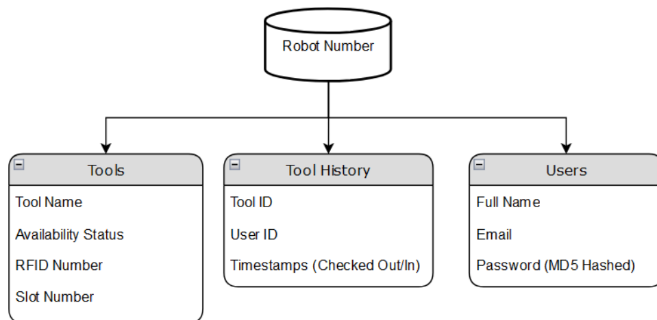
Image 7.1: MongoDB data structure diagram
