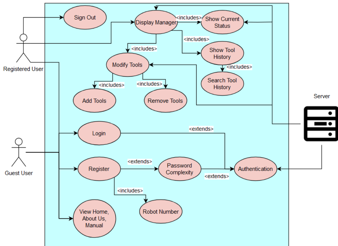
Image 7.3: Website Use Case Diagram
