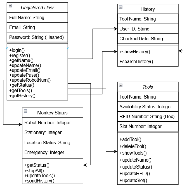
Image 7.5: Class Diagram of Mobile Application
