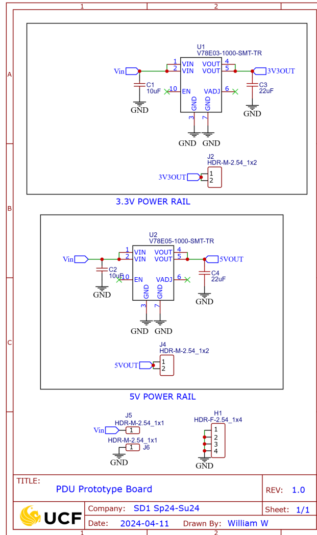
Image 6.5: Power Distribution Unit Board Schematic
