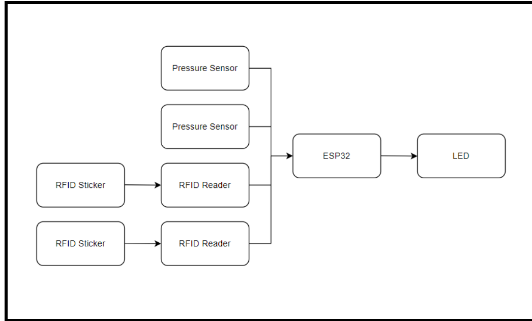
Image 6.1: Tool Detection Block Diagram
