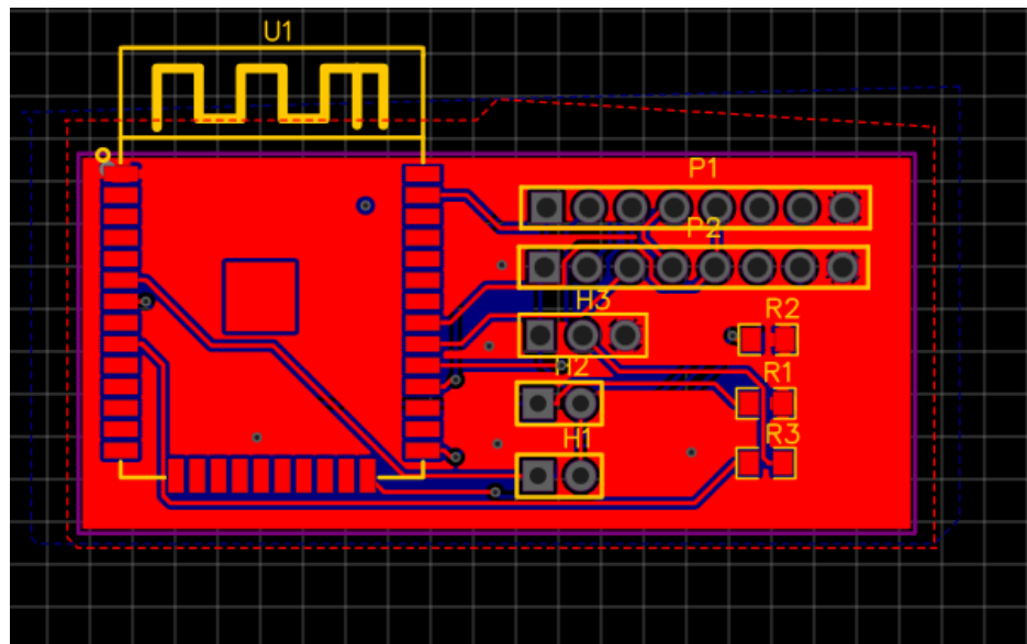
Image 8.1: Tool detection and Lighting Control PCB
