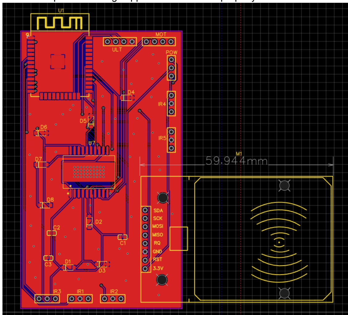
Image 8.3: Main Control Board Prototype PCB
