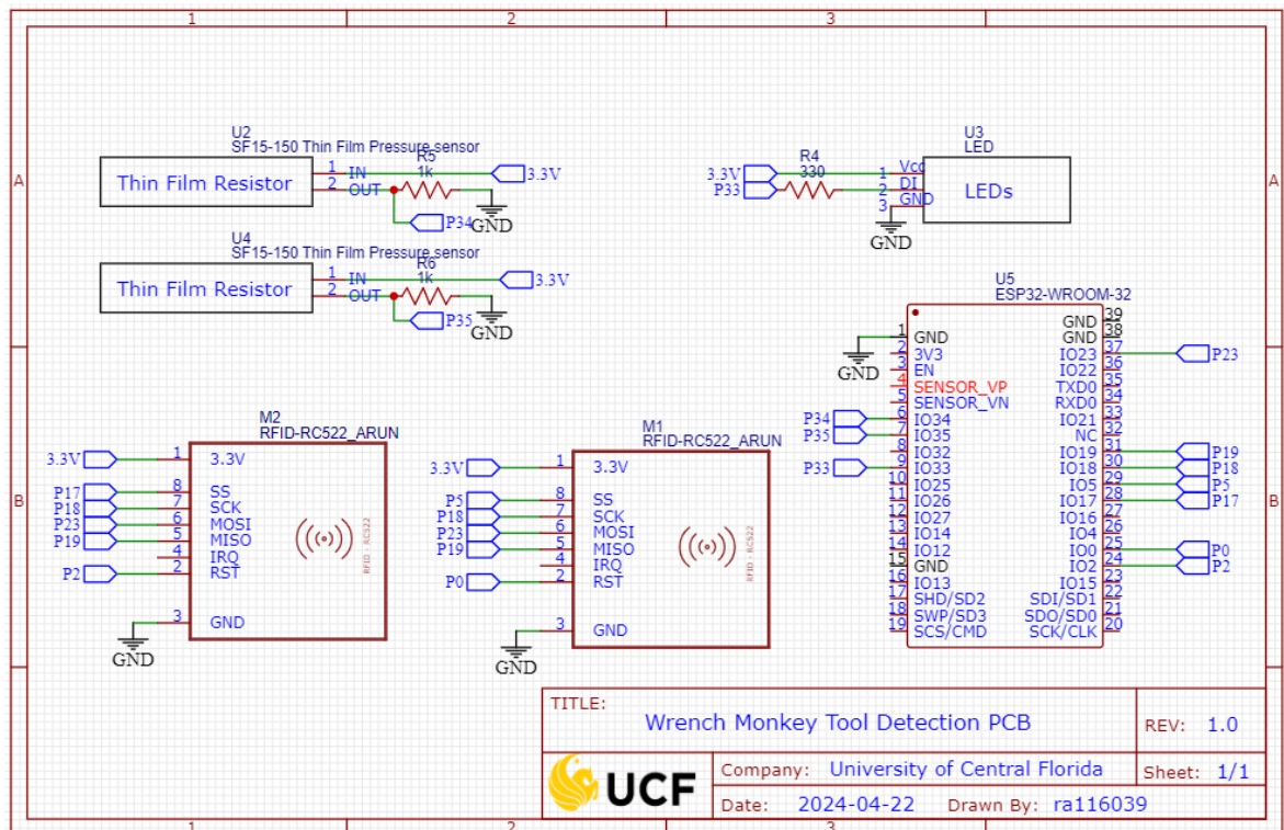
Image 6.2: Tool Detection Schematic
