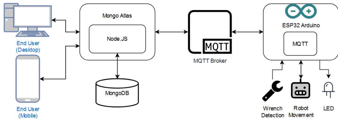
Image 7.6: Data Transfer Diagram (Atlas to ESP32)
