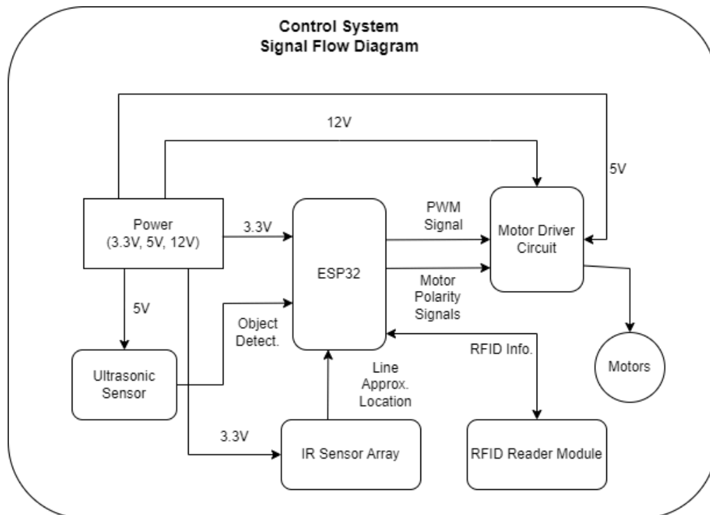
Image 6.6: Control System Signal Flow Diagram
