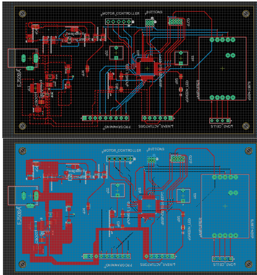
Figure 34– PCB Design
