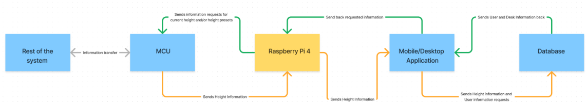
Figure 20 - Data Transfers and Requests Flow Chart
