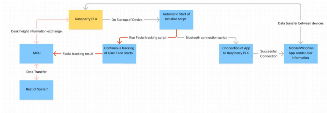
Figure 21 - Software Flowchart of Raspberry Pi 4
