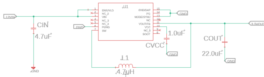
Figure 12 – 12V to 3.3V Voltage Regulator Schematic
