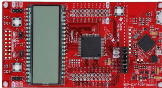
Figure 14 - MSP430FR6989 LaunchPad Development Kit [52]
