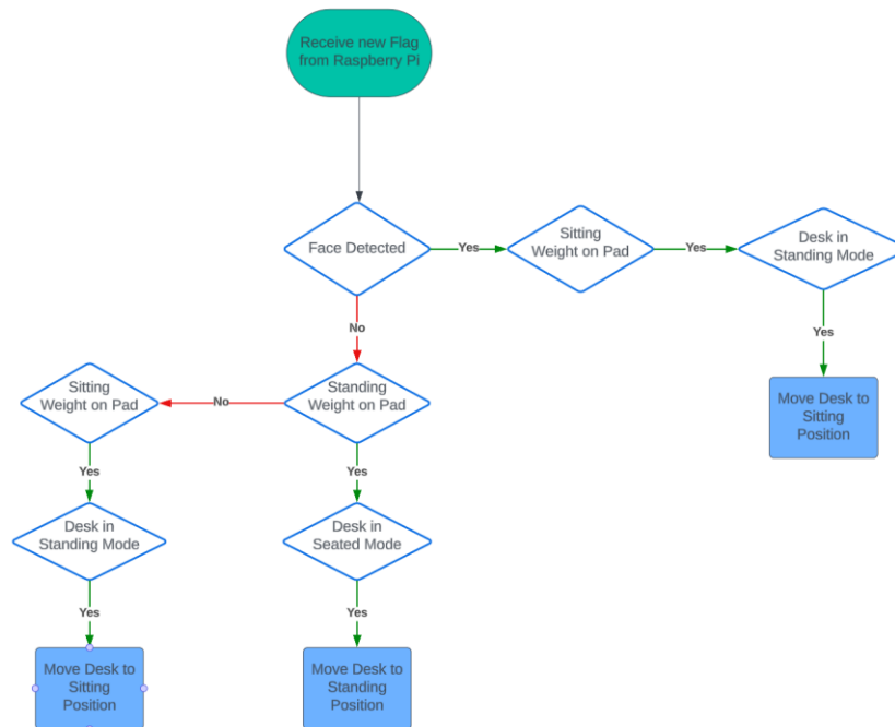
Figure 16 - Flowchart of Desk Position Change Logic
