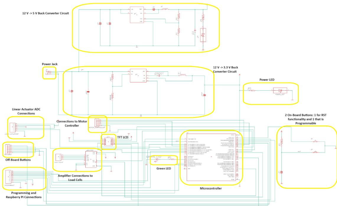
Figure 10– Revised Peripheral Schematic
