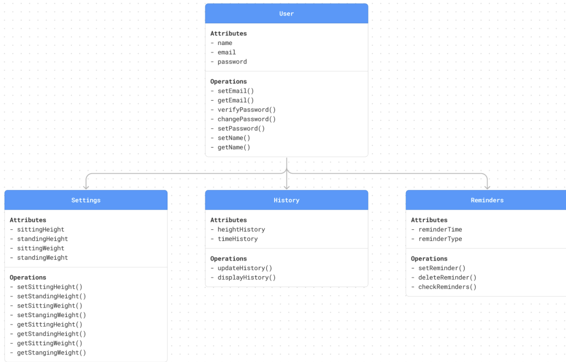
Figure 31 – UML Diagram of Database Structure of the Application
