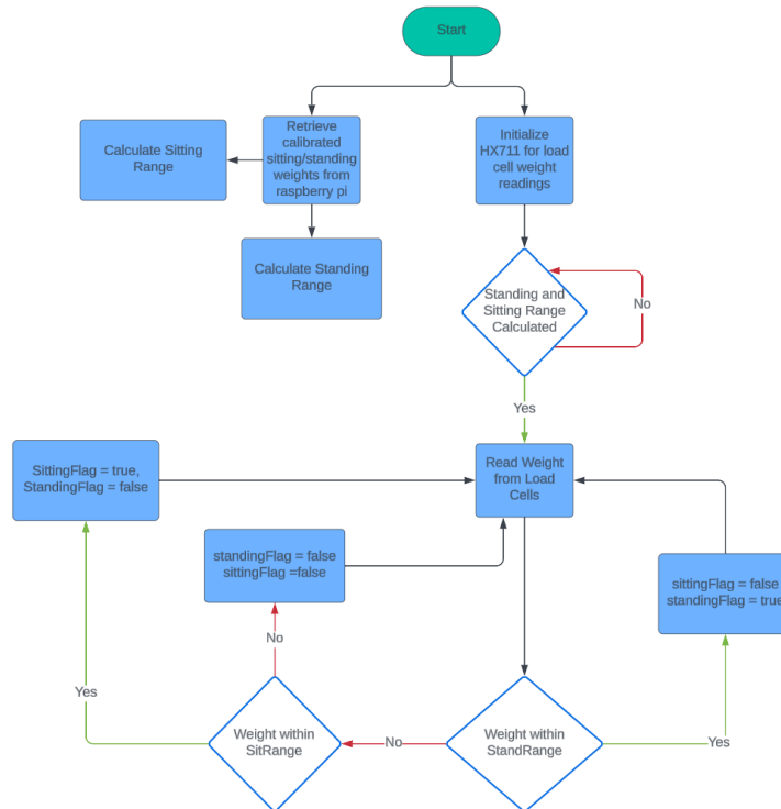
Figure 15 - Load Cell Logic Overview
