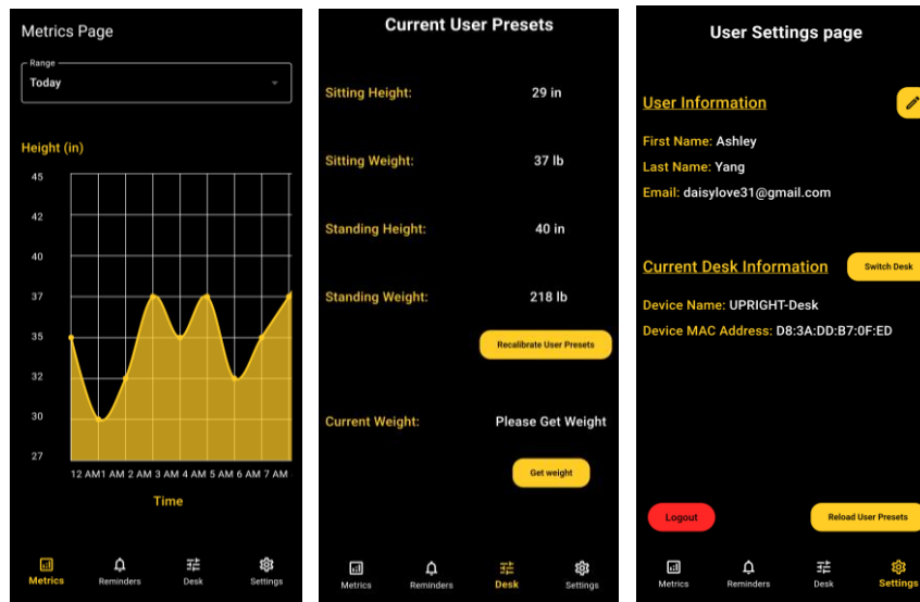
Figure 25 – Metrics, Desk and Settings Mobile Interface
