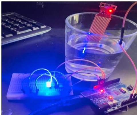
Figure 9.3 Water level sensor
