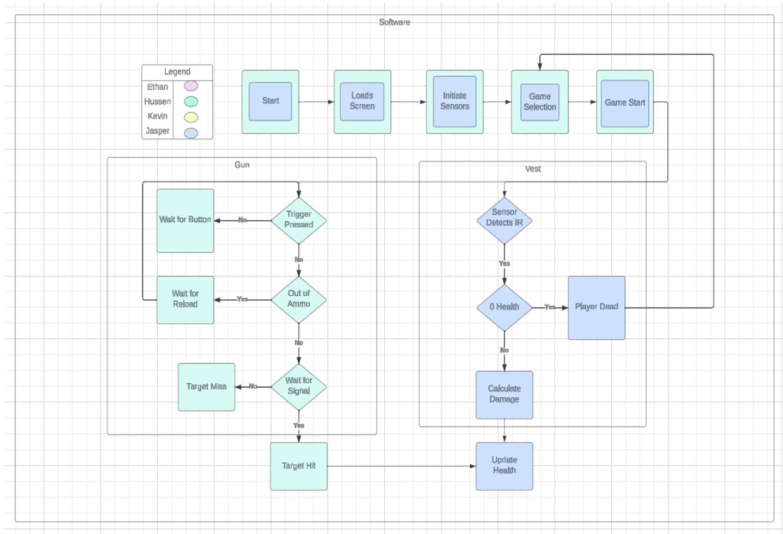
Figure 3. Software Flowchart
