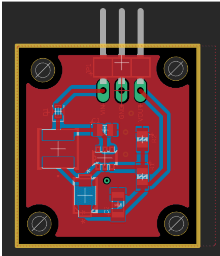
12V converter PCB.
