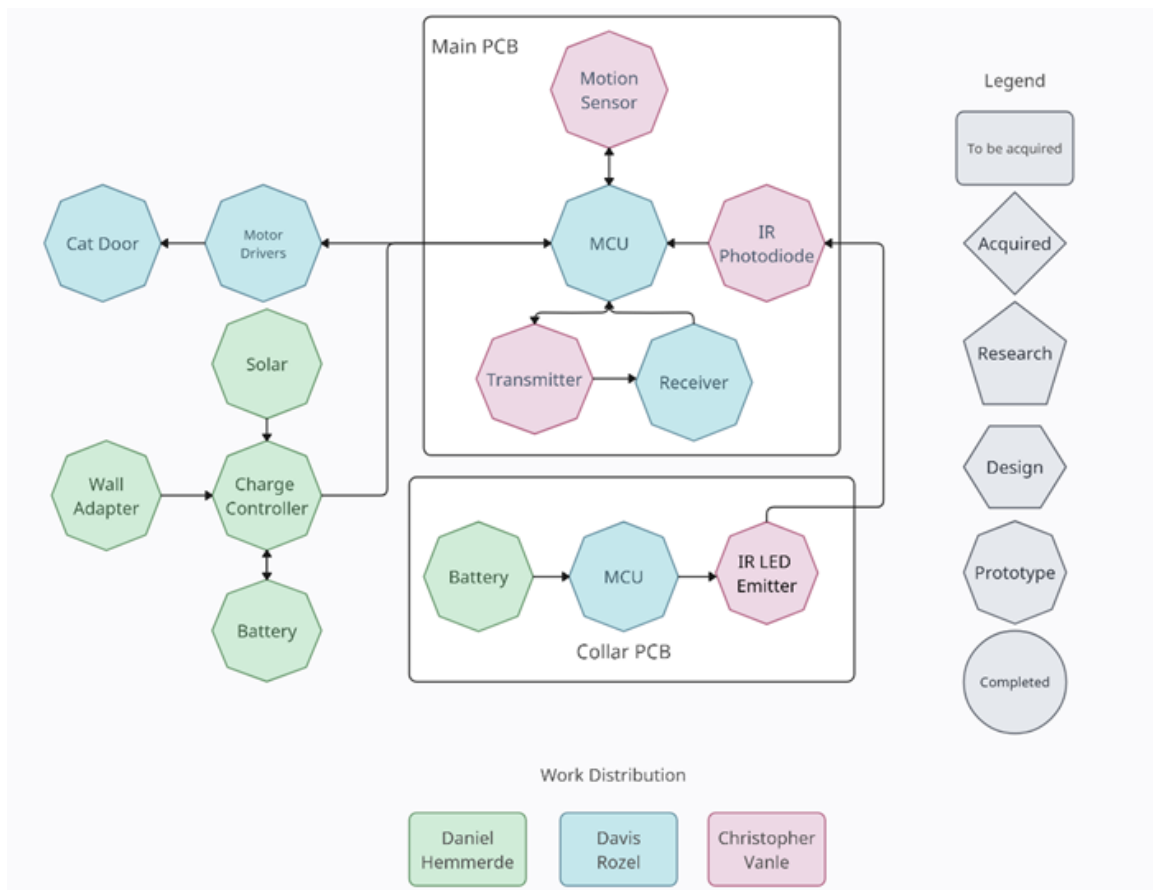
Hardware block diagram with work distributions and progress.
