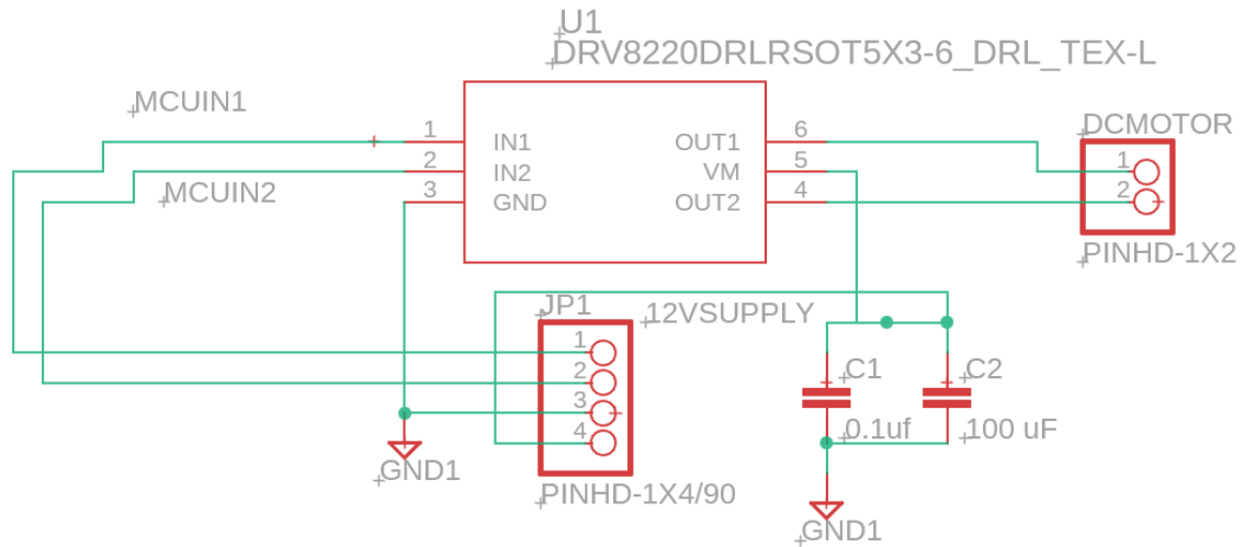
12V motor controller schematic.
