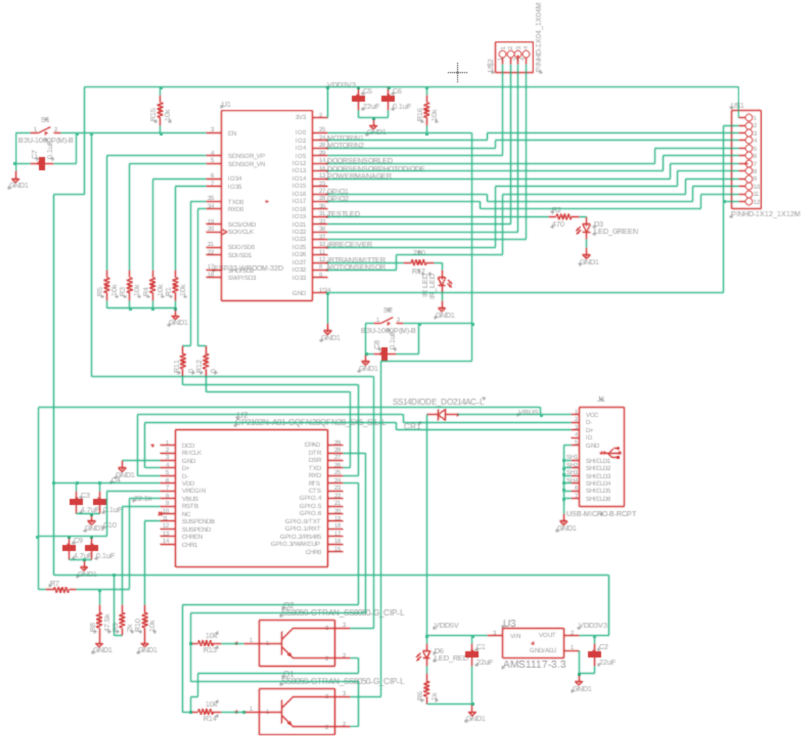
Main board schematic.
