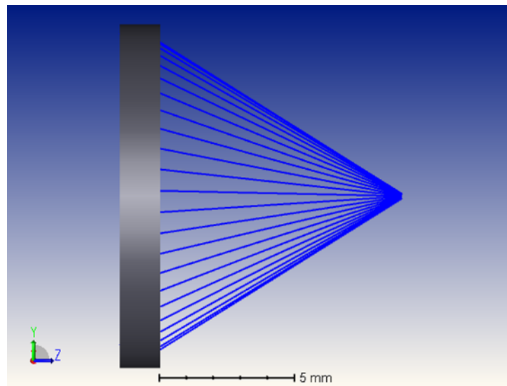
Zemax simulation of FRP0510 Fresnel lens from Thorlabs (ray from left to right).
