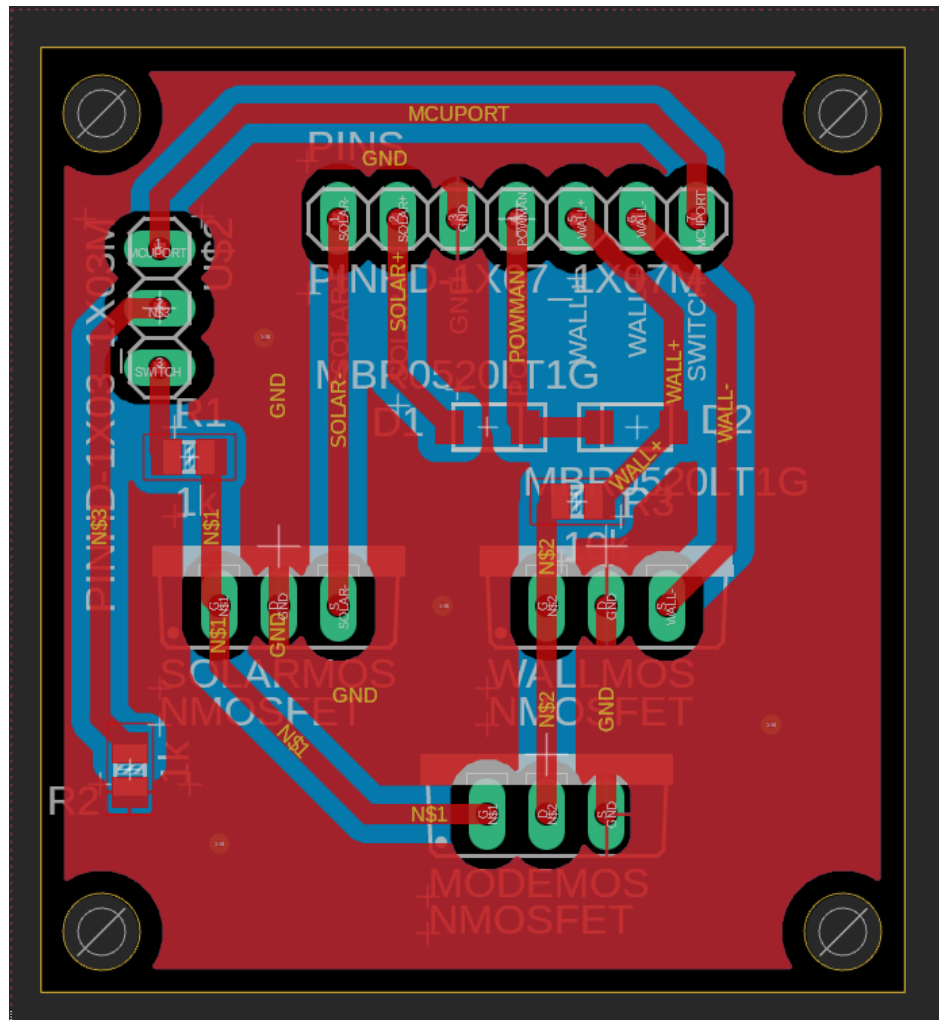
Battery subsystem PCB.
