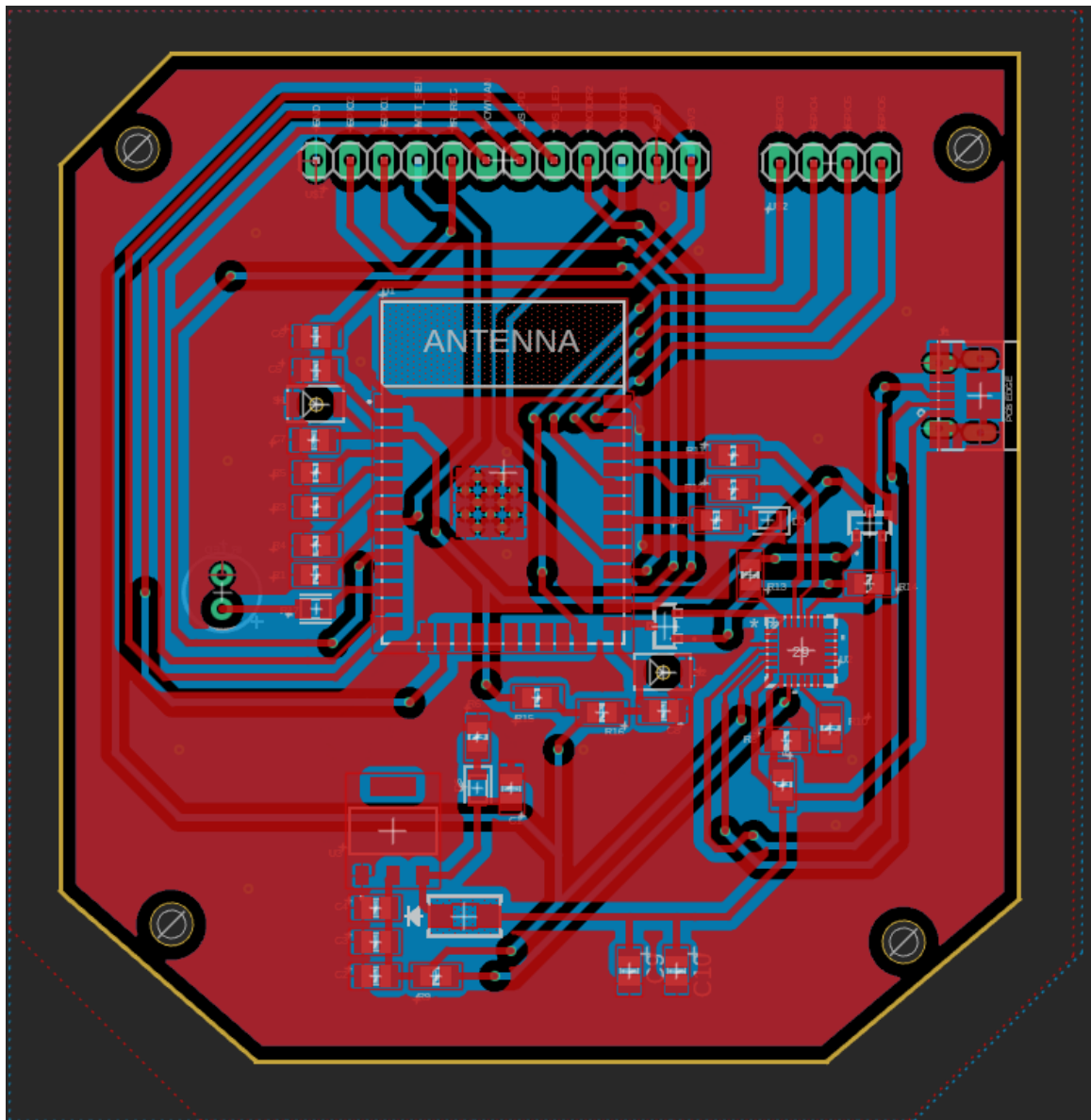
Main board PCB.
