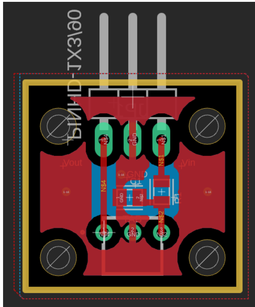
IR receiver PCB.
