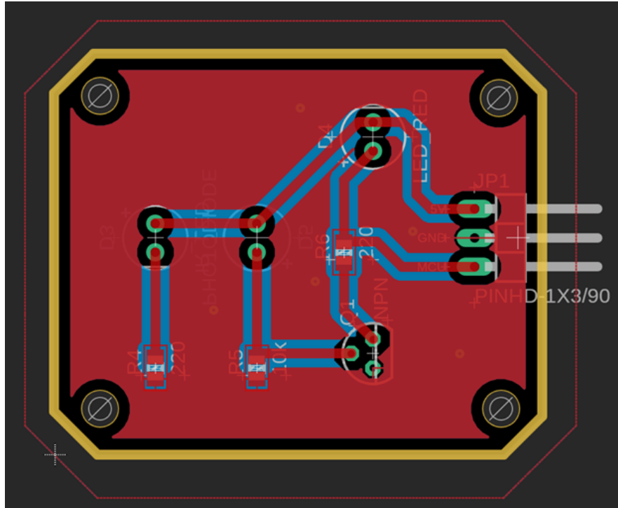
Motion sensor PCB.
