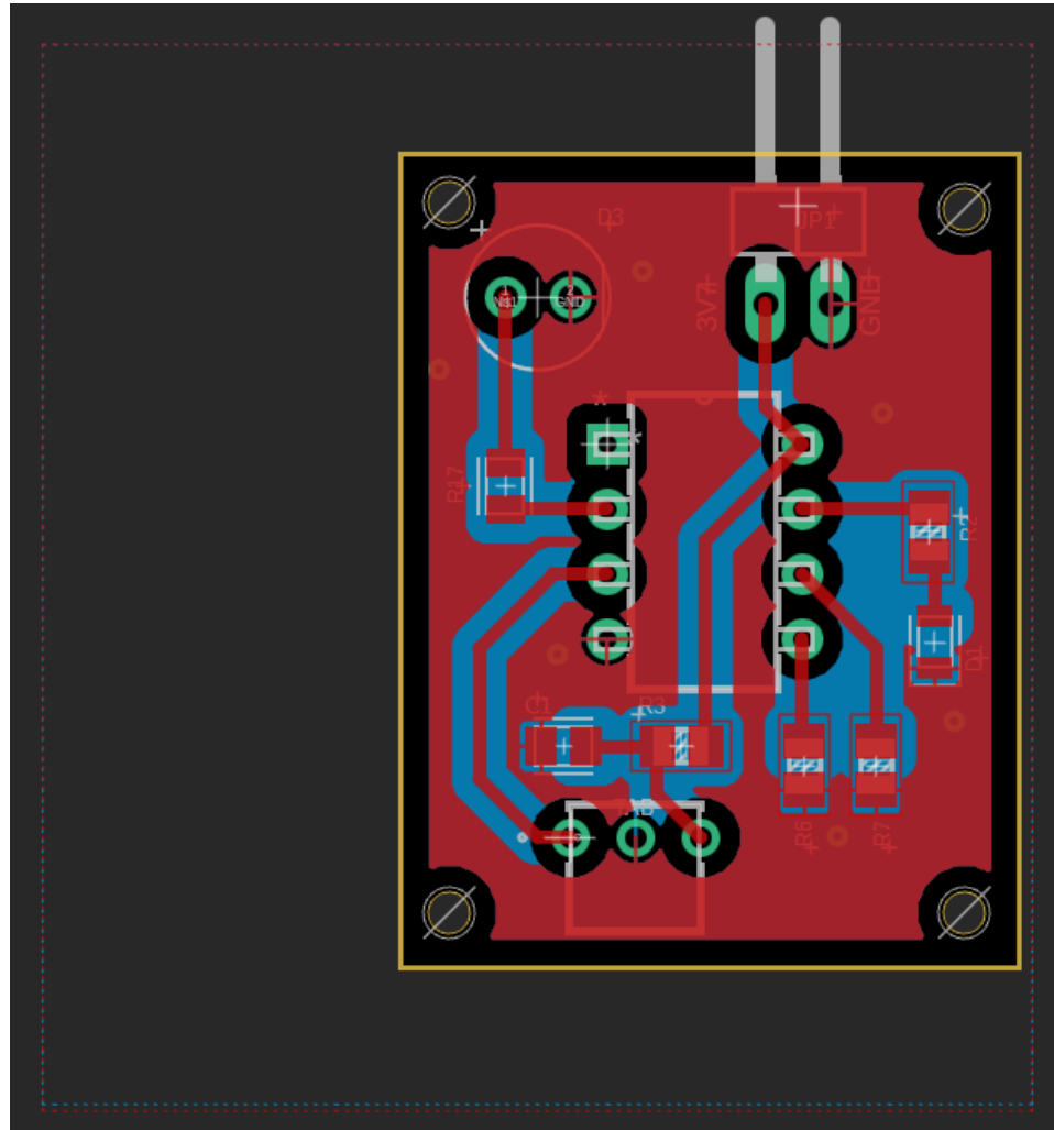
Collar PCB.
