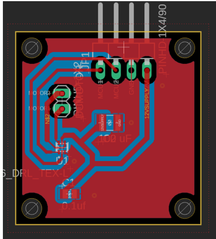
12V motor controller PCB.
