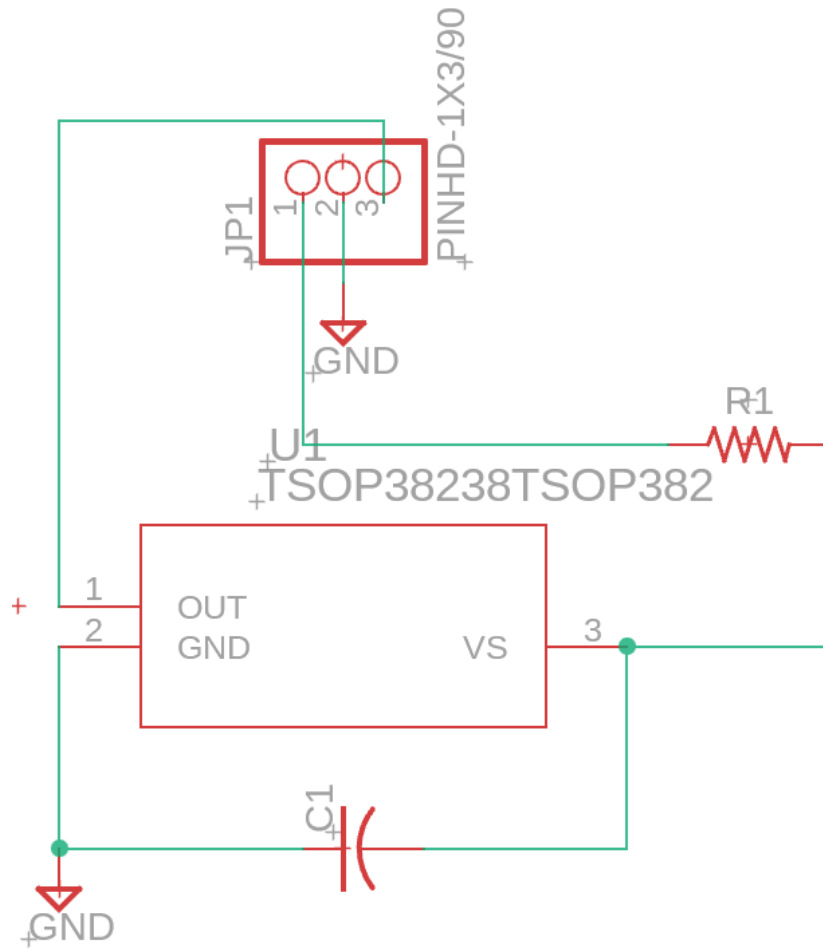
IR Receiver circuit
