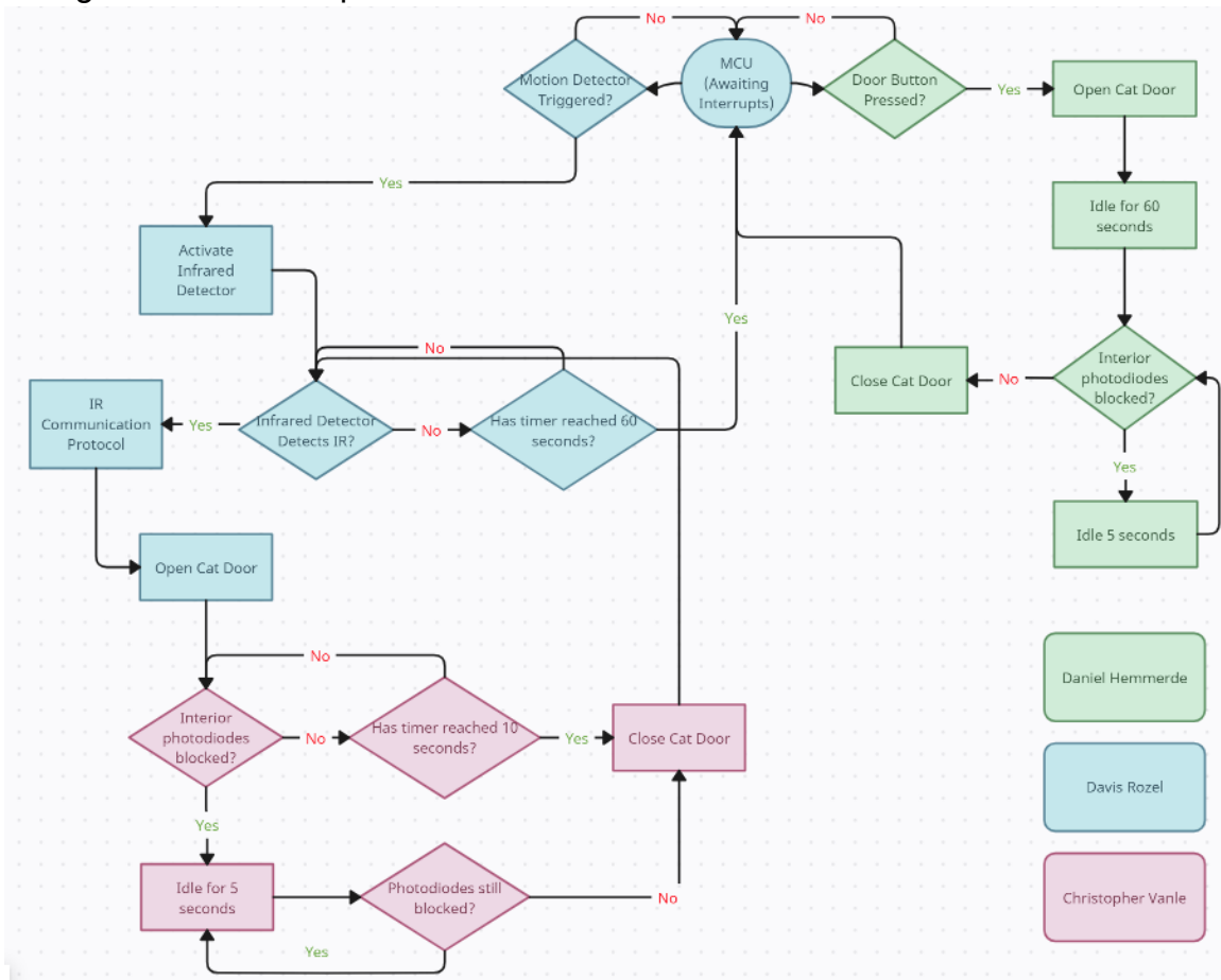
Software block diagram with work distributions.
