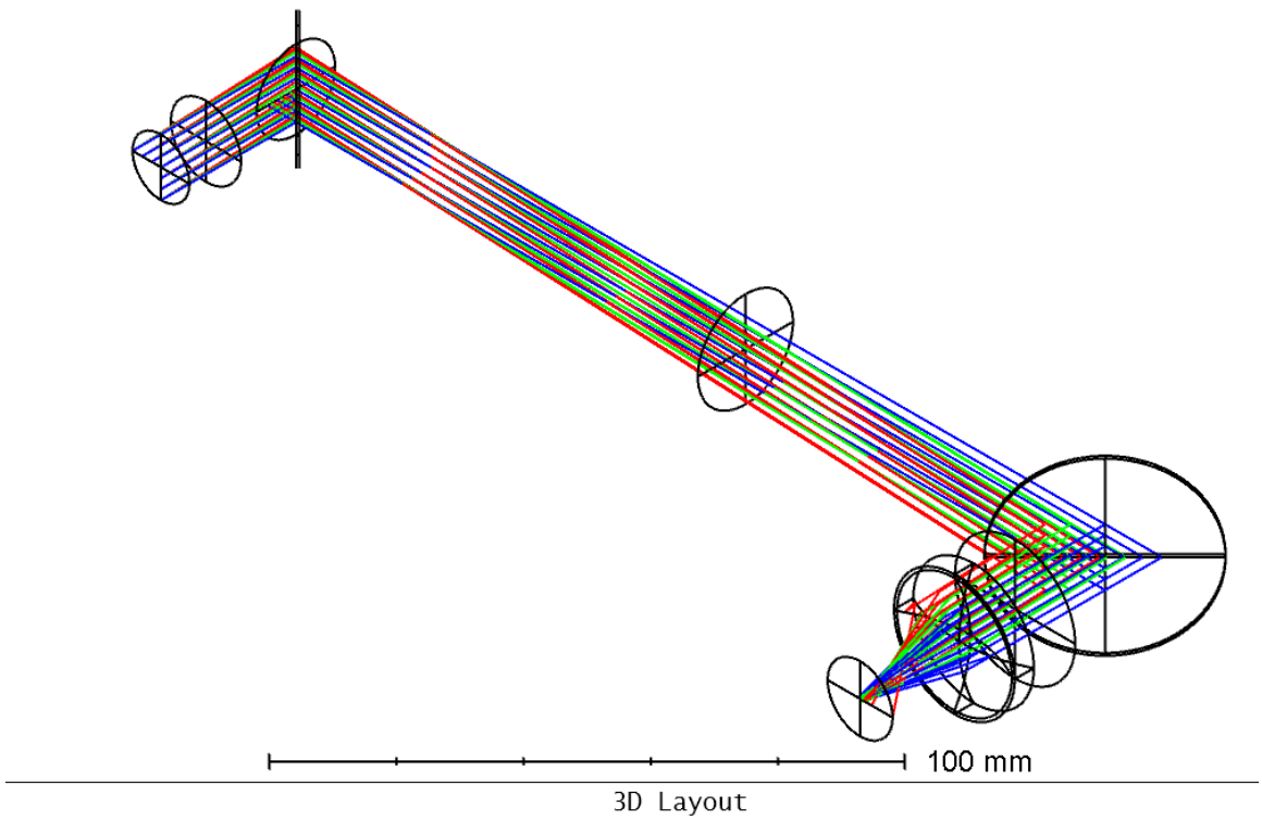
Figure 9.1: 3D model of the optical system in Zemax
