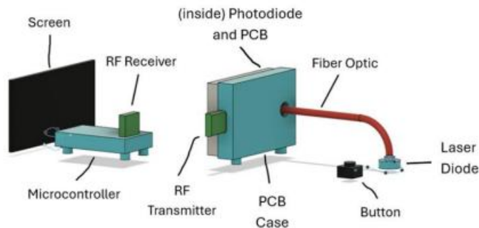
Figure 8.6: Iteration of Optics 1.0
