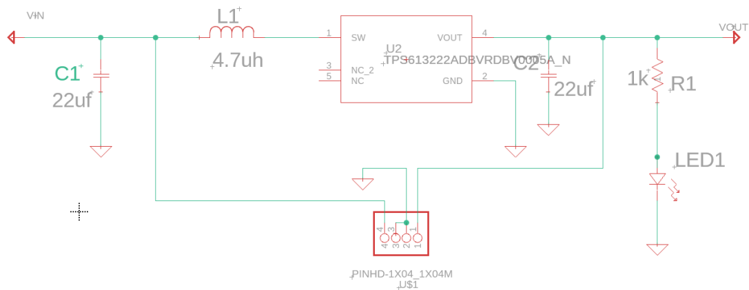
Figure 6.6: 5V Regulator
