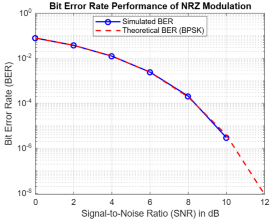
Figure 9.8: Theoretical bit error rate with 10^6 bits with NRZ from code generated by Gemini
