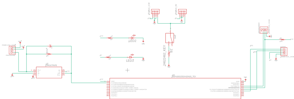
Figure 6.3: Overall Circuit Diagram
