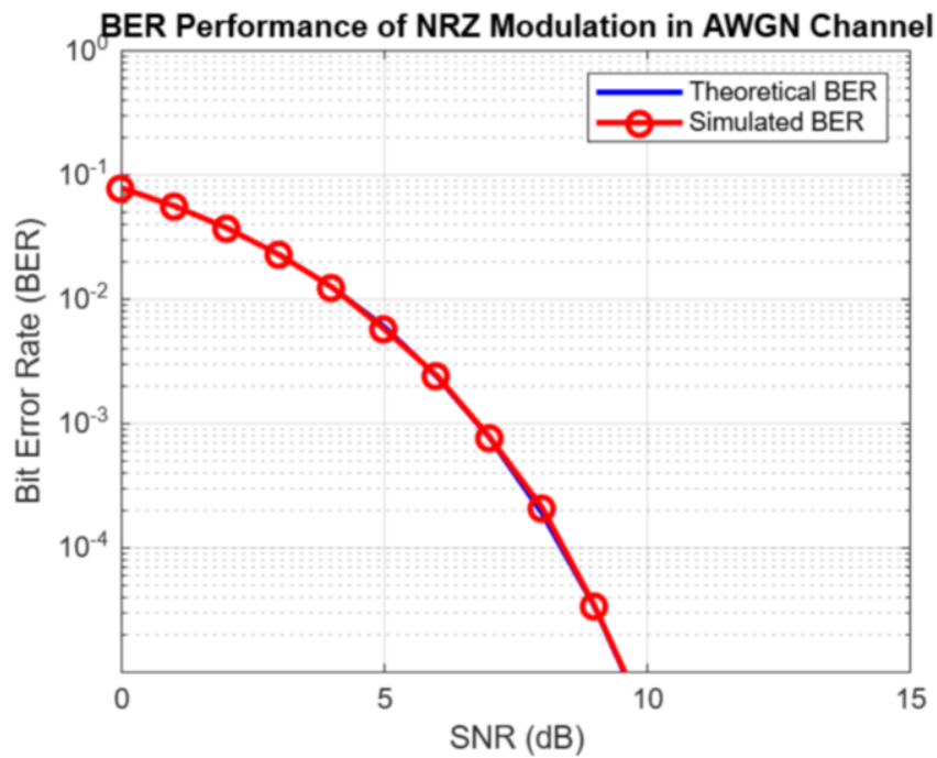
Figure 9.9: Theoretical bit error rate with 10^6 bits with NRZ from code generated by Claude AI
