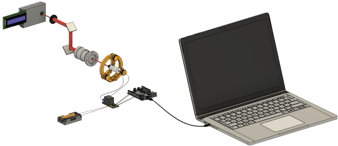
Figure 8.7: Iteration of Optics 2.0
