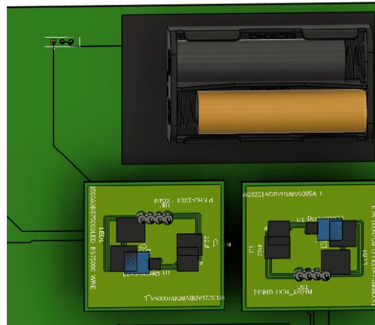
Figure 6.23: Battery Pack and regulators for PCB
