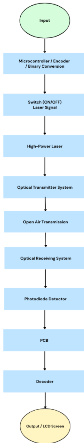
Figure 7.1: Software Flowchart
