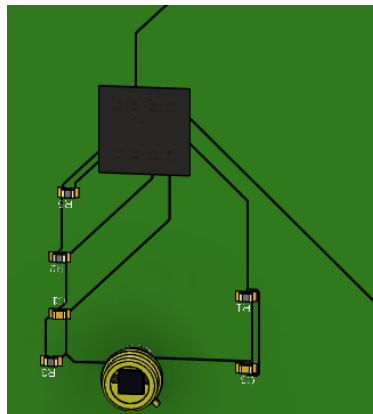
Figure 6.19: Photodiode and Transimpedance Circuit
