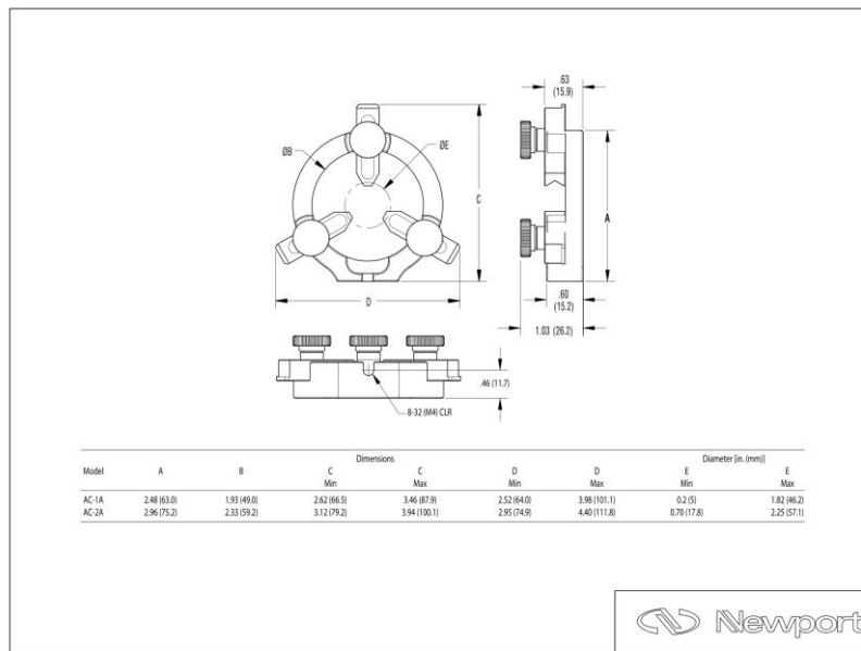
Figure 6.16: Dimensions of AC-2A
