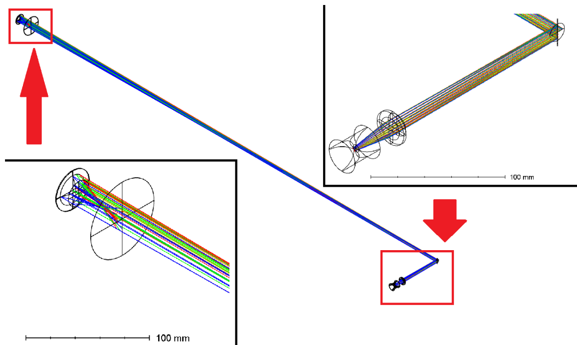
Figure 9.4: Approximate 3D model of the optical system with the beam expander (top right) and focusing lens (bottom left)
