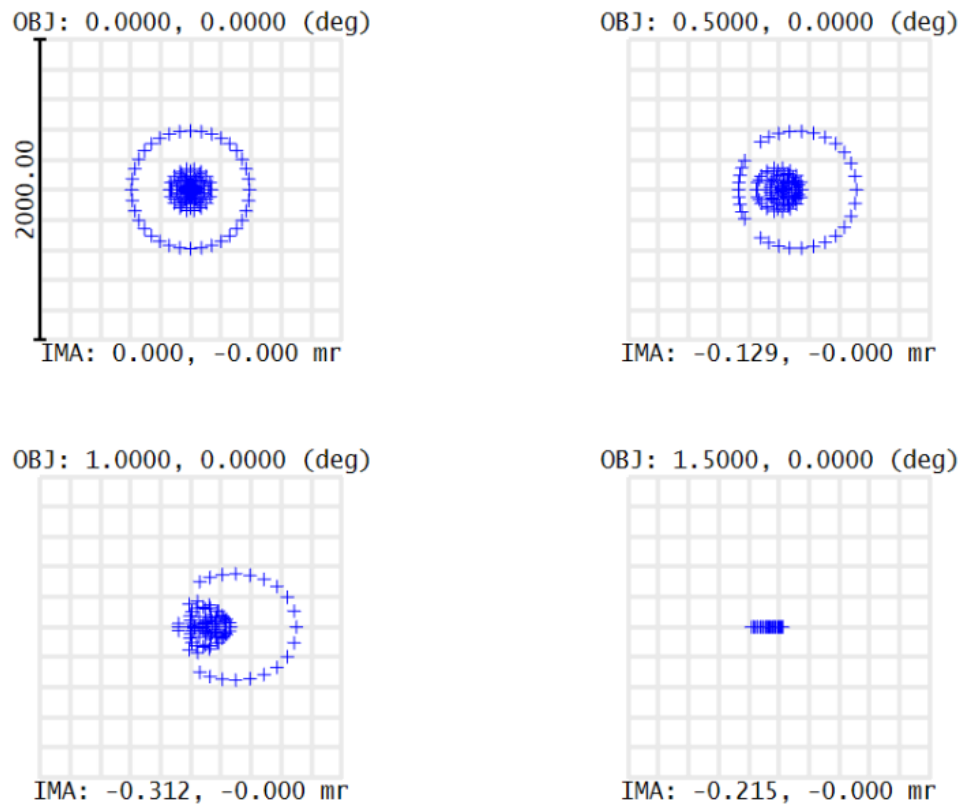
Figure 9.5: Spot diagram of the optical system at different angles
