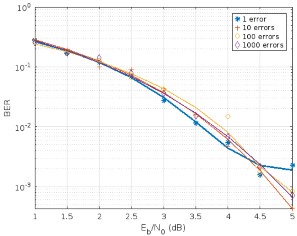
Figure 9.7: Theoretical bit error rate plot from 1 error to 1000 errors with 10^6 bits with BPSK
