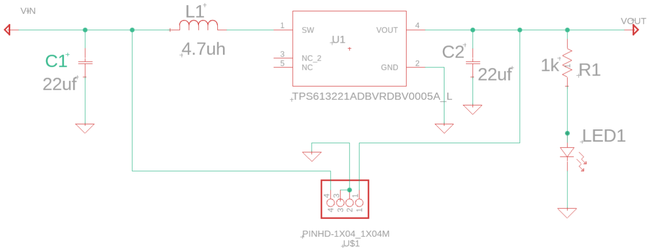
Figure 6.5: 3.3V Regulator
