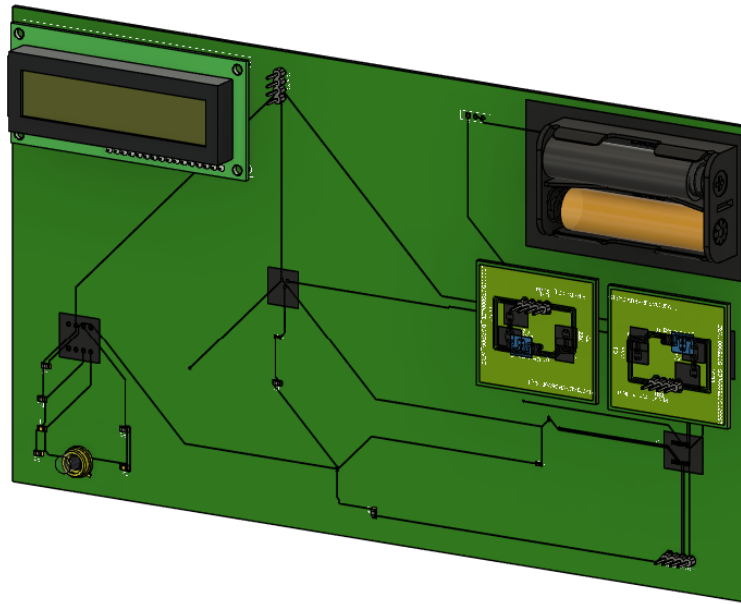
Figure 6.18: Entire PCB
