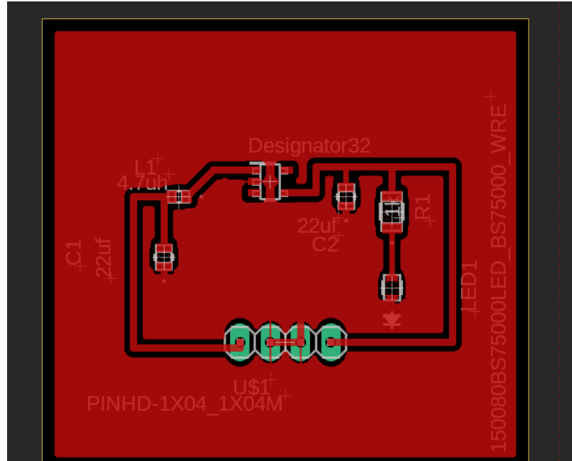
Figure 8.2: 5V regulator design
