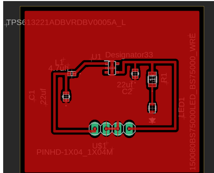
Figure 8.1: 3.3V regulator design
