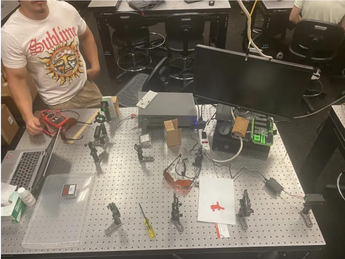
Figure 8.9: Final optical demo setup with lens tube to eliminate back reflections (toward the left side)
