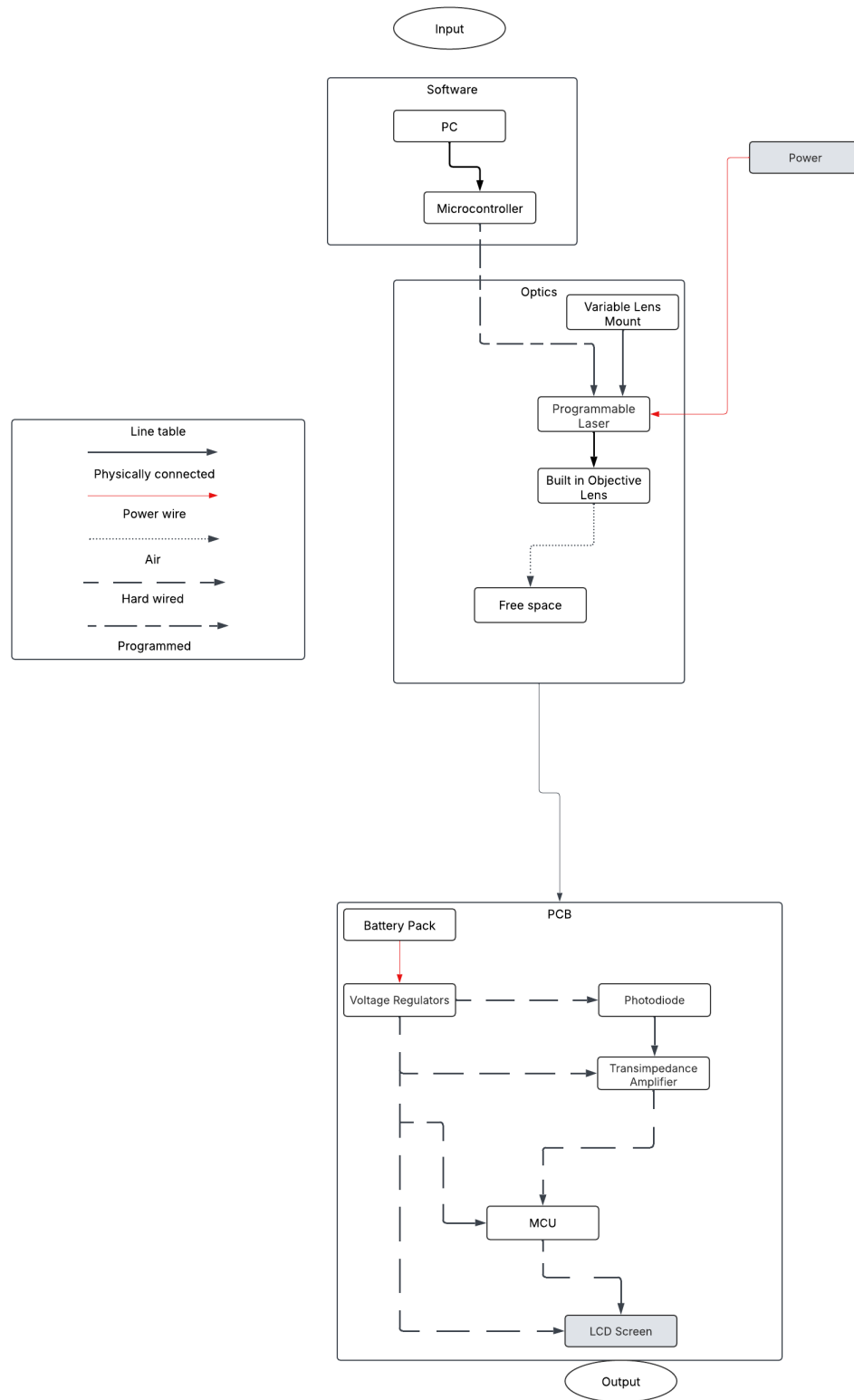
Figure 6.2: Block Diagram
