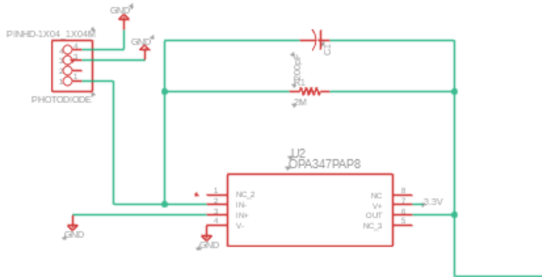
Figure 6.7: Photodiode Circuit
