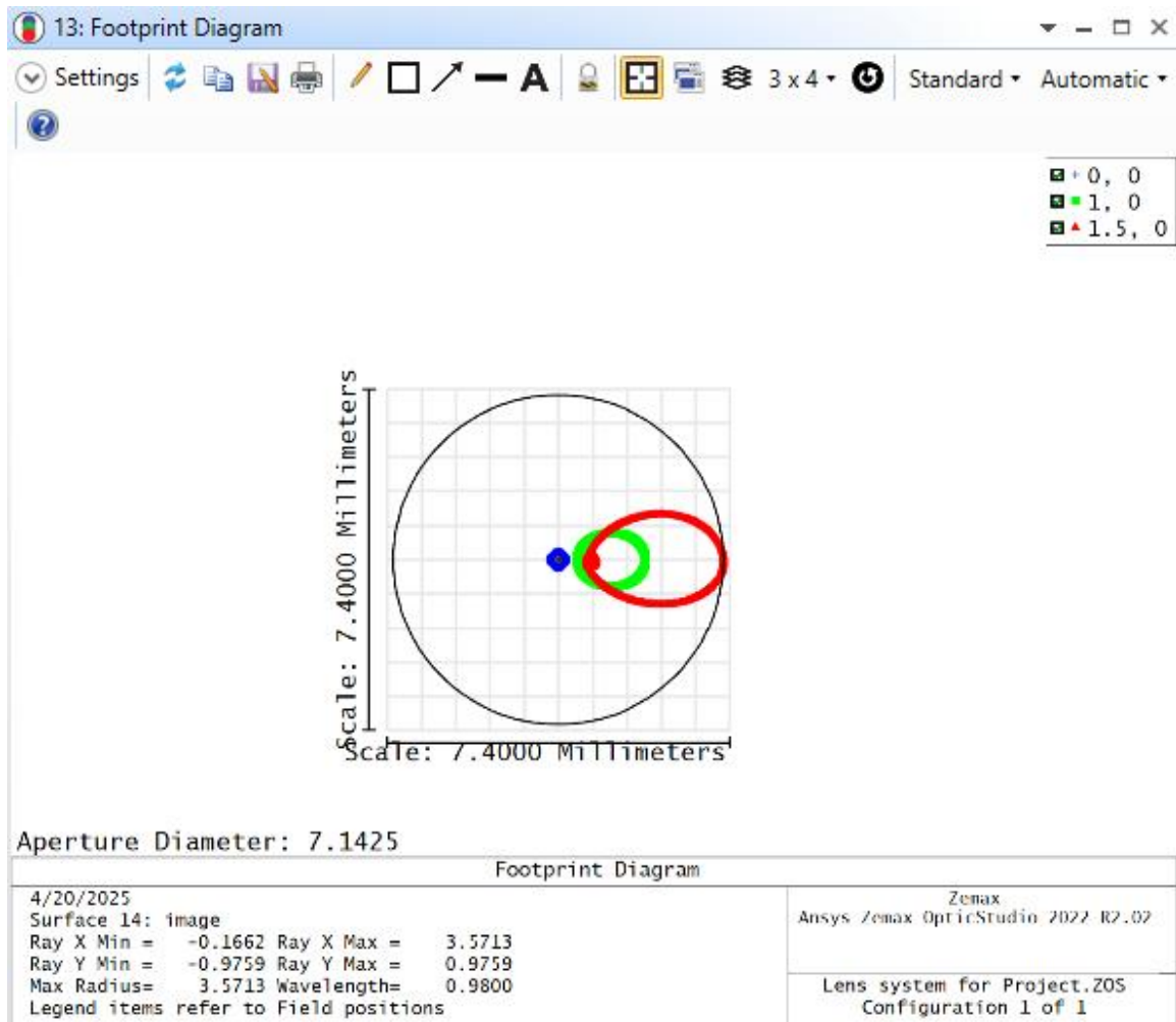
Figure 9.2: A footprint diagram of the optical system with off-axis patterns
