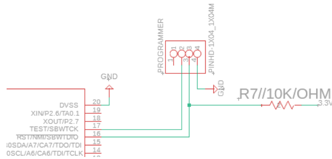
Figure 6.9: Four-pin programmer
