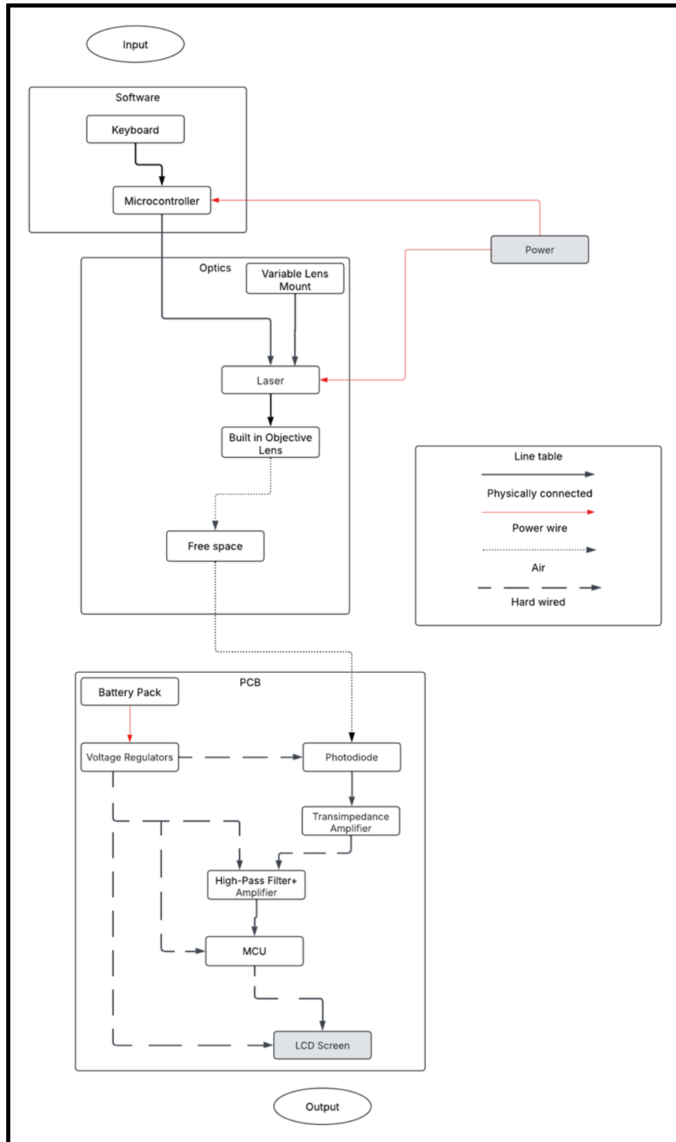
Figure 2.1: Hardware Block Diagram
