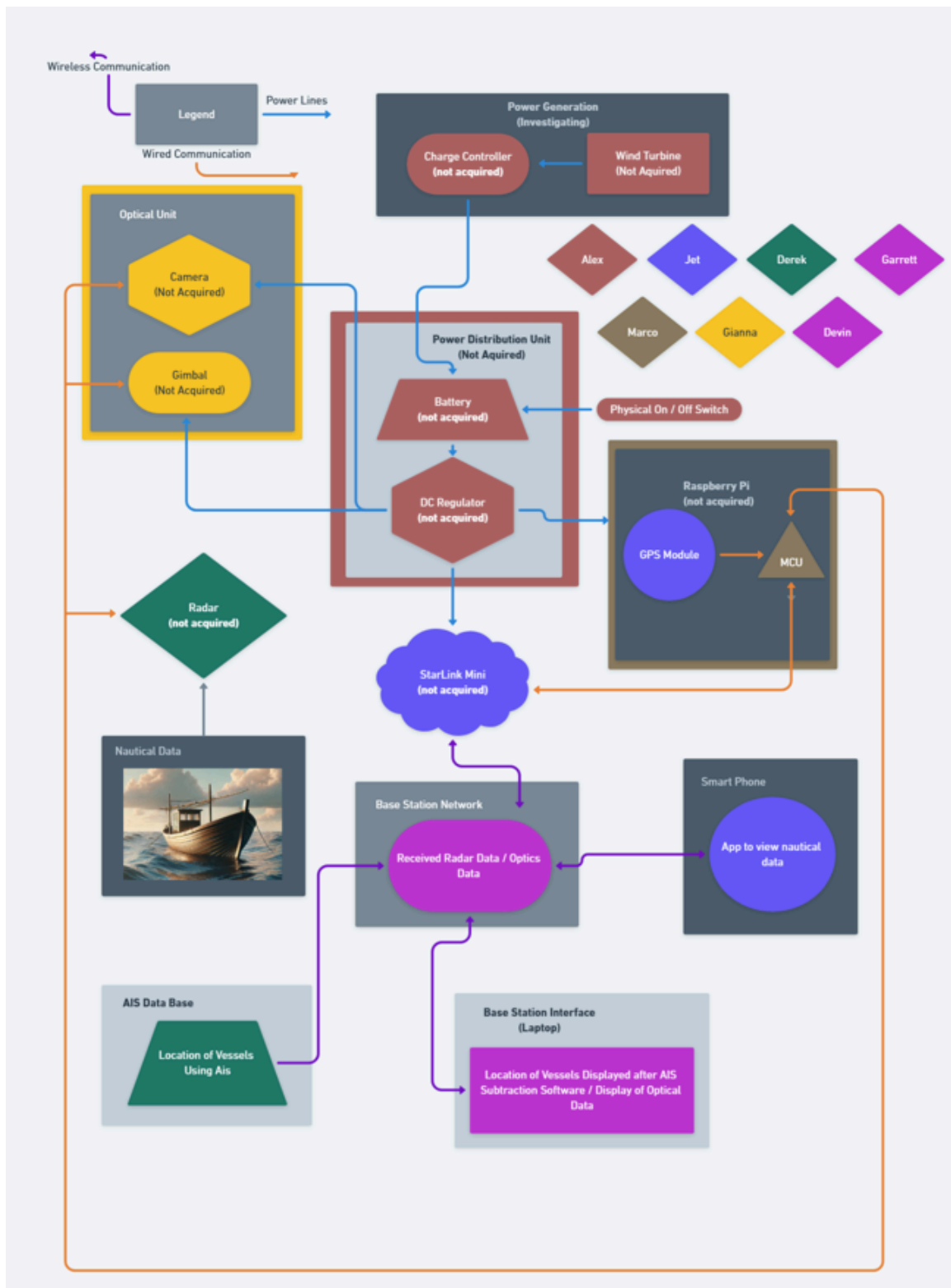
Figure 2.1 - Hardware block diagram [1]
