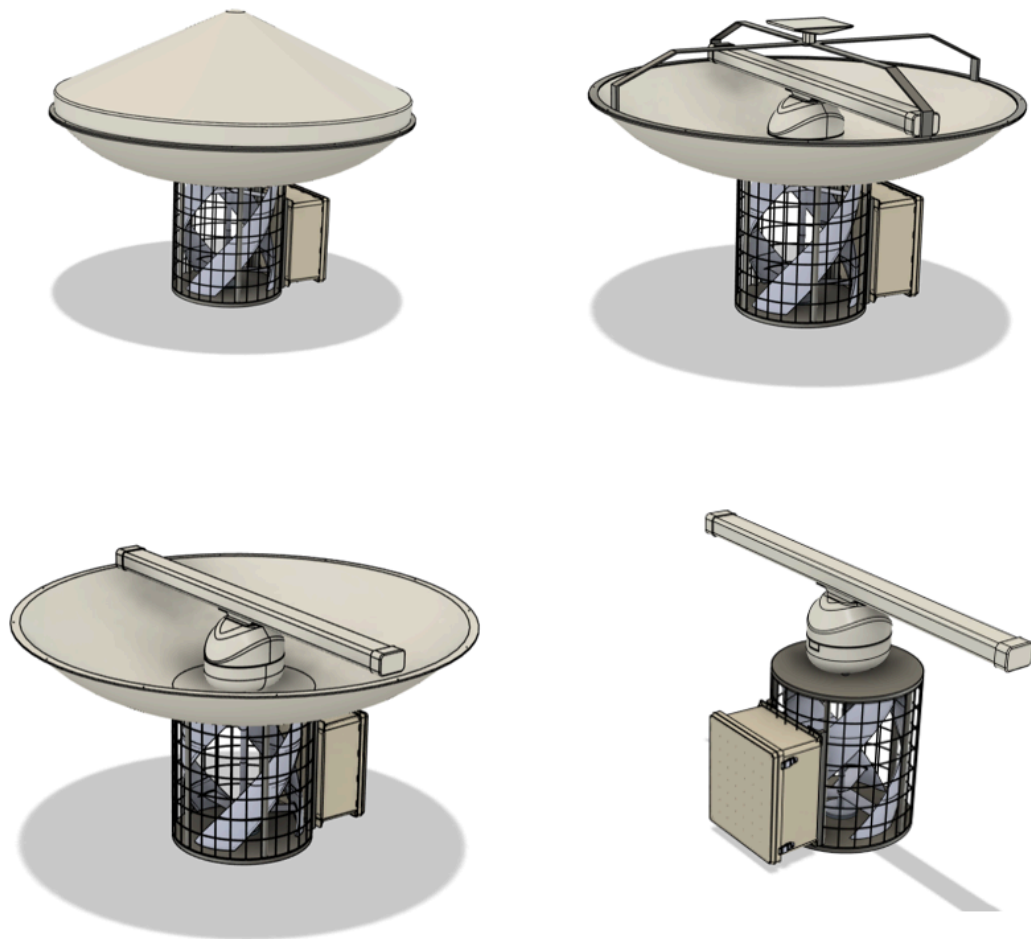
Figure 2.5 - MDAS Prototype CAD [93]
