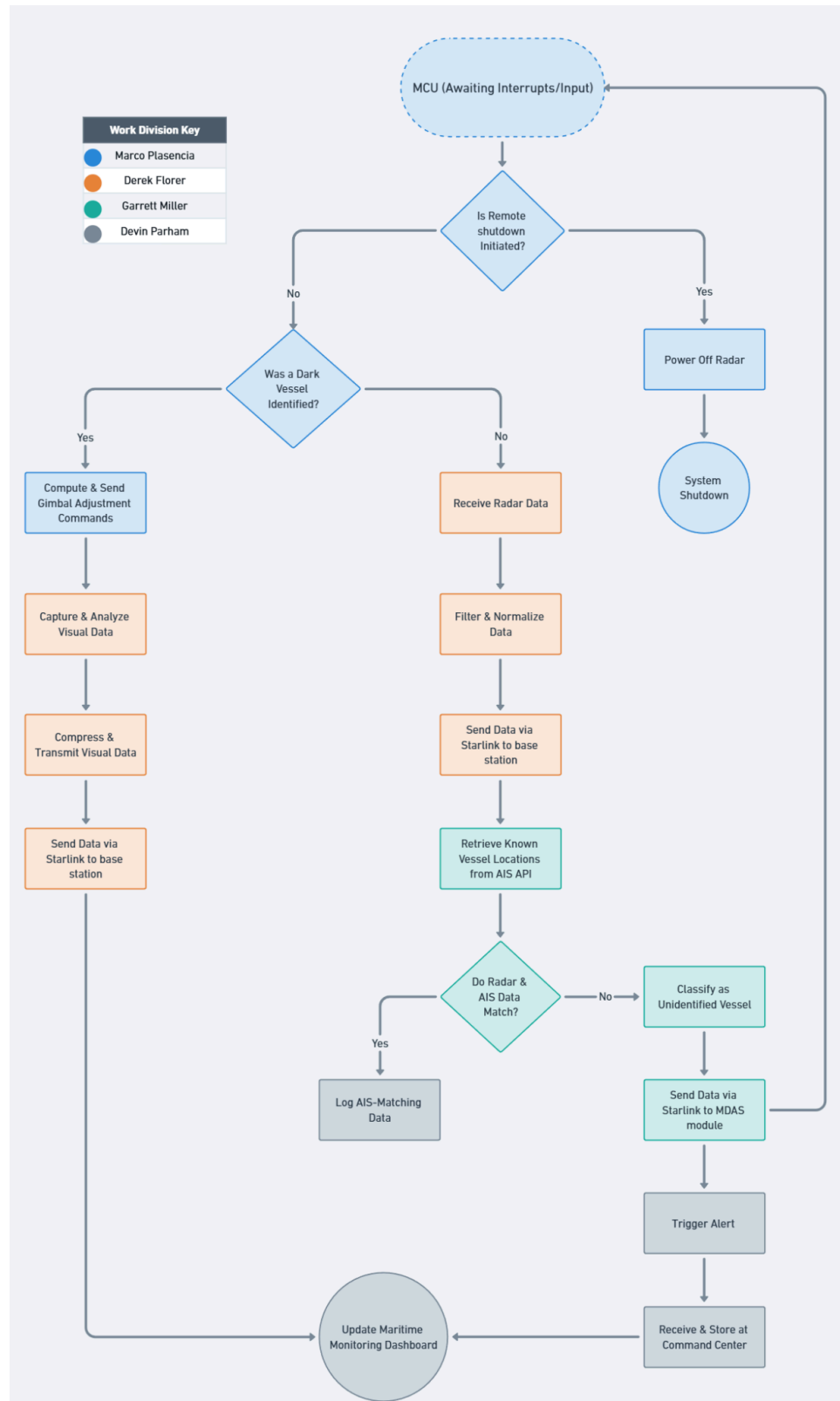
Figure 2.2 - Software block diagram [1]
