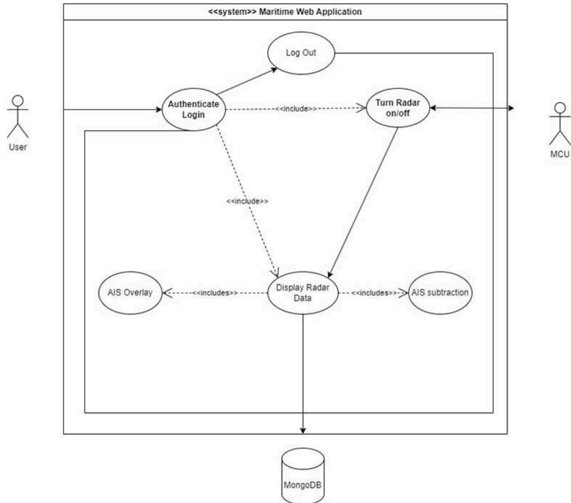
Figure X.X - Use Case Diagram for XXXX
