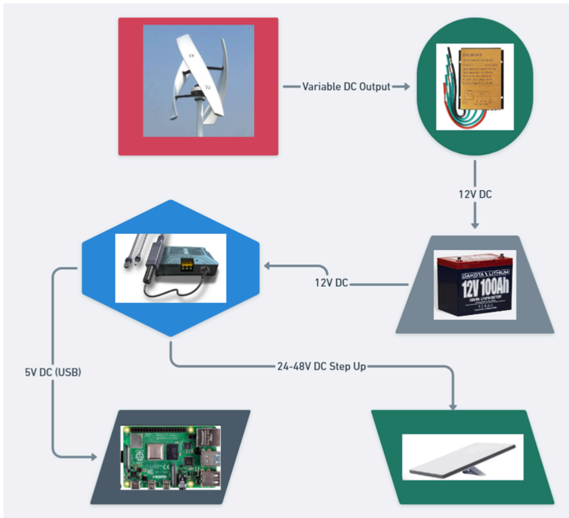
Figure 6.1 - Power System to deliver DC Voltage to the Pi MCU and Starlink Mini Terminal
