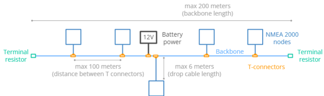
Figure: NMEA 2000 Network Topology
