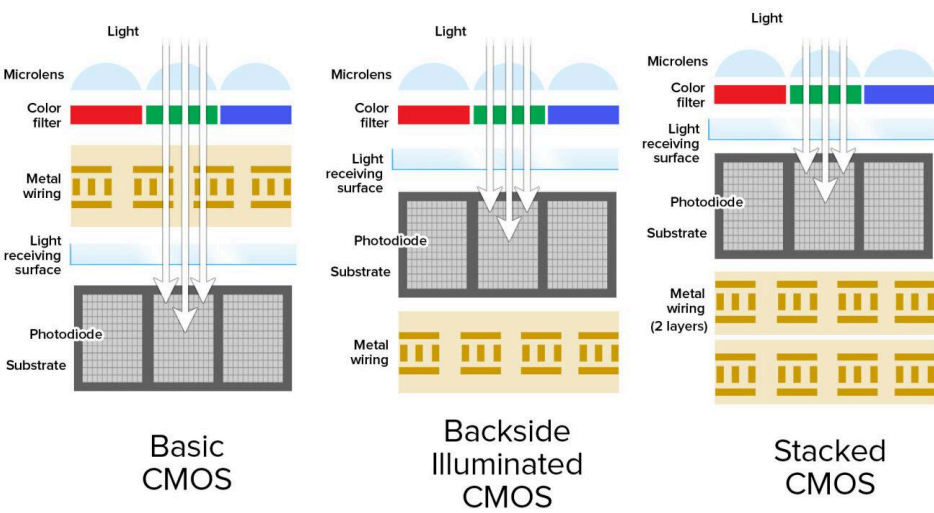
Front v back illumination v stacked (68)
