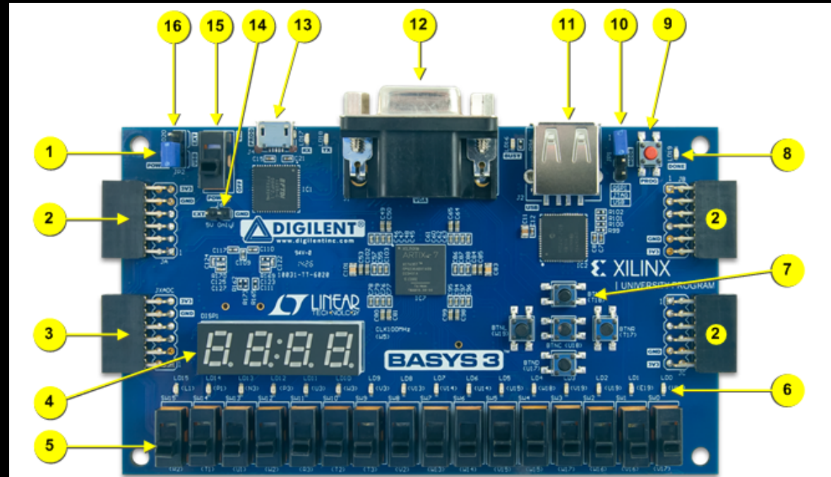
Figure 1. Basys3 board features
