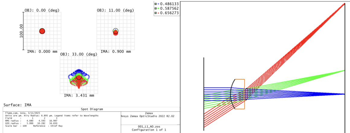
Figure 13. Optimized Imaging System Lens Radius
