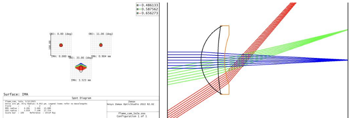
Figure 15. Lateral Color and Coma Correction Results
