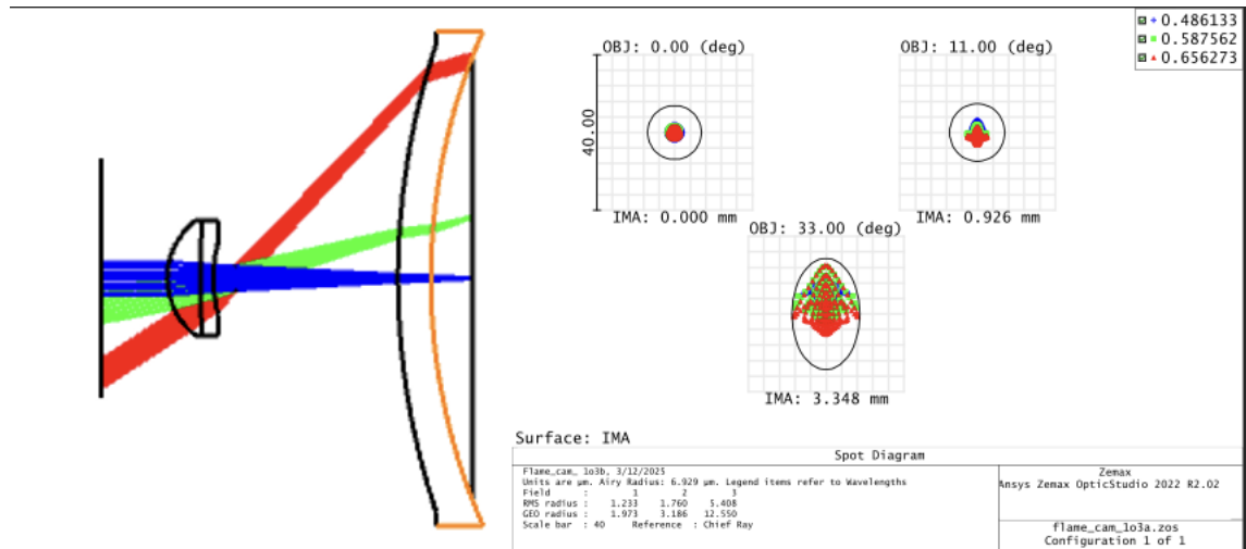
Figure 16. Finalized Simulated Imaging System
