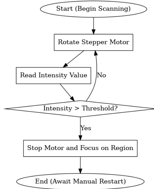
Figure 27. System Software Motor Positioning Diagram
