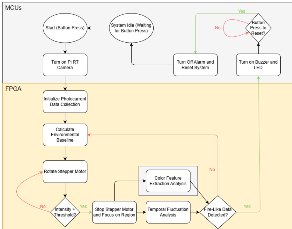
Figure 3. Software Flowchart by Authors
