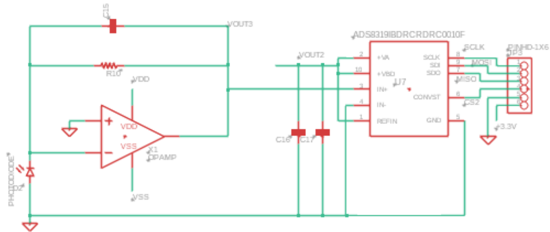
Figure 22. Optoelectronics Subsystem
