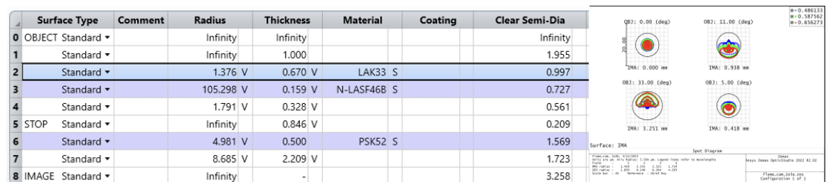
Figure 17. Imaging System Prescription and Spot Diagram
