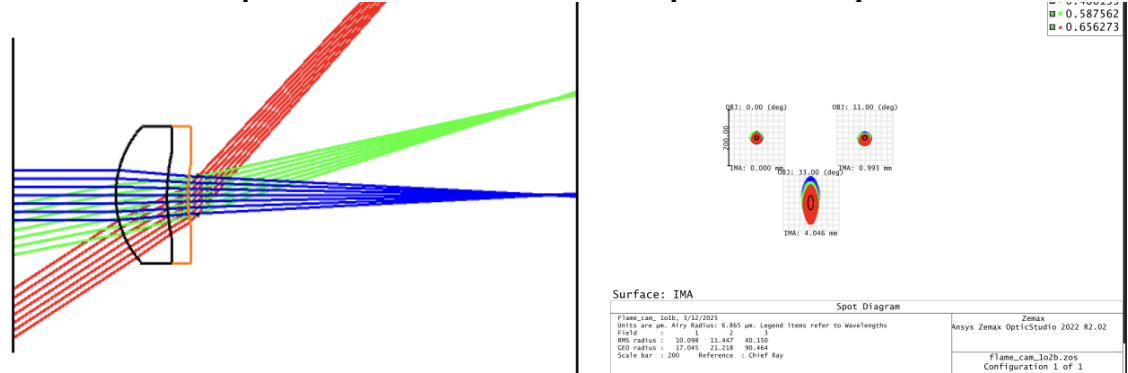
Figure 14. Achromatic Doublet Simulation Results
