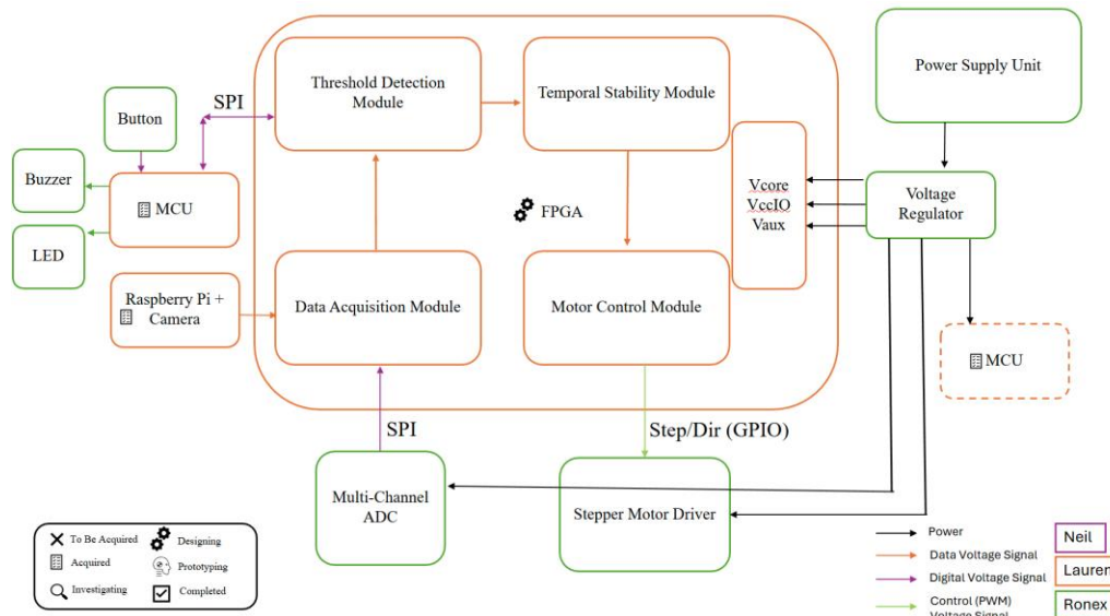
Figure 2. FPGA Hardware Diagram
