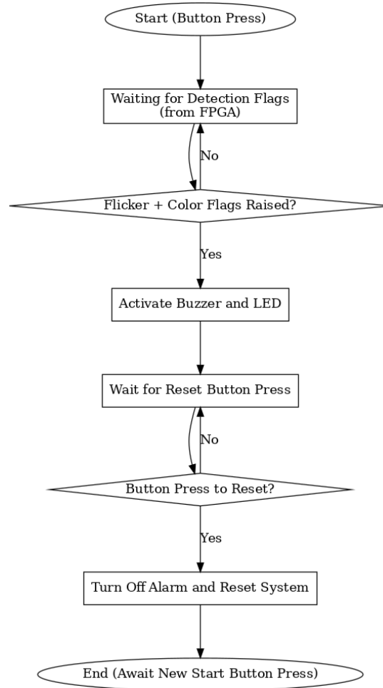
Figure 29. System Software System Response & Notification Handling Diagram
