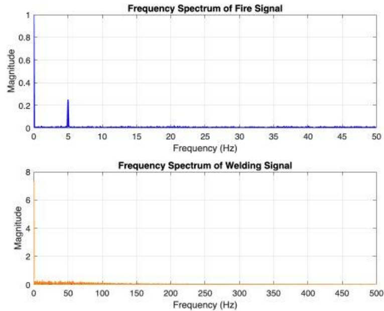
Figure 9. Frequency Domain Representation
