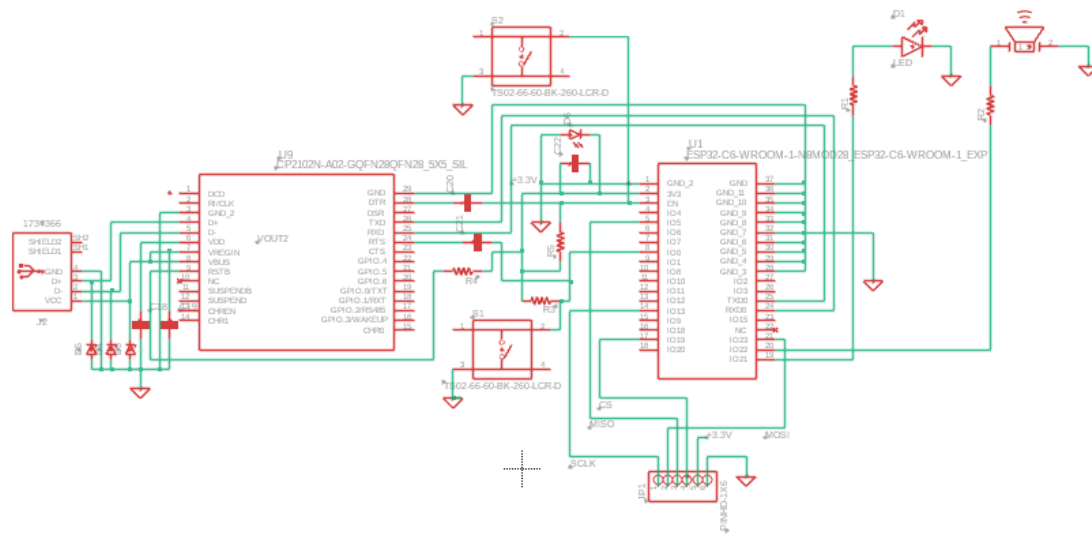
Figure 21. Visual and Audio Alert Feedback System
