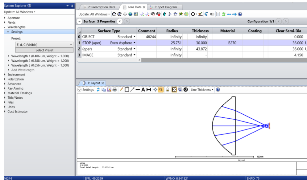
Figure 10. Edmund Optics 46-244 Aspheric Condenser Zemax Simulation
