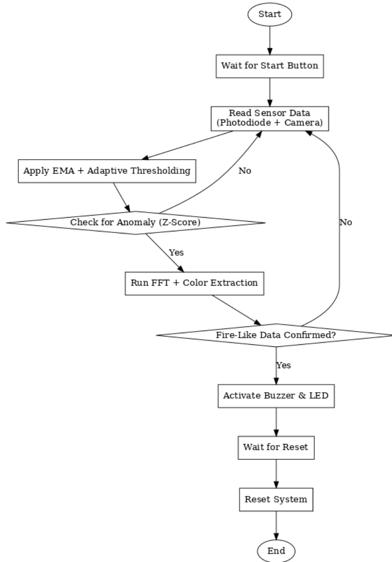
Figure 25. System Software Activity Diagram
