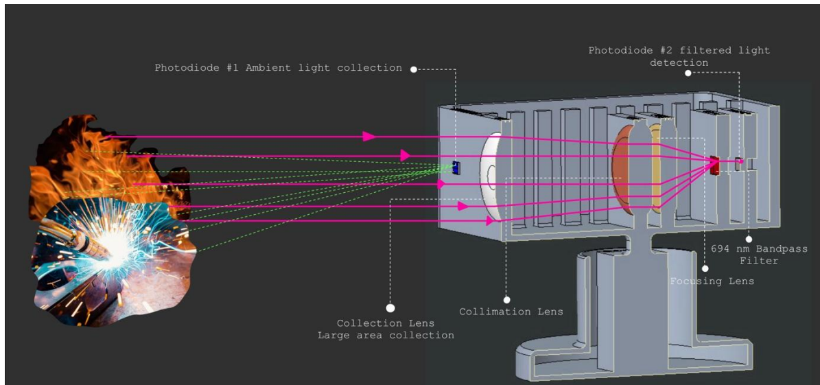
Figure 6. Ray Interaction at Lens Surface
