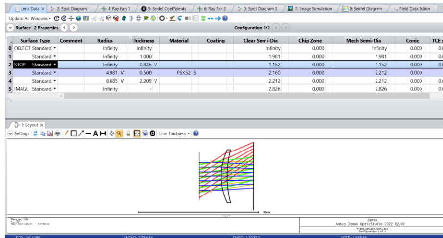
Figure 19. Effective Focal Length Due to 2nd Element
