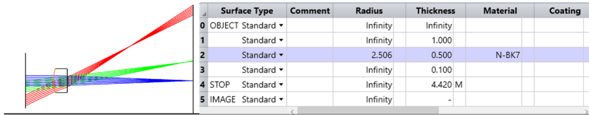
Figure 12. Flame Camera Initial Simulation
