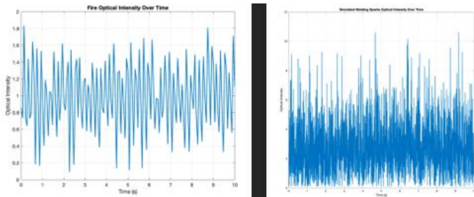
Figure 8. Temporal Characteristics of a Flame Vs. a Spark
