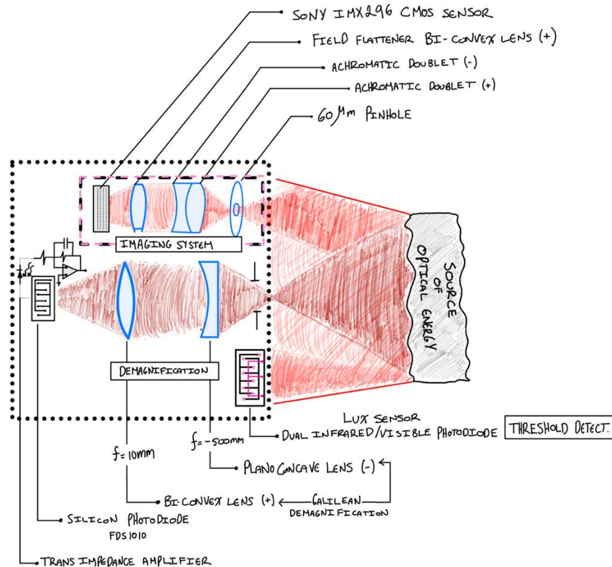
Figure 5. Optical System Schematic
