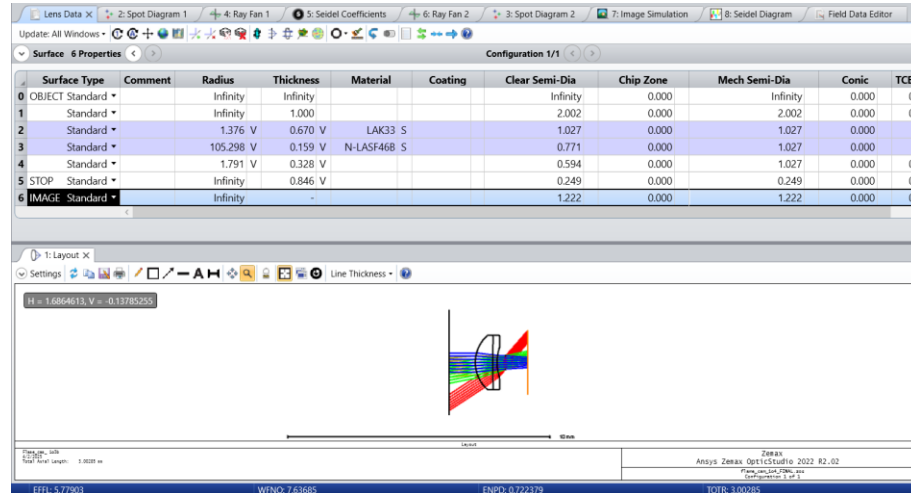
Figure 18. Effective Focal Length Due to 1 st Element
