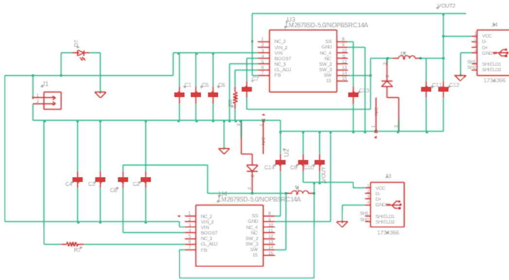
Figure 23. Power Delivery Schematic
