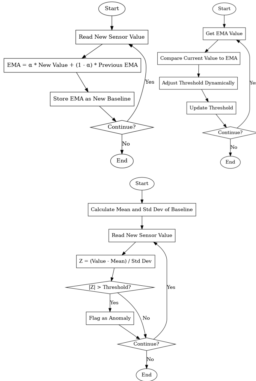
Figure 26. System Software EMA, Adaptive Thresholding, & Z-Score Anomaly Diagrams
