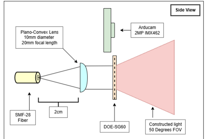
Fig. 1. Collimation Diagram
