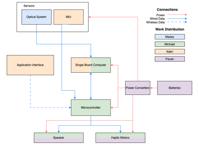
Fig. 2. Hardware Block Diagram
