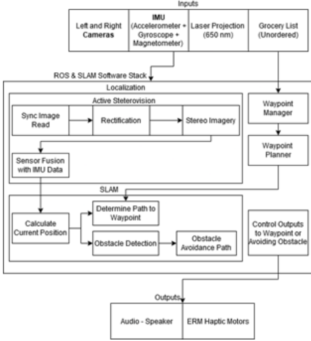
Fig. 3. Software Control Flow Diagram
