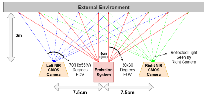
Fig. 4. Optical Components for Active Stereovision
