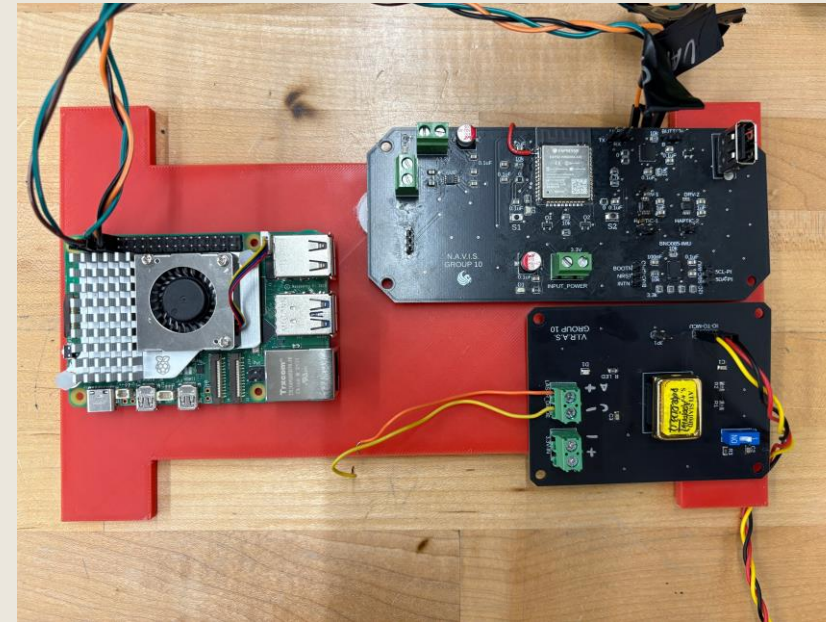
Logic boards assembly
