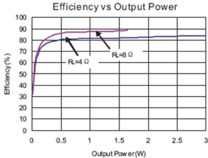
Figure 6.5.2: Efficiency v. Output Power graph of PAM 8403 (Courtesy of Diodes Incorporated)
