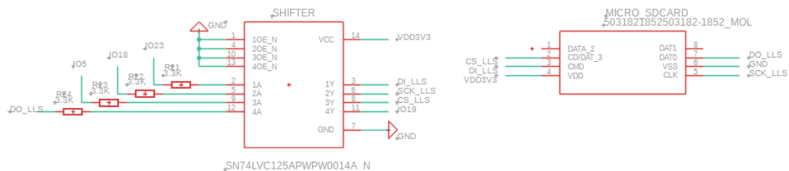
Figure 6.6.1: The schematic of the microSD card reader module
