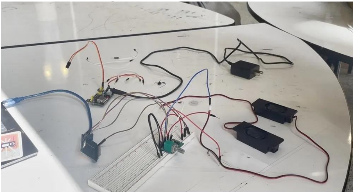
Figure 9.1.3: Prototype of Speaker System with Amplifier
