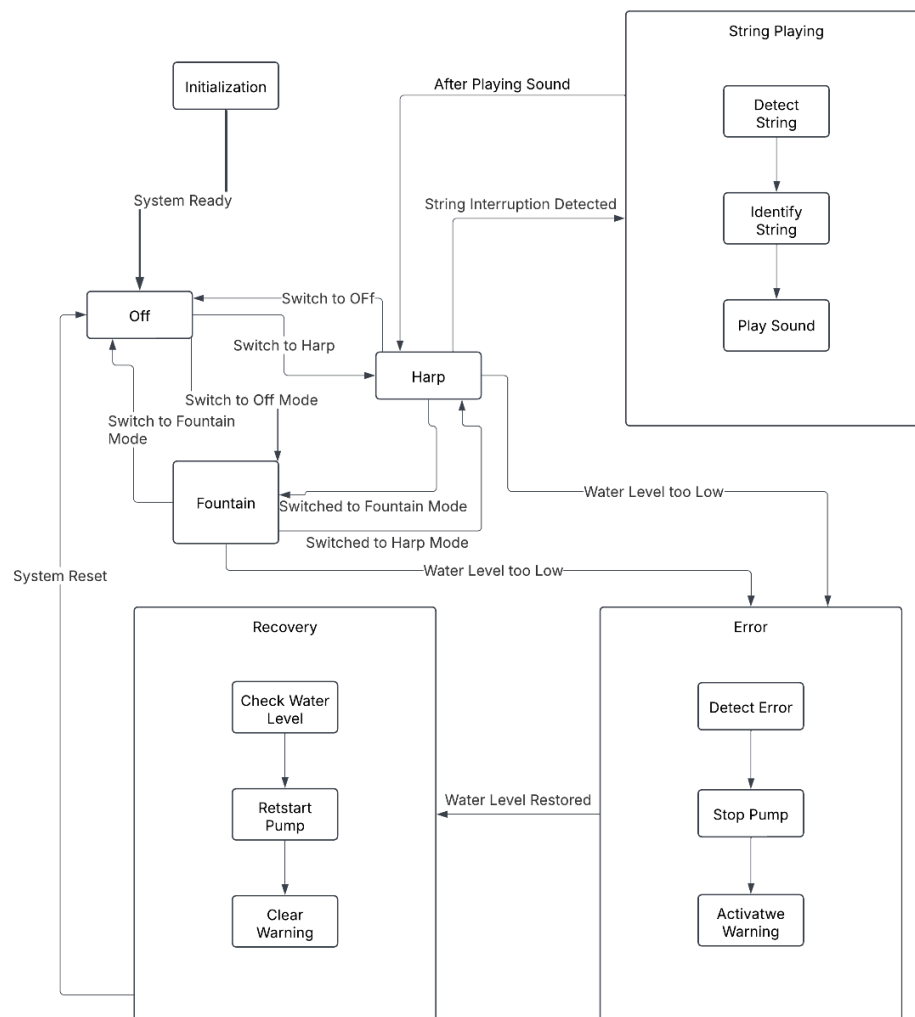
Figure 7.3.1: System State Diagram
