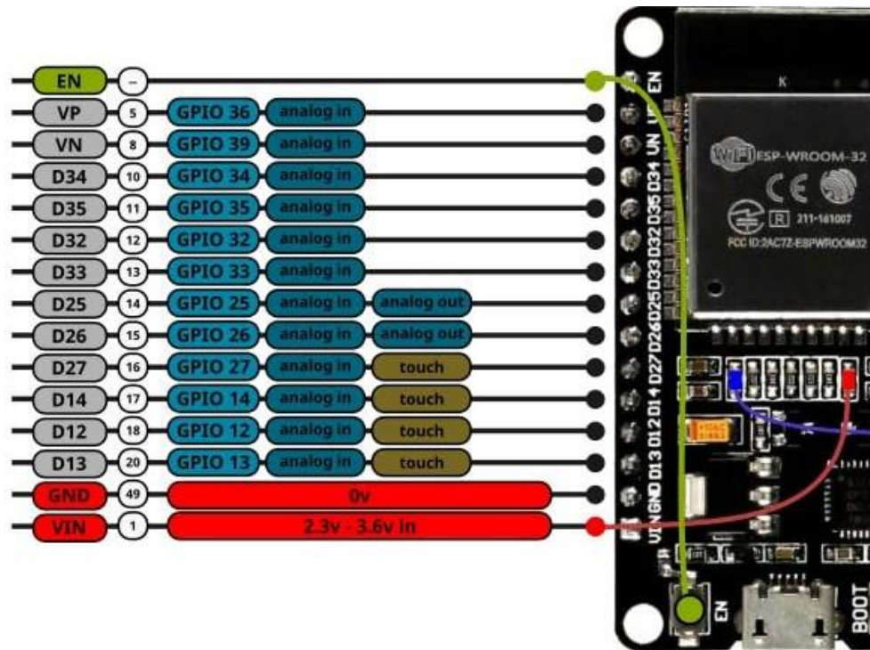
Figure D1: ESP32 WROOM Left Side Pinouts
