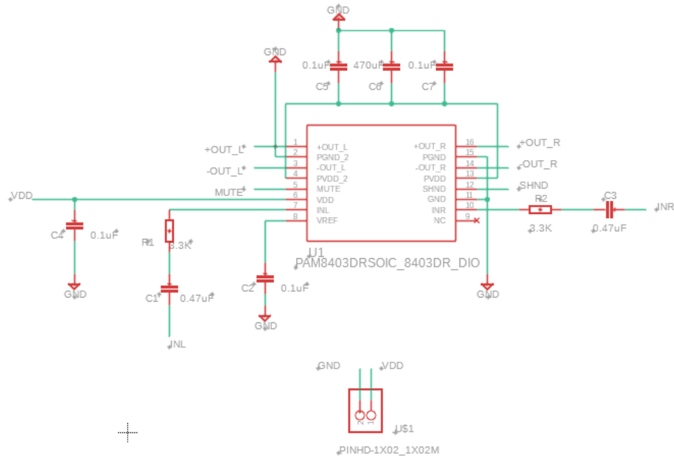
Figure 6.5.1: The schematic of the amplifier module
