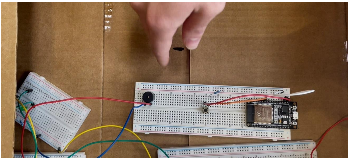
Figure 9.1.2: Prototype of Audio Triggering with Laser-Photodiode System
