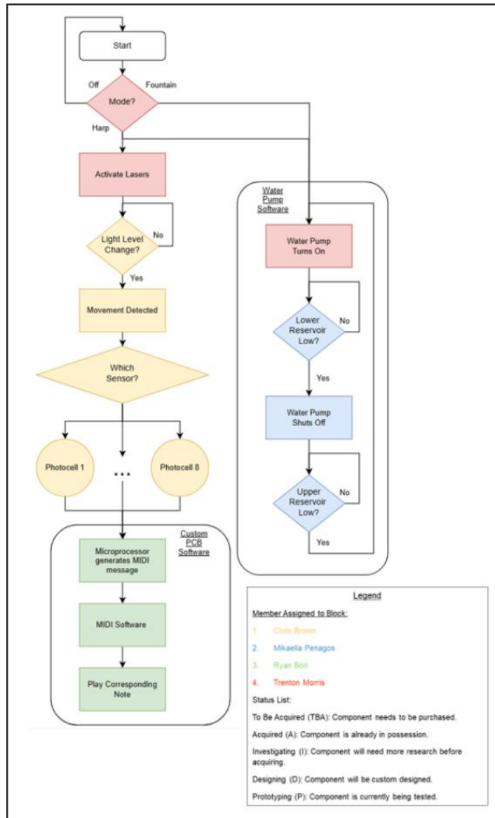
Figure 5.2.2: Example Software Diagram
