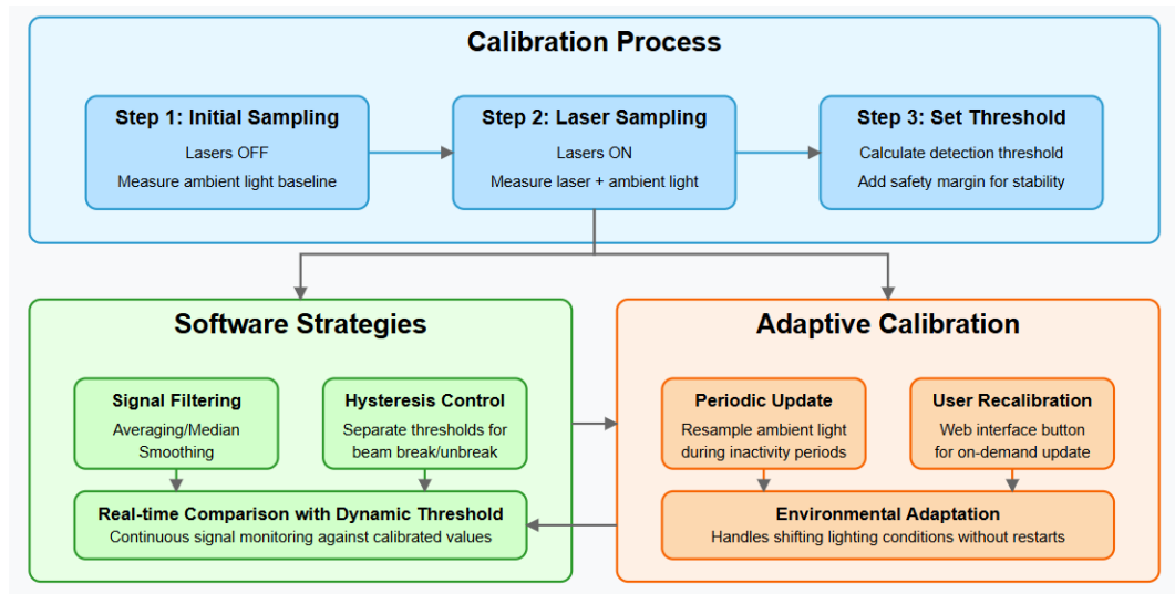
Figure 7.6.3.1: Photodiode Calibration and Ambient Light Compensation
