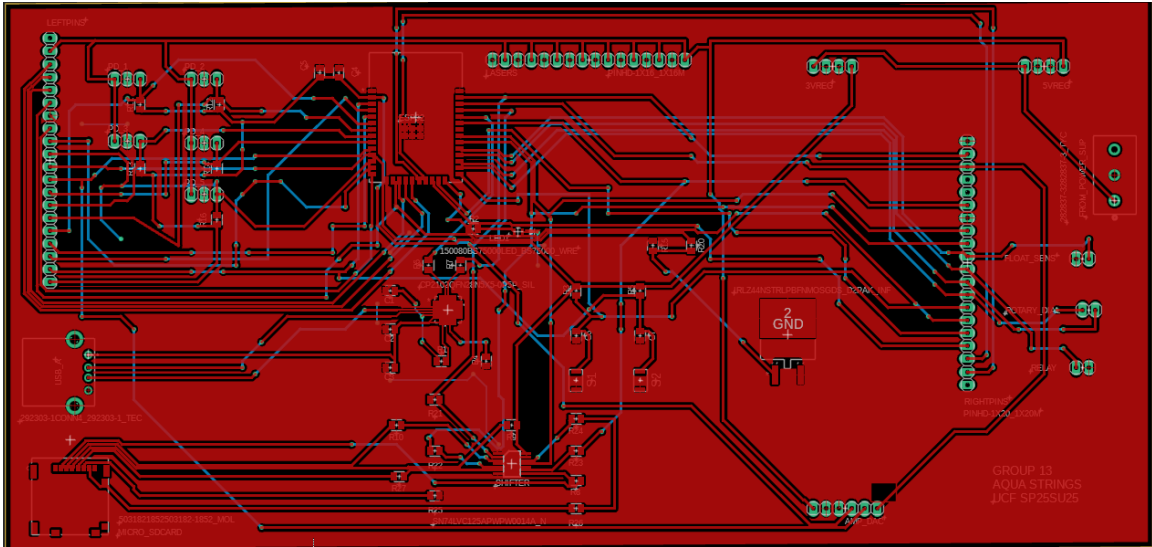
Figure 8.1.2.1: PCB Design of Microcontroller Board
