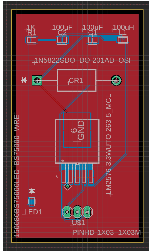
Figure 8.1.1.1: PCB Design of Voltage Regulator (identical for both 3.3V and 5V
