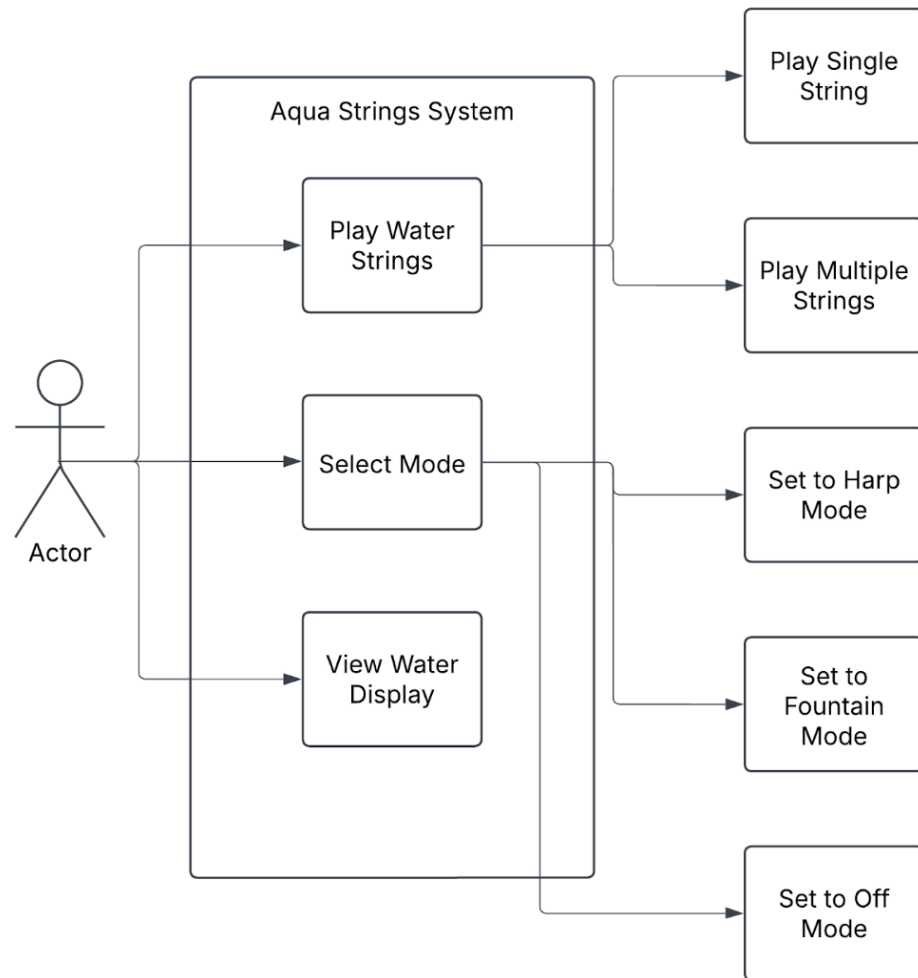
Figure 7.2.1: Use Case Diagram
