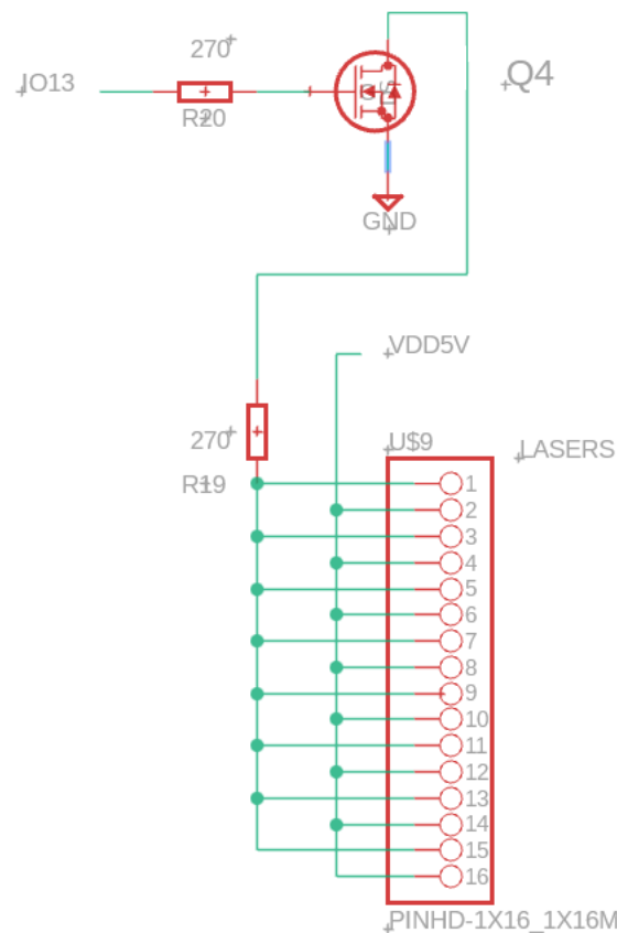
Figure 6.3.1: Laser diode schematic with MOSFET on main board
