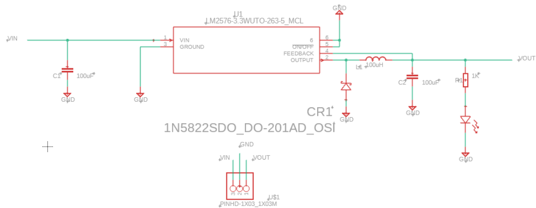
Figure 6.2.2: The schematics of 3.3V and 5V regulator (same design)
