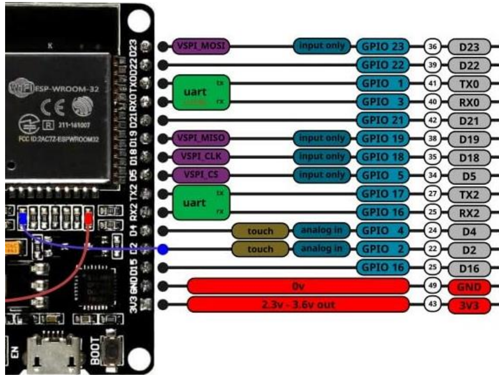
Figure D2: ESP32 WROOM Right Side Pinouts
