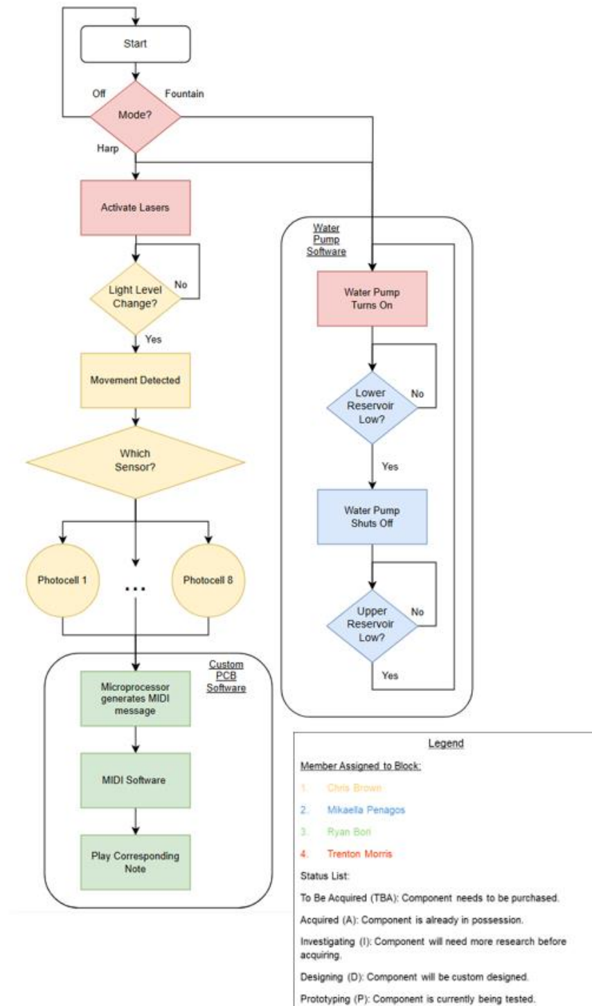
Figure 2.8.1: Software Block Diagram
