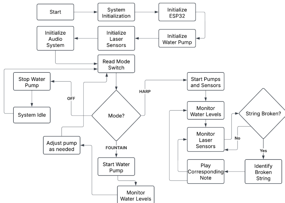
Figure 7.1.1: Main Program Block Diagram
