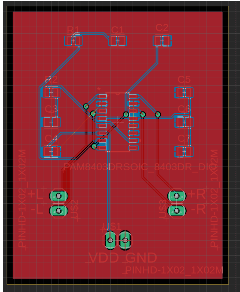
Figure 8.1.3.1: PCB Design of Audio Amplifier Board
