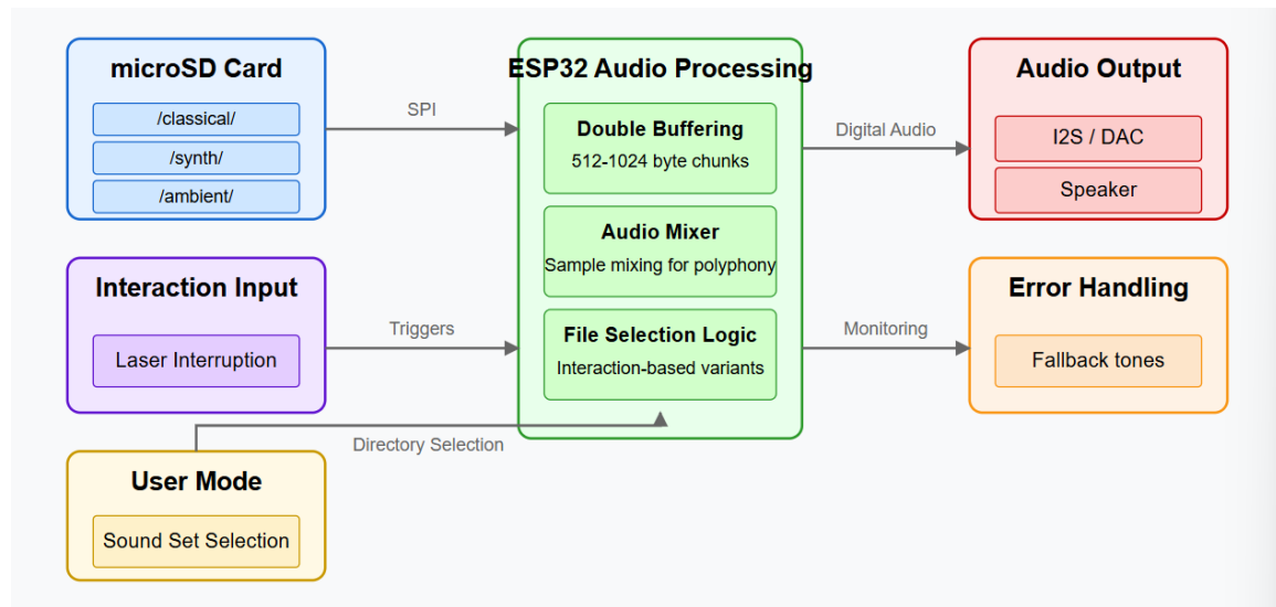
Figure 7.5.1.1: SD Card Audio System Architecture
