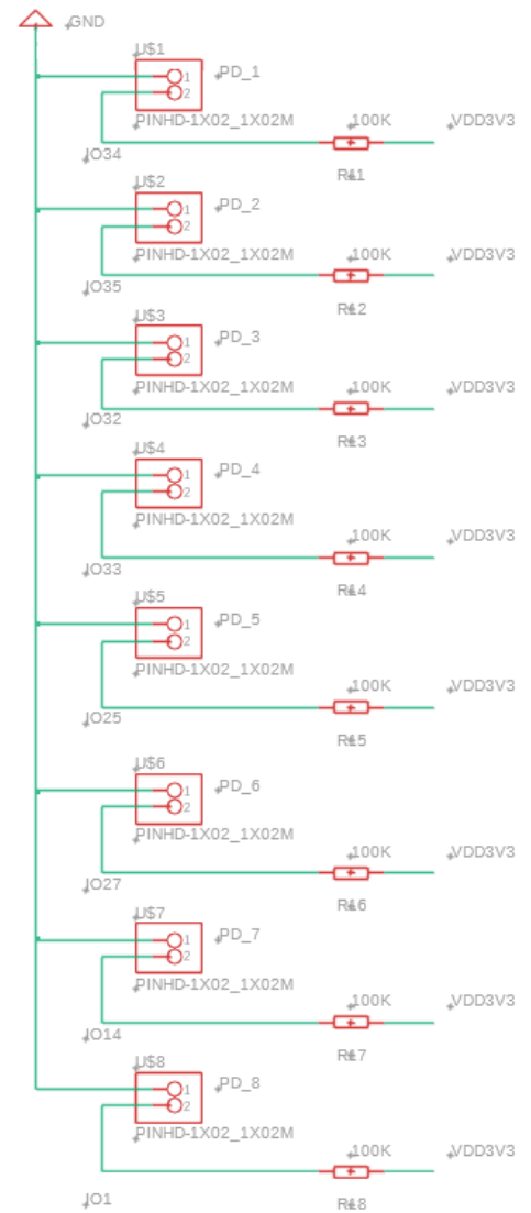
Figure 6.3.2: Photodiode schematic on main board
