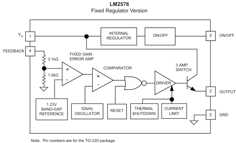
Figure 6.2.1: Internal schematic of the LM2576 regulator
